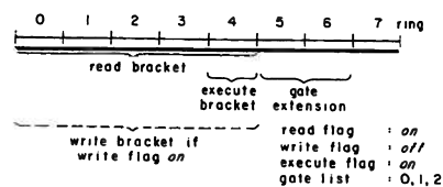
Fig. 2. Example access indicators for a pure procedure segment which contains gates.
