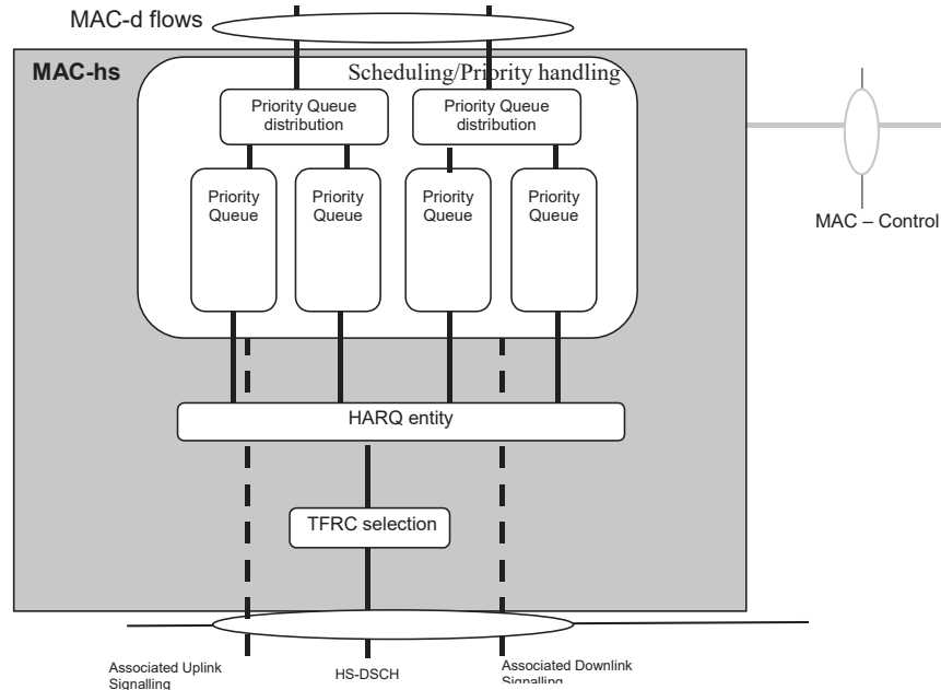
Figure 4.2.4.3.1: UTRAN side MAC architecture / MAC-hs details
