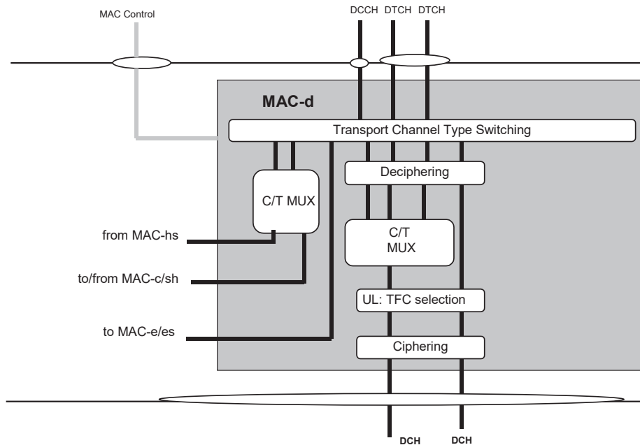
Figure 4.2.3.2.1: UE side MAC architecture / MAC-d details
