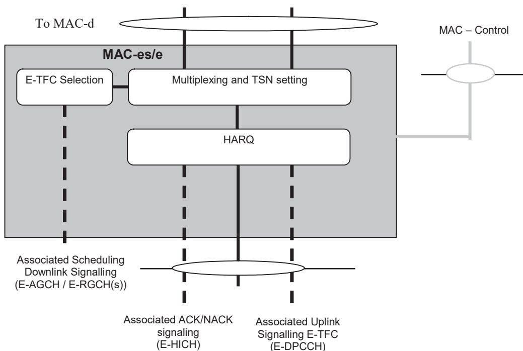
Figure 4.2.3.4.1: UE side MAC architecture / MAC-e/es details
