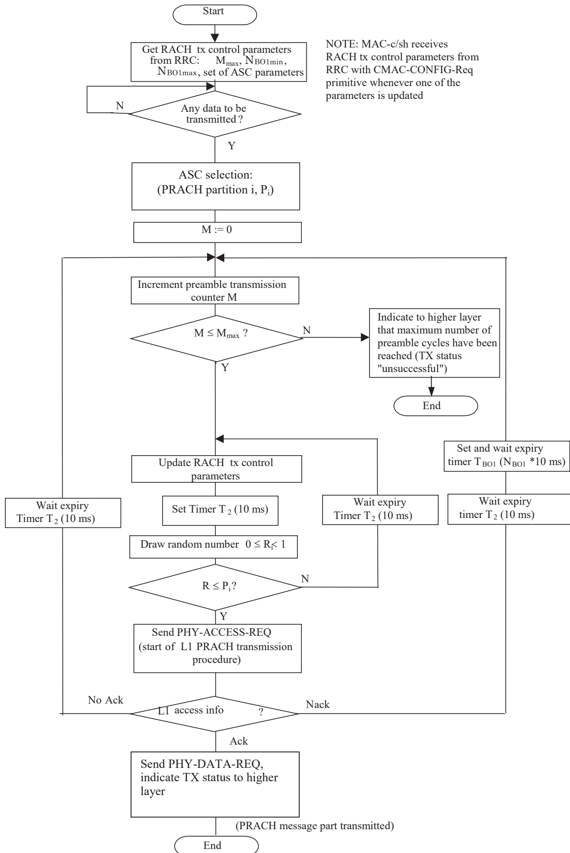
Figure 11.2.2.1: RACH transmission control procedure (UE side, informative)
