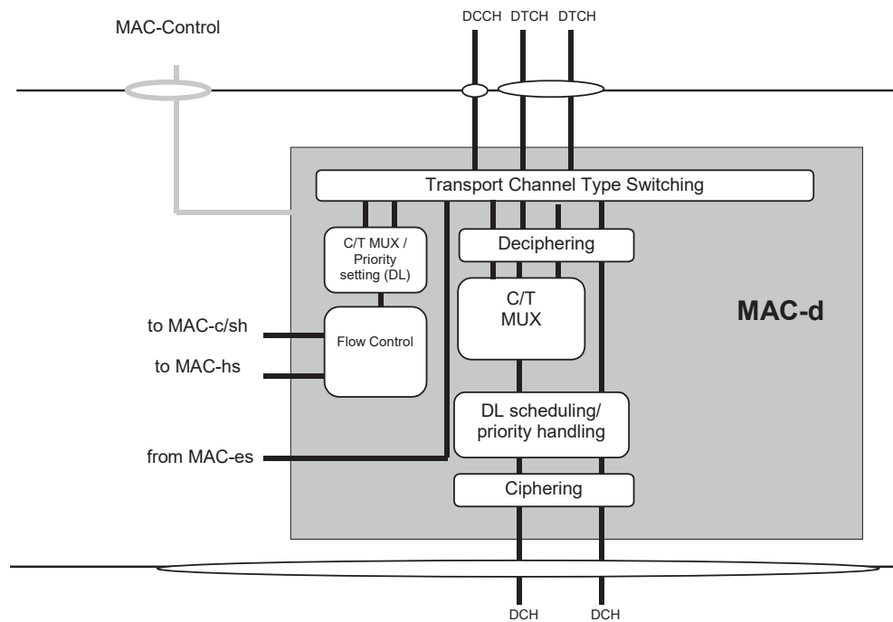
Figure 4.2.4.2.1: UTRAN side MAC architecture / MAC-d details
