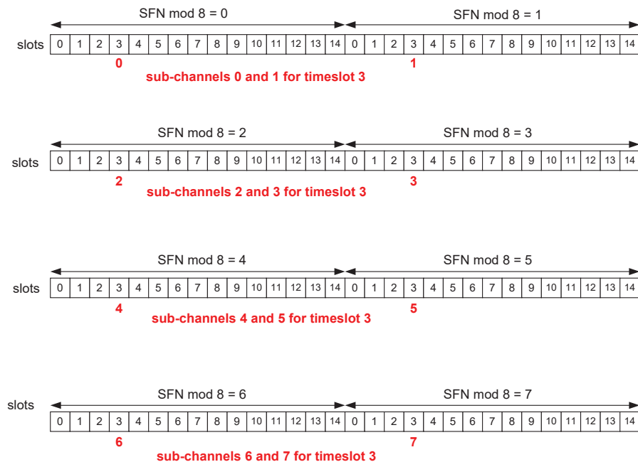
Figure 11.2.3.1 Eight sub-channels for timeslot 3
