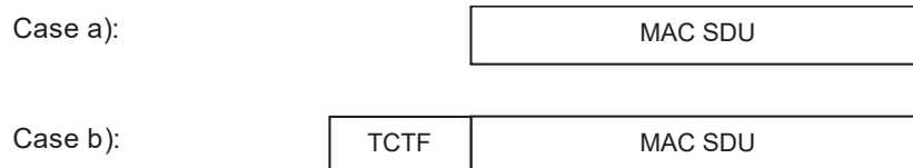
Figure 9.2.1.7.1: MAC PDU format for MCCH
