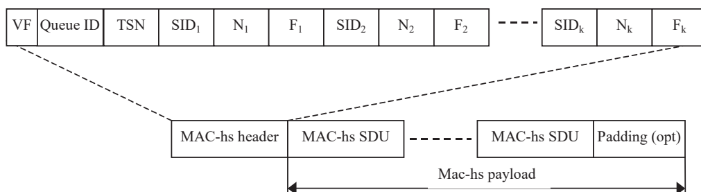
Figure 9.1.4.1: MAC-hs PDU
