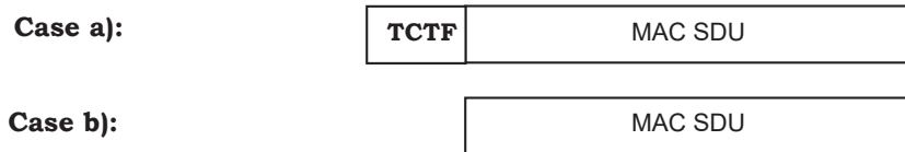
Figure 9.2.1.6.1: MAC PDU format for SHCCH
