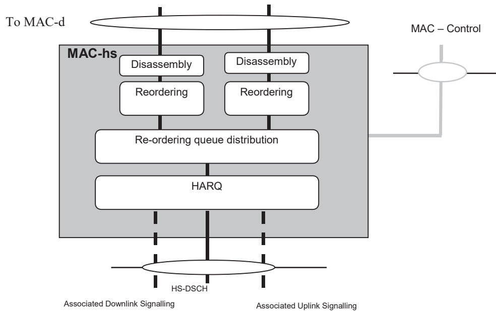
Figure 4.2.3.3.1: UE side MAC architecture / MAC-hs details
