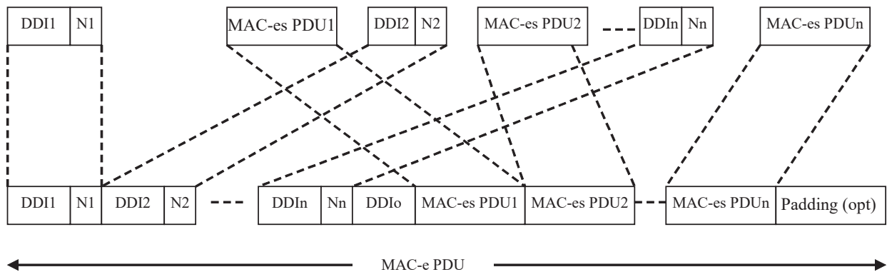
Figure 9.1.5.2: MAC-e PDU
