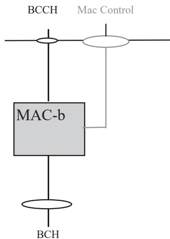
Figure 4.2.2.1: UE side and UTRAN side architecture
