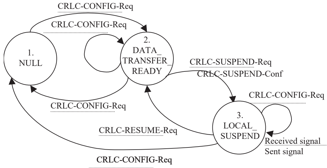
Figure 9.17: The state model for unacknowledged mode entities
