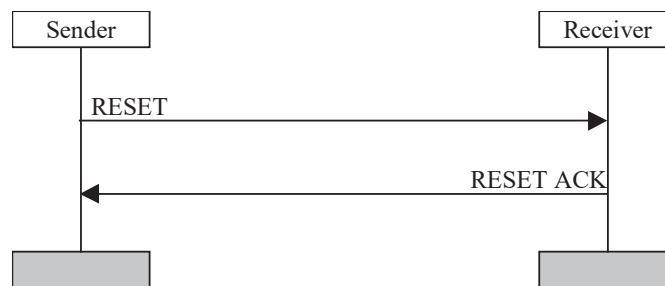
Figure 11.4: RLC reset procedure
