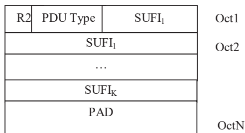
Figure 9.5: Piggybacked STATUS PDU
