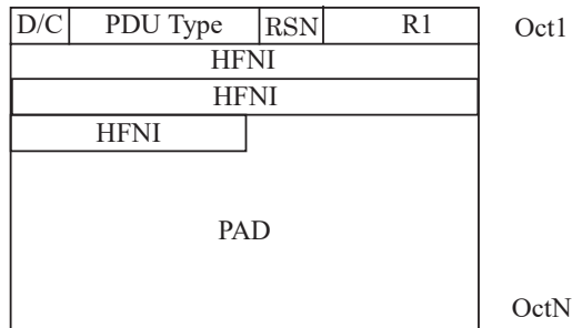
Figure 9.6: RESET, RESET ACK PDU
