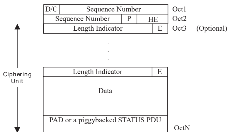
Figure 9.20: Ciphering unit for an AMD PDU
