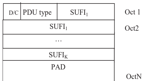
Figure 9.4: STATUS PDU
