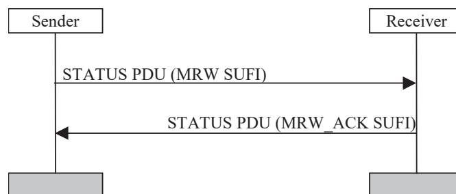
Figure 11.6: SDU discard with explicit signalling
