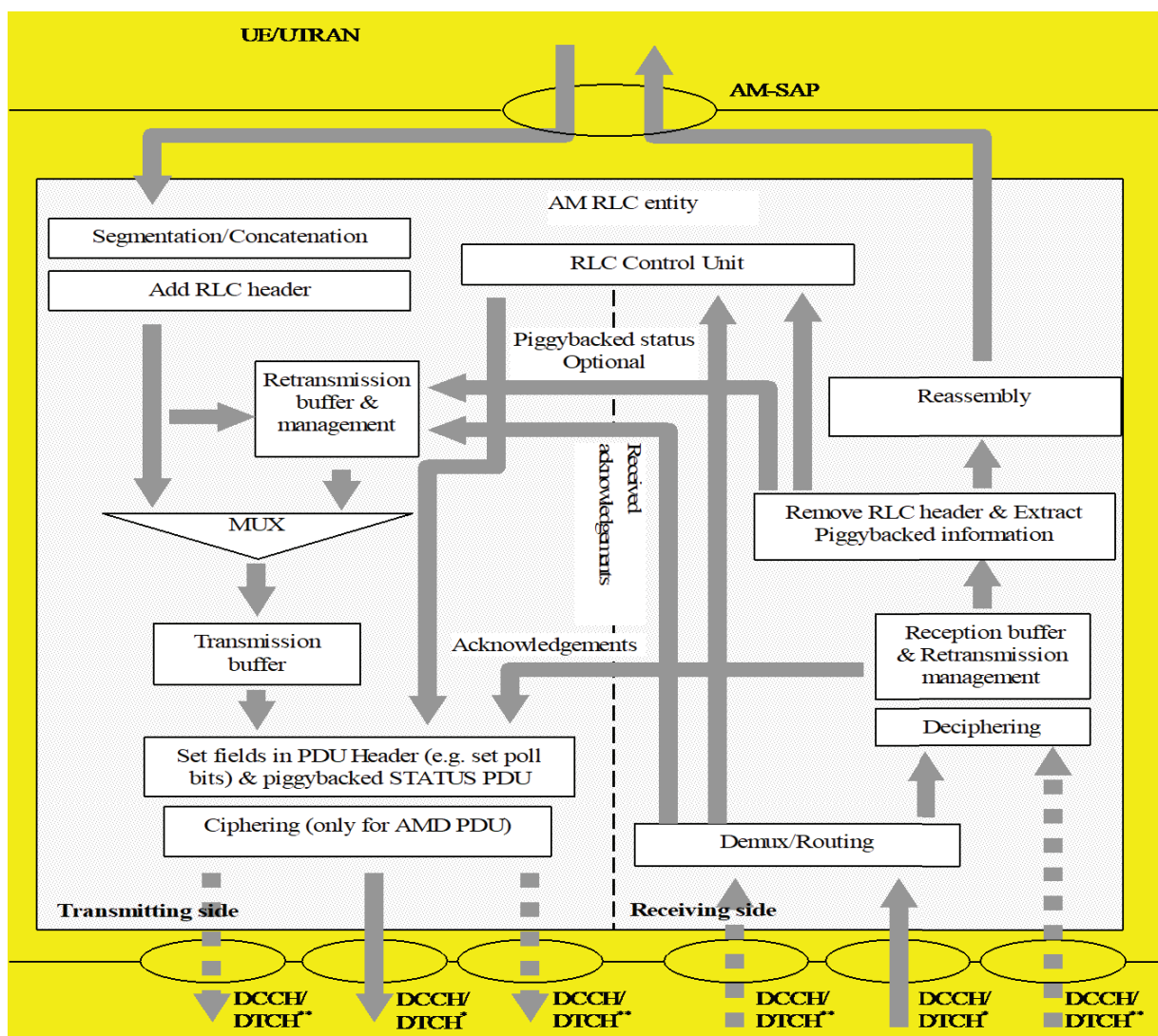
Figure 4.4: Model of an acknowledged mode entity
