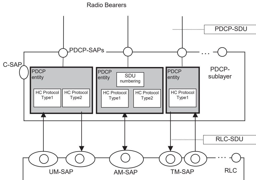
Figure 1: PDCP structure
