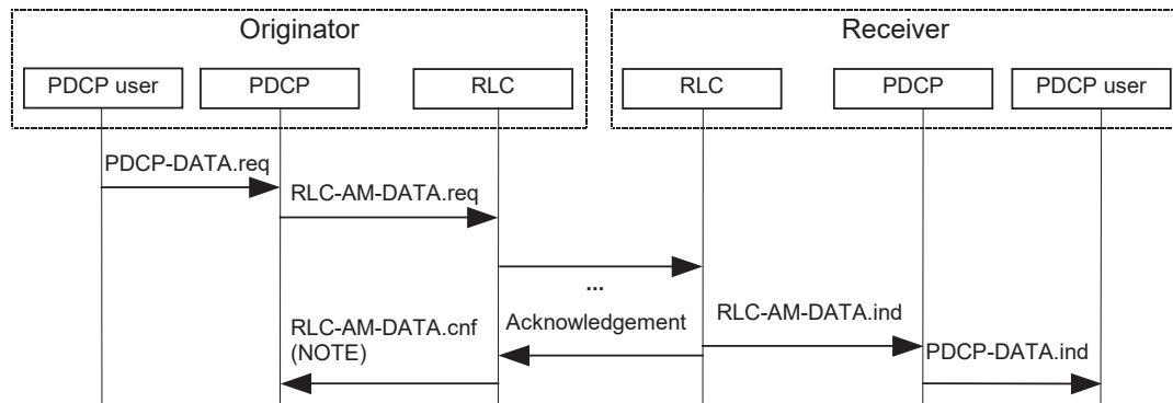
Figure 2: PDCP data transfer over acknowledged mode RLC
