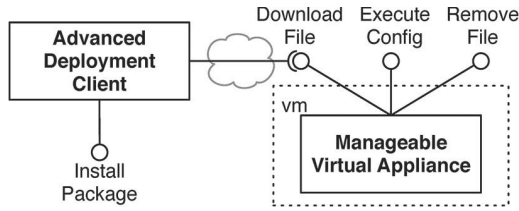
Fig. 2. Basic management interfaces.
