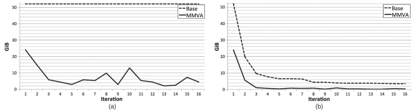
Fig. 8. Transferred data for VM instantiations during size optimization. (a) Without creating intermediate appliances: ut = \infty . (b) While creating intermediate appliances: ut = 1.1
