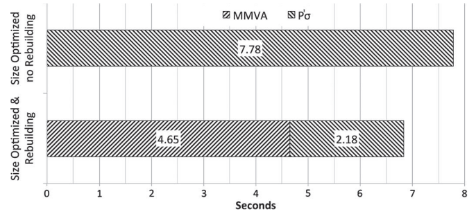
Fig. 9. Comparing the delivery of the Apache appliance.
