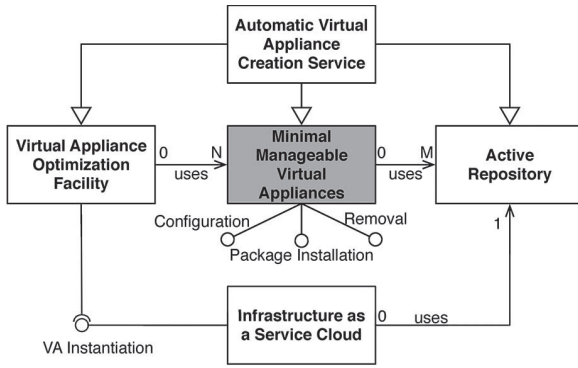
Fig. 5. Automated Virtual appliance creation Service.
