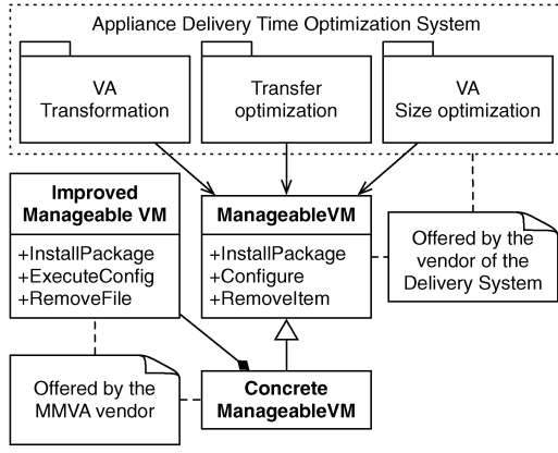
Fig. 4. MMVA interfacing with delivery systems.
