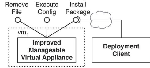
Fig. 3. Improved management interfaces.
