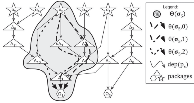
Fig. 1. Hypothetical dependency graph of six services.
