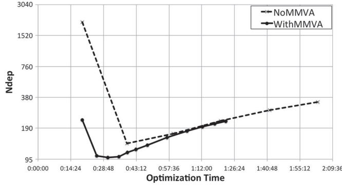
Fig. 7. Number of future deployments required.
