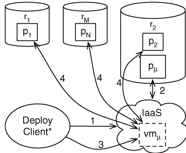
Fig. 6. Deployment client using an MMVA for rebuilding.
