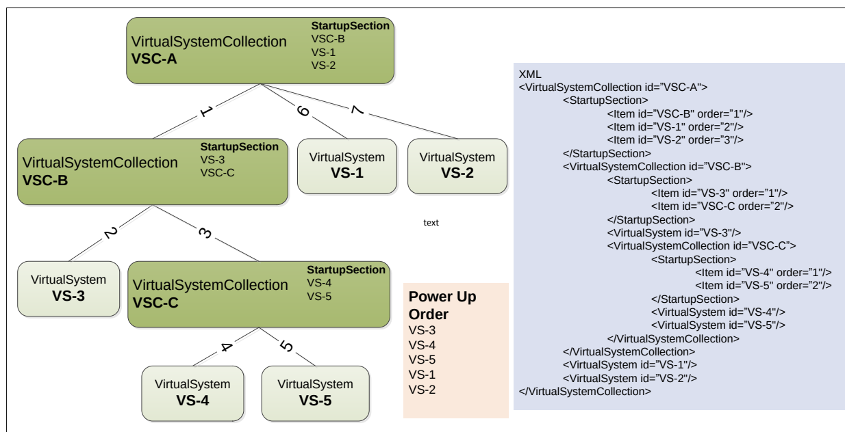
Figure 10 – StartupSection traversal
