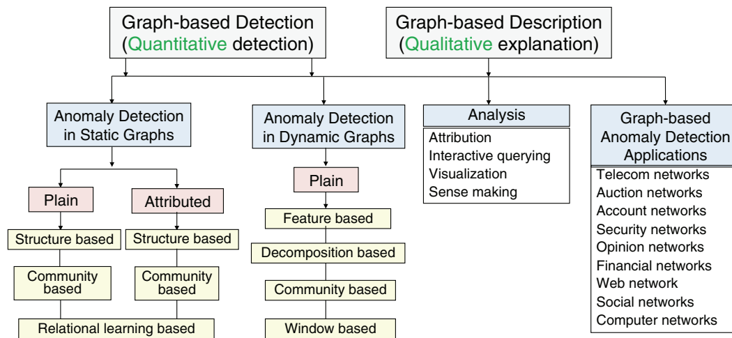
Fig. 2 Graph-anomaly detection: the outline of the survey
