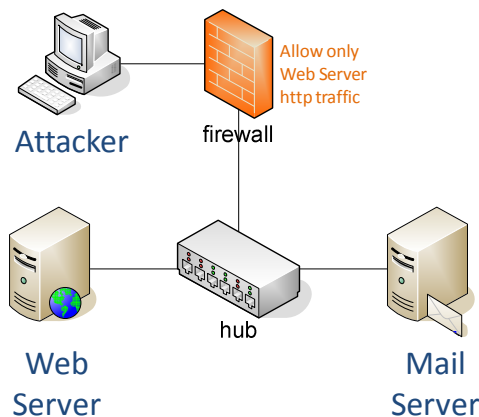
Figure 2. Small example network
