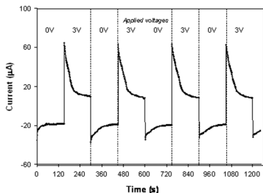
Figure 2 Switching cycles of current through the device
