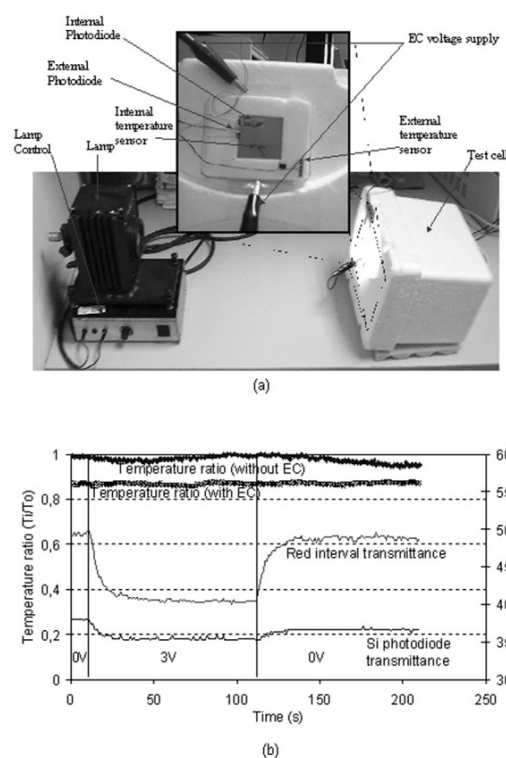
Figure 3 (a) Experimental setup for the test cell and the EC transmittance control application (inset: detail of the EC window and sensors while working); (b) results given directly by the system
