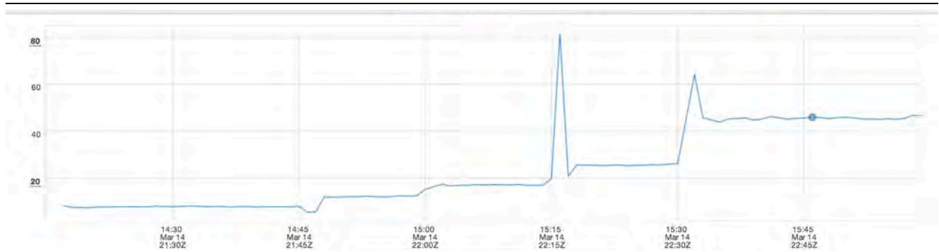
Figure 10: Latency Measurements
