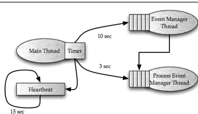
Figure 4: Supervisor architecture
