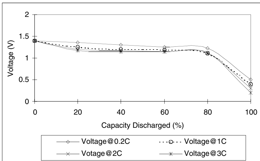
Figure 6–7 Variation of battery cell discharge voltage with discharge capacity.
