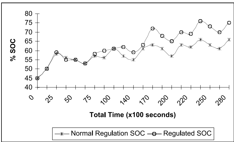
Figure 3–4 Comparison of normal SOC and regulated SOC.
