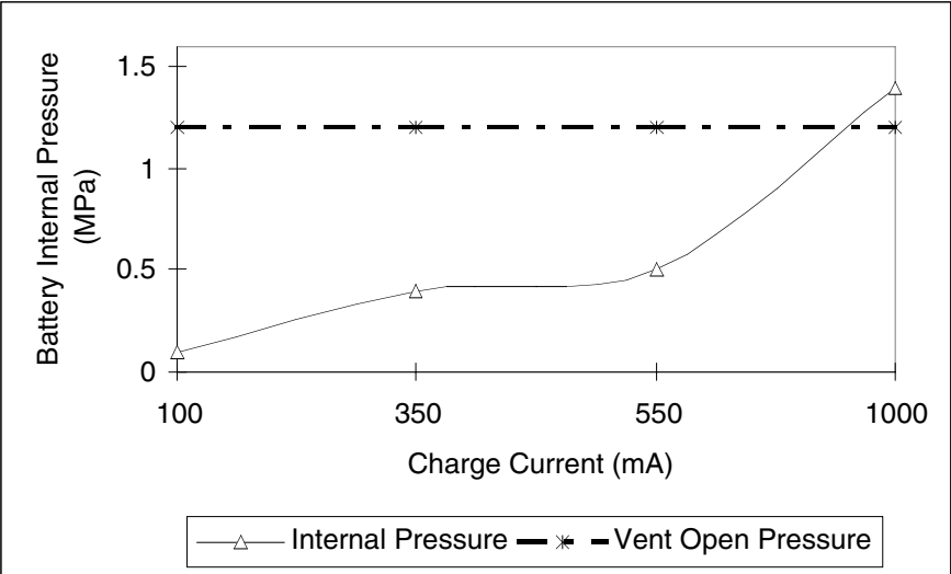
Figure 4–10 Variation of battery pressure during charging.
