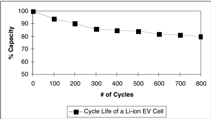
Figure 1–1 Life cycle of a Li-ion EV cell.
