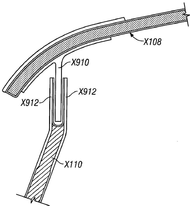
SECTION E-E FIG. 8H
