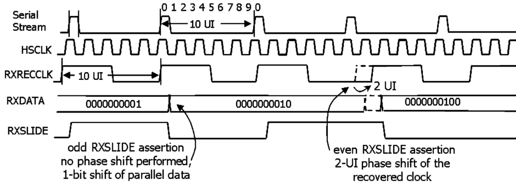
Fig. 4. Recovered clock phase adjustment by means of bit slips.
