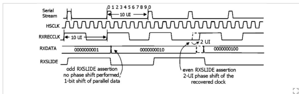
Fig. 4. Recovered clock phase adjustment by means of bit slips.
