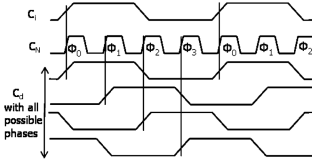
Fig. 2. Clock multiplication and subsequent division (case N = 4 ).
