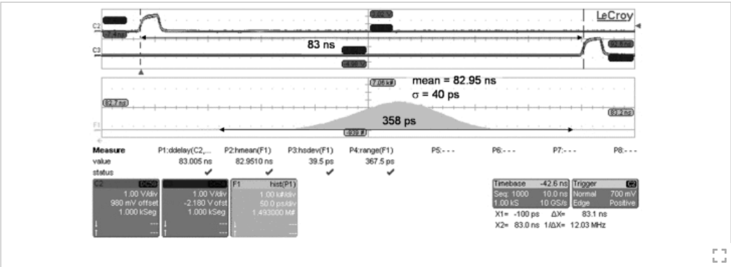
Fig. 7. Histogram of the latency of the link. Topmost trace: transmitted payload bit. Second trace: corresponding received bit. Down: histogram of the latency.
