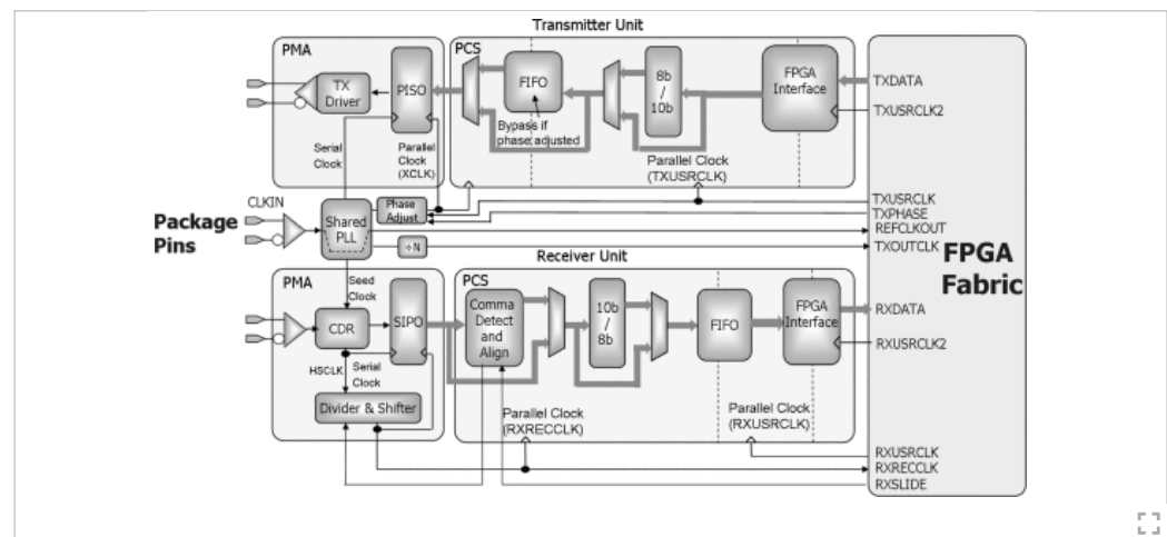
Fig. 1. Simplified block diagram of the GTP transceiver. Half a tile is shown.
