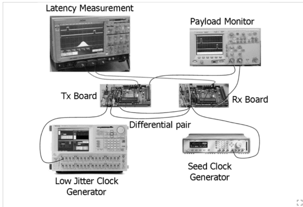
Fig. 6. Experimental setup for latency tests.
