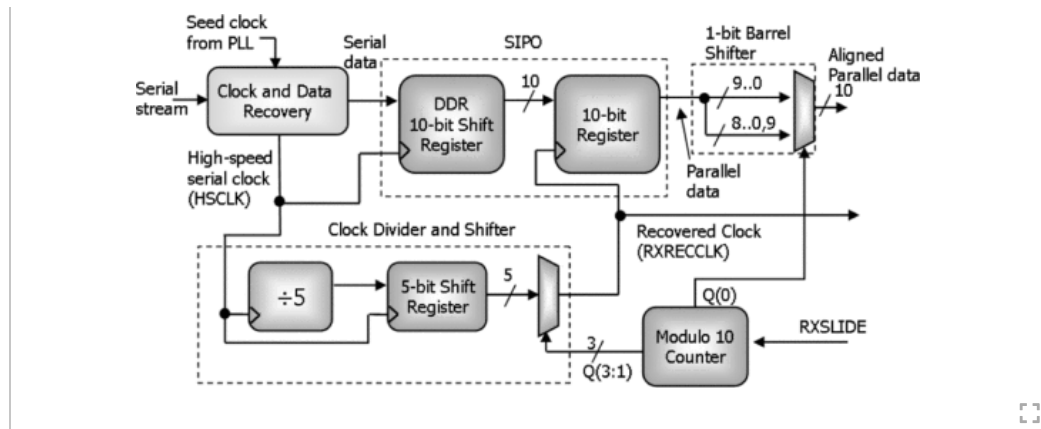
Fig. 3. Conceptual block diagram of the shift architecture used in PMA mode.
