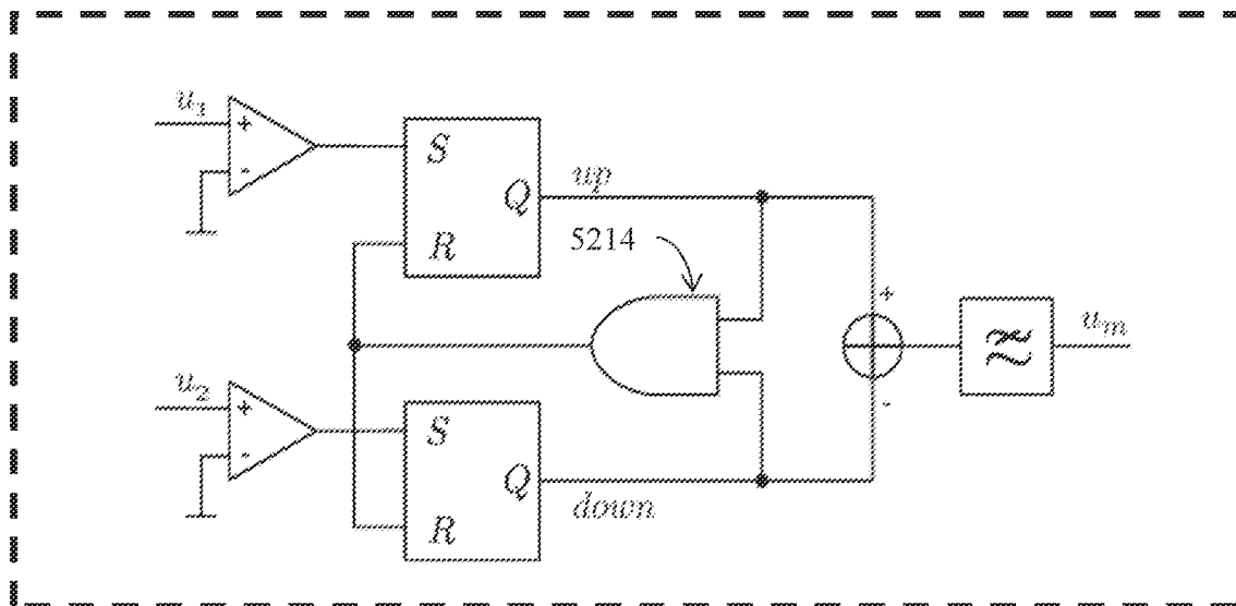
Phase Detector 3206''
