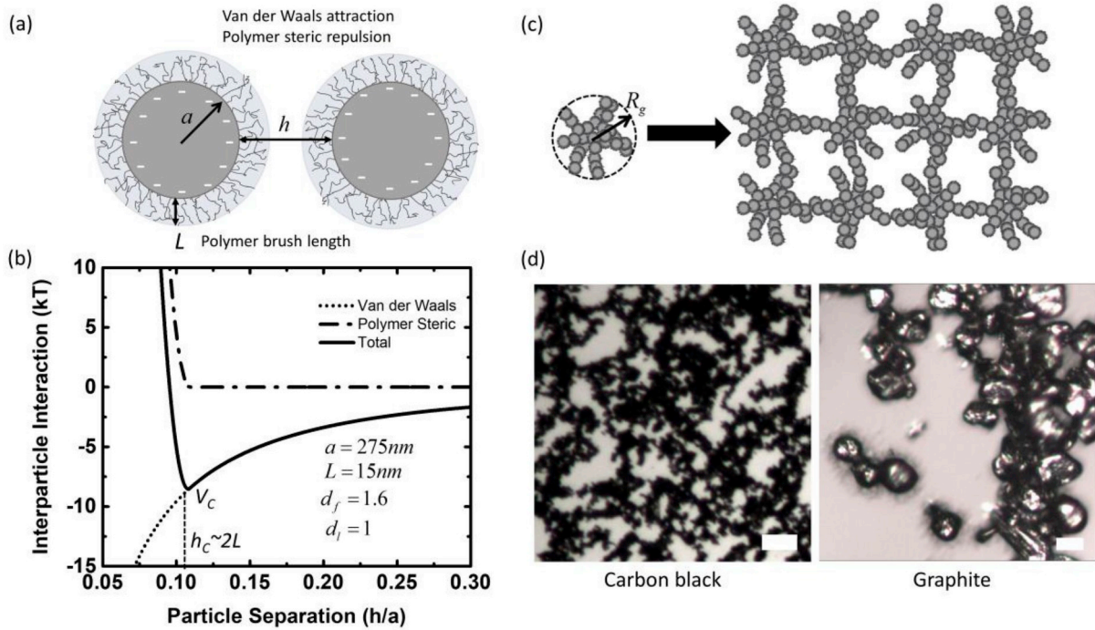
Fig. 1. Interparticle colloidal interaction and assembly behaviors of particles in anode slurry. (a) Schematic illustration of polymer-coated carbon black particles and interparticle colloidal interactions. (b) Typical interparticle potential between two carbon black particles coated with PVDF (KF1700). (c) Schematic representation of primary carbon black particles assembled into secondary aggregates with the aggregates connected into networks. (d) Optical images of assemblies of carbon black (left) and graphite (right) particles. The scale bar is 10 \mu\text{m} .
