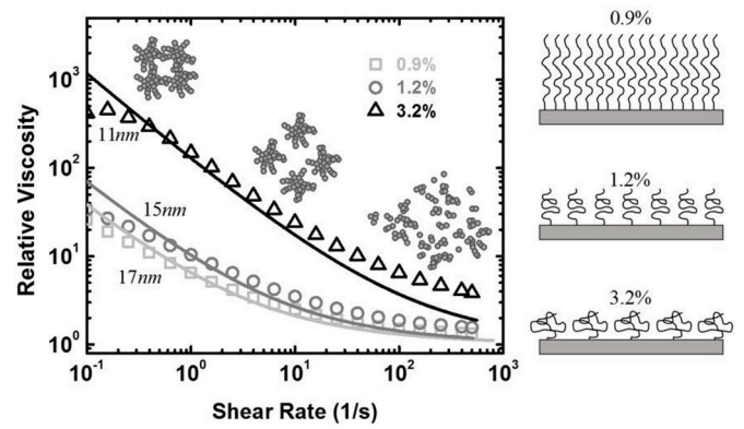
Fig. 3. Experimental and modeling results (assuming df = 1.6 ) for the viscosities of carbon black and PVDF (KF1700) slurries for three different particle concentrations. The light grey squares, dark circles, and black triangles are the experimental rheological data for \phi_p = 0.9\% , 1.2\% , and 3.2\% , respectively, and the light grey, dark, and black lines are the modeling rheological data for \phi_p = 0.9\% , 1.2\% , and 3.2\% , respectively. The schematic illustrations on the right side show the morphologies of PVDF on the carbon black surface for the three different particle volume fractions.
