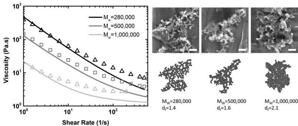
Fig. 4. Rheological properties of 3.2 vol% carbon black particles in polymer suspension with three different molecular weights: M_w(\text{KF1100}) = 280,000 , M_w(\text{KF1700}) = 500,000 , and M_w(\text{KF9300}) = 1,000,000 . SEM images and schematic illustrations of carbon black fractal aggregates in different polymer solutions. The scale bar is 500 nm.
