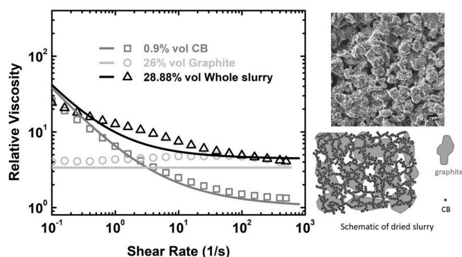
Fig. 5. The experimental (markers) and modeling (solid lines) results of the carbon black/polymer slurry, graphite/polymer slurry, and entire anode slurry are shown on the left side. An SEM image of the dried slurry is shown on the upper right side. The larger particles are graphite, and the interconnected smaller particles covering the graphite are carbon black particles. A schematic illustration of the entire dried slurry is presented below the SEM image. The scale bar is 10 \mu\text{m} .
