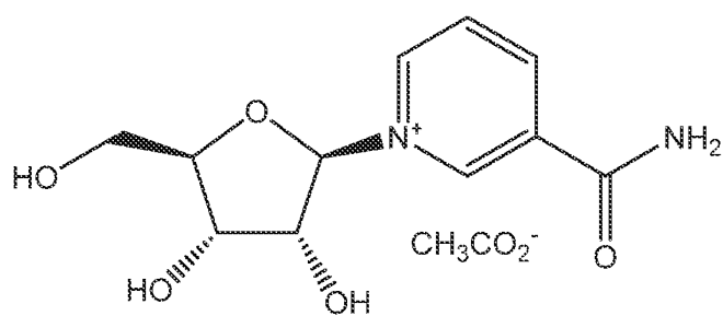
nicotinamide riboside, acetate salt
