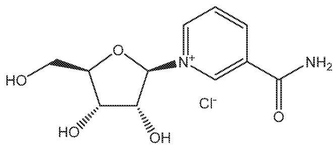
nicotinamide riboside, chloride salt
