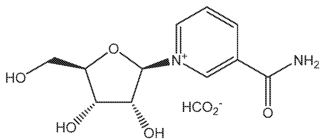
nicotinamide riboside, formate salt
