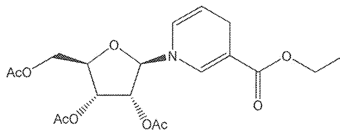
triacetyl O-ethyl-1,4-dihydronicotinate riboside
