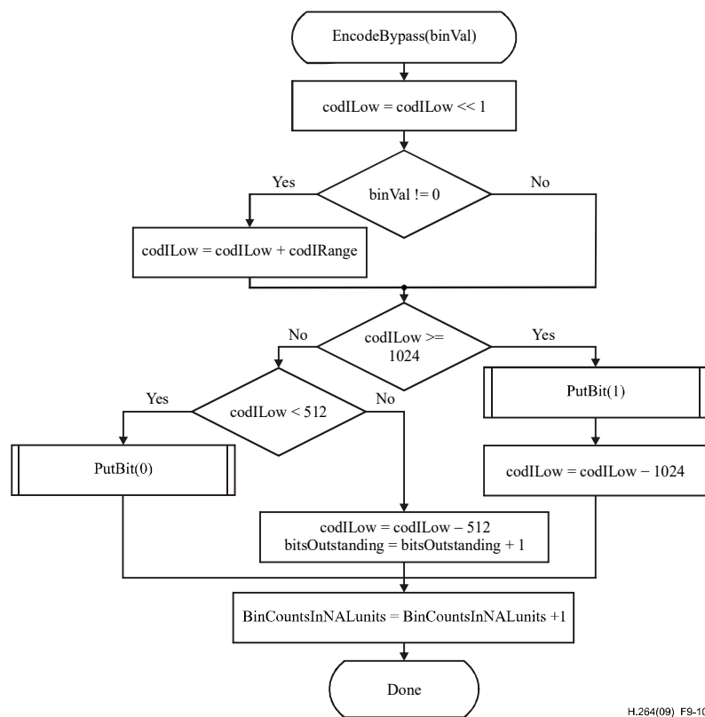
Figure 9-9 – Flowchart of encoding bypass
