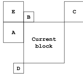
Figure 8-4 – Spatial neighbours, that can be used to derive reference indices for temporal merging candidates, (informative) illustrates the position of the spatial neighbours A, B, C, D and E relative to the current prediction unit.
