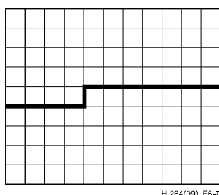
Figure 6-4 – A picture with 11 by 9 treeblocks that is partitioned into two slices
