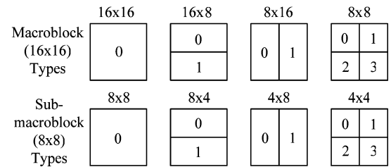
Fig. 7. Segmentations of the macroblock for MC. Top: segmentation of macroblocks, bottom: segmentation of 8 × 8 partitions.
