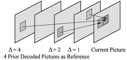
Fig. 8. Multipicture MCP. In addition to the MV, reference indexes ( \Delta ) are transmitted. The concept is similarly extended for B slices.
