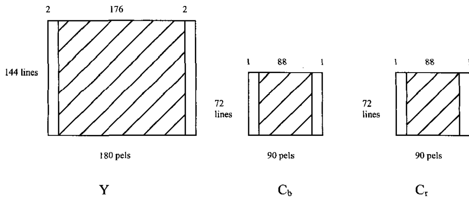
Fig. 17. QCIF (Quadrature Common Intermediate Format)
