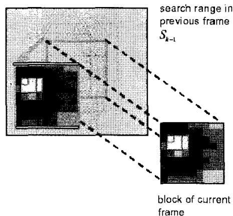
Fig. 30. Searching the best match from a previous frame
