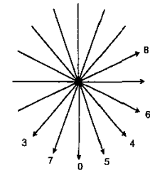
Fig. 21. Intra-prediction directions [1]
