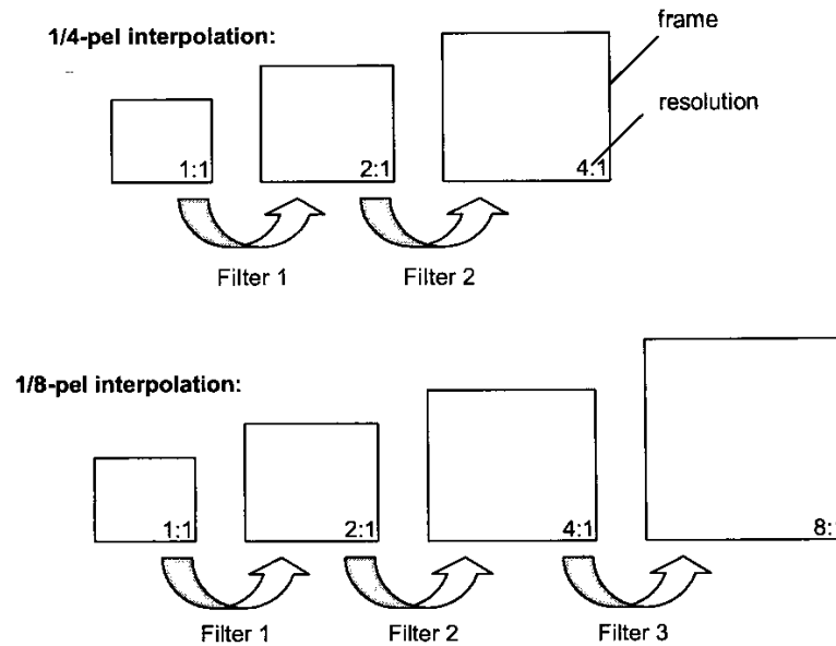
Fig. 37. Illustration of interpolation for fractional pel accuracy [2]
