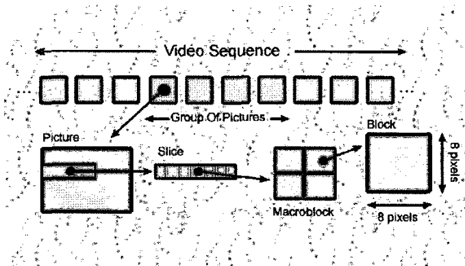
Fig. 18. Sequence-GOP-picture-slice-macroblock-block
