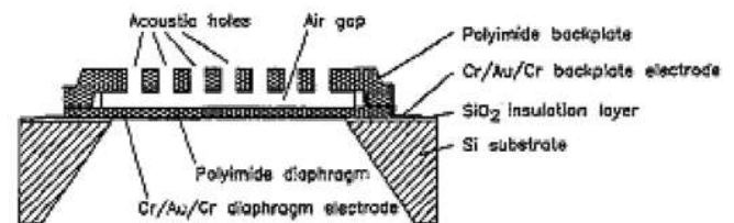
Fig 14. Polyimide capacitive microphone. 36
