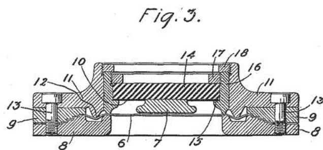
Fig 3. Image from Edward Wenté's 1917 patent of the condenser microphone. 6
