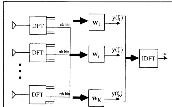
Figure 2.4 Beamforming is sometimes performed in the frequency domain when broadband signals are of interest. This figure illustrates transformation of the data at each sensor into the frequency domain. Weighted combinations of the data at each frequency (bin) are formed. An inverse discrete Fourier transform produces the output time series.
