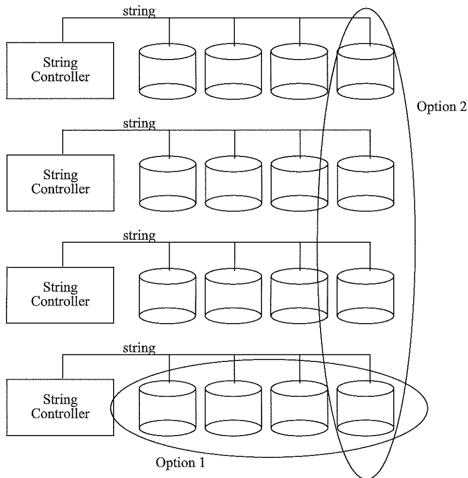
Figure 7: Orthogonal RAID. This figure present two options of how to organize error-correction groups in the presence of shared resources, such as a string controller. Option 1 groups four disks on the same string into an error-correction group; Option 2 groups one disk from each group into a group. Option 2 is preferred over Option 1 because the failure of a string controller will only render one disk from each group inaccessible.
