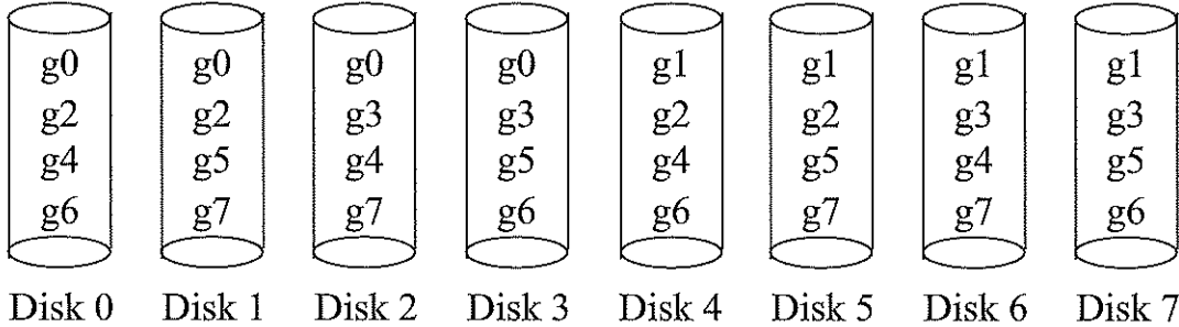
Declustered Parity RAID
