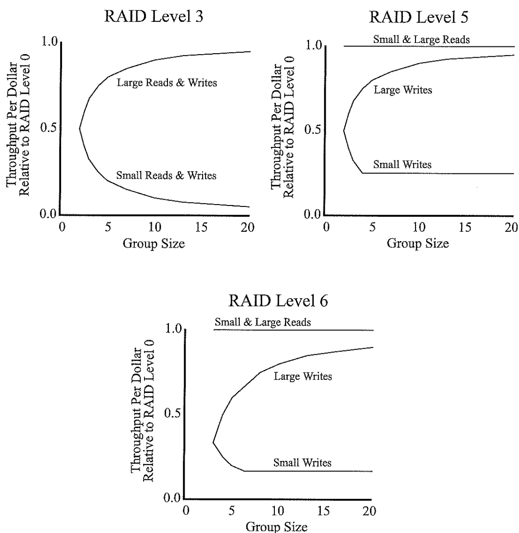
Figure 6: Throughput Per Dollar Relative to RAID Level 0. The graphs illustrate the tradeoff in performance/cost versus group size for each specified RAID level. Note that in this comparison, mirroring (RAID level 1) is the same as RAID level 5 with a group size of two.
