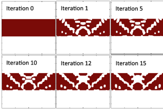
Fig. 5. Top view and iterative evolution of a \text{Ta}_2\text{O}_5 slab waveguide core (red) patterned with \text{SiO}_2 holes (white). This computer-generated pattern offers more absorption in the hotspot and reduced unintentional erasure of adjacent tracks.
