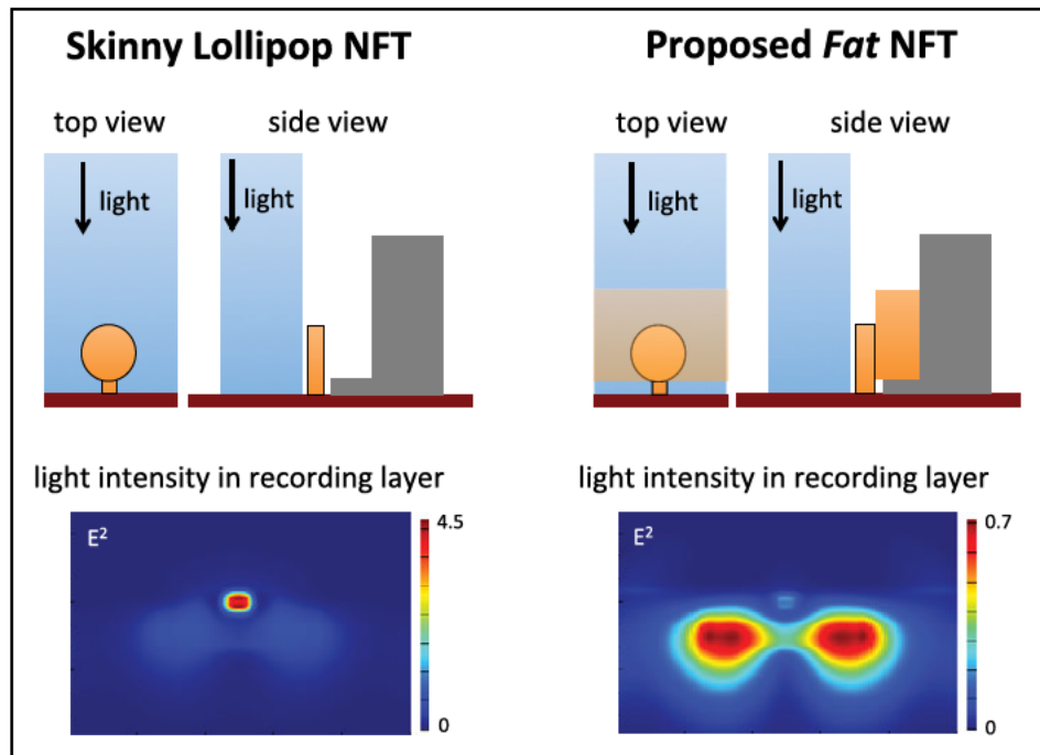
Fig. 3. HAMR optical system composed of a \text{Ta}_2\text{O}_5 waveguide (blue), gold NFT (yellow), CoFe write pole (gray), and magnetic media (red). Left: typical skinny lollipop NFT produces a confined hotspot in the storage layer. Right: proposed fat NFT has different electromagnetic behavior and is a poor mode match to a PSIM-like waveguide mode.
