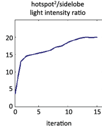
Fig. 6. Convergence plot of the optimized FOM versus iteration. FOM was the square of the peak light intensity in the media hotspot divided by the peak light intensity in the unwanted sidelobes.
