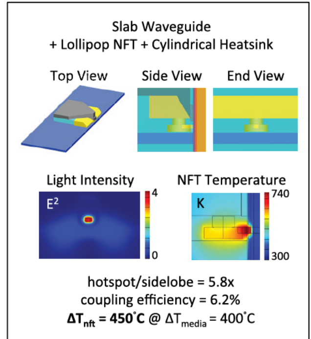
Fig. 7. Top: structural model of a slab waveguide, lollipop NFT, narrow cylindrical heatsink, and write pole. Mid: simulated light intensity in the media and side-view temperature profile of the NFT, heatsink, and media. This design suffers from severe self-heating.
