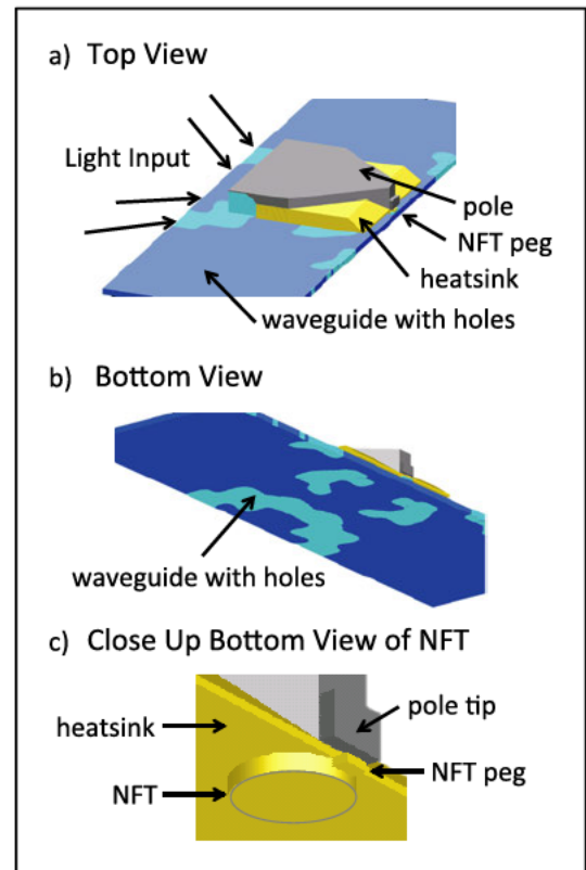
Fig. 4. 3-D views of the proposed HAMR light delivery structure. Fat NFT is a thin-film disk embossed on a bulk chunk of gold, and the slab waveguide contains a pattern of low-index material.
