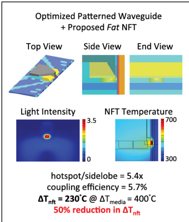
Fig. 8. Top: structural model of the proposed HAMR structure consisting of a patterned waveguide, fat NFT, and write pole. Mid: simulated light intensity in the media and side-view temperature profile of the NFT, heatsink, and media. This design achieves desirable optical properties and significantly reduced self-heating.
