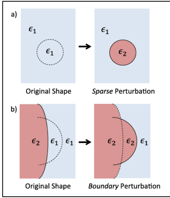
Fig. 2. (a) Sparse perturbation is the inclusion of an isolated small sphere displacing a material of different permittivity. (b) Boundary perturbation is the inclusion of a locally flat bump at the interface between materials of different permittivity.
