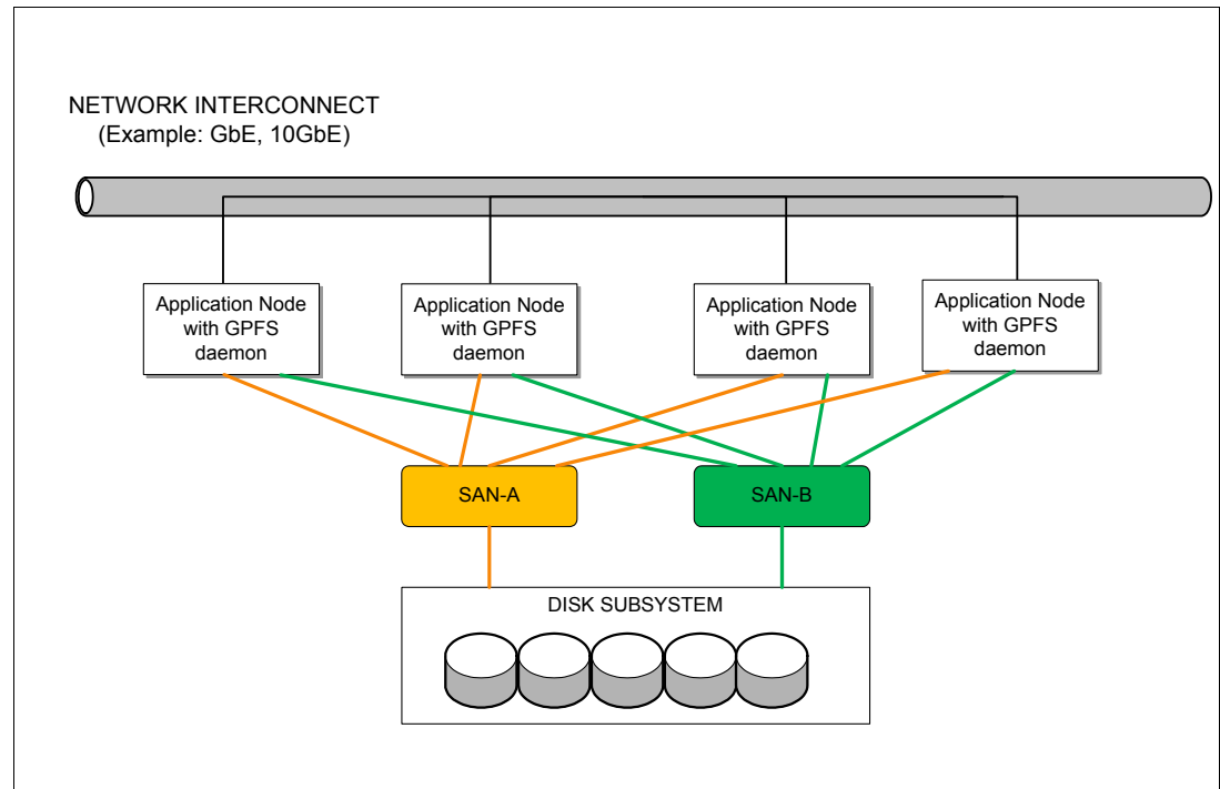
Figure 2-2 Direct storage access configuration
