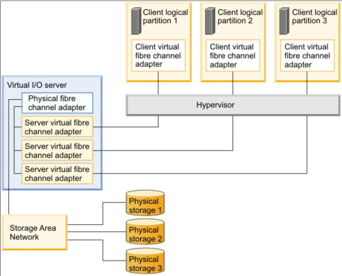
Figure 1-3 NPIV functionality illustration
