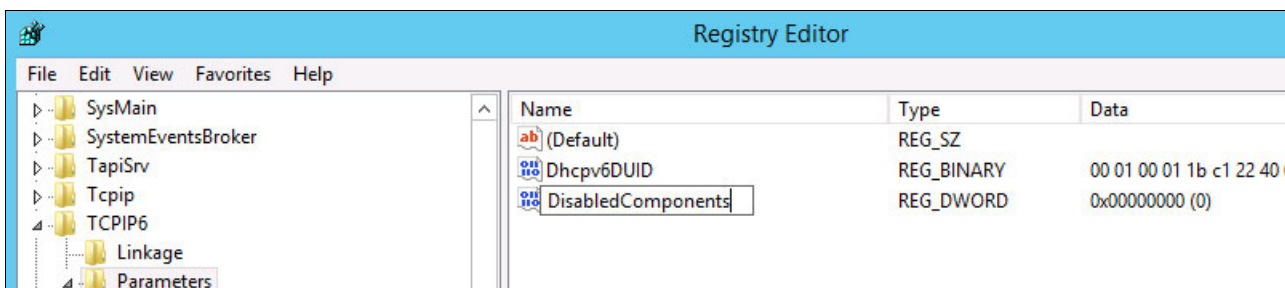
Figure 3-6 Naming the DWORD to DisabledComponents
