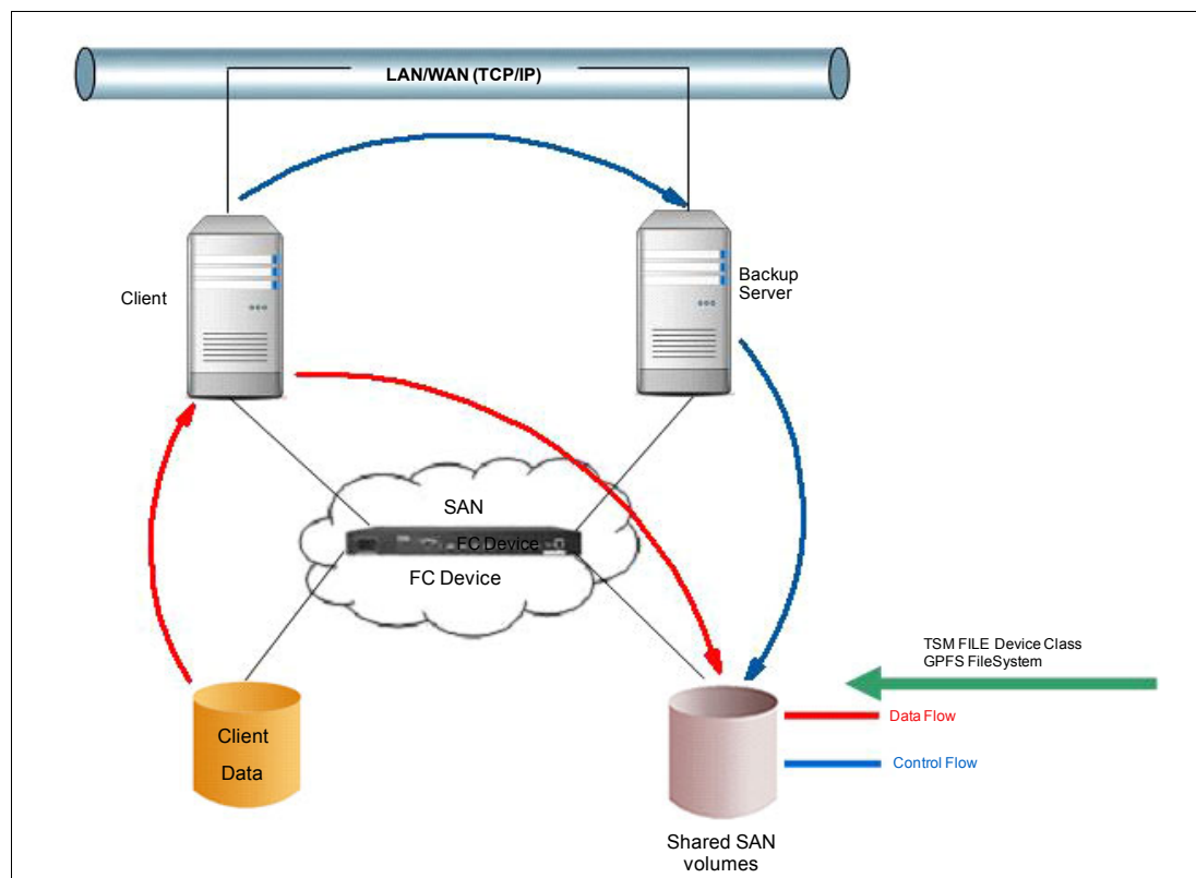
Figure 3-34 Spectrum Protect LAN-free with Spectrum Scale
