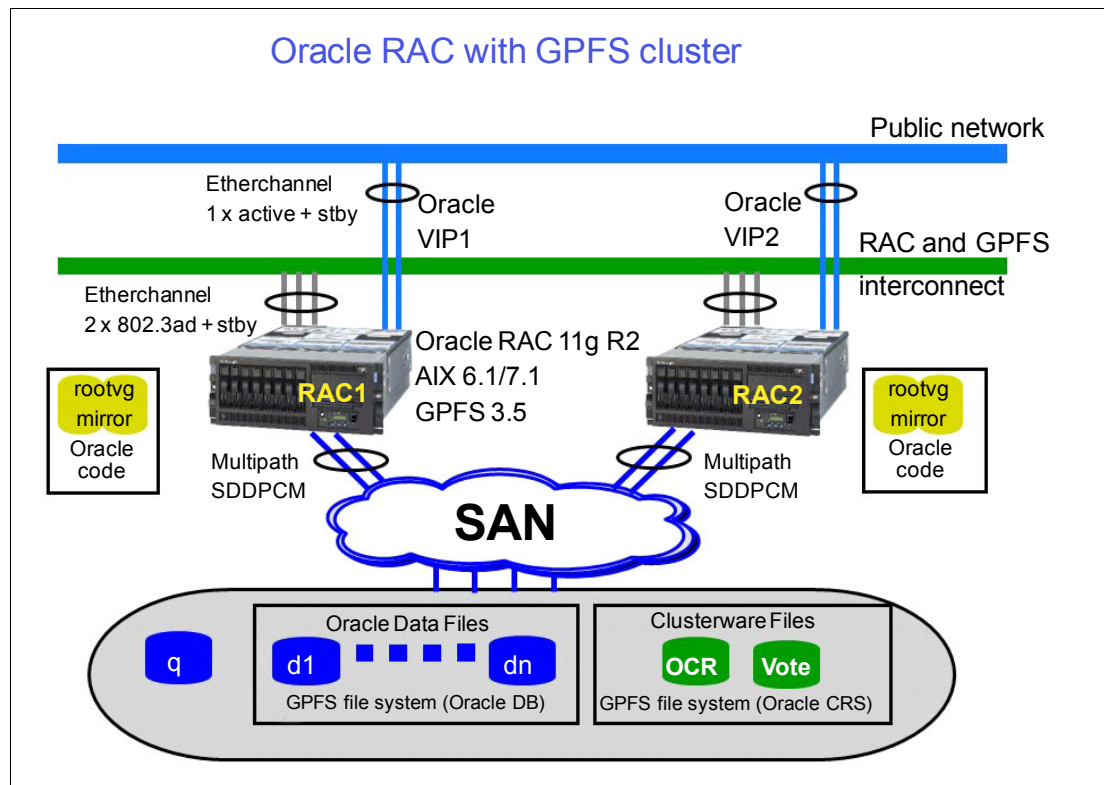
Figure 3-33 Oracle RAC cluster using IBM Spectrum Scale
