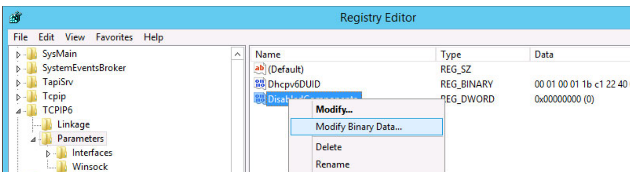
Figure 3-7 Editing the DWORD binary value
