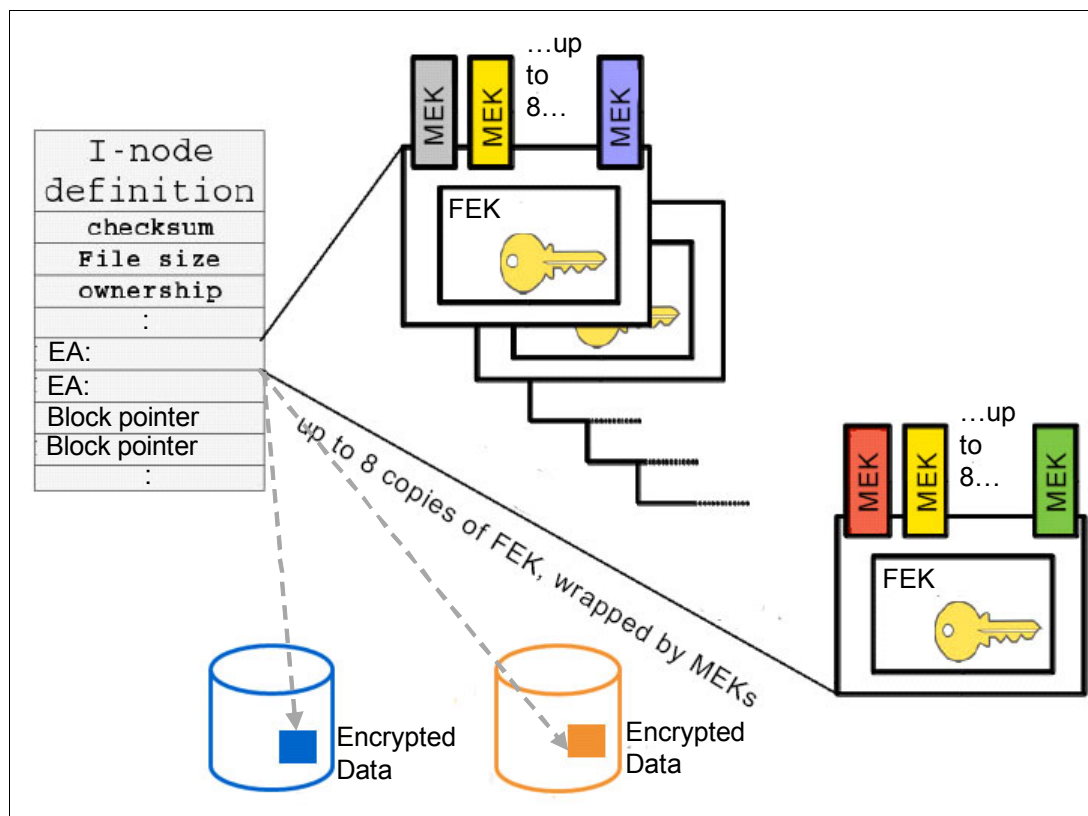
Figure 9-1 Mode information with MEK/FEK
