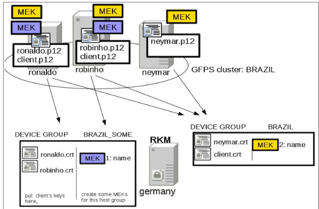
Figure 9-22 Organize node certificates
