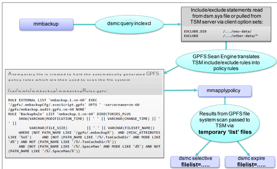
Figure 7-6 mmbackup flow
