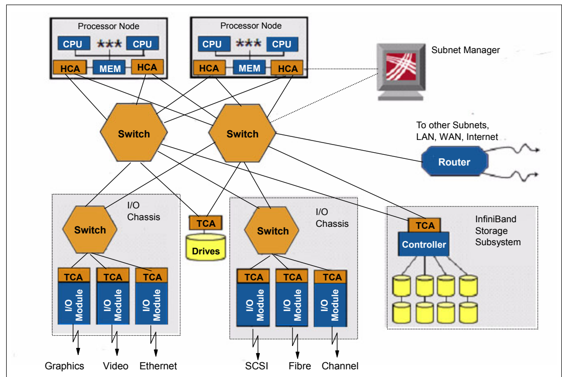
Figure 2-5 InfiniBand architecture
