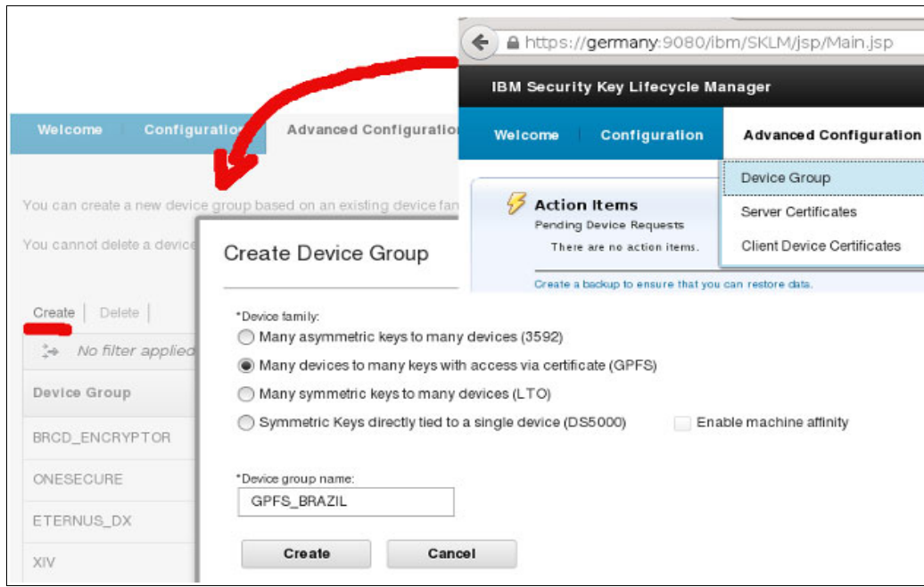
Figure 9-11 Creating a device group (DG)
