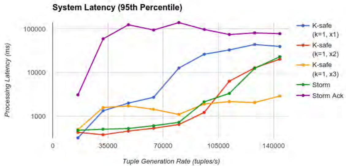
Figure 2: Benchmark results for stateless topologies
