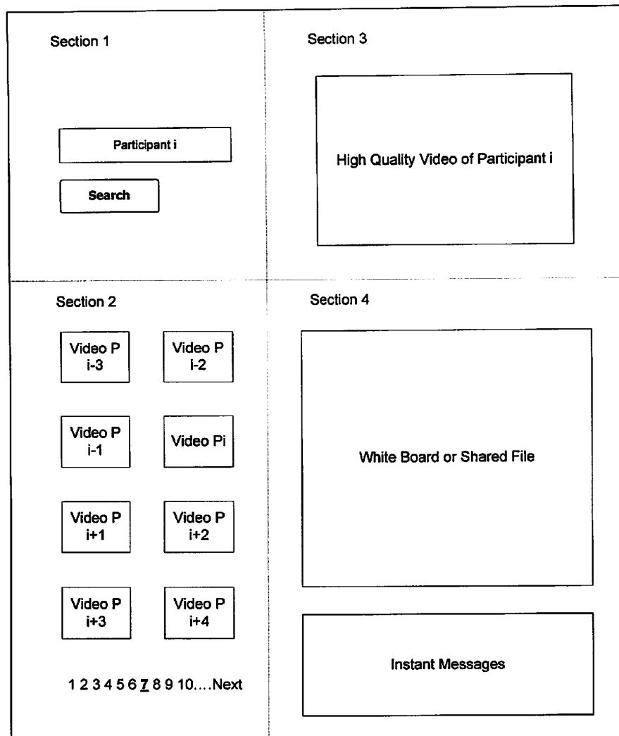
FIG. 4 Search Result Page
