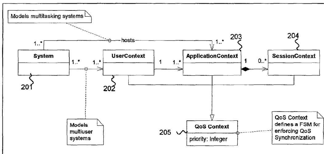
Figure 2 General Data Model: QoS Context
