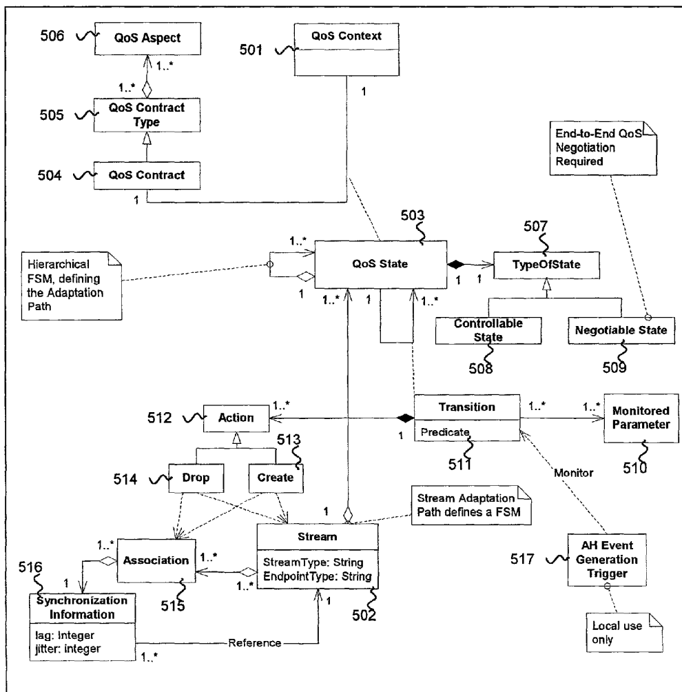
Figure 5: QoS- and synchronisation-specification model
