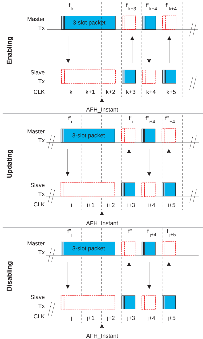
Figure 70—AFH_Instant changes during multislot packets transmitted by the master
