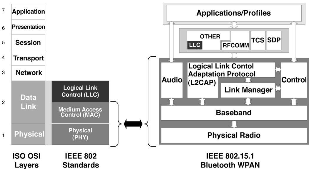
Figure 227—OSI and Bluetooth protocols
