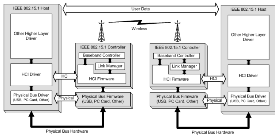
Figure 92—End-to-end overview of lower software layers to transfer data
