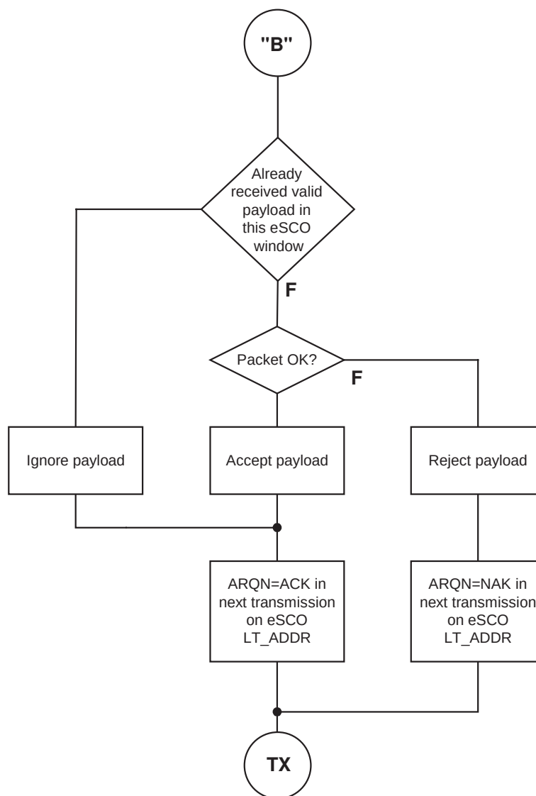
Figure 56—Stage 2 (eSCO) of the receive protocol for determining the ARQN bit
