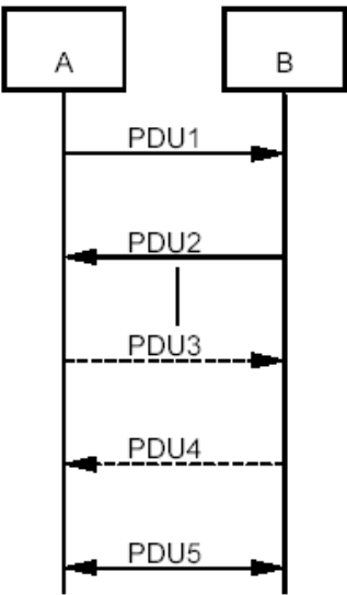
Figure 87—Symbols used in sequence diagrams
