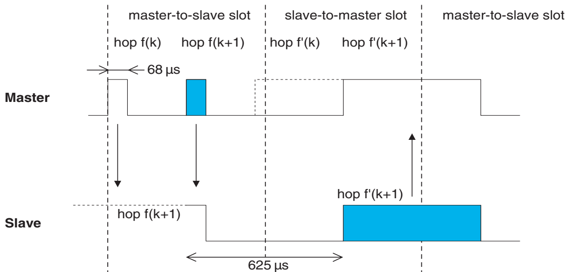
Figure 22—Timing of inquiry response packet on successful inquiry in second half slot
