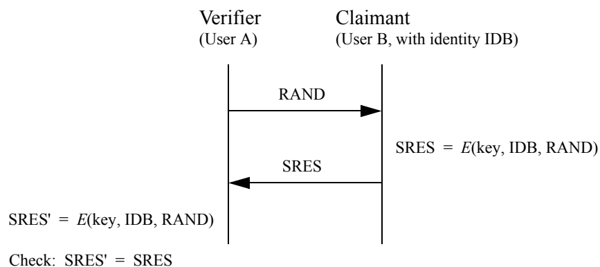
Figure 178—Challenge-response for symmetric key systems
