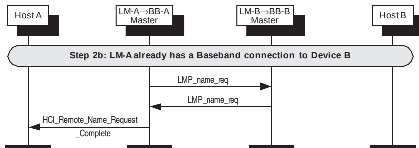
Figure 102—Remote name request with BB connection
