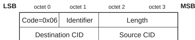
Figure 203—Disconnection Request packet
