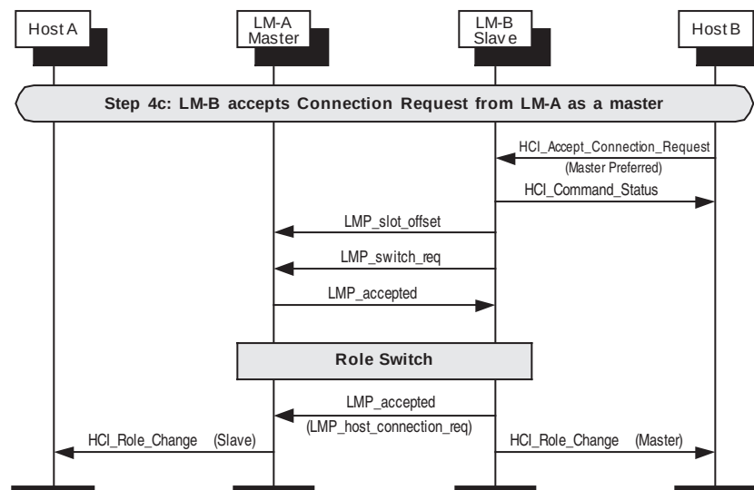
Figure 117—Device B accepts connection requests as master
