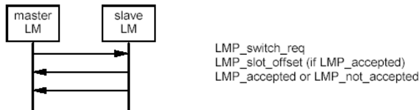
Sequence 46: Role switch (master initiated).
