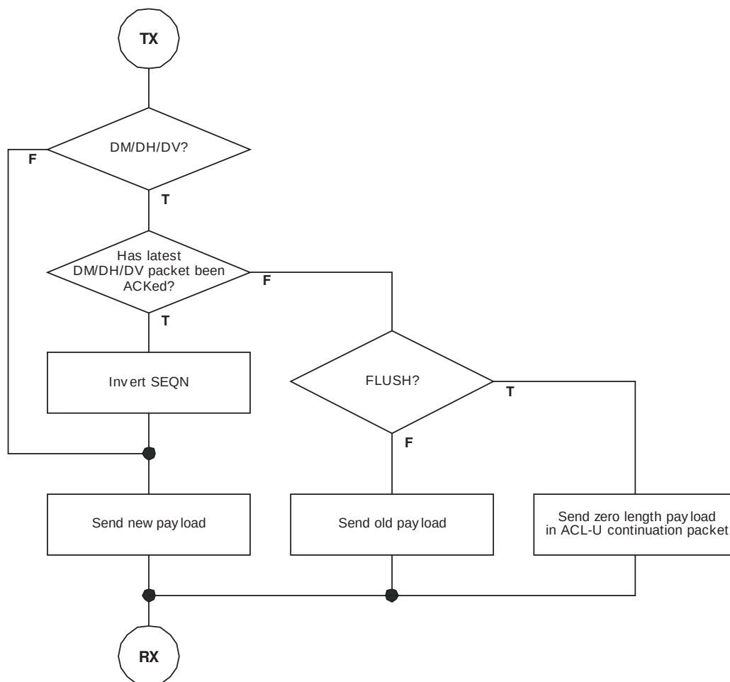
Figure 57—Transmit filtering for packets with CRC
