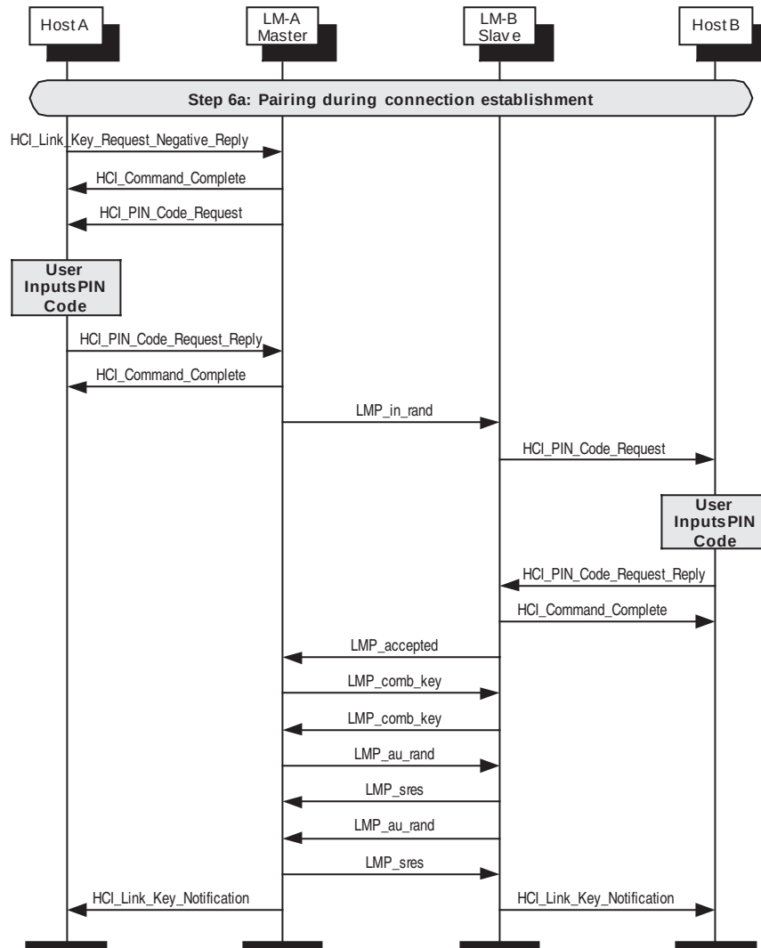
Figure 120—Pairing during connection setup
