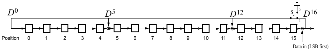
Figure 48—The LFSR circuit generating the CRC
