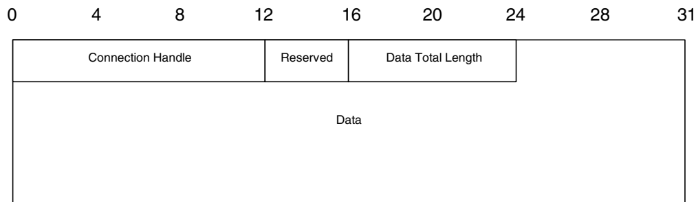
Figure 95—HCI synchronous data packet
