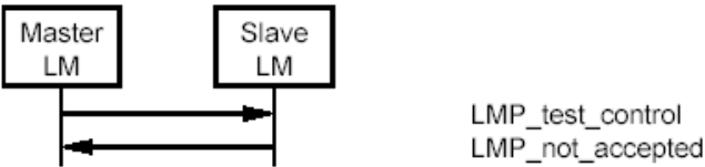
Sequence 72: Control of test mode rejected since slave is not in test mode.
