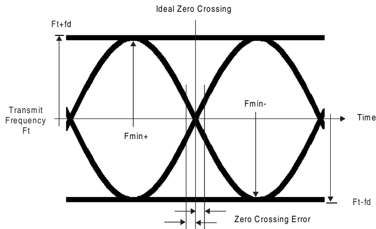
Figure 7—GFSK parameters definition
