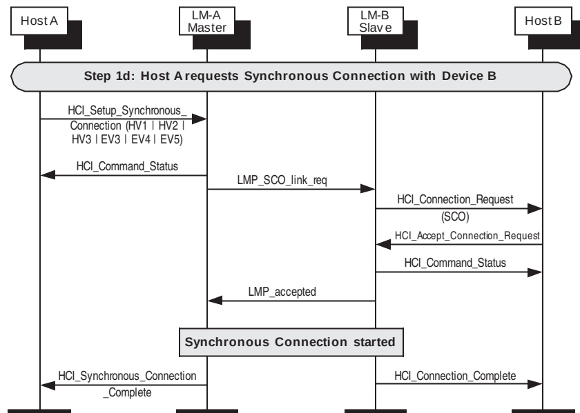
Figure 142—Master requests synchronous connection with legacy slave
