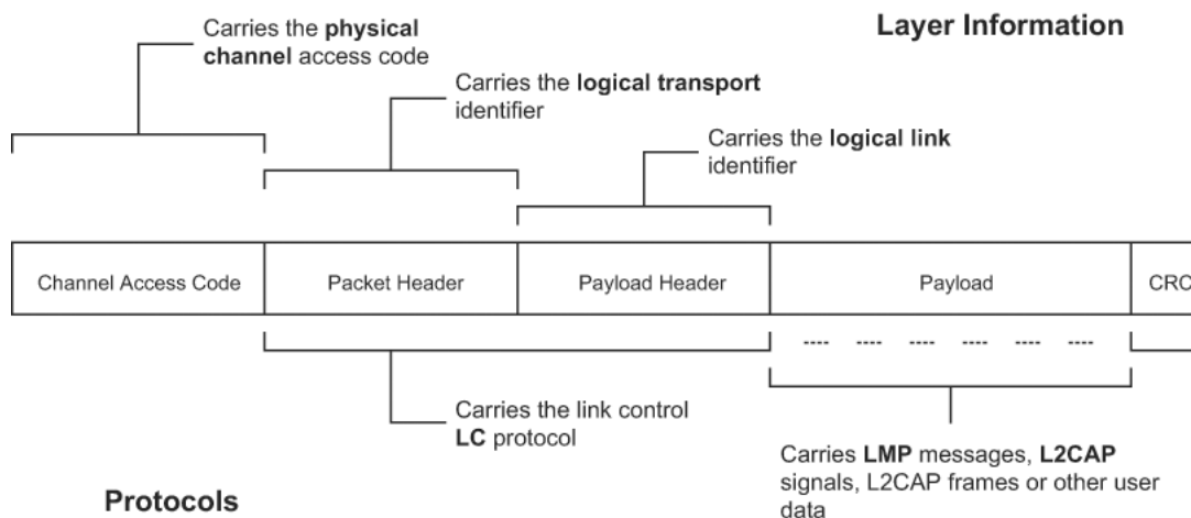
Figure 5—Packet structure
