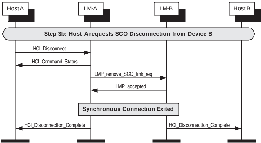
Figure 147—Synchronous disconnection of SCO connection
