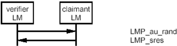
Sequence 20: Authentication. Claimant has link key.
