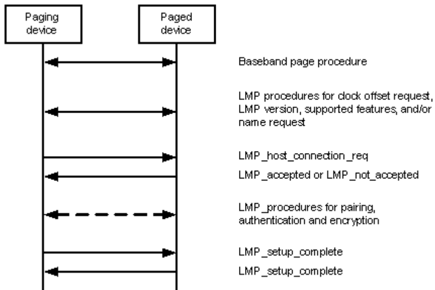
Figure 89—Connection establishment with host request
