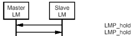
Sequence 48: Slave forces master into HOLD mode.
