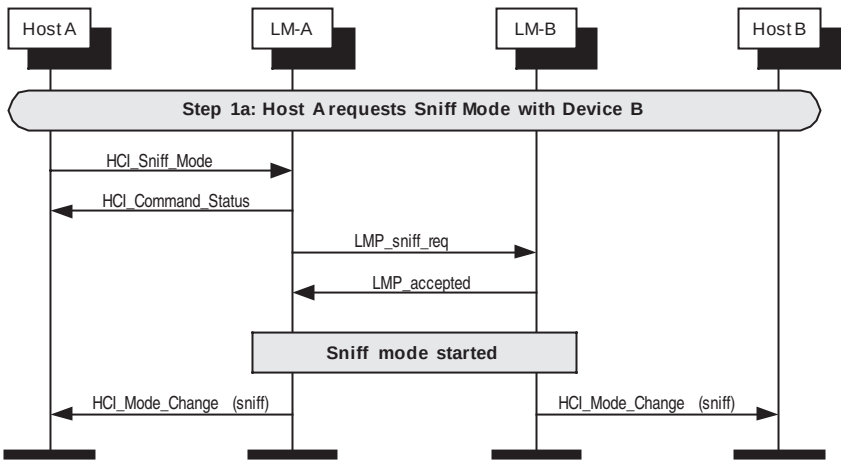
Figure 148—SNIFF mode request
