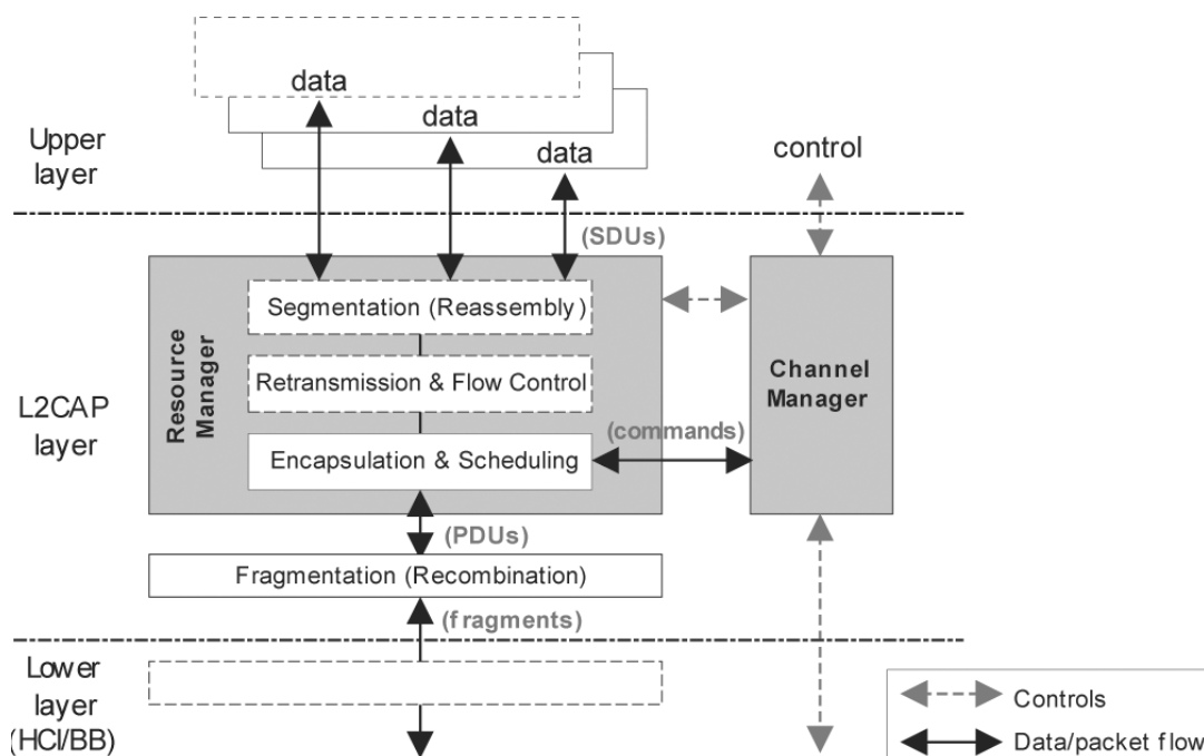
Figure 186—L2CAP architectural blocks
