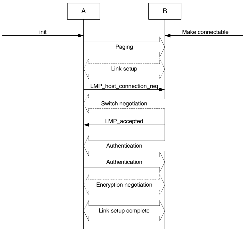
Figure B.14—Link establishment procedure when both the paging device (A) and the paged device (B) are in security mode 3
