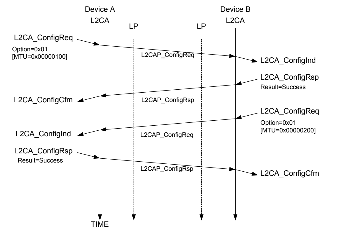
Figure 223—Basic MTU exchange
