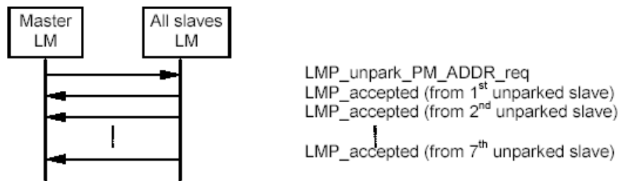
Sequence 58: Master unparks slaves addressed with their PM_ADDR.
