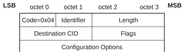
Figure 199—Configuration Request packet
