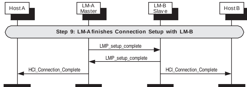
Figure 123—LM-A and LM-B finish connection setup
