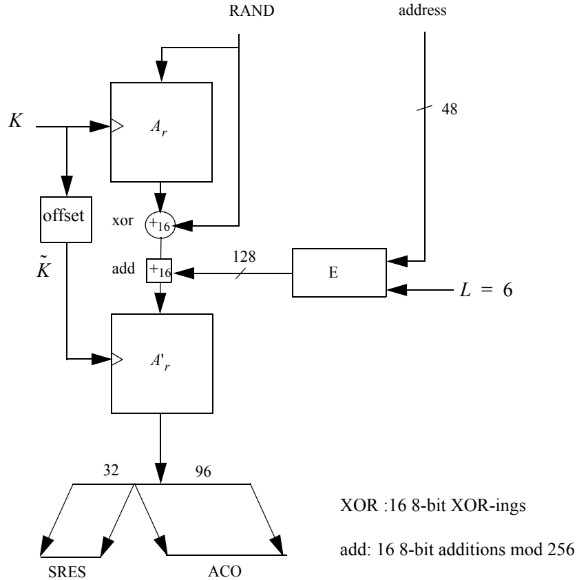
Figure 179—Flow of data for the computation of E_1
