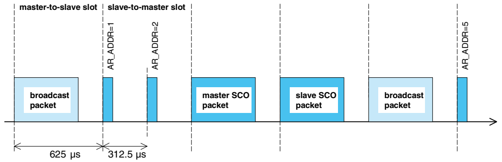
Figure 75—Disturbance of access window by SCO traffic
