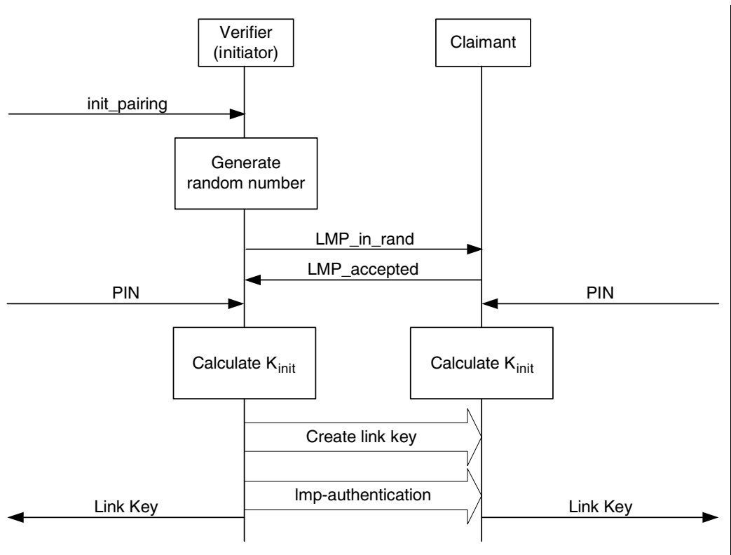
Figure B.20—LMP-pairing as defined in Clause 9
