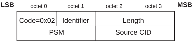
Figure 197—Connection Request packet
