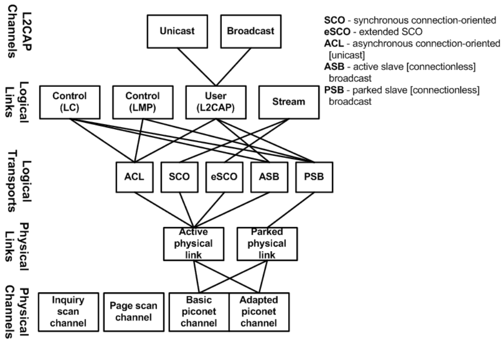
Figure 4—Overview of transport architecture entities and hierarchy
