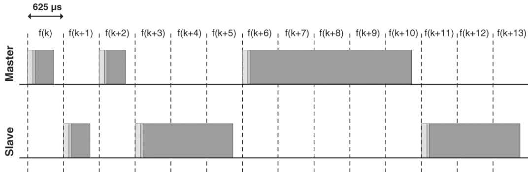
Figure 12—Multislot packets
