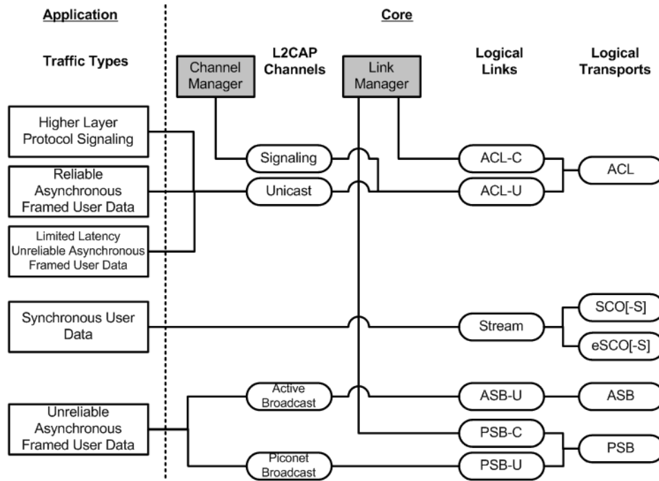
Figure 3—Traffic bearers
