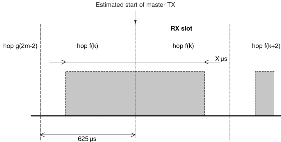
Figure 16—RX timing of slave returning from HOLD mode
