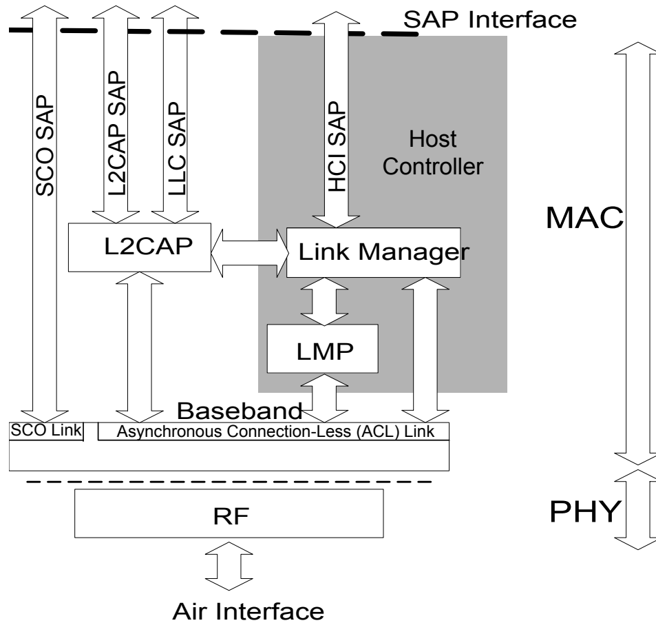
Figure 232—Bluetooth protocol entities mapped onto IEEE 802 constructs
