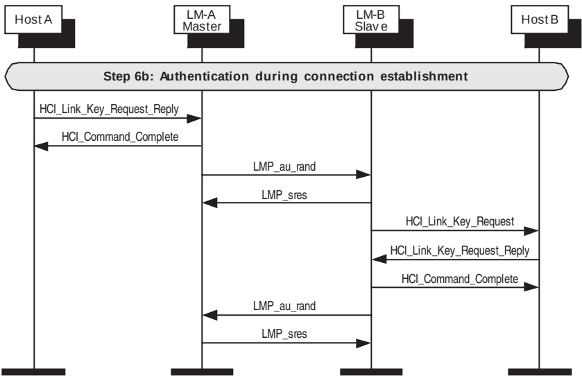
Figure 121—Authentication during connection setup
