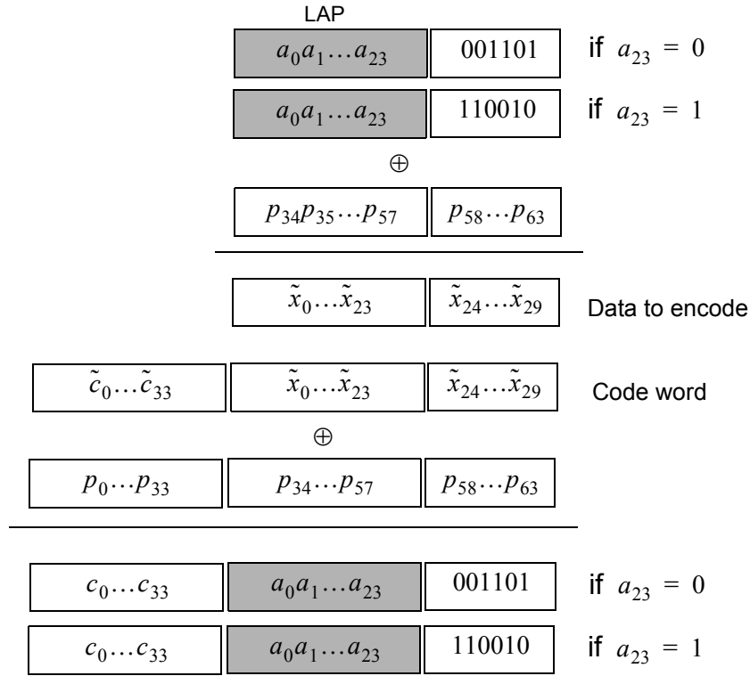
Figure 35—Construction of the sync word
