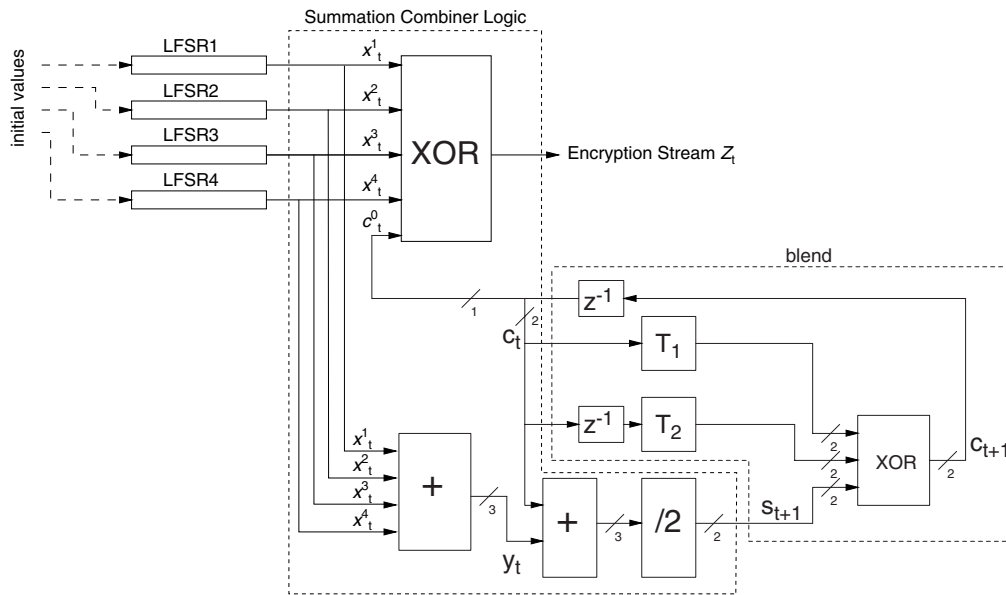
Figure 173—Concept of the encryption engine
