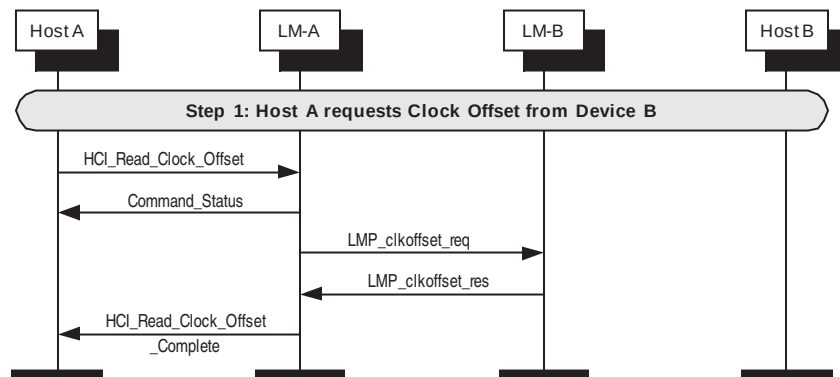
Figure 133—Read clock offset
