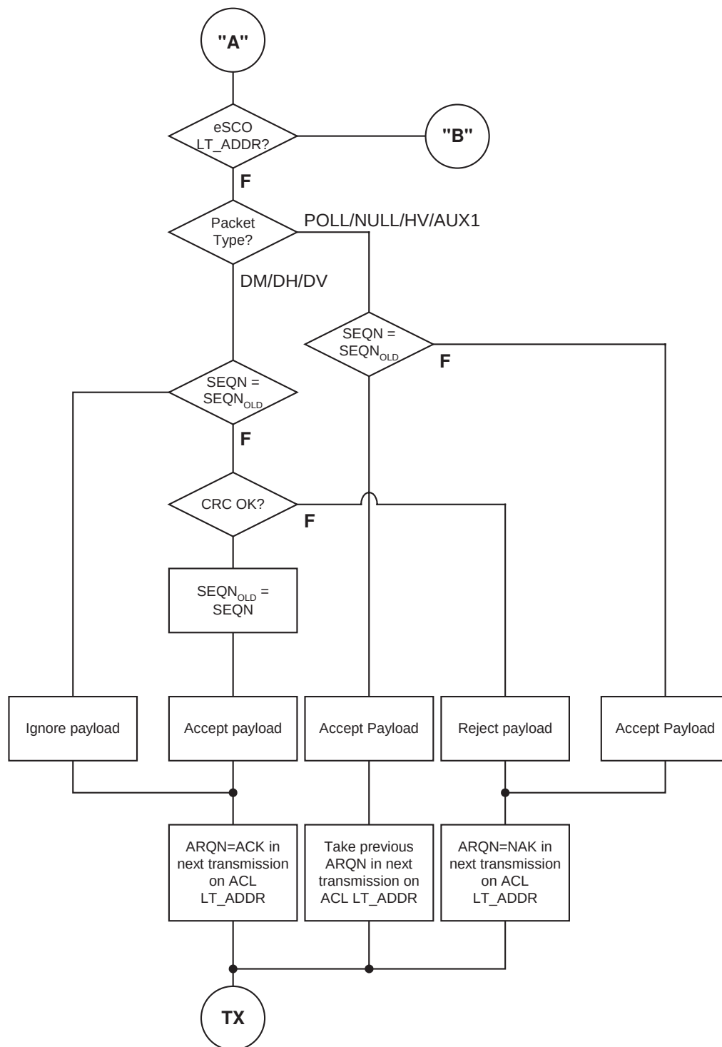
Figure 55—Stage 2 (ACL) of the receive protocol for determining the ARQN bit
