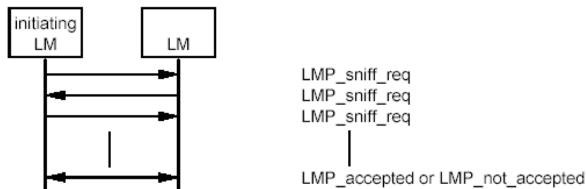
Sequence 59: Negotiation for SNIFF mode.
