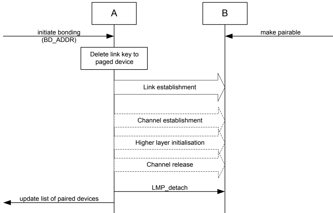
Figure B.11—General bonding, where the link establishment procedure is executed under specific conditions on both devices, followed by an optional higher layer initialization process
