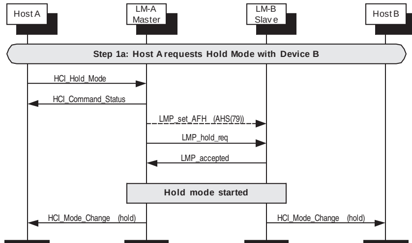
Figure 150—HOLD request
