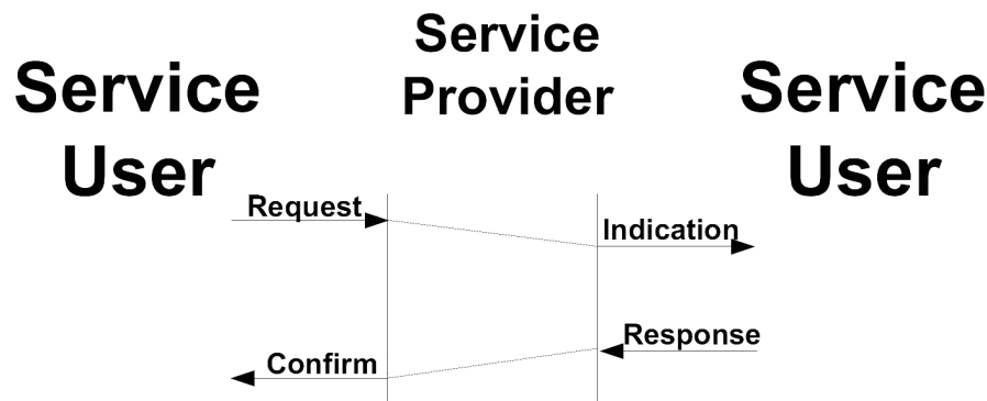
Figure 228—Service primitives
