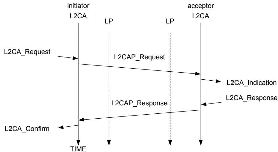
Figure 231—L2CA interaction
