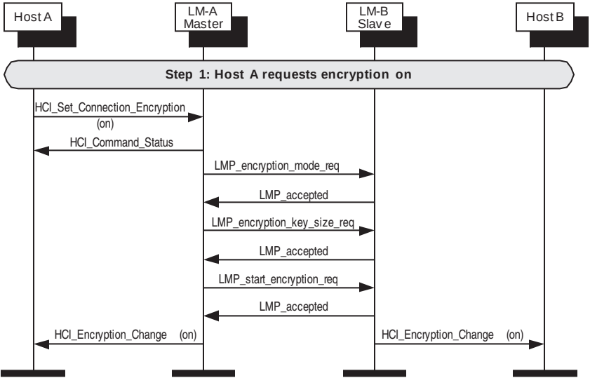
Figure 126—Encryption requested
