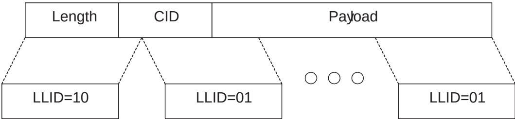
Figure 216—L2CAP fragmentation
