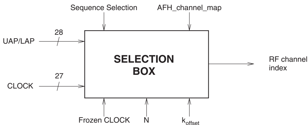
Figure 23—General block diagram of hop selection scheme
