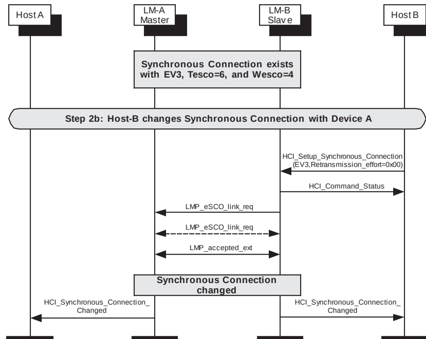
Figure 145—Slave renegotiates eSCO connection
