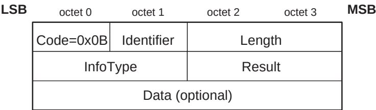
Figure 208—Information Response packet
