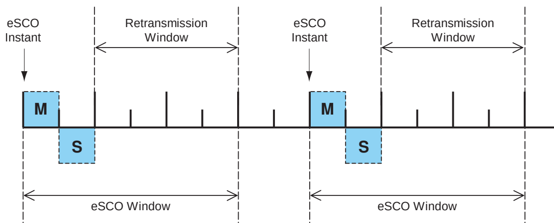
Figure 66—eSCO window details for single-slot packets
