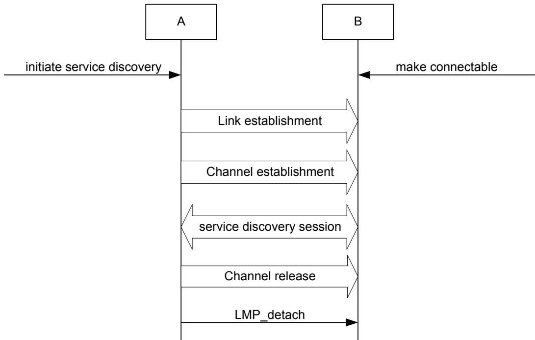
Figure B.21—SD procedure
