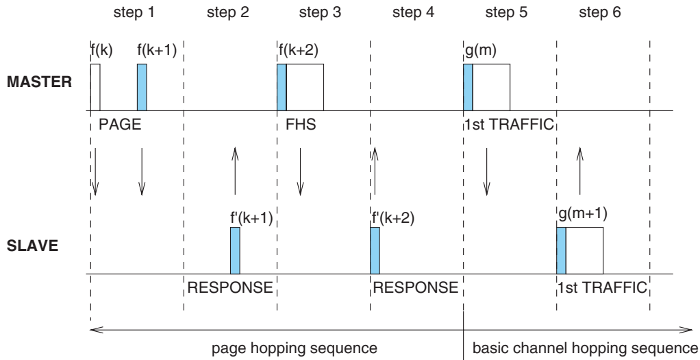
Figure 63—Messaging at initial connection when slave responds to second page message
