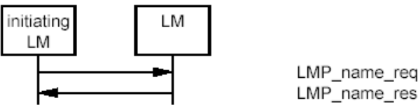
Sequence 43: Device’s name requested and responses.
