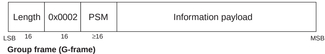
Figure 190—L2CAP PDU format in basic L2CAP mode on connectionless channel
