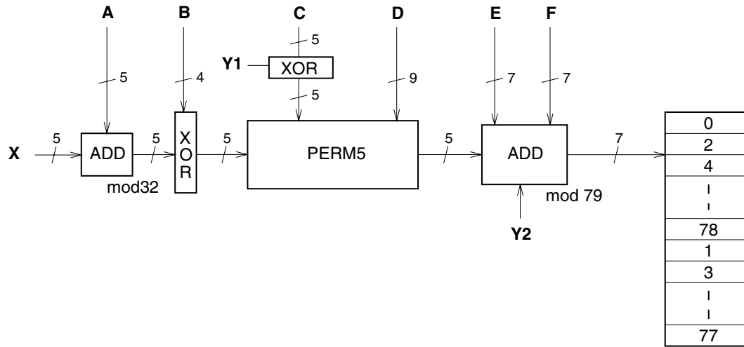
Figure 27—Block diagram of the basic hop selection kernel for the hop system
