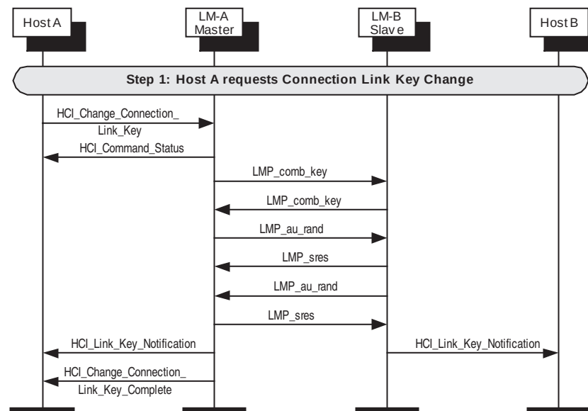
Figure 128—Change connection link key
