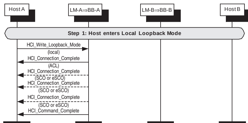
Figure 161—Entering local loopback mode
