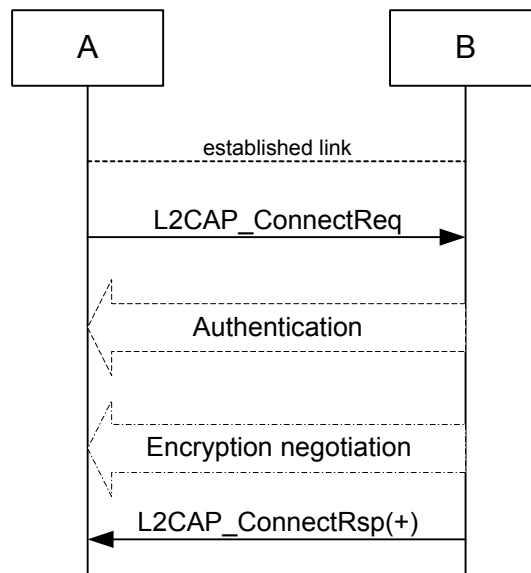
Figure B.15—Channel establishment procedure when the initiator (A) is in security mode 3 and the acceptor (B) is in security mode 2
