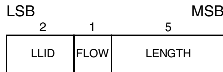
Figure 41—Payload header format for single-slot ACL packets
