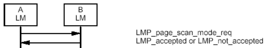
Sequence 16: Negotiation for page scan mode.
