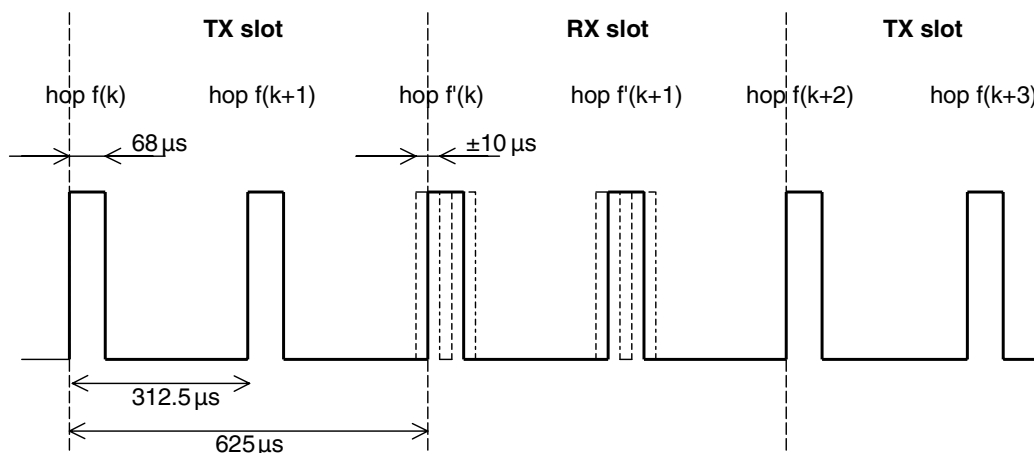
Figure 18—RX/TX cycle of transceiver in page mode
