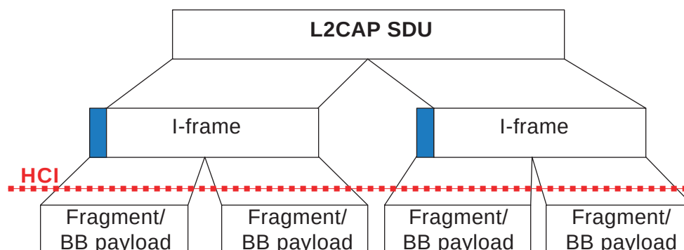
Figure 218—Segmentation and fragmentation of an SDU
