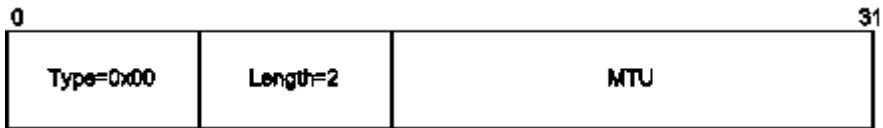
Figure 210—MTU option format
