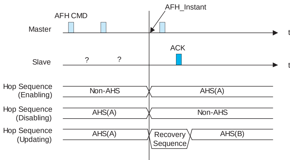
Figure 69—Recovery hop sequences
