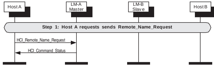
Figure 100—Remote name request
