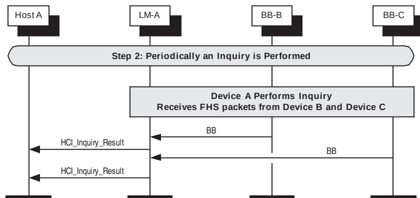
Figure 108—LM-A periodically performs an inquiry and reports result
