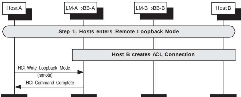
Figure 165—Entering remote loopback mode
