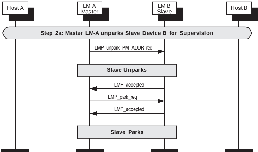
Figure 156—Master unparks slave for supervision
