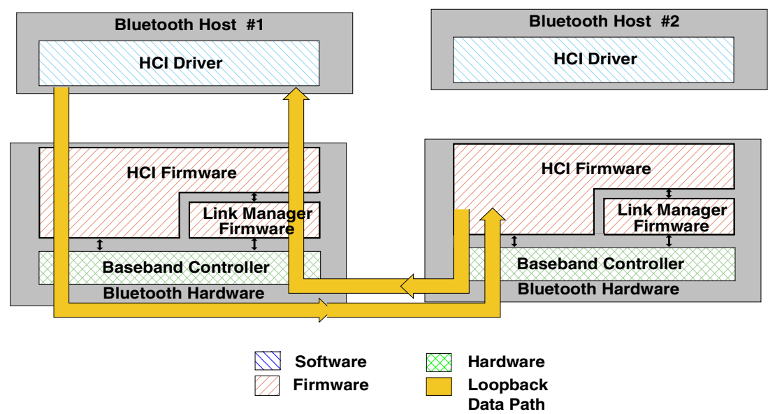
Figure 98—Remote loopback mode
