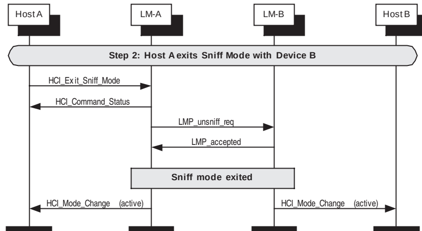
Figure 149—Exit SNIFF mode request
