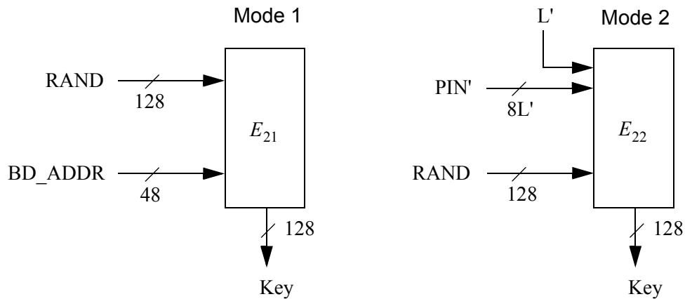
Figure 182—Key generating algorithm E_2 and its two modes
