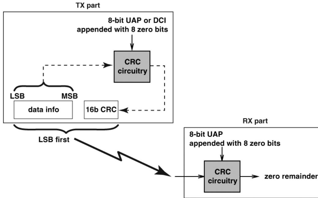
Figure 50—CRC generation and checking
