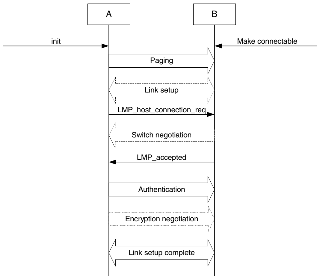
Figure B.13—Link establishment procedure when the paging device (A) is in security mode 3 and the paged device (B) is in security mode 1 or 2
