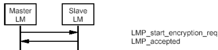
Sequence 34: Start of encryption.
