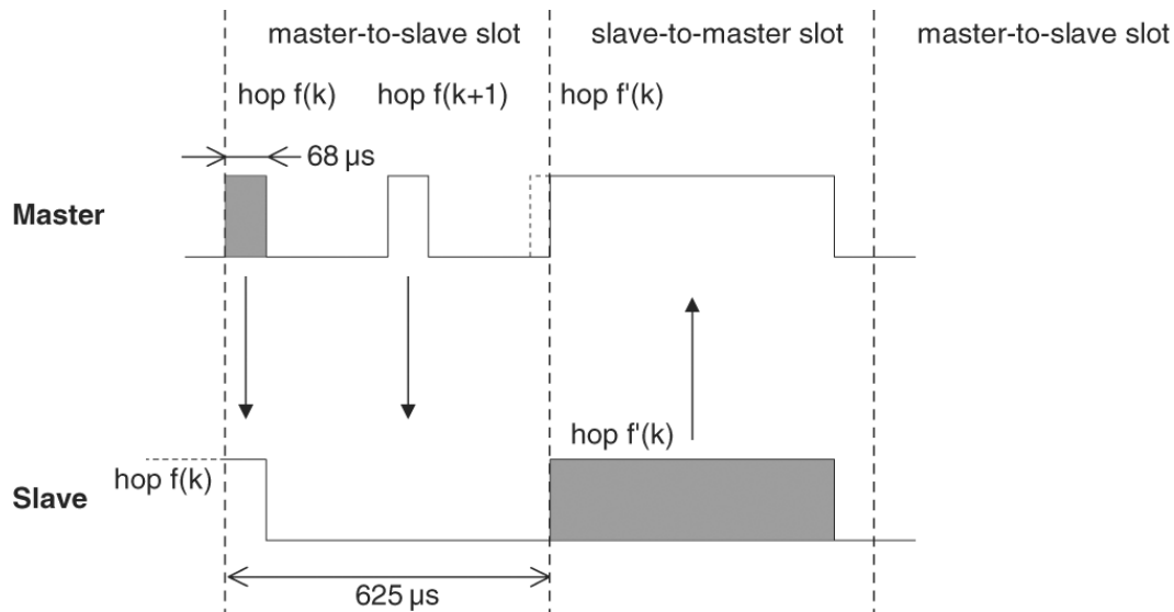
Figure 21—Timing of inquiry response packet on successful inquiry in first half slot
