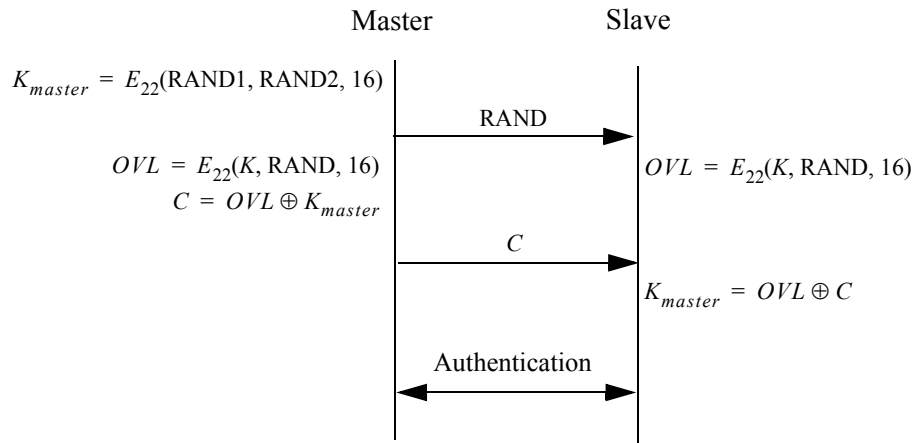
Figure 170—Master link key distribution and computation of the corresponding encryption key
