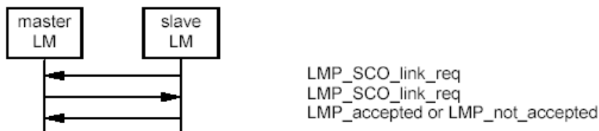
Sequence 63: Master accepts slave's request for an SCO link.
