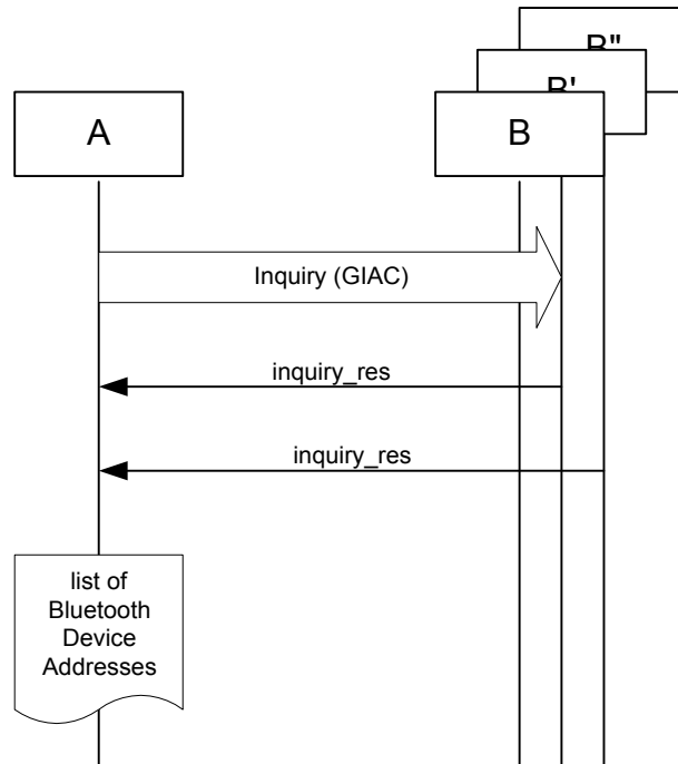
Figure B.6—General inquiry, where device B is in nondiscoverable mode, device B' is in limited discoverable mode, and device B'' is in general discoverable mode
