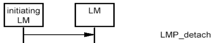
Sequence 1: Connection closed by sending LMP_detach.
