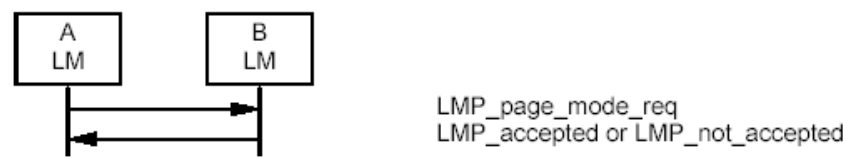
Sequence 15: Negotiation for page mode.
