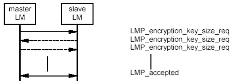
Sequence 32: Encryption key size negotiation successful.
