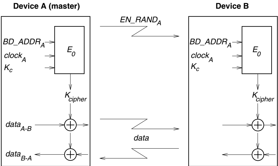
Figure 172—Functional description of the encryption procedure
