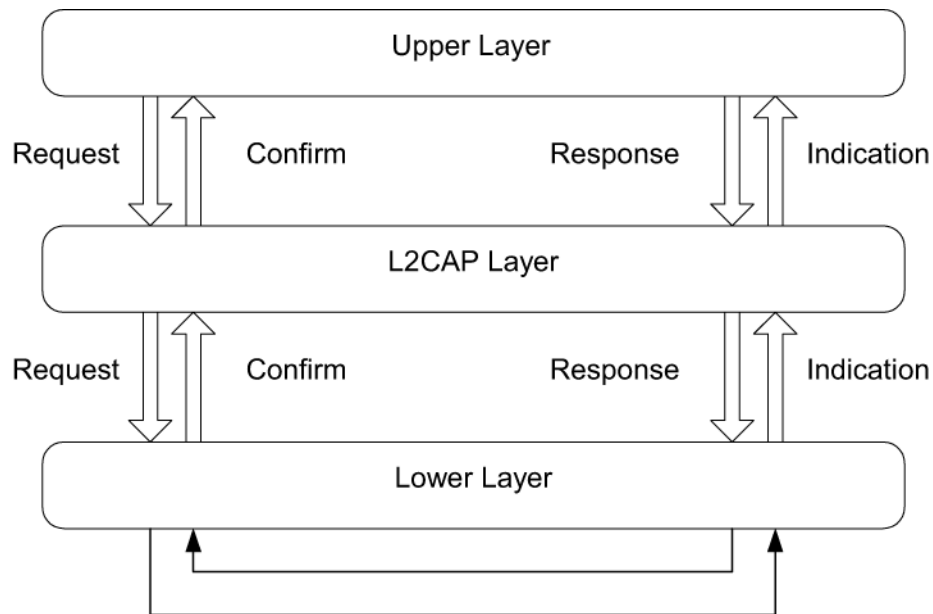
Figure 188—L2CAP transaction model
