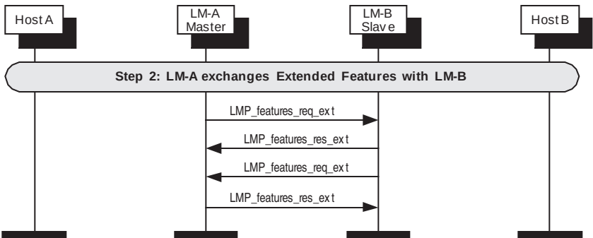
Figure 113—LM-A and LM-B exchange features
