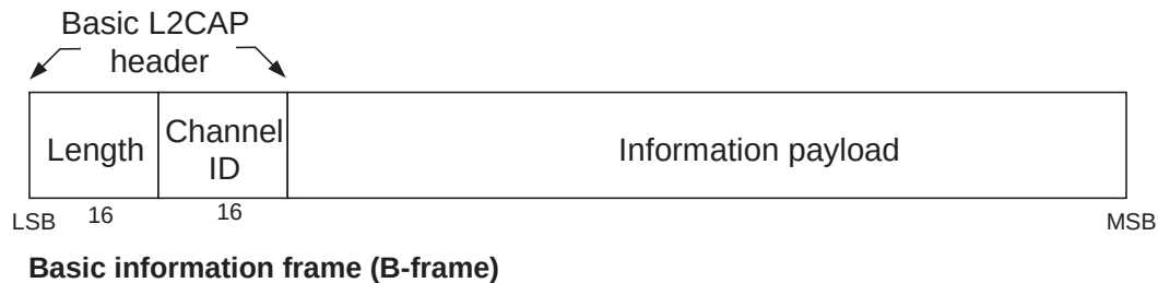
Figure 189—PDU format in basic L2CAP mode on connection-oriented channels (field sizes in bits)
