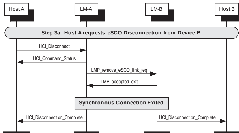
Figure 146—Synchronous disconnection of eSCO connection
