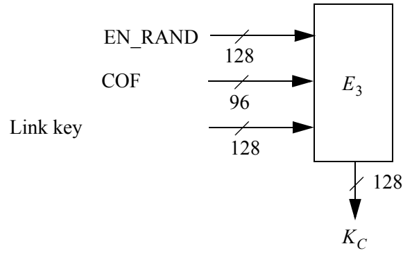
Figure 183—Generation of the encryption key
