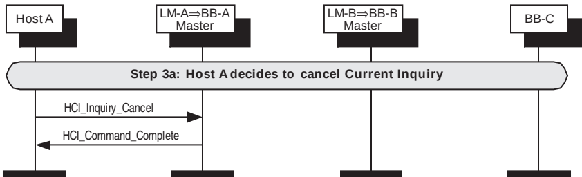
Figure 105—Host A cancels inquiry
