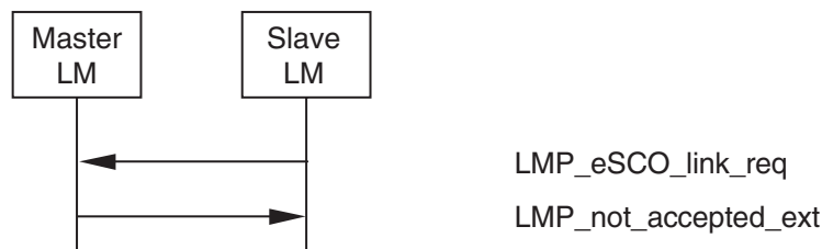
Sequence 67: Master rejects slave's request for an eSCO link.
