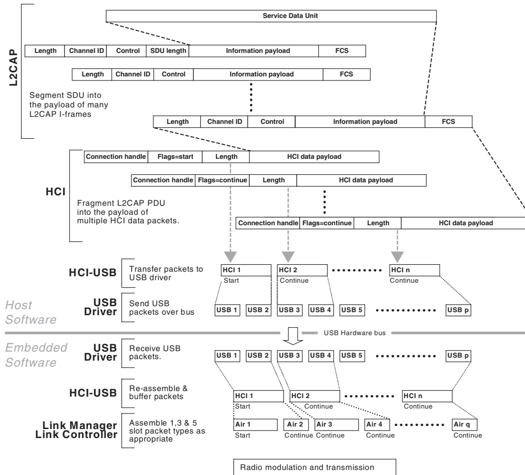
Figure 219—Example of segmentation and fragment processes in device with HCI
