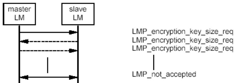
Sequence 33: Encryption key size negotiation failed.
