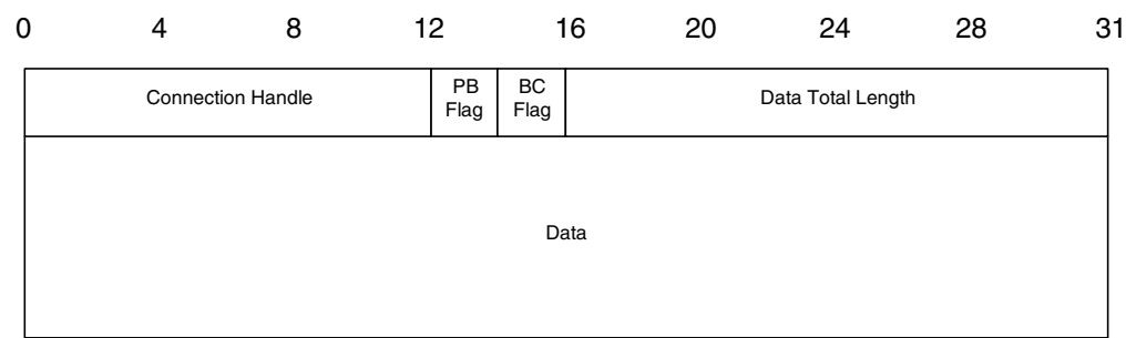
Figure 94—HCI ACL data packet
