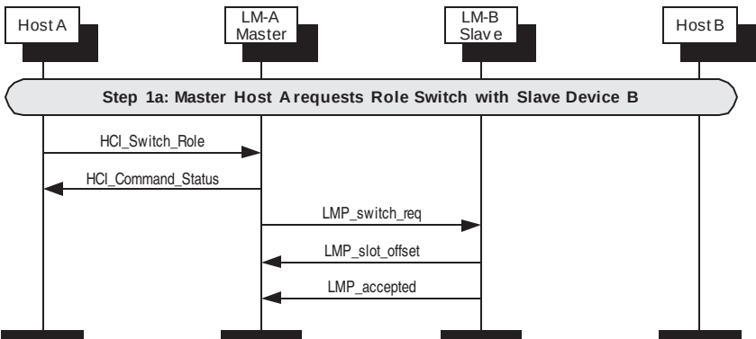
Figure 136—Master requests role switch
