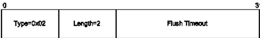
Figure 211—Flush timeout option format
