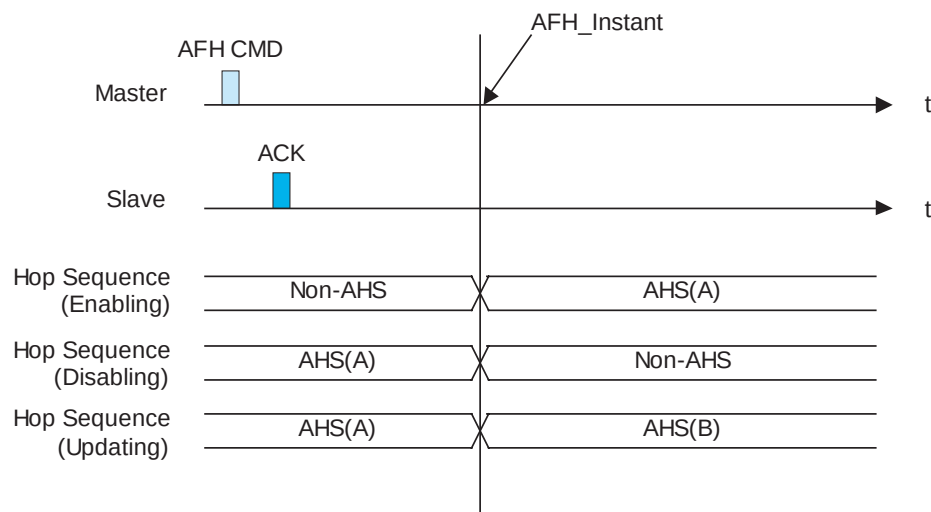
Figure 68—Successful hop sequence switching
