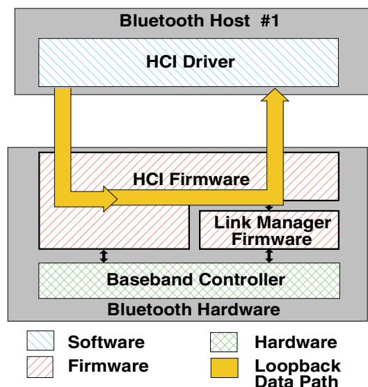
Figure 97—Local loopback mode
