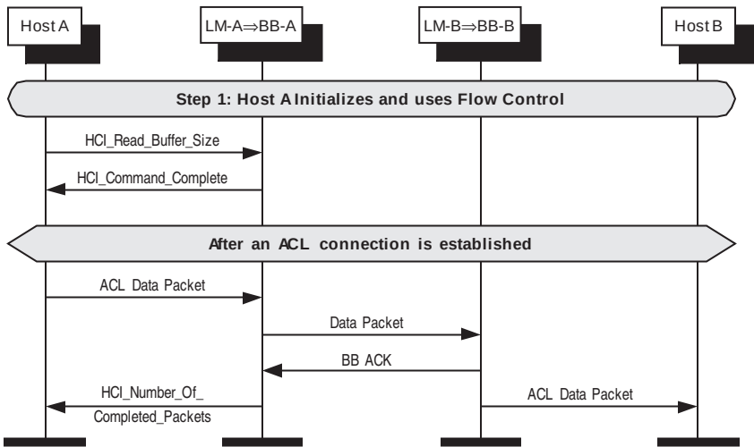
Figure 159—Host-to-controller flow control
