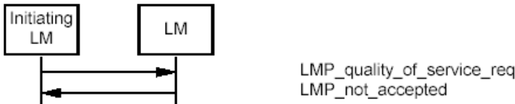
Sequence 14: Device rejects new QoS.
