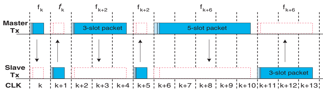
Figure 26—Example of the same channel mechanism
