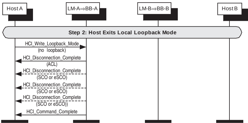
Figure 164—Exiting local loopback mode
