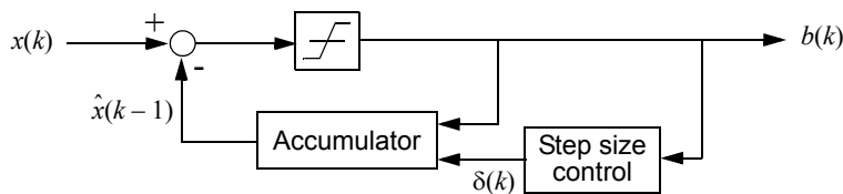
Figure 77—Block diagram of CVSD encoder with syllabic companding
