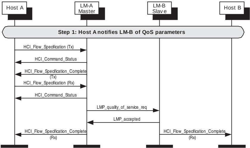
Figure 135—QoS flow specification
