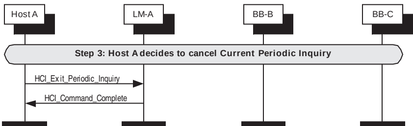
Figure 110—Host A decides to exit periodic inquiry
