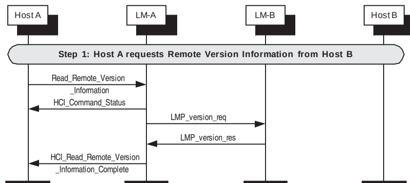
Figure 134—Read remote version information
