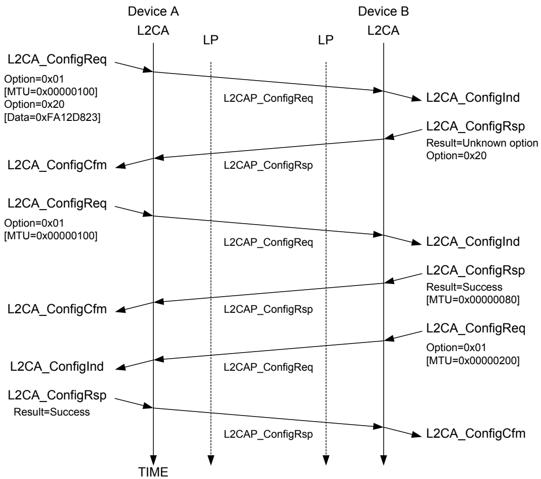
Figure 224—Dealing with unknown options
