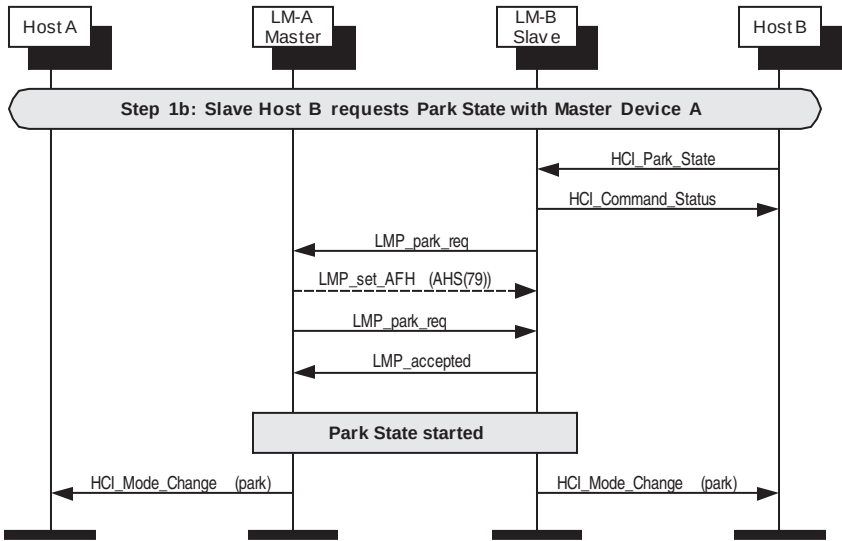
Figure 155—PARK state request from slave
