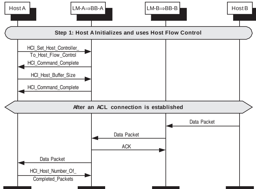
Figure 160—Controller-to-host flow control
