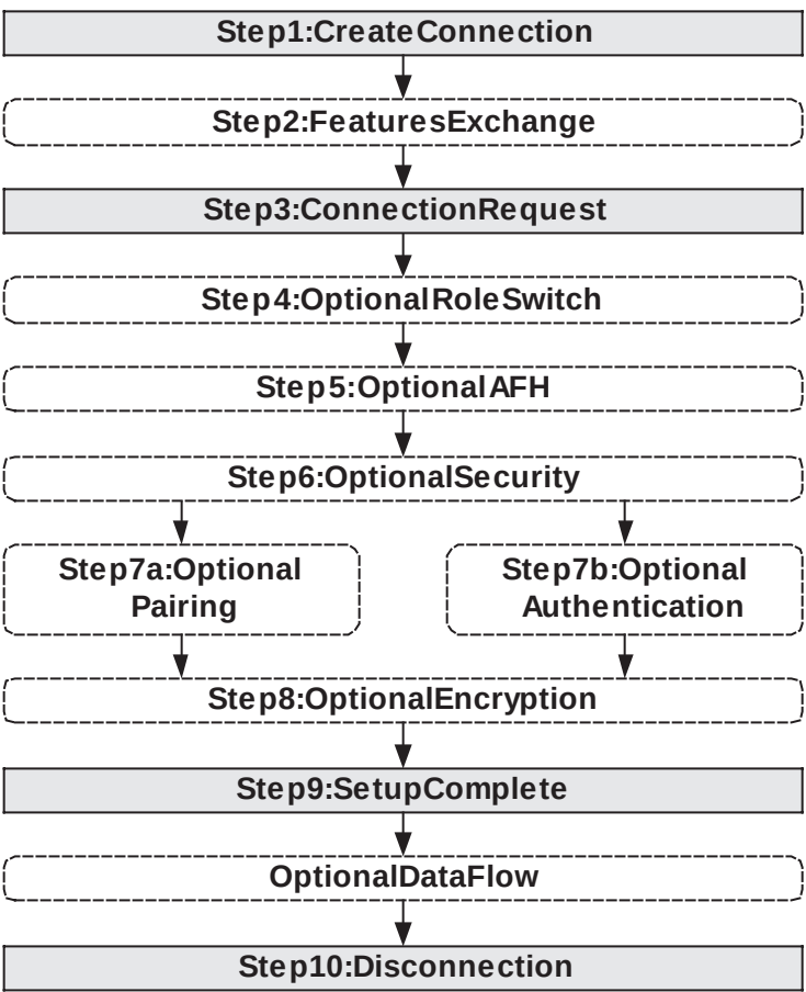
Figure 111—Overview diagram for connection setup
