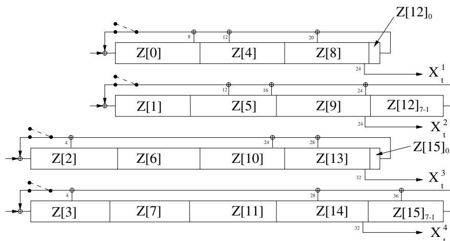
Figure 176—Distribution of the 128 last generated output symbols within the LFSRs
