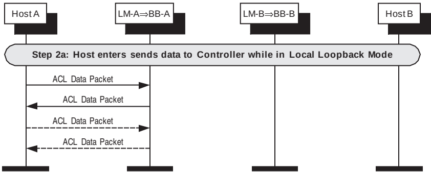
Figure 162—Looping back data in local loopback mode
