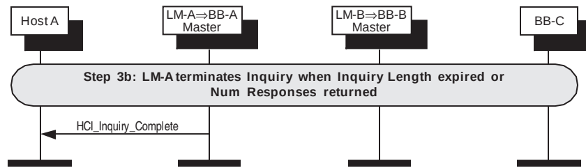
Figure 106—LM-A terminates current inquiry
