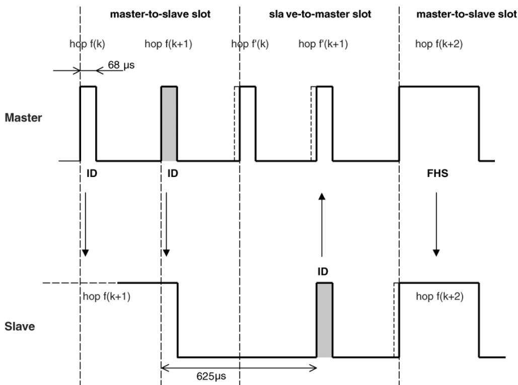
Figure 20—Timing of page response packets on successful page in second half slot
