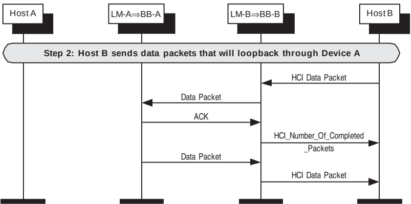
Figure 166—Looping back data in remote loopback mode
