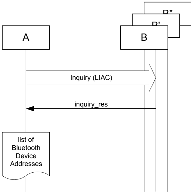
Figure B.7—Limited inquiry, where device B is in nondiscoverable mode, device B' is in limited discoverable mode, and device B'' is in general discoverable mode
