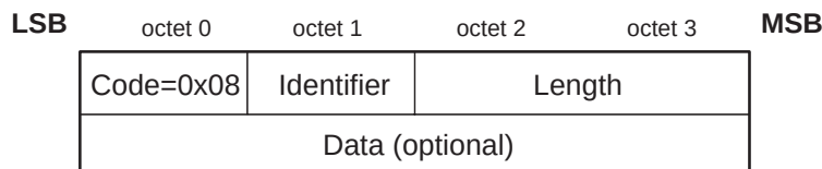
Figure 205—Echo Request packet
