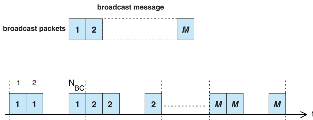
Figure 58—Broadcast repetition scheme
