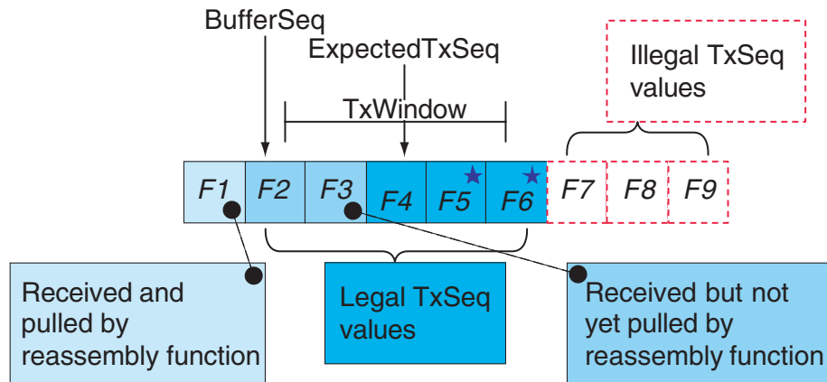
Figure 221—Example of receiver side
