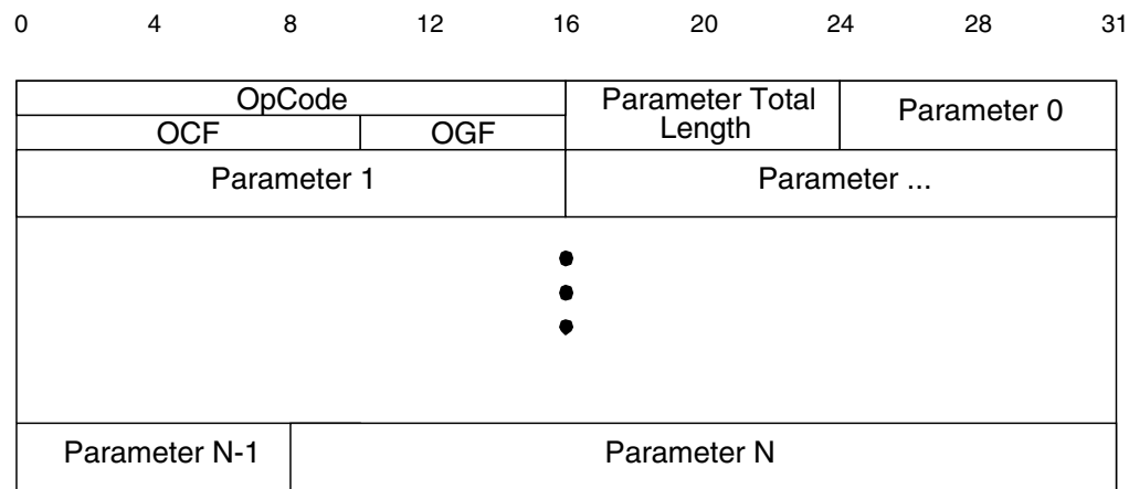
Figure 93—HCI command packet
