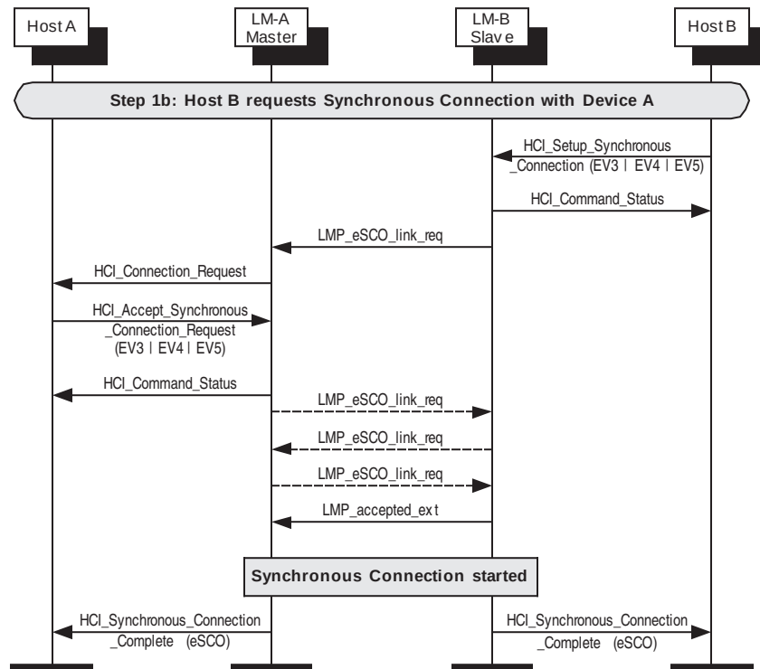
Figure 140—Slave requests synchronous EV3, EV4, OR EV5 connection
