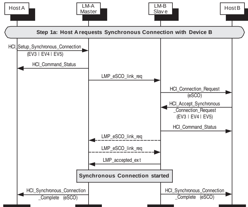
Figure 139—Master requests synchronous EV3, EV4, OR EV5 connection
