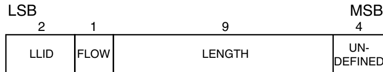
Figure 42—Payload header format for multislot ACL packets
