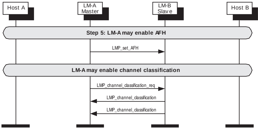
Figure 118—LM-A starts AFH
