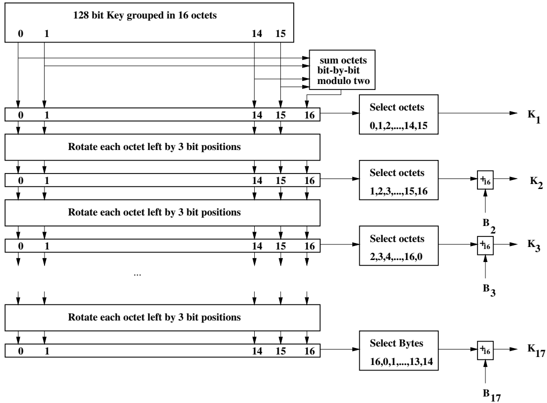
Figure 181—Key scheduling in A_r
