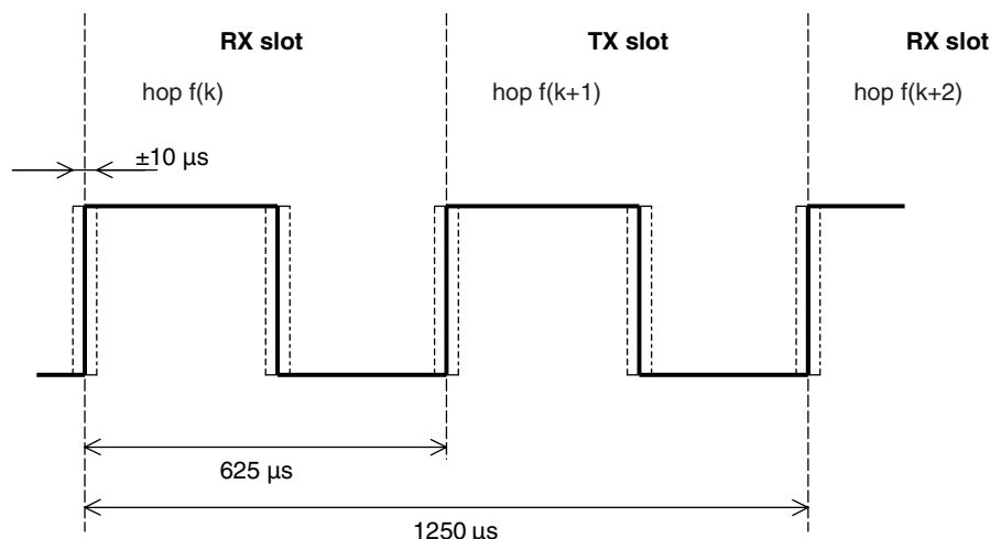
Figure 15—RX/TX cycle of slave transceiver for single-slot packets
