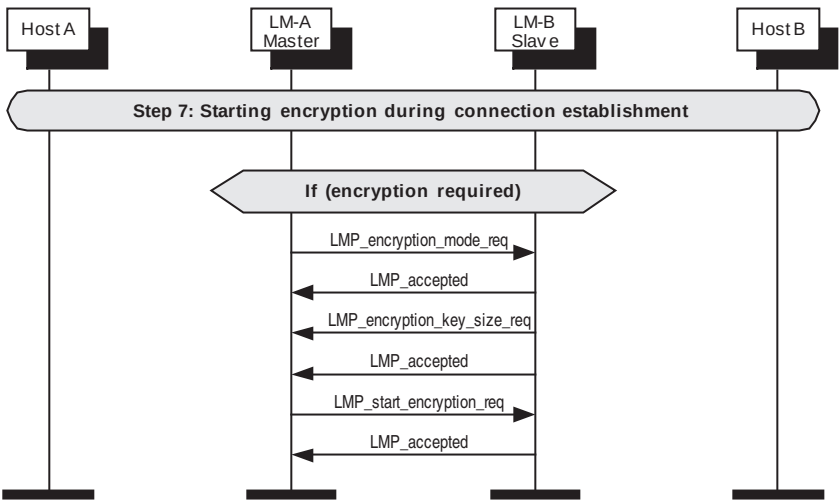
Figure 122—Starting encryption during connection setup
