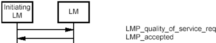
Sequence 13: Device accepts new QoS.
