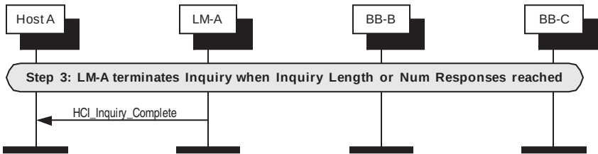
Figure 109—LM-A terminates current inquiry
