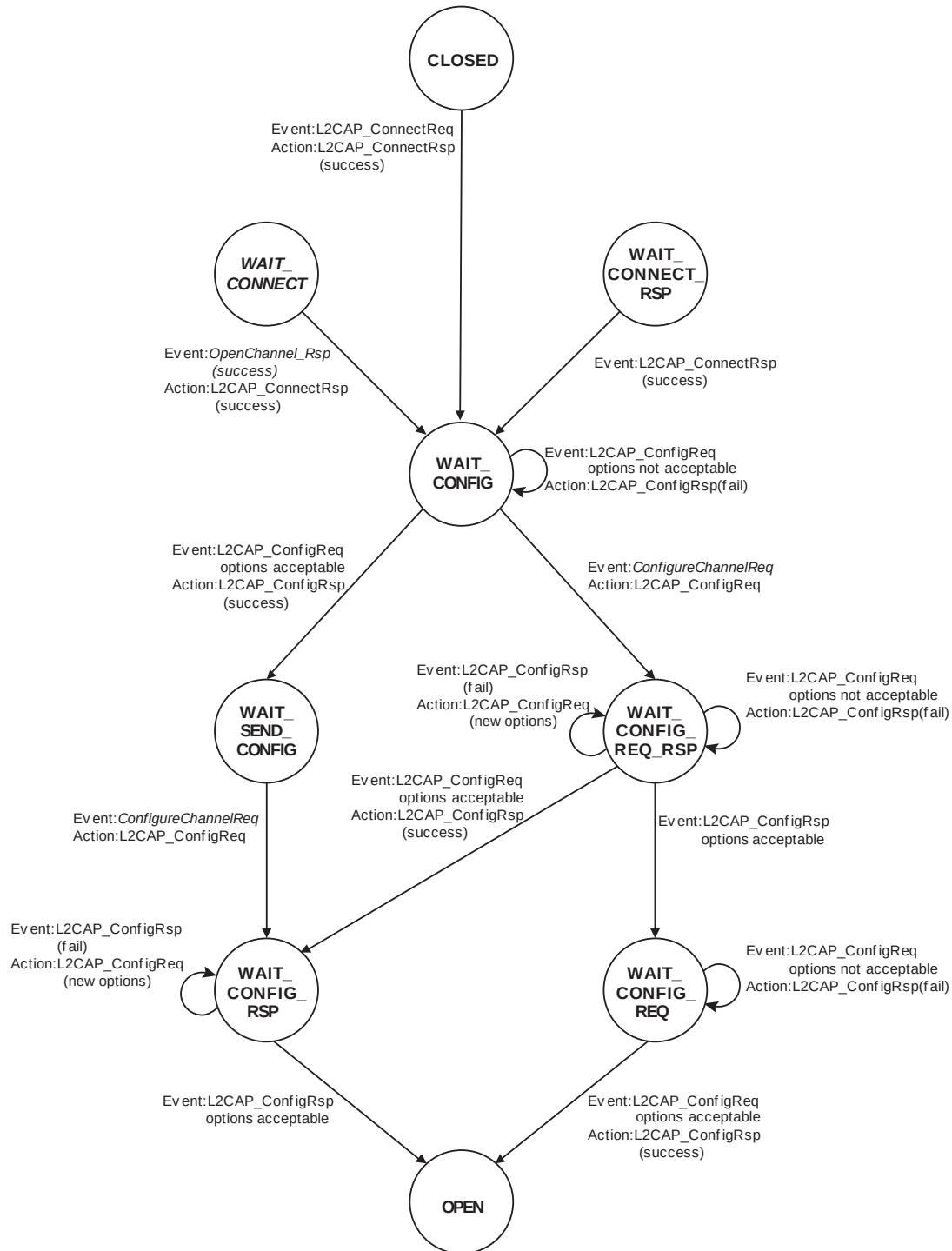
Figure 215—Configuration states and transitions
