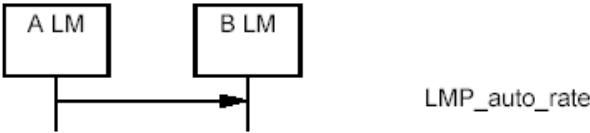
Sequence 10: Device A notifies device B to enable CQDDR.
