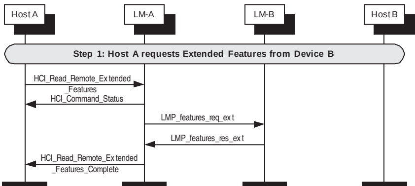
Figure 132—Read remote extended features
