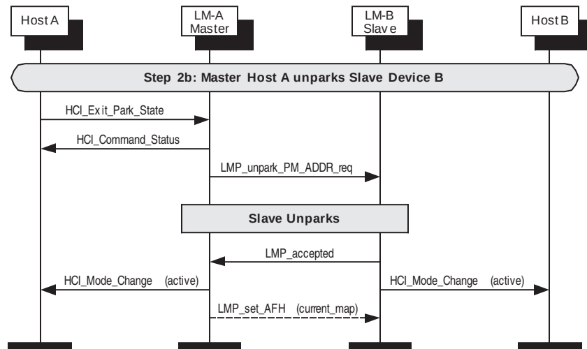
Figure 157—Master exits PARK state with slave
