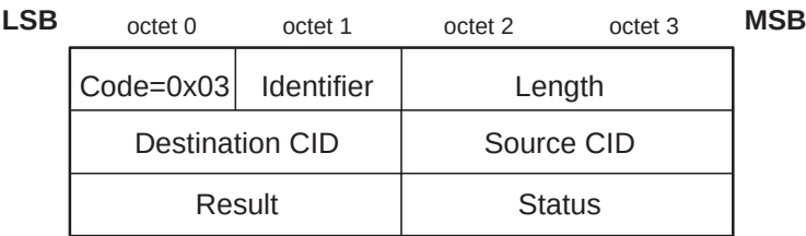
Figure 198—Connection Response packet
