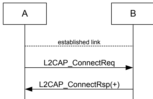
Figure B.16—Channel establishment procedure when the initiator (A) is in security mode 3 and the acceptor (B) is in security mode 1 or 3
