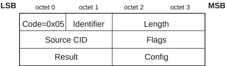
Figure 201—Configuration Response packet
