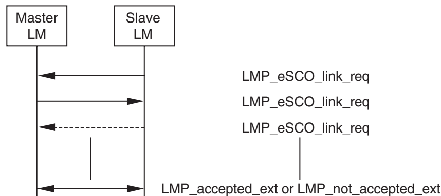
Sequence 66: Slave requests an eSCO link.
