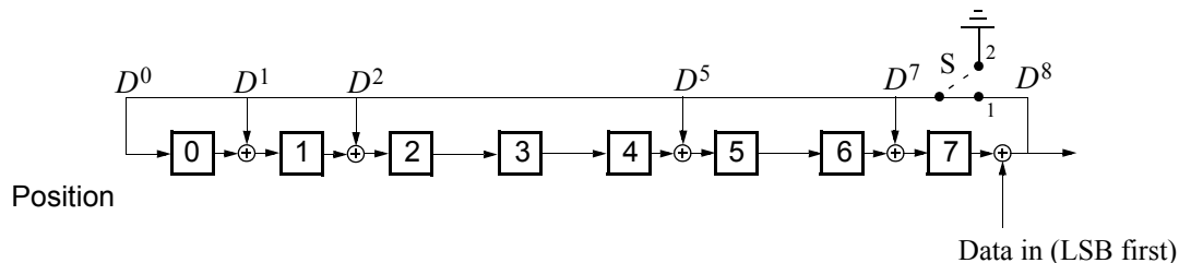
Figure 45—The LFSR circuit generating the HEC
