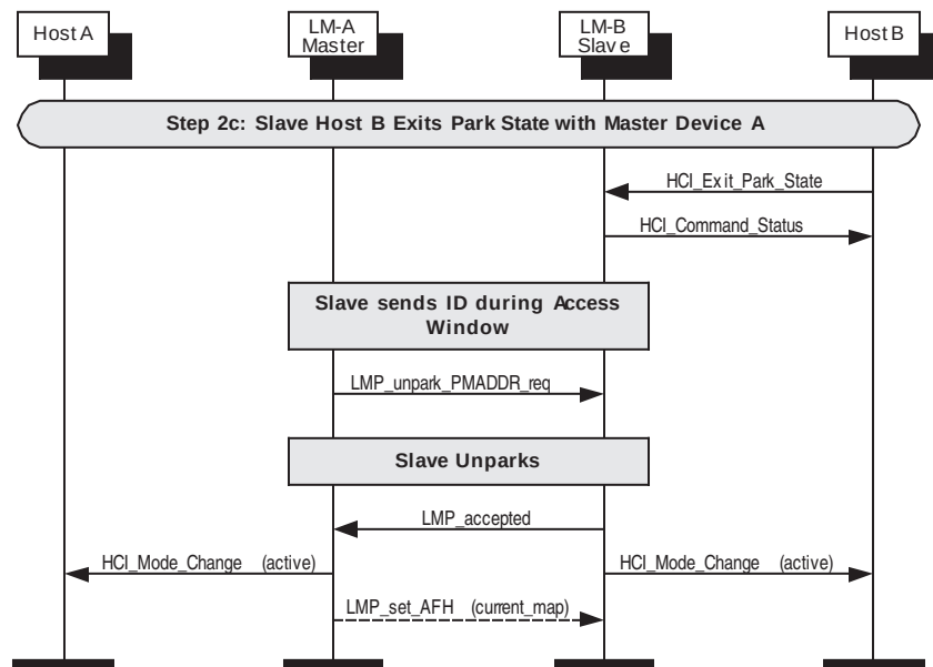
Figure 158—Slave exits PARK state with master
