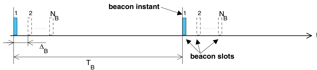
Figure 72—General beacon train format
