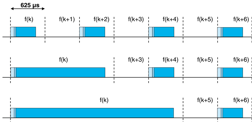
Figure 25—Single- and multislot packets
