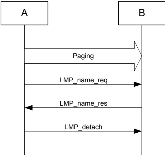
Figure B.8—Name request procedure
