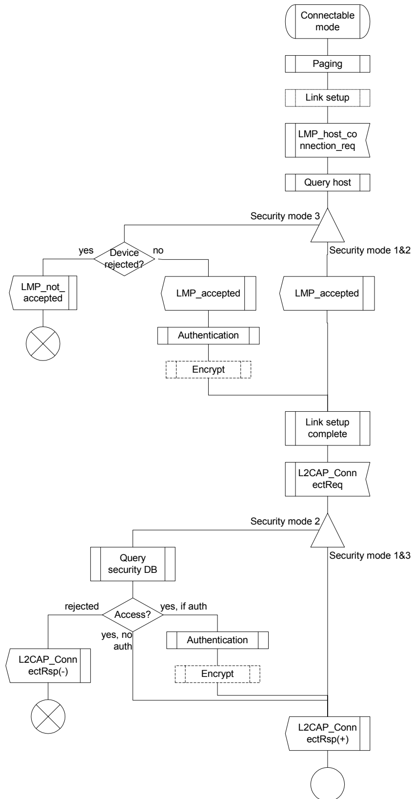
Figure B.5—Illustration of channel establishment using different security modes
