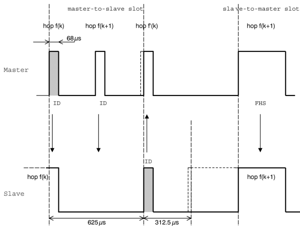
Figure 19—Timing of page response packets on successful page in first half slot
