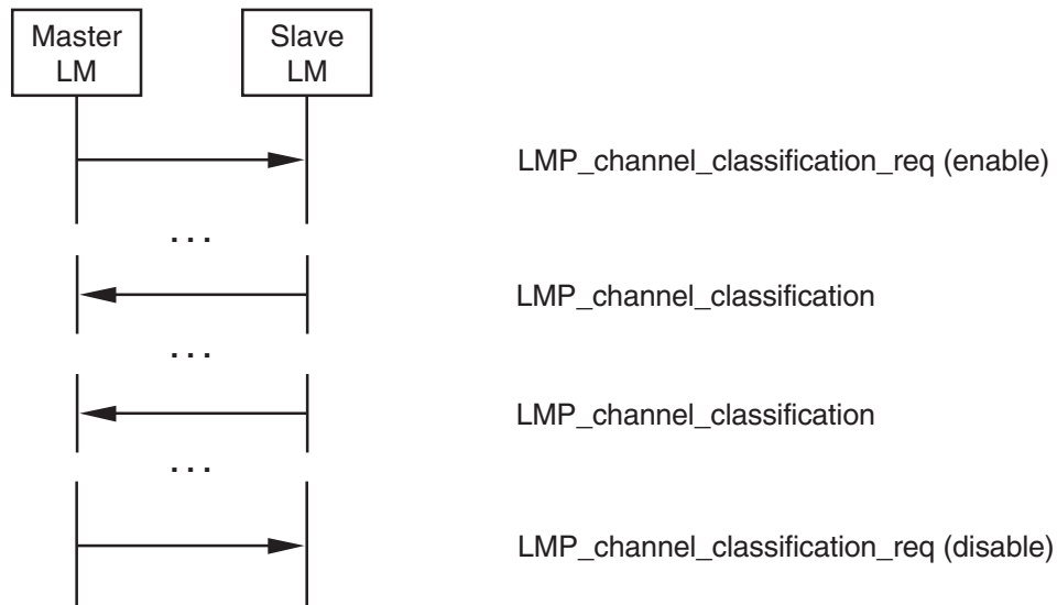
Sequence 8: Channel classification reporting.
