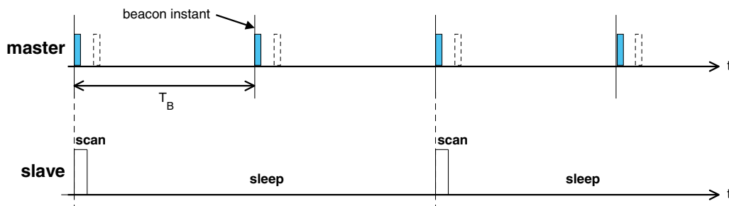
Figure 76—Extended sleep interval of parked slaves
