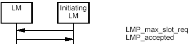
Sequence 18: Device requests a maximum number of slots. Remote device accepts.
