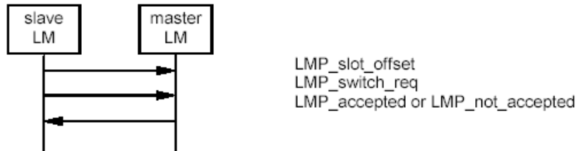
Sequence 45: Role switch (slave initiated).
