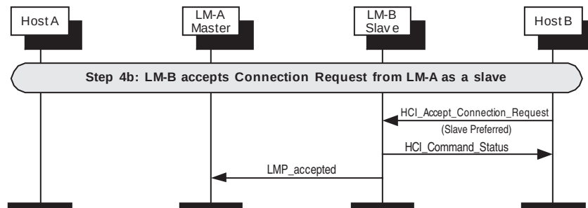
Figure 116—Device B accepts connection request
