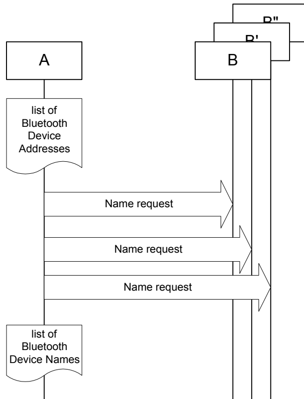
Figure B.9—Name discovery procedure
