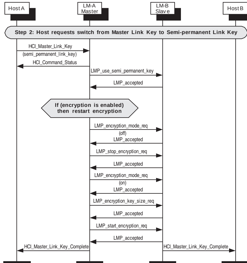
Figure 130—Change to semi permanent link key
