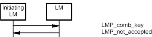
Sequence 28: Change of the link key not possible since the other device uses a unit key.
