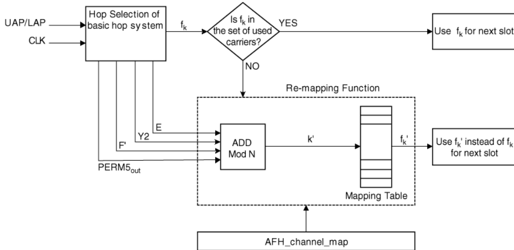
Figure 31—Block diagram of adaptive hop selection mechanism
