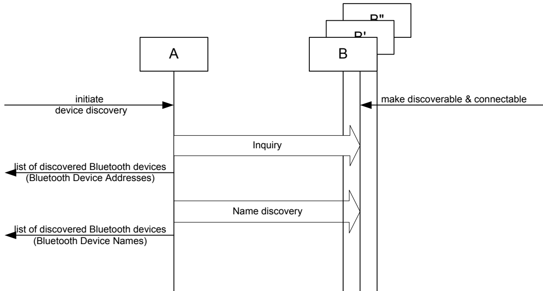
Figure B.10—Device discovery procedure
