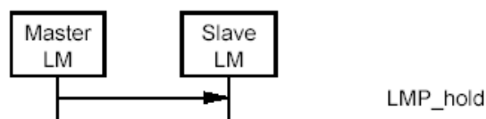
Sequence 47: Master forces slave into HOLD mode.
