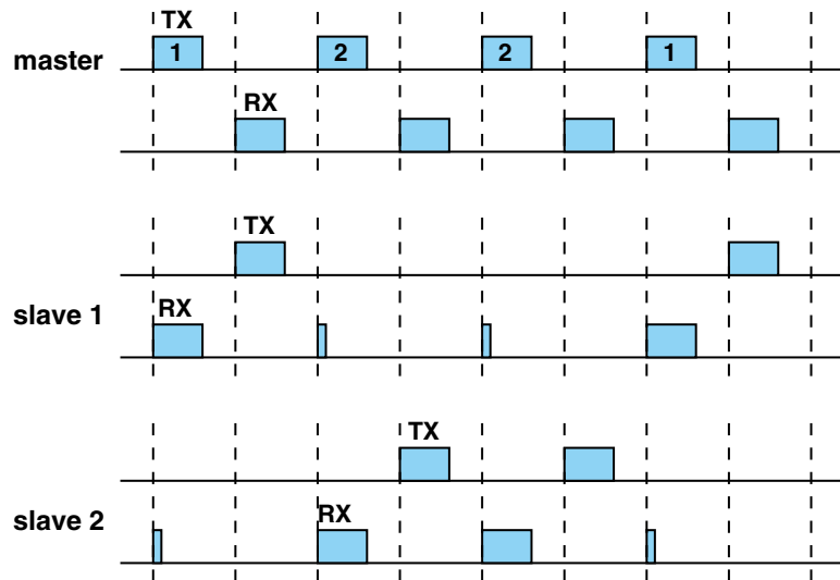
Figure 65—RX/TX timing in multislave configuration
