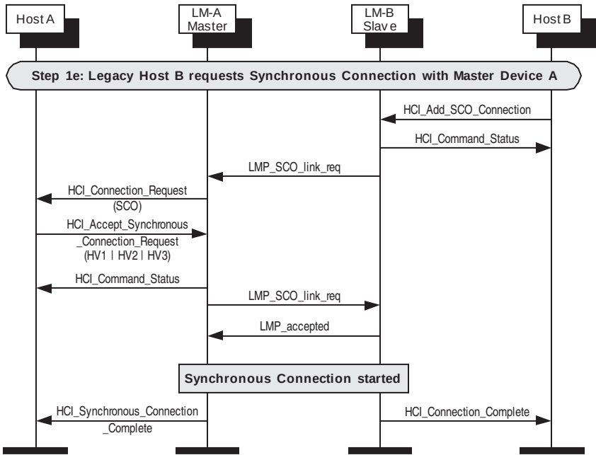
Figure 143—Any device that supports only SCO connections requests a synchronous connection with a device
