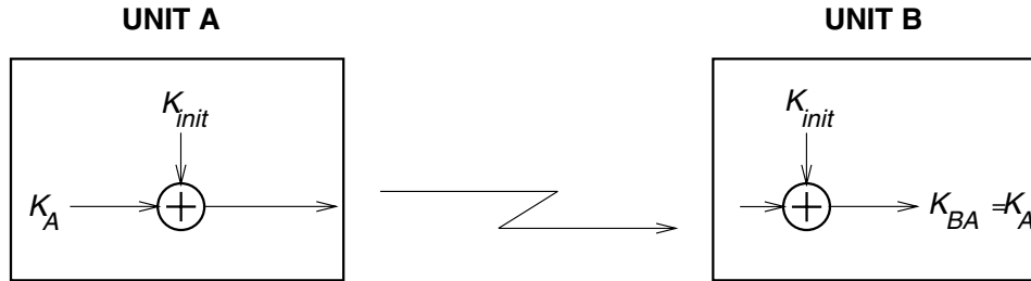
Figure 168—Generating a unit key
