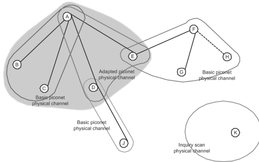
Figure 6—Example of IEEE 802.15.1-2005 topology
