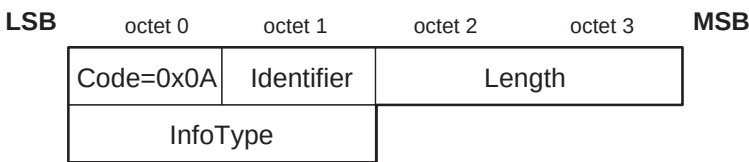
Figure 207—Information Request packet
