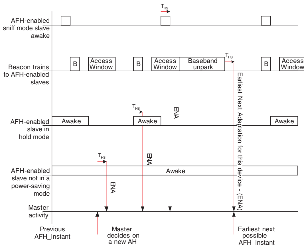
Figure 83—Timing constraint on AFH_Instant with slaves in PARK, HOLD, and SNIFF
