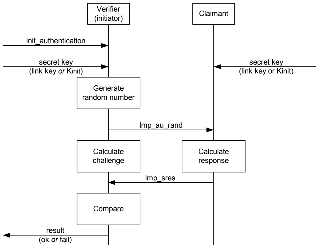
Figure B.19—LMP authentication as defined by Clause 9
