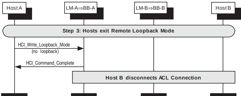
Figure 167—Exiting remote loopback mode
