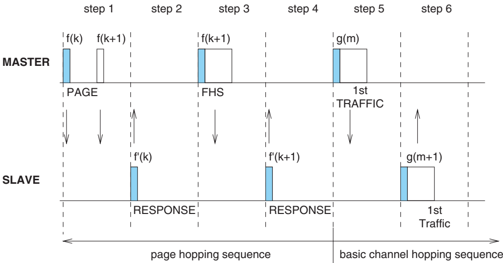
Figure 62—Messaging at initial connection when slave responds to first page message
