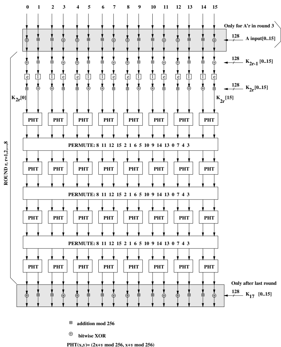
Figure 180—One round in A_r and A'_r
