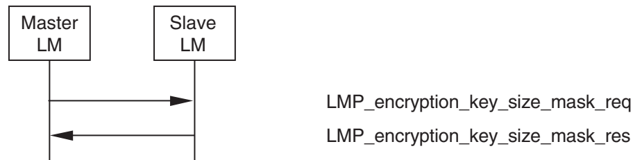
Sequence 36: Request for supported encryption key sizes.
