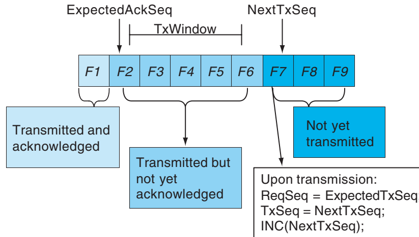
Figure 220—Example of transmitter side
