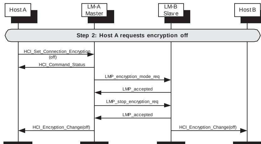
Figure 127—Encryption off requested
