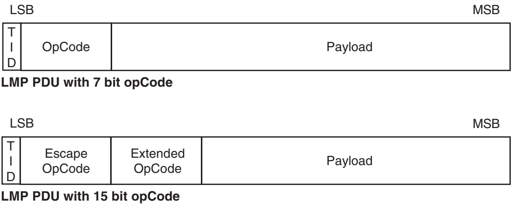
Figure 86—Payload body when LMP PDUs are sent
