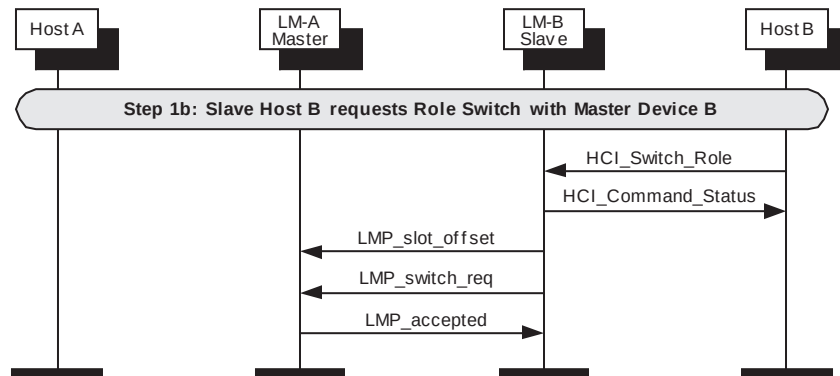
Figure 137—Slave requests role switch
