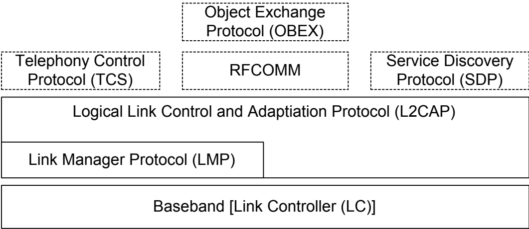
Figure B.2—Profile stack covered by this profile
