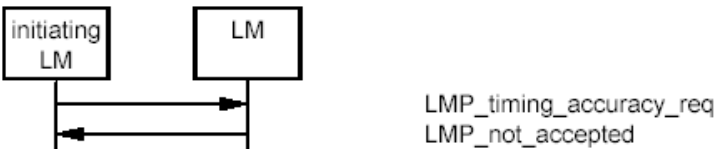
Sequence 38: The requested device does not support timing accuracy information.
