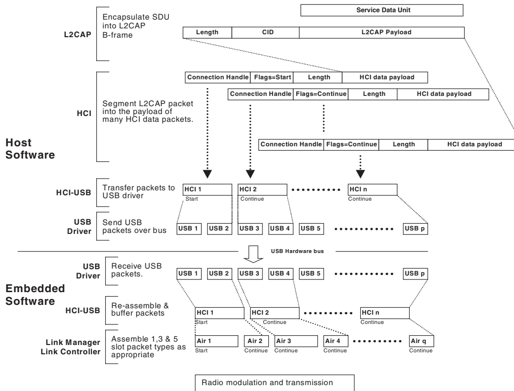
Figure 217—Example of fragmentation processes in a device with HCI
