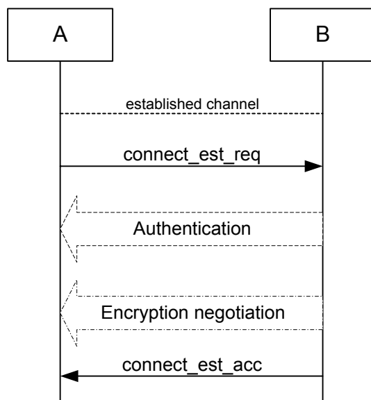
Figure B.17—Connection establishment procedure when the initiator (A) is in security mode 3 and the acceptor (B) is in security mode 2
