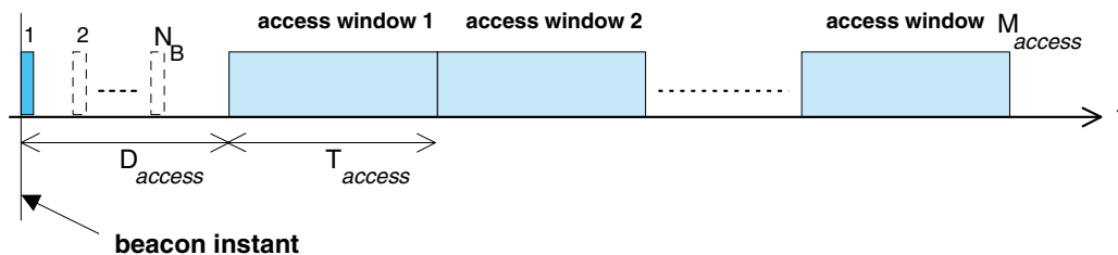
Figure 73—Definition of access window
