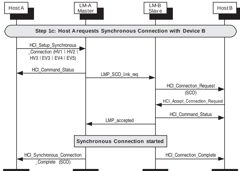
Figure 141—Master requests synchronous connection using SCO
