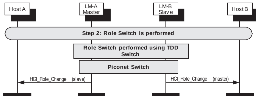
Figure 138—Role switch is performed
