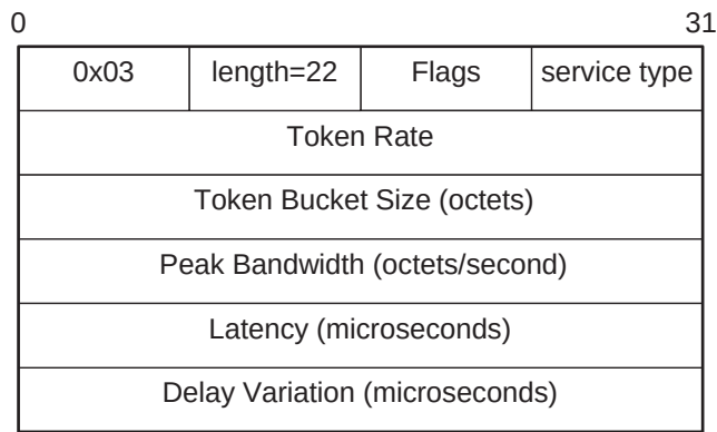
Figure 212—QoS option format containing flow specification
