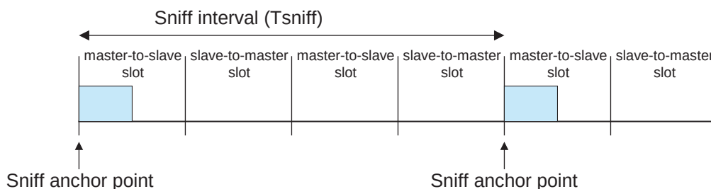
Figure 71—Sniff anchor points
