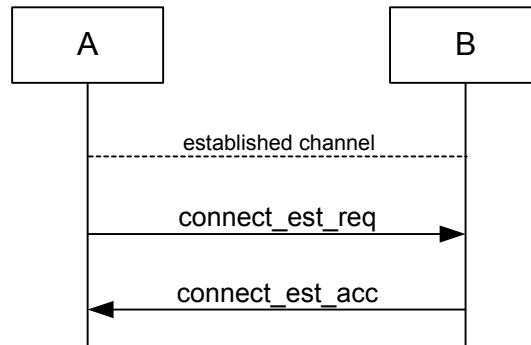
Figure B.18—Connection establishment procedure when the initiator (A) is in security mode 3 and the acceptor (B) is in security mode 1 or 3
