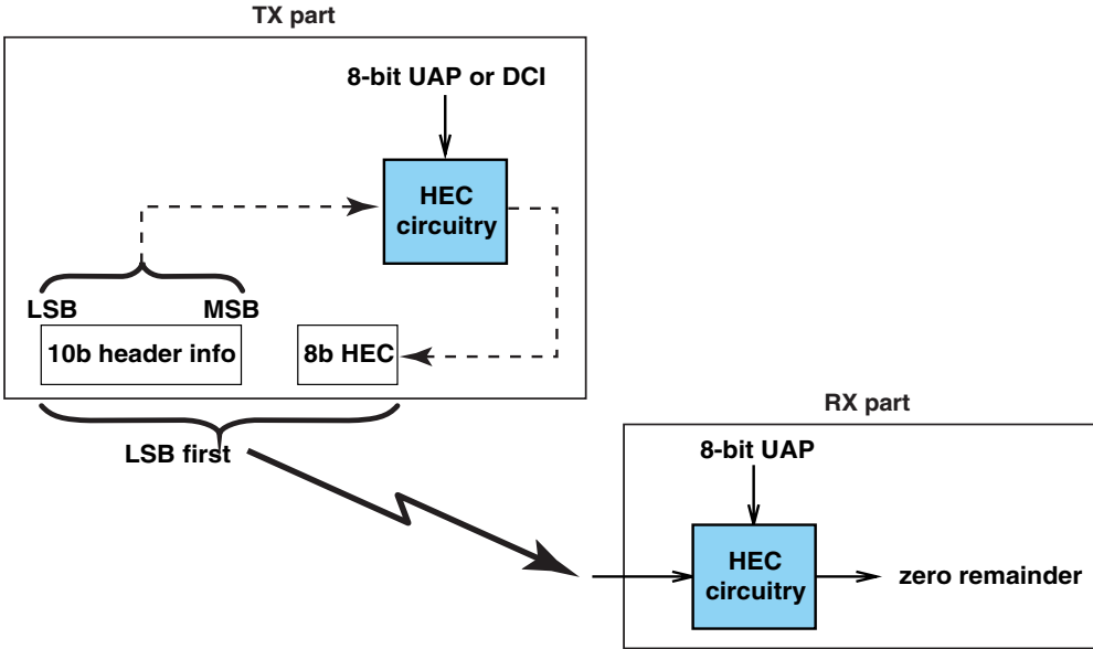
Figure 47—HEC generation and checking
