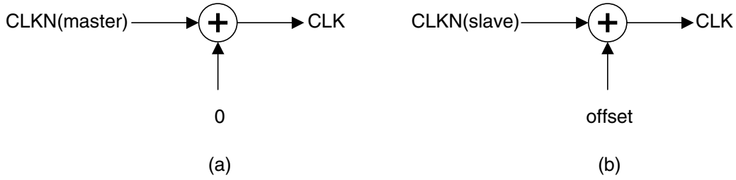
Figure 13—Derivation of CLK in master (a) and in slave (b)
