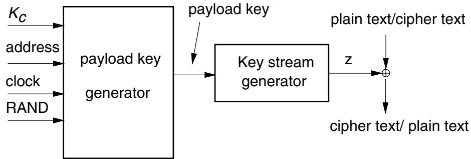
Figure 171—Stream ciphering for IEEE 802.15.1-2005 with E_0
