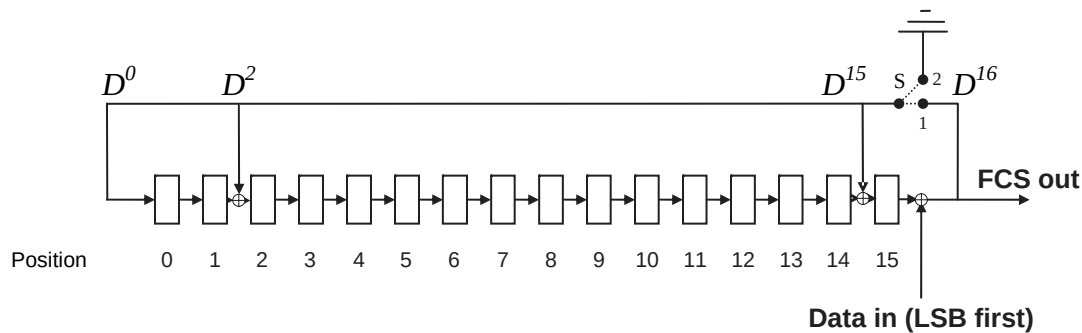
Figure 192—The LFSR circuit generating the FCS
