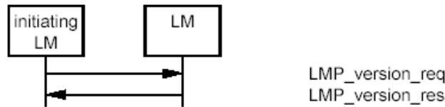
Sequence 40: Request for LMP version.
