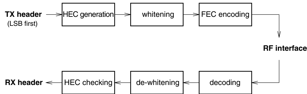
Figure 43—Header bit processes
