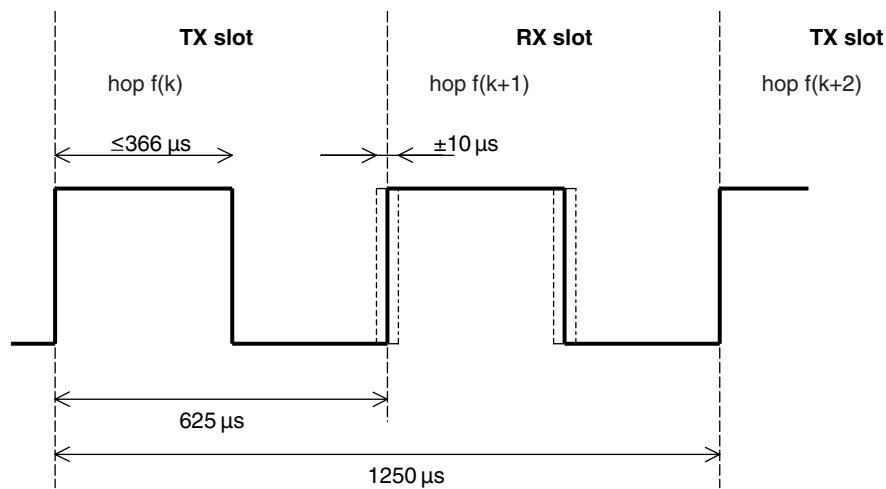
Figure 14—RX/TX cycle of master transceiver in normal mode for single-slot packets
