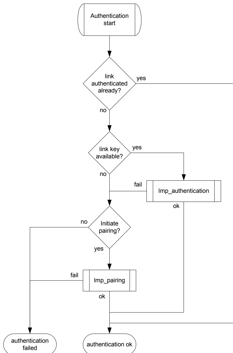
Figure B.4—Definition of the generic authentication procedure
