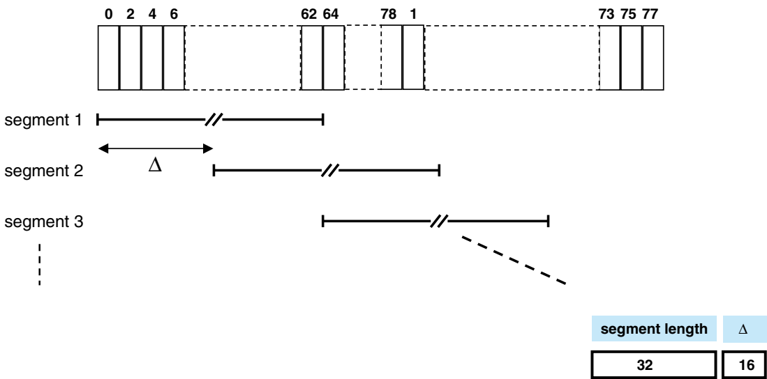
Figure 24—Hop selection scheme in CONNECTION state
