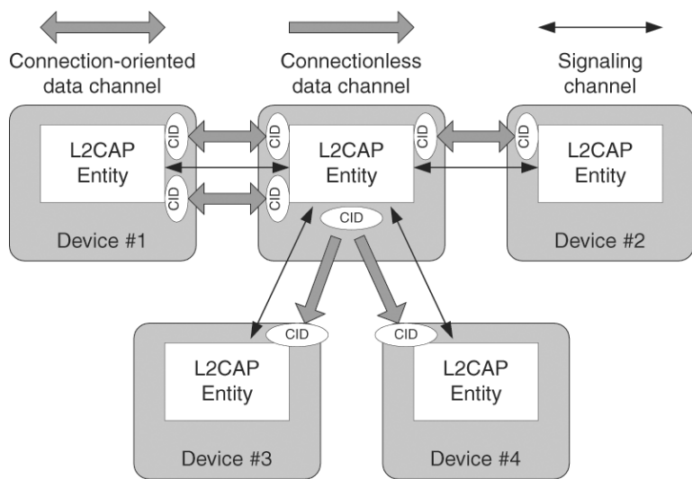
Figure 187—Channels between devices
