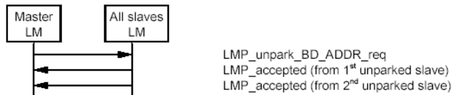
Sequence 57: Master unparks slaves addressed with their BD_ADDR.
