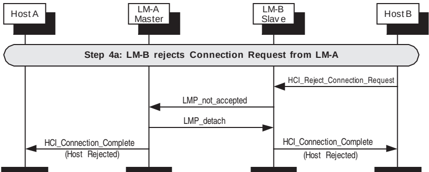
Figure 115—Device B rejects connection request
