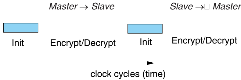
Figure 174—Overview of the operation of the encryption engine
