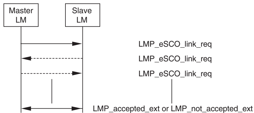
Sequence 65: Master requests an eSCO link.
