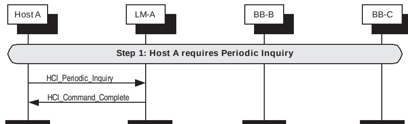
Figure 107—Host A starts periodic inquiry
