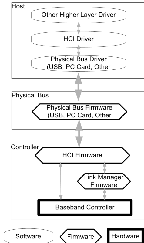
Figure 91—Overview of the lower software layers
