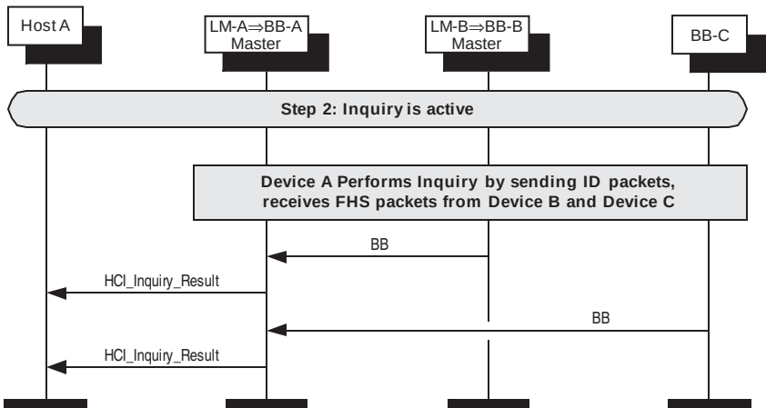
Figure 104—LM-A performs inquiry and reports result
