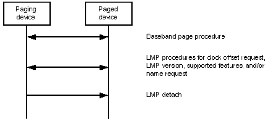
Figure 88—Connection establishment without host request
