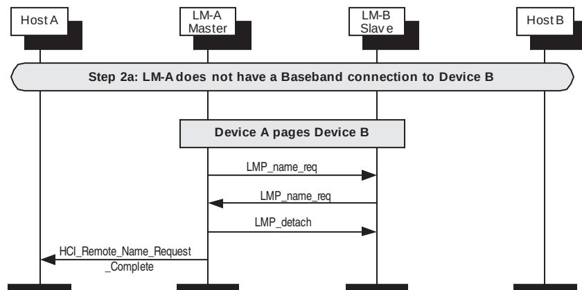
Figure 101—Remote name request if no current BB connection
