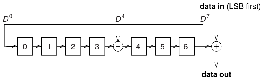
Figure 51—Data whitening LFSR
