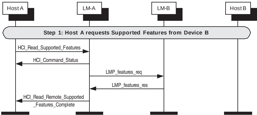
Figure 131—Read remote supported features
