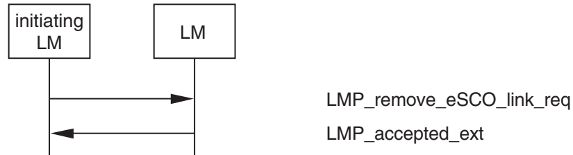
Sequence 68: eSCO link removed.
