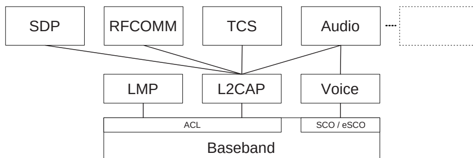
Figure 185—L2CAP data flows in IEEE 802.15.1-2005 architecture
