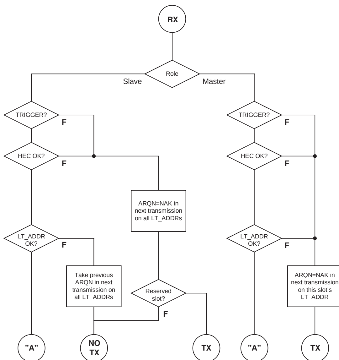
Figure 54—Stage 1 of the receive protocol for determining the ARQN bit
