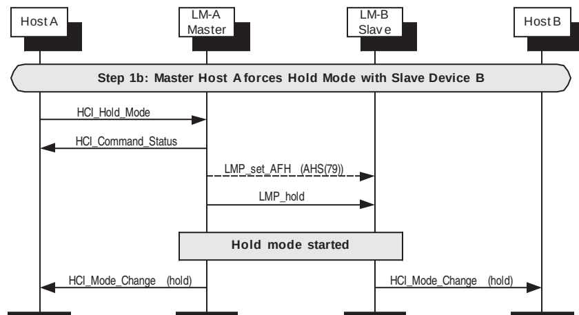
Figure 151—Master forces HOLD mode
