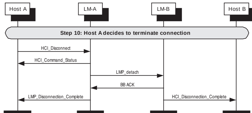
Figure 124—Host A decides to disconnect
