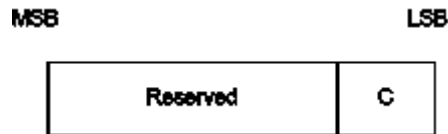
Figure 200—Configuration Request packet Flags field format
