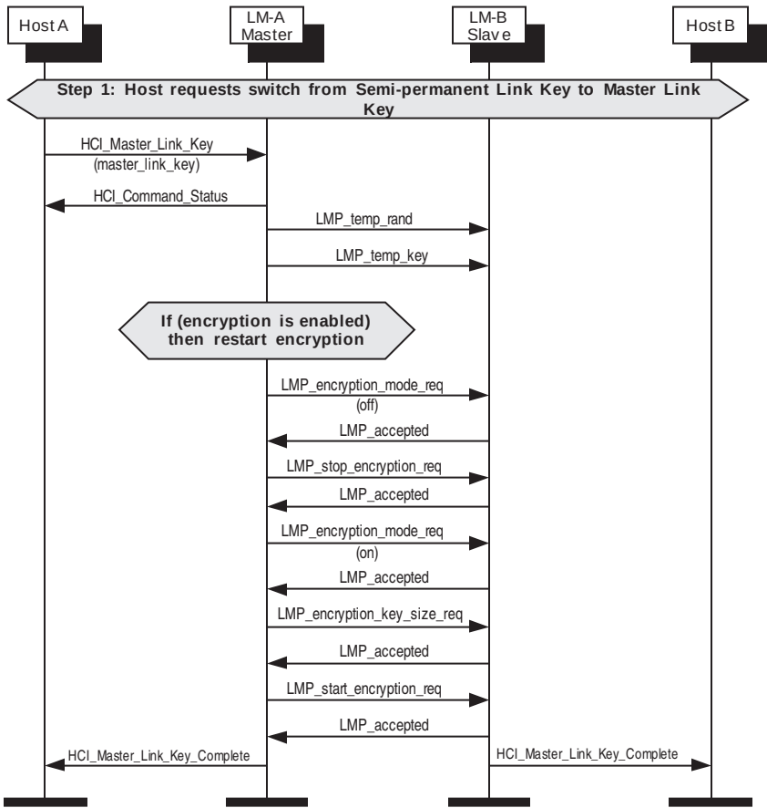
Figure 129—Change to master link key
