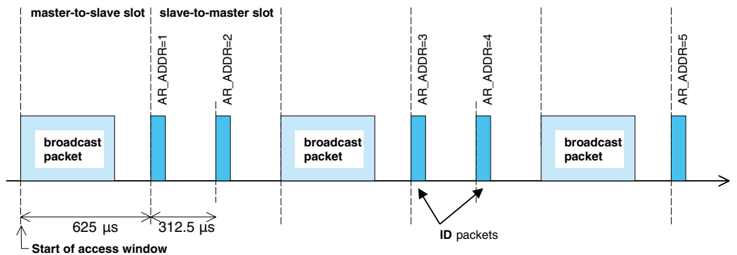
Figure 74—Access procedure applying the polling technique
