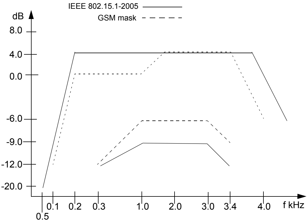
Figure 82—Plot of recommended frequency mask for IEEE 802.15.1-2005 with GSM send frequency mask given for comparison
