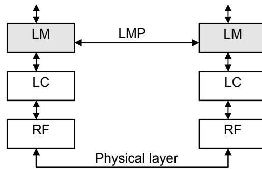
Figure 84—LMP signalling
