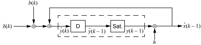
Figure 79—Accumulator procedure
