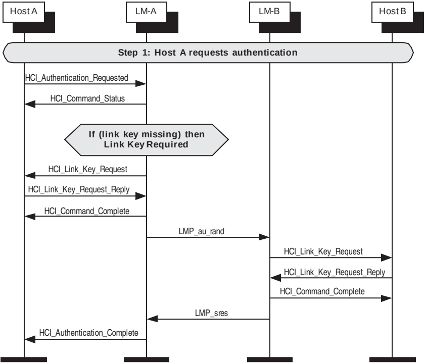
Figure 125—Authentication requested
