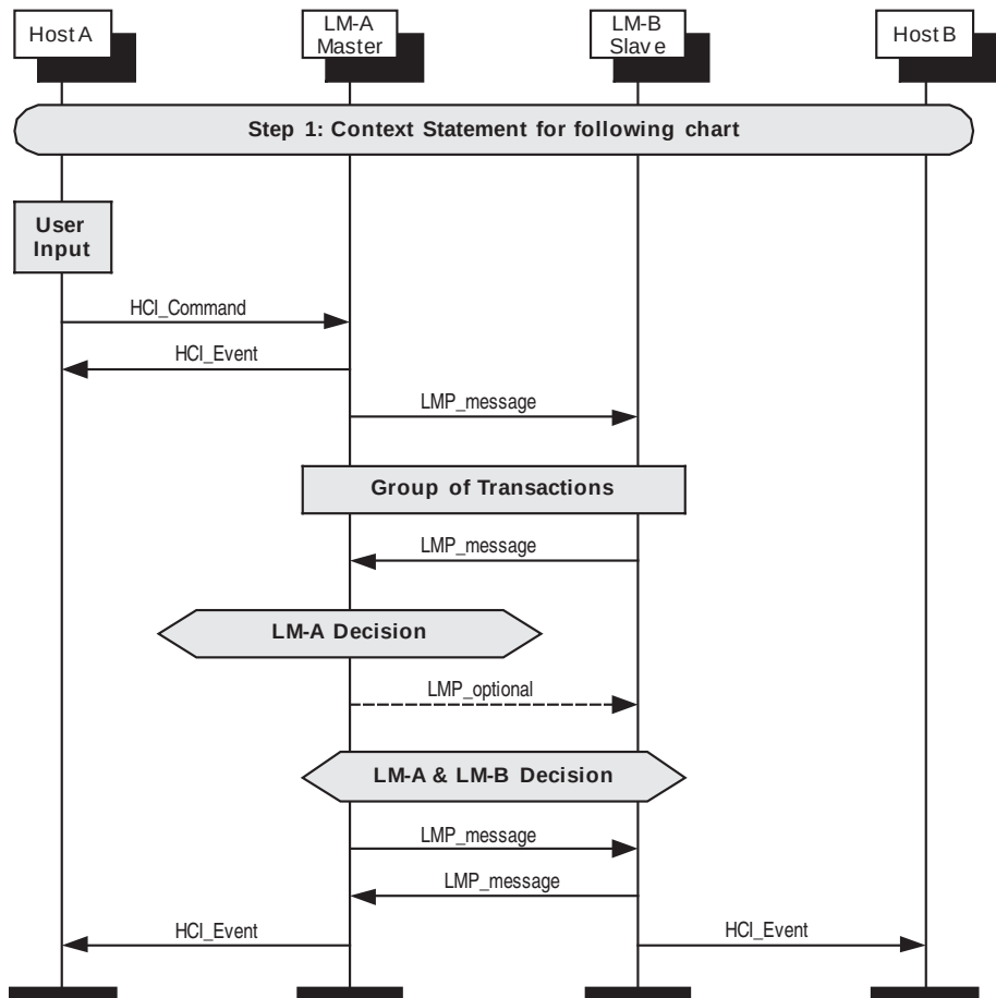
Figure 99—Sample MSC
