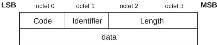
Figure 195—Command format
