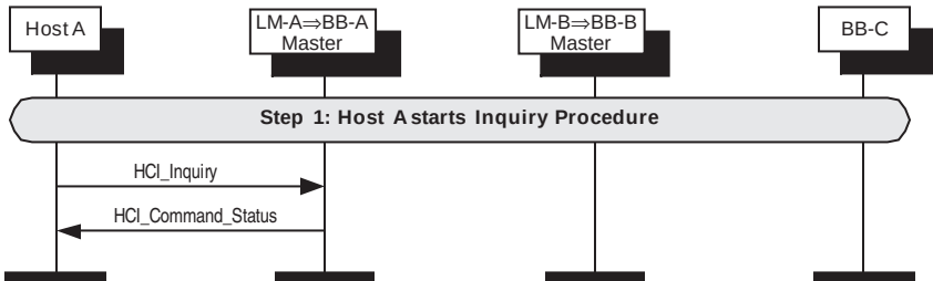
Figure 103—Host A starts inquiry procedure
