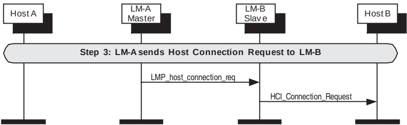
Figure 114—LM-A requests host connection
