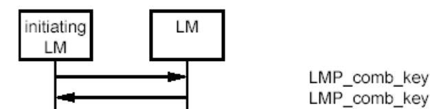
Sequence 27: Successful change of the link key.
