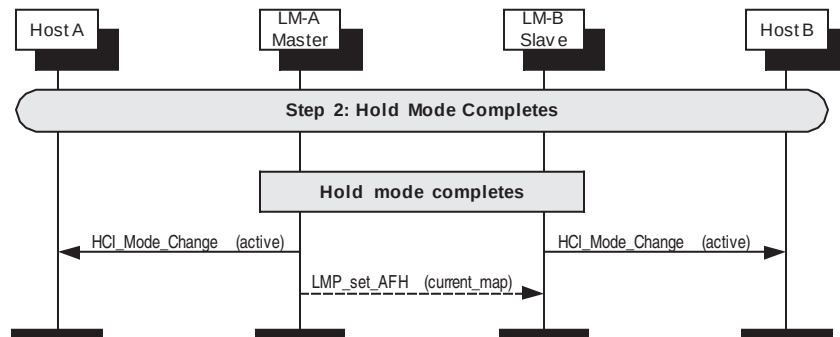
Figure 153—HOLD mode completes
