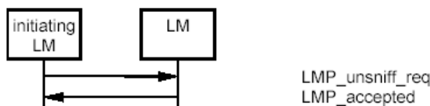
Sequence 60: Slave moved from SNIFF mode to active mode.
