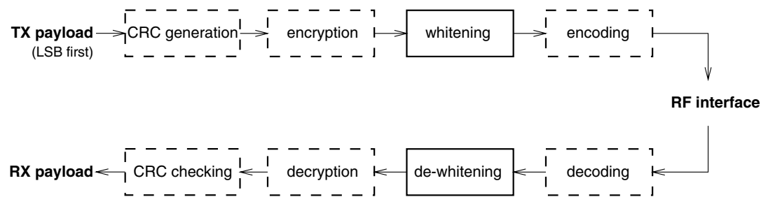
Figure 44—Payload bit processes
