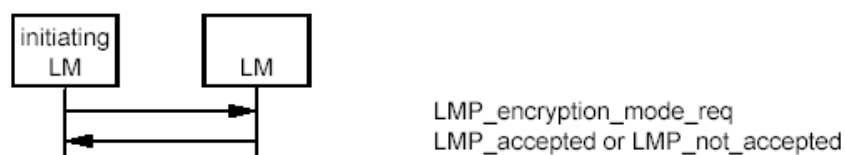
Sequence 31: Negotiation for encryption mode.
