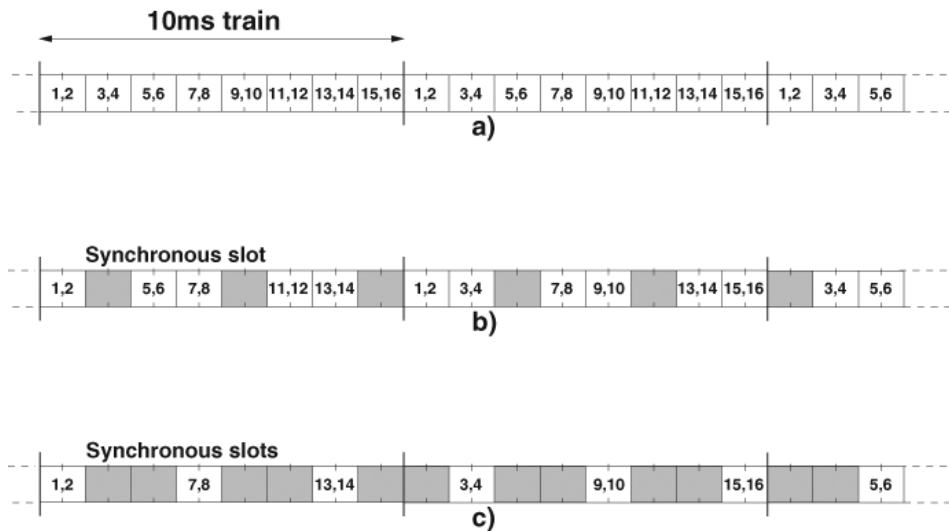
Figure 61—Conventional page (a), page while one synchronous link present (b), page while two synchronous links present (c)
