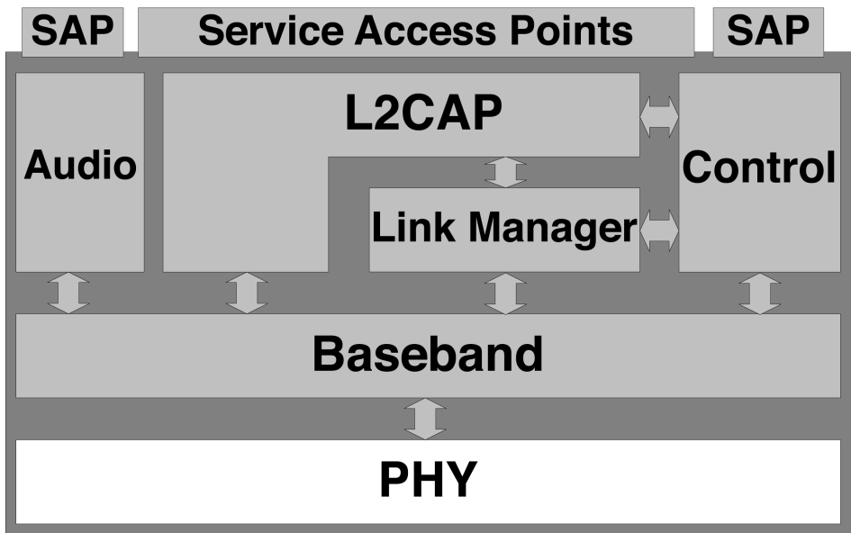
Figure 226—SAP relationships
