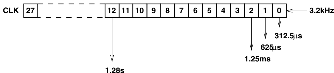
Figure 10—IEEE 802.15.1-2005 clock
