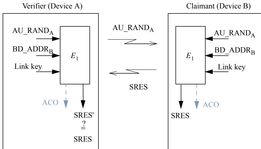
Figure 177—Challenge-response
