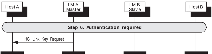
Figure 119—Authentication initiated
