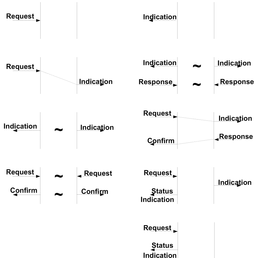
Figure 229—Sequence diagrams
