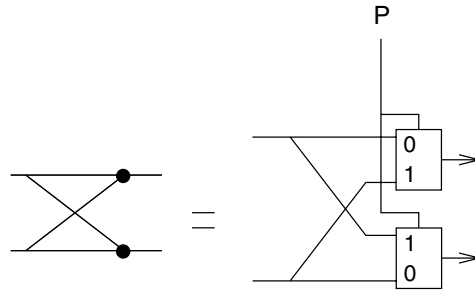
Figure 30—Butterfly implementation
