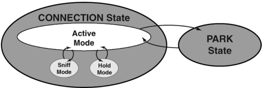
Figure 64—Connection state
