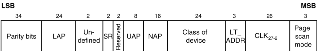
Figure 39—Format of the FHS payload
