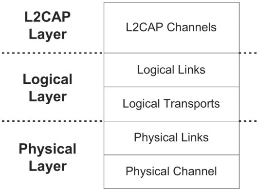
Figure 2—Generic data transport architecture
