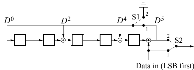
Figure 53—LFSR generating the (15,10) shortened Hamming code
