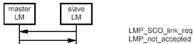
Sequence 62: Master rejects slave's request for an SCO link.
