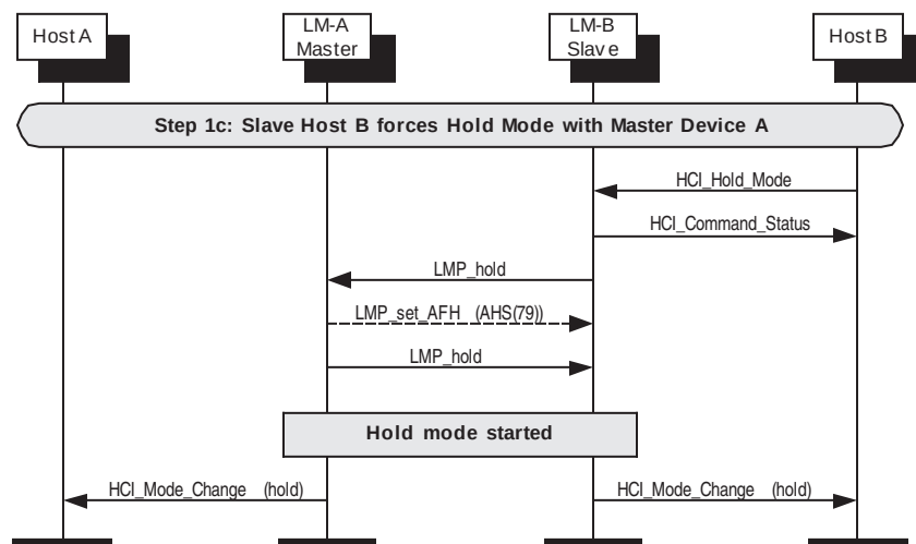
Figure 152—Slave forces HOLD mode
