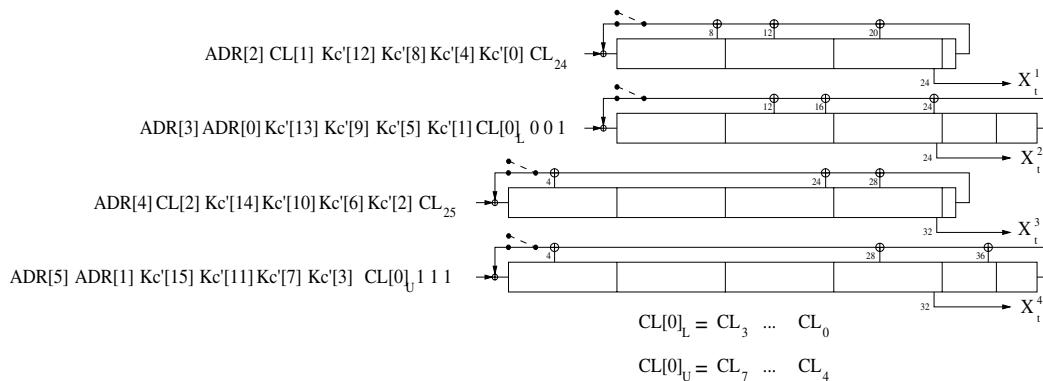
Figure 175—Arranging the input to the LFSRs
