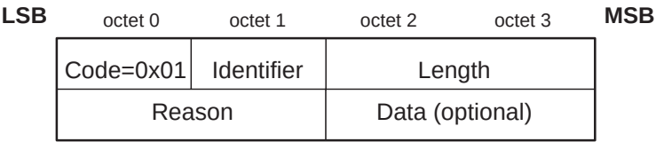
Figure 196—Command Reject packet
