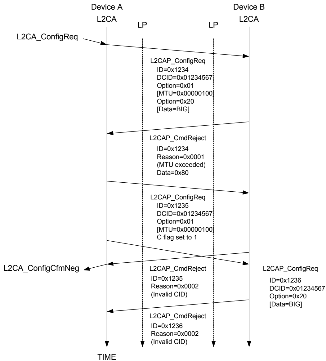
Figure 225—Unsuccessful configuration request
