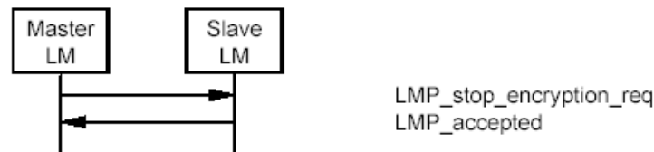
Sequence 35: Stop of encryption.
