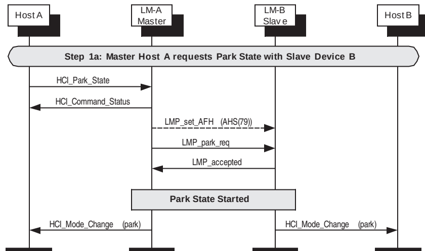
Figure 154—PARK state request from master
