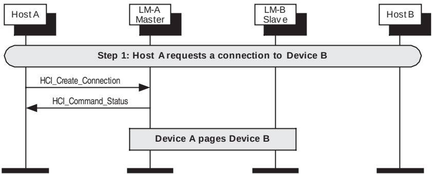
Figure 112—Host A requests connection with device B
