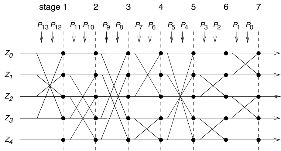
Figure 29—Permutation operation for hop system
