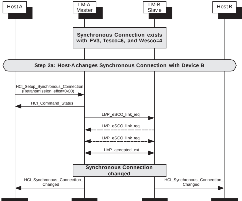
Figure 144—Master renegotiates eSCO connection
