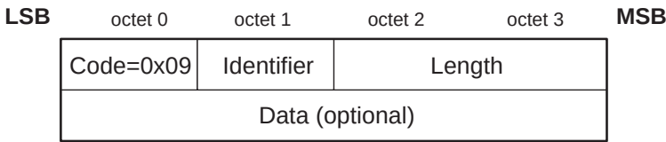
Figure 206—Echo Response packet
