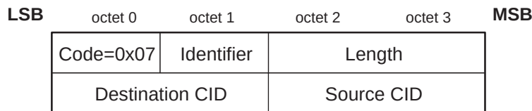
Figure 204—Disconnection Response packet
