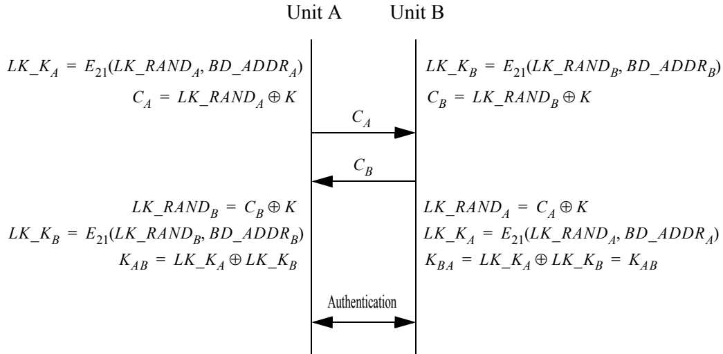
Figure 169—Generating a combination key
