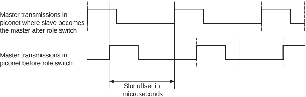
Figure 90—Slot offset for role switch
