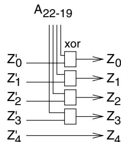
Figure 28—XOR operation for hop system
