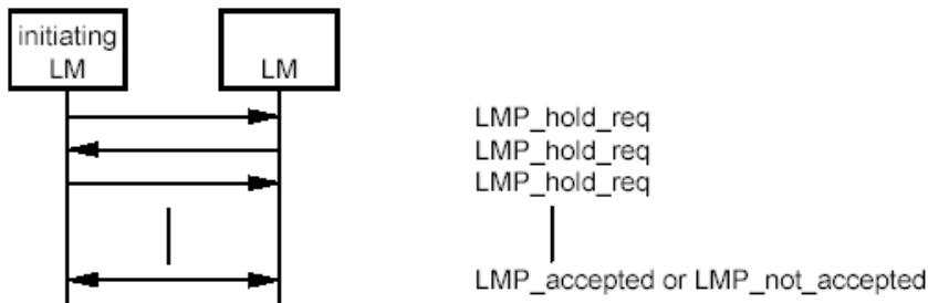
Sequence 49: Negotiation for HOLD mode.
