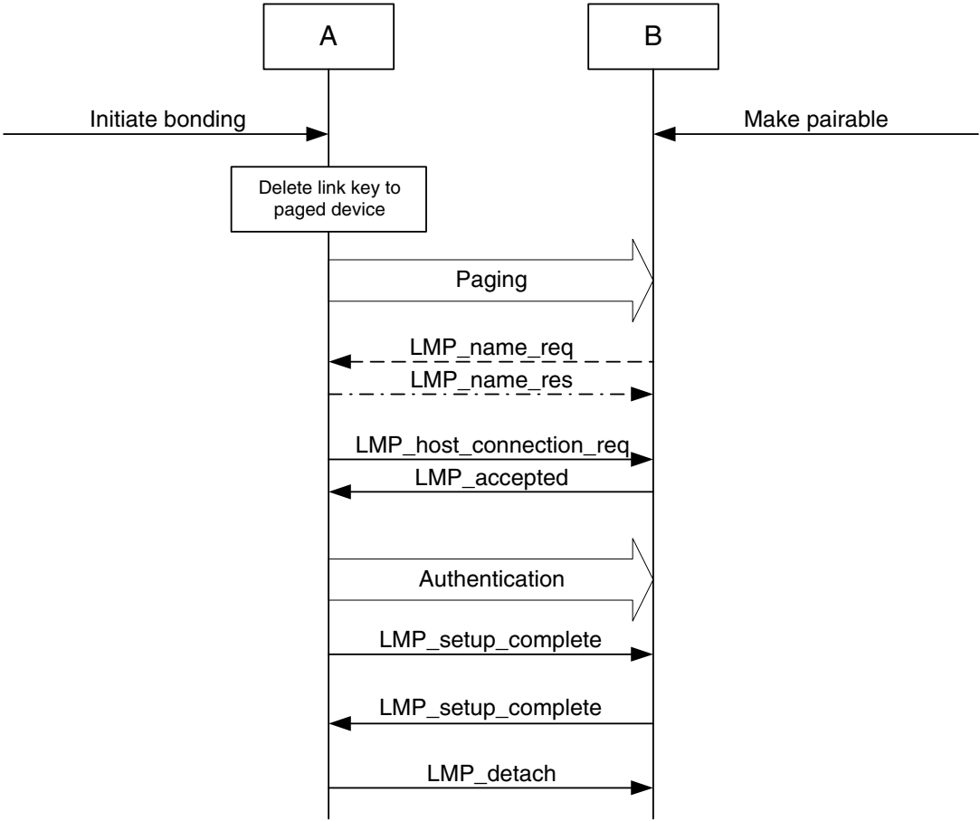
Figure B.12—Dedicated bonding, when the purpose of the procedure is only to create and exchange a link key between two devices
