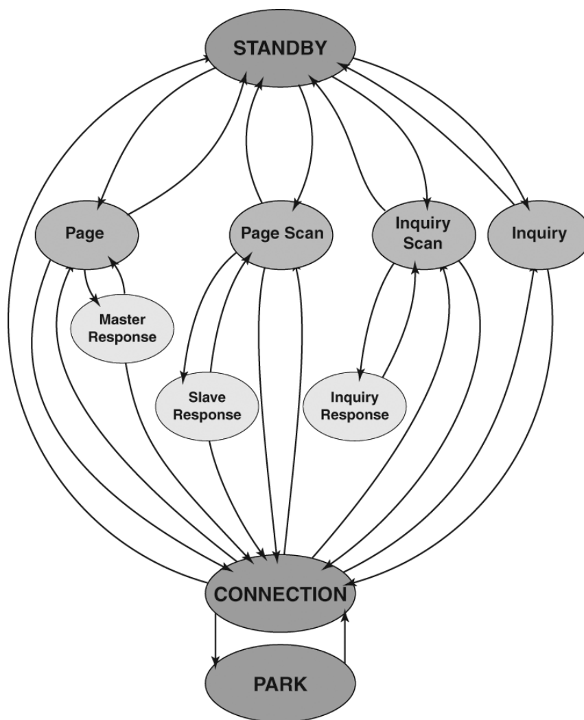
Figure 59—State diagram of link controller
