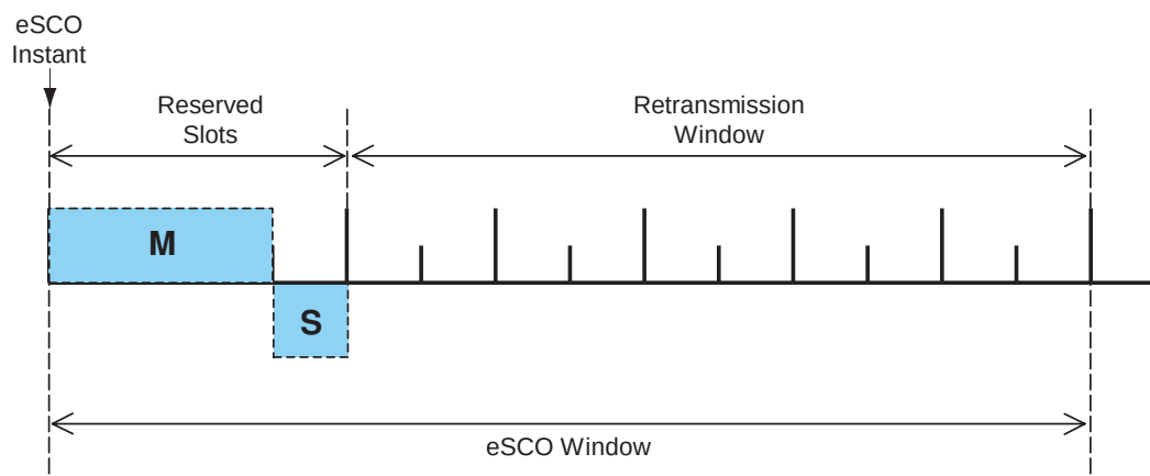
Figure 67—eSCO window details for asymmetric traffic
