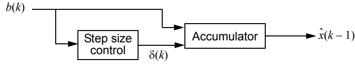
Figure 78—Block diagram of CVSD decoder with syllabic companding
