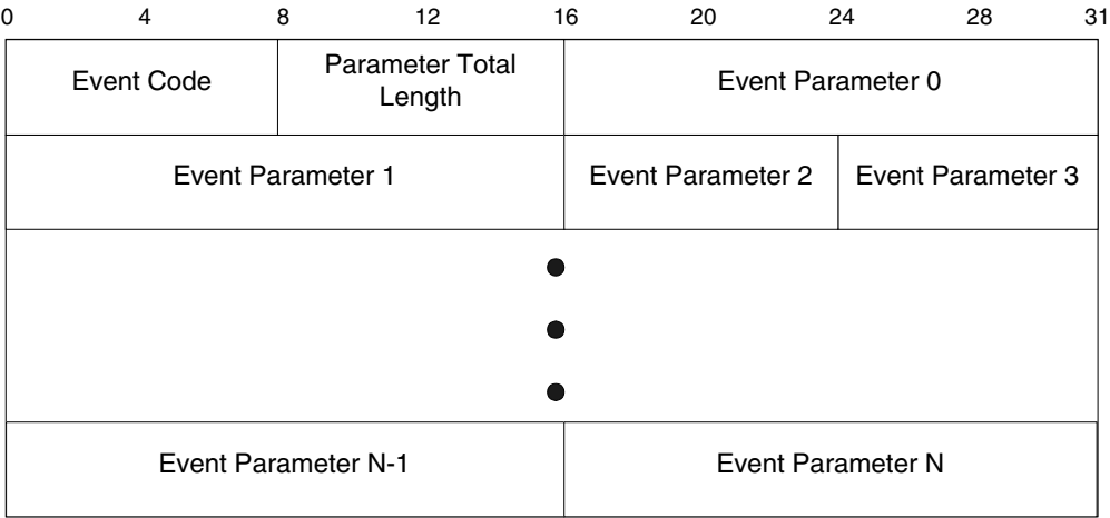
Figure 96—HCI event packet
