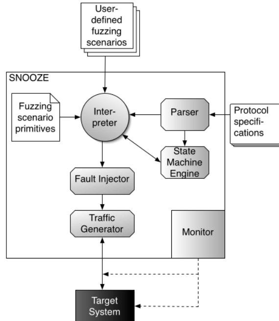
Fig. 1. Main components of SNOOZE
