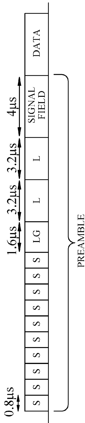
FIG. 1 (PRIOR ART)
