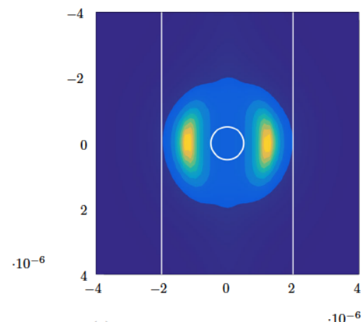
(a) linear plot of energy density
