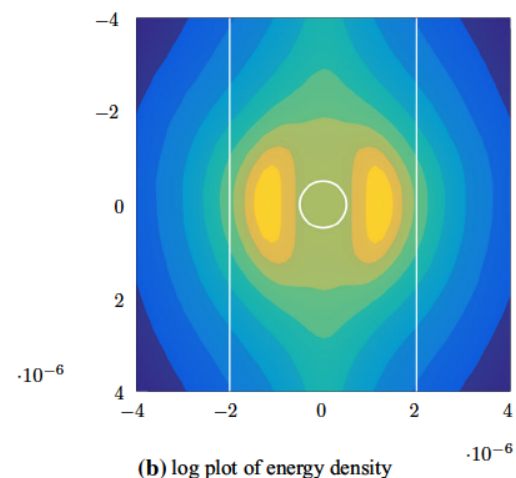
Fig. 7 The white lines represent a 4 \mu\text{m} Casimir cavity, and the circle represents the 1 \mu\text{m} pillar located at the midplane of the cavity. Panel (a) shows the linear 2D plot of the energy density and panel (b) shows the log 2D plot. The bright yellow regions show the impact of the presence of the pillar on the energy density, and the log plot shows that the pillars do not self-screen themselves from the background field gradient resulting from the presence of just the plates (lime-green color)
