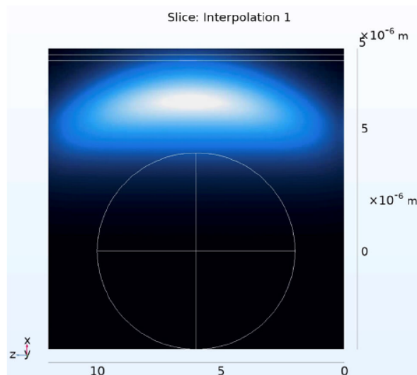
(a) 2 dimensional cut of a sphere-plate case
