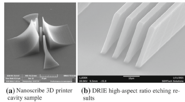
Fig. 2 Initial results from current nanofabrication trial runs: the left panel in the figure depicts a recent result obtained utilizing a Nanoscribe 3D printer to evaluate a range of cavity gaps and pillar sizes; the right panel shows recent etching results using Deep Reactive Ion Etching (DRIE) equipment to etch the high-aspect ratio cavity planes into a silicon wafer substrate
