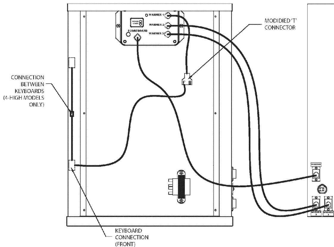
FWM3 - 2 High/4 High SB1 Interface Cable Schematic
