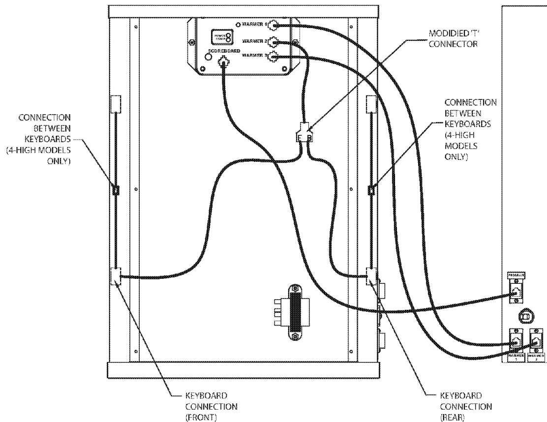
FWM3 - 2 High/4 High MB1 Interface Cable Schematic
