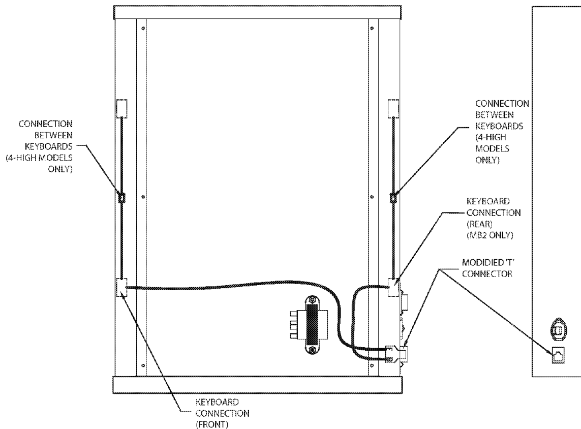
FWM3 - 2 High/3 High/4 High MB2 & SB2 Interface Cable Schematic
