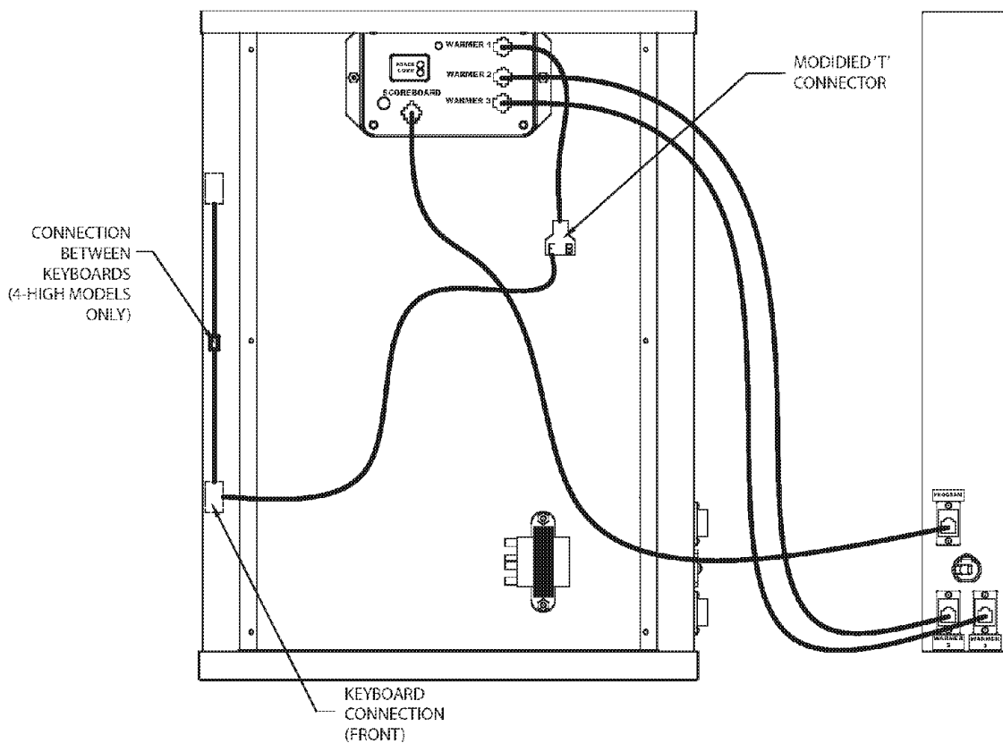
FWM3 - 2 High/4 High SB1 Interface Cable Schematic
