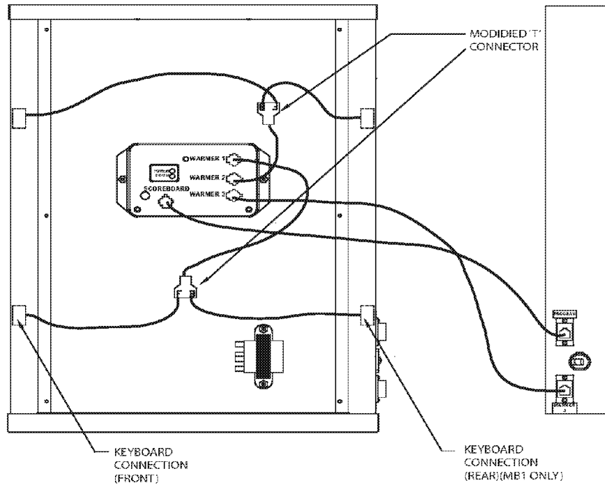
FWM3-34 MB1 & SB1 Interface Cable Schematic
