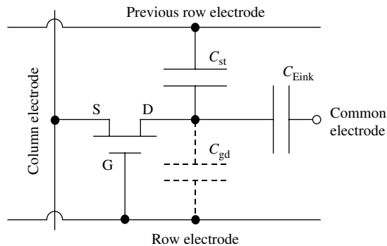
Figure 13.4 Equivalent circuit of one pixel. The source, drain, and gate of the TFT are indicated by S, D, G, respectively. The storage capacitor is C_{\text{st}} , the pixel capacitor is C_{\text{Eink}} and the parasitic gate–drain capacitance is C_{\text{gd}}
