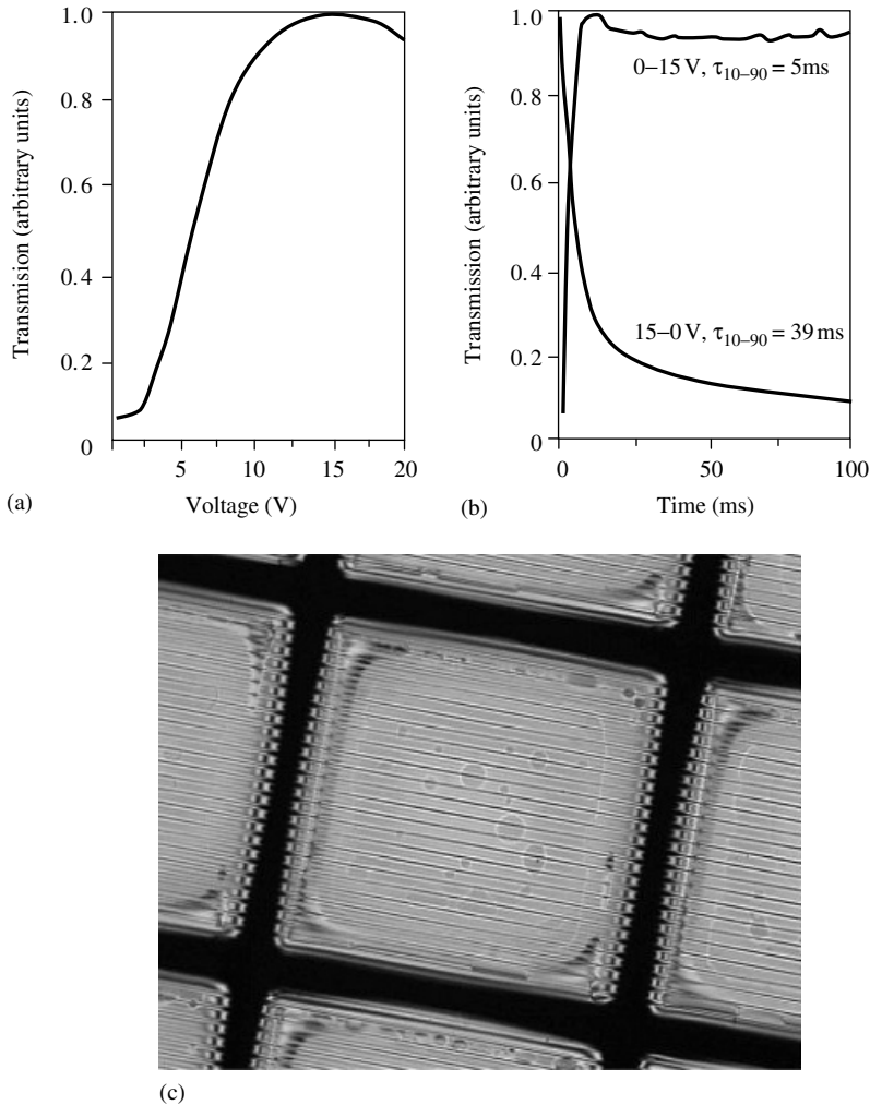
Figure 18.7 The electro-optical characteristics of the paintable LCD between crossed polars (normally black mode). (a) The transmission voltage curve and (b) the switching curves. The LC (E7) is driven by in-plane switching. The interdigitated electrode structure has a pitch of 18\text{ }\mu\text{m} and a spacing of 9\text{ }\mu\text{m} . (c) The microscope picture of a pixel driven in the on-state clearly shows that the LC is partially switched. Above the electrodes, the pixel stays dark. Obviously the isotropic walls stay dark as well
