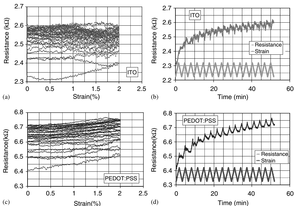
Figure 9.5 Fatigue test data for the cyclic loading of (a, b) ITO-coated PET and (c, d) PEDOT:PSS coated PET loaded in tension
