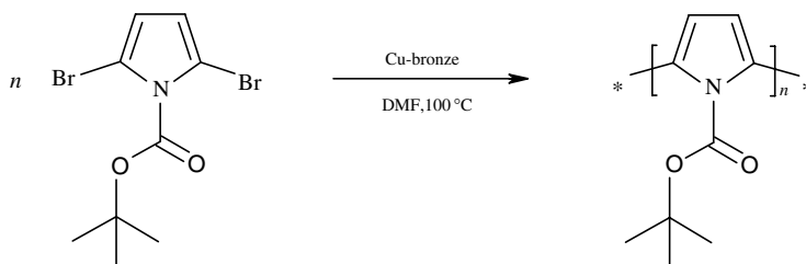
Scheme 8.3 Reductive polymerization of a pyrrole derivative via the Ullmann reaction (Groenendaal et al. 1995)
