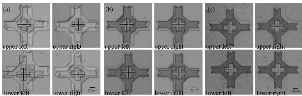
Figure 14.18 Overlay misalignment between the first, bottom gate, and second, source/drain, photolithography levels in back channel etched a-Si TFT process with (a) 5 W gate \text{SiN}_x , (b) 12 W gate \text{SiN}_x and (c) 25 W gate \text{SiN}_x . The frames lie 52 mm apart near the corners of the 70 mm square substrate. The dashed crosses mark the center at the gate mask level and the solid crosses the center at the source/drain mask levels. The sample is seen to shrink substantially with 5 W \text{SiN}_x , to shrink slightly with 12 W \text{SiN}_x , and to expand substantially with 25 W \text{SiN}_x (Cheng 2004)
