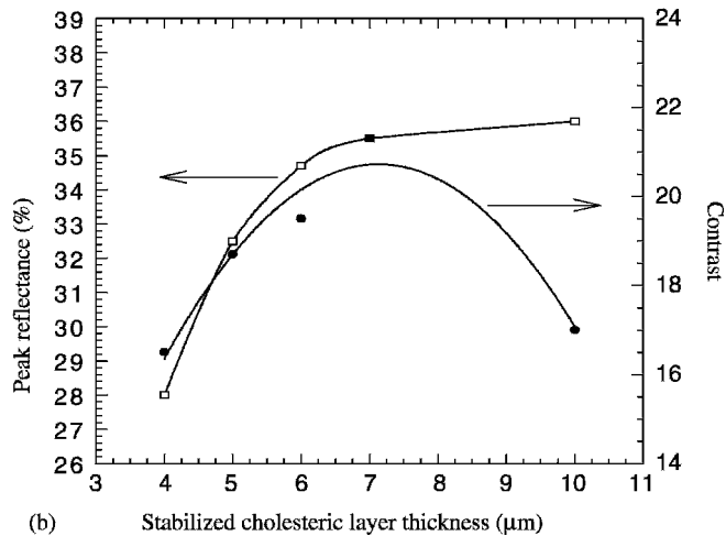
Figure 17.8 (a) Calculated reflection spectra versus cell thickness, d , in units of pitch length, p_0 , where np_0 = 0.54 , \Delta n = 0.23 , and n = 1.63 . (b) Experimental plot of reflectance and the contrast versus cell gap thickness for a cholesteric material of \Delta n = 0.26 , \Delta \epsilon = +16.8 and for substrates that have been treated for small micrometer-sized domains. The measurements were made at room temperature with a 250 Hz pulse of width 100 ms. Part (a) reproduced by the permission of the Society for Information Display
