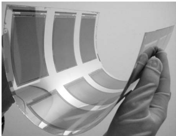
Figure 23.4 A flexible LTPS TFT on a 300 mm × 350 mm and 0.2 mm thick plastic substrate with nine dies for 3.8 inch diagonal LCDs. Color filters and post spacers have been formed on the TFT substrate. The radius of curvature is about 75 mm. Reproduced by permission of SID
