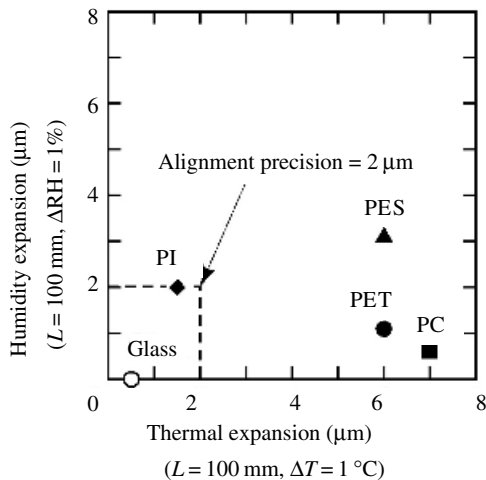
Figure 24.1 Dimensional instability of typical plastic materials
