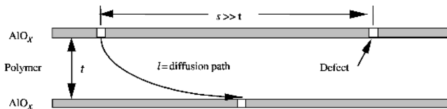
Figure 4.8 The multilayer geometry provides a long effective diffusion path when the defects in adjacent \text{AlO}_x layers are widely spaced. For large defect spacings and thin polymer layers the diffusion path ( l_{\text{eff}} ) is approximately one-half the defect spacing
