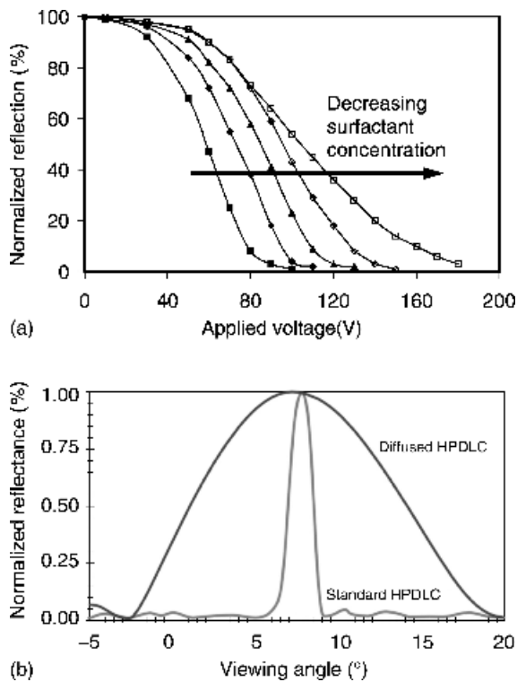
Figure 16.9 (a) Reflectance versus voltage of an H-PDLC that has been doped with a surfactant to lower its drive voltage and (b) a comparison of the viewing angle for a standard H-PDLC and one that has been fabricated using a diffusion plate during exposure. Reproduced by the permission of the Society for Information Display
