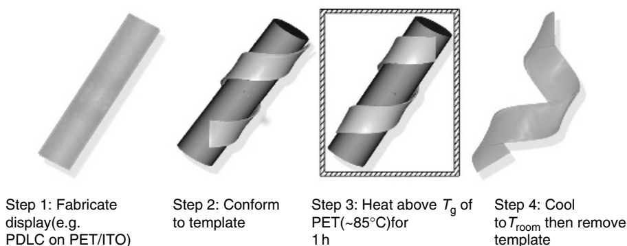
Figure 16.4 The four steps used to create a conformal PDLC. The box in step 3 represents the oven. Reproduced by the permission of the Society for Information Display
