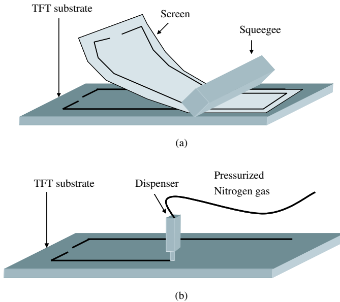
Figure 22.15 Seal formation by (a) screen printing and (b) dispensing
