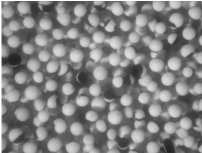
Figure 20.8 A photomicrograph of an obliquely illuminated Gyricon sheet. The dark spaces between beads are seen to be lower-level beads that receive less illumination
