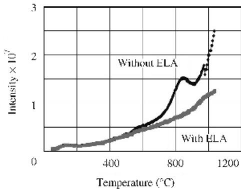
Figure 24.5 TDS analysis for hydrogen contained in the sacrificial silicon layer
