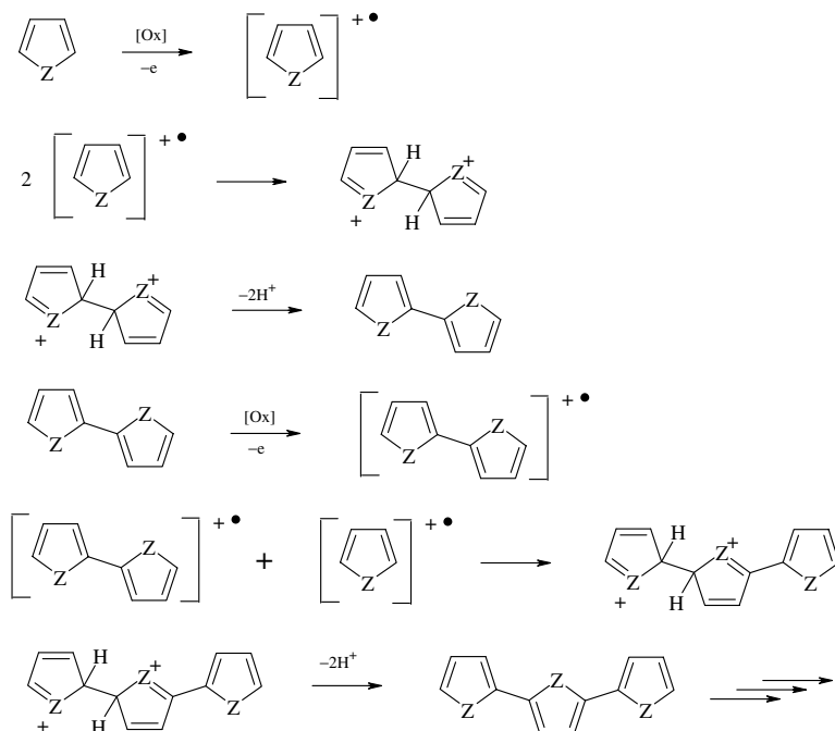
Scheme 8.9 Mechanism for the electrochemical polymerization of a five-membered heteroaromatic monomer
