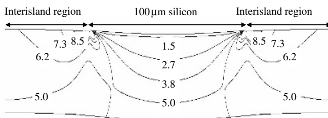
Figure 14.10 Contour plot of the radial strain (%) in a polyimide substrate with a round silicon island, after stretching. See text for details (Hsu 2003)
