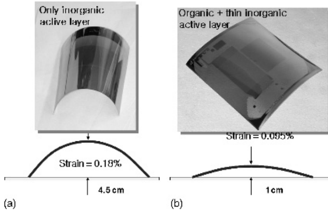
Figure 22.7 The shape of PES after deposition of TFT layers
