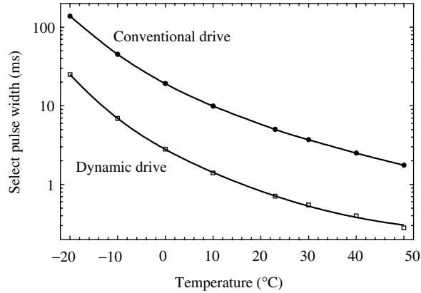
Figure 17.10 Update rates as indicated by the select pulse width for the conventional drive scheme versus the dynamic drive scheme. The difference is quite dramatic at low temperature. Reproduced by the permission of the Society for Information Display
