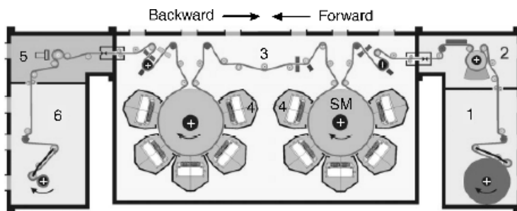
Figure 21.3 Web-based coater: (1) unwinder chamber, (2) pretreatment chamber, (3) intermediate chamber, (4) sputter compartment, (5) marking chamber, (6) rewinder chamber, (●) seven driven rollers including winders, (●) six tension measurement rollers, (●) nine spreader rollers, (SM) speed master. Courtesy of Von Ardenne Anlagentechnik GmbH
