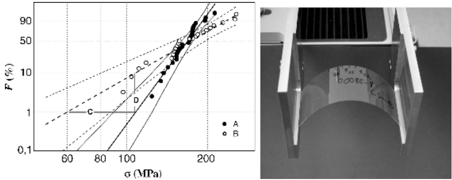
Figure 3.11 Setup for the two-point bending procedure and the influence of edge positioning
