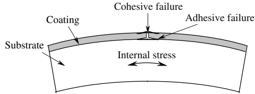
Figure 6.3 The durability of thin film/polymer layered composites is determined by the internal stress (coating and interfacial region), the coating cohesive strength and related crack onset strain, and the coating/substrate adhesion.
