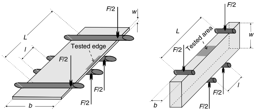
Figure 3.9 Four-point bending test
