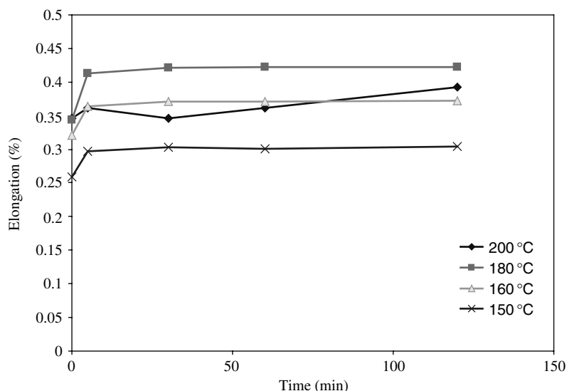
Figure 2.5 Thermomechanical analysis of polyethylene naphthalate film
