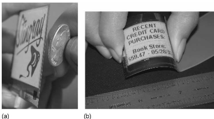
Figure 19.17 Thin, conformable, active matrix displays made using E Ink's electrophoretic film on an a-Si active matrix backplane fabricated on passivated steel foil. (a) The 300 \mu\text{m} thickness is shown and (b) a curved display. Reproduced by the permission of the Society for Information Display
