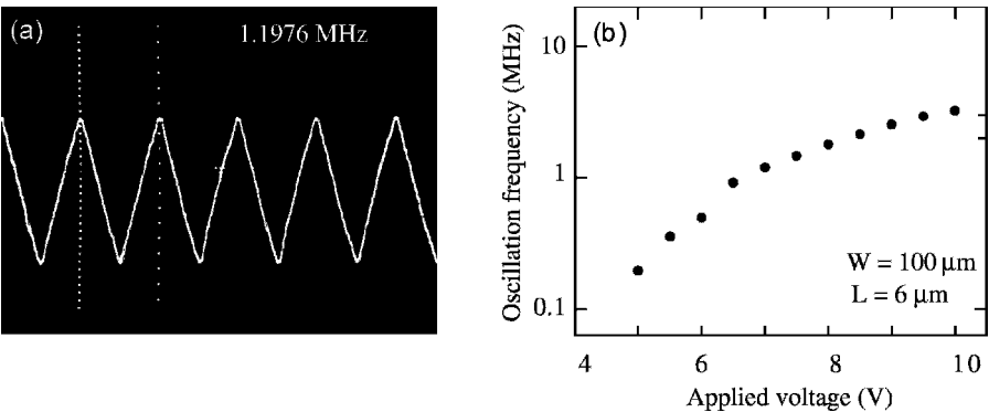
Figure 24.10 Operation of the 15-stage ring oscillator measured after transfer to the PES film: (a) output waveform and (b) the maximum operative frequency as a function of the applied voltage
