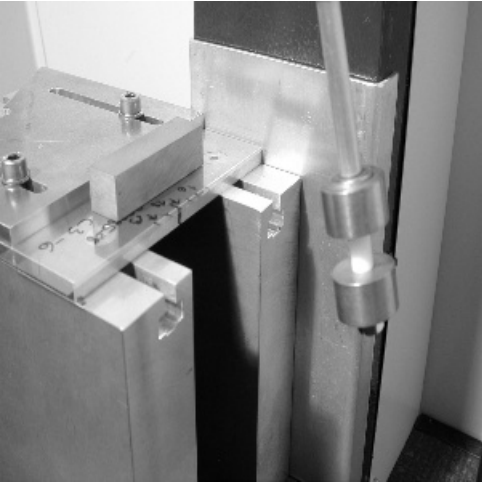
Figure 3.10 Edge impact test
