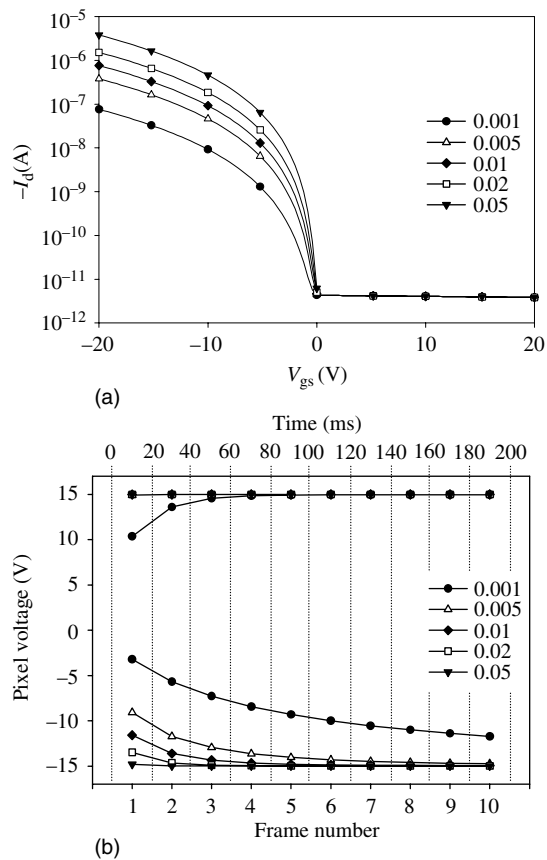
Figure 13.5 (a) Simulated transfer characteristics at five different values of parameter \mu_0 in (13.1) for V_{sd} = 20 V. The key shows the resulting field-effect mobility (cm 2 /V s) at V_{sg} - V_T = 25 V and parameter \gamma = 1.1 . The leakage current was set to 3 pA. (b) Simulated charging behavior of a pixel with the same five values for the mobility. The vertical axis shows the pixel voltage, the horizontal axis shows the frame number. The simulated frame rate was 50 Hz
