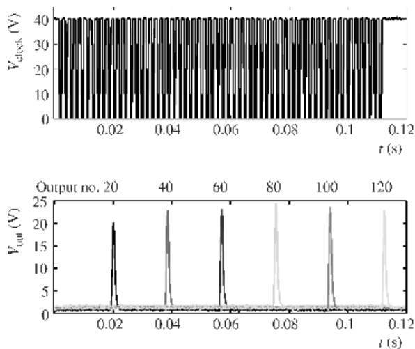
Figure 13.13 Measurement results of the 120-stage shift register, showing the clock pulses and the output pulses for every 20th stage
