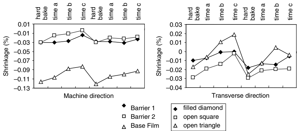
Figure 15.7 Substrate dimensional changes during process simulation
