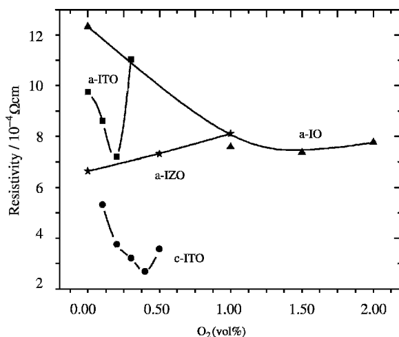
Figure 5.2 DC magnetron sputter deposition oxygen optimization curves for pure amorphous indium oxide (a-IO), a-ITO, c-ITO, and a-IZO. These curves are for films of roughly equivalent thickness (100 nm) and were sputtered at similar total pressure (mtorr) and power (0.25 W/cm 2 )
