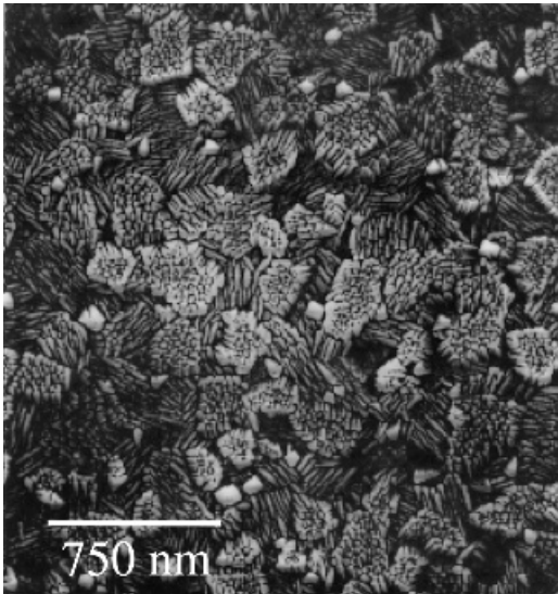
Figure 5.4 High-quality crystalline ITO deposited by DC magnetron sputtering at 350 °C with a resistivity of 1.1 \times 10^{-4} \Omega \text{ cm} and transmissivity of better than 90%. Note the presence of subgrain regions known colloquially as the rice field structure
