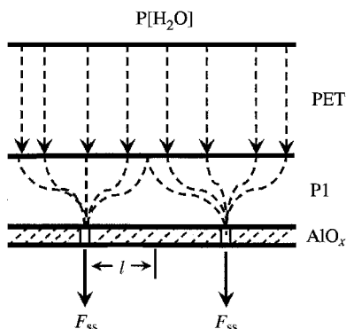
Figure 4.7 Flow paths for water vapor through defects in AlO x coating when the defects are small and spaced far apart
