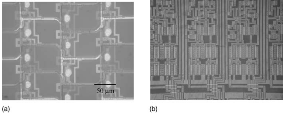
Figure 23.3 Optical microscope images of the transferred device layer patterns on a plastic substrate: (a) a pixel area and (b) a driver area
