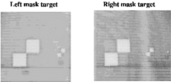
Figure 15.4 Metal layer photomask (bright squares) misaligned from the left-hand side of the device to the right-hand side by \sim 5\text{ }\mu\text{m} after ITO patterning (dark squares) on PET substrate without heat stabilization and dimensional controls; the substrate has shrunk during ITO patterning
