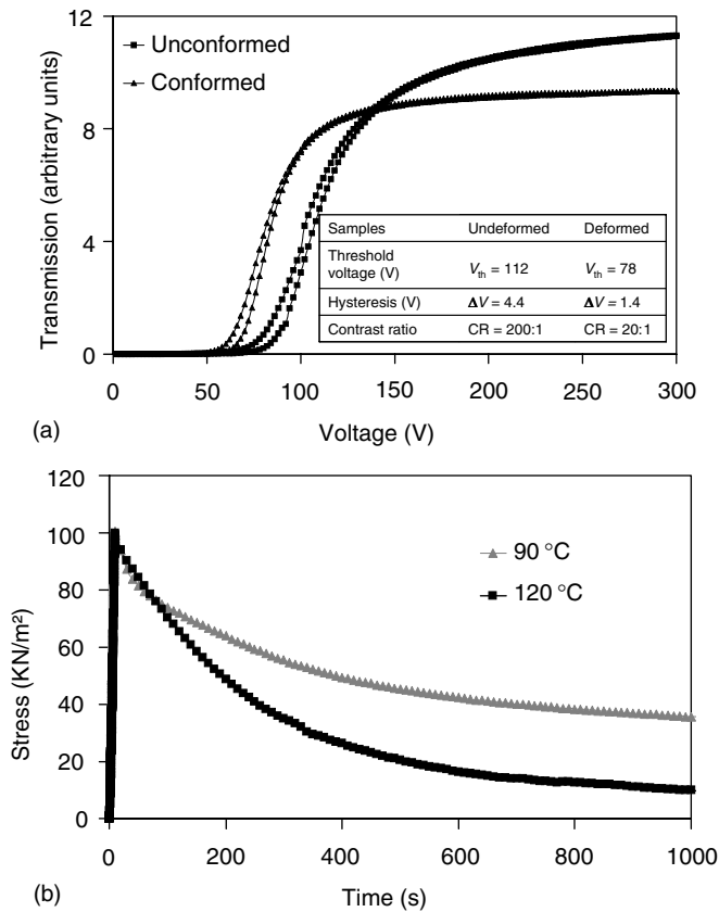
Figure 16.6 (a) Transmission–voltage curve for the conformed PDLC and (b) stress relaxation curve for PET/ITO. Reproduced by the permission of the Society for Information Display
