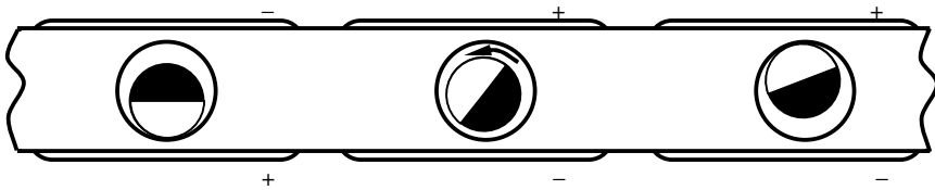
Figure 20.3 Dipole and monopole charges are associated with the Gyricon bead. On application of a field, the bead traverses the cavity and rotates. On reaching the wall it adheres
