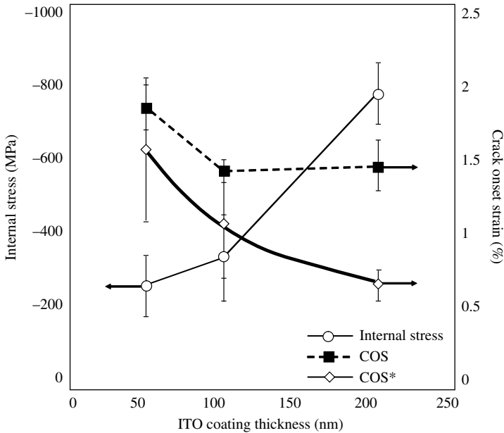
Figure 6.11 Coating thickness dependence of internal stress, measured crack onset strain (COS) and intrinsic crack onset strain (COS*). The thick continuous line is a power-law fit to the intrinsic crack onset strain data. Reproduced by the permission of Elsevier and SVC
