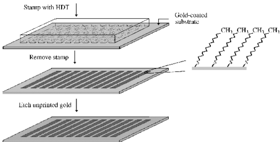
Figure 11.3 Steps for microcontact printing. The stamp is first inked with a solution of a material that is capable of forming a self-assembled monolayer (SAM) on the substrate that will be printed. In the case illustrated here, the ink is a millimolar concentration of hexadecanethiol (HDT) in ethanol. The substrate consists of a thin layer of Au on a flat support. Removing the stamp after a few seconds of contact leaves a patterned SAM of HDT on the surface of the Au film. The printed SAM can act as a resist for the aqueous wet etching of the exposed regions of the Au. The pattern of Au that results after etching and removal of the ink can be used to build devices of various types, including thin film transistors for flexible electronic systems. Reproduced by permission of the American Institute of Physics
