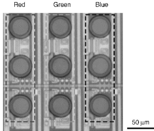
Figure 24.16 Pixel circuit layout of the TFT OLED display circuit
