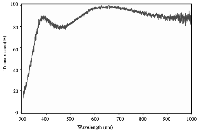
Figure 5.5 Transmission spectrum for crystalline ITO deposited at 250–350 °C to a thickness of 110 nm
