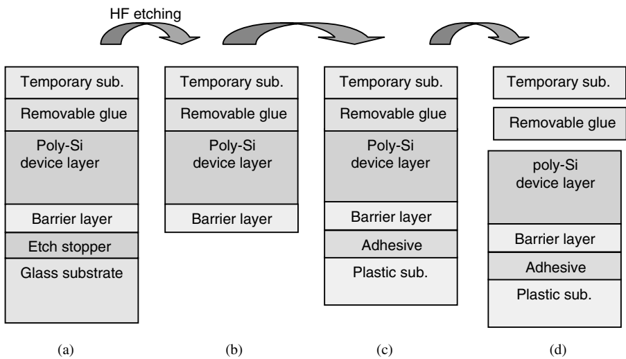
Figure 23.2 Flow diagram of the transfer process to transfer a thin film device layer from a glass substrate onto a plastic substrate
