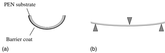
Figure 2.13 Bending geometries
