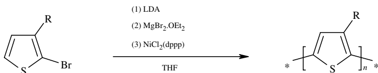
Scheme 8.4 Synthesis of regioregular polythiophenes applying the Kumada methodology (McCullough et al. 1993)
