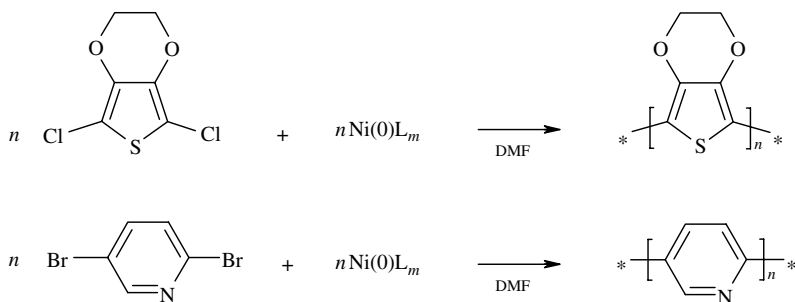
Scheme 8.2 Examples of Yamamoto-type reductive polymerization reactions (Yamamoto et al. 2000)
