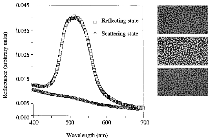
Figure 17.13 Microscope photographs of cholesteric droplet dispersions with three different Bragg-reflective colors and the reflection spectra of the yellow droplet in the planar reflective texture and nonreflective focal conic texture
