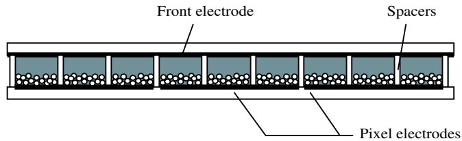
Figure 19.6 A series of ribs extending across the display limit lateral migration of pigment
