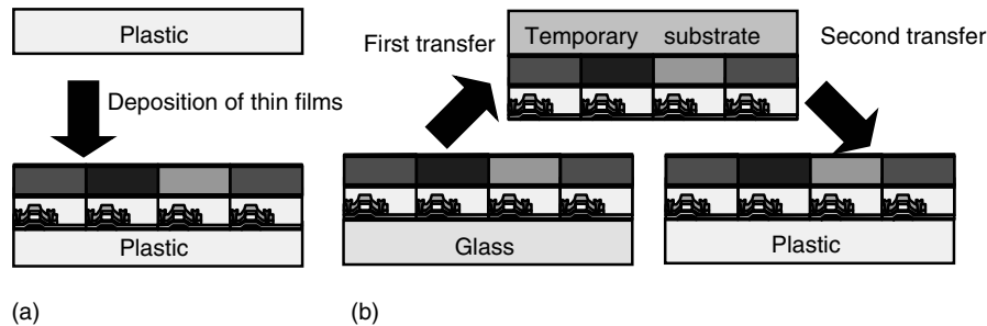
Figure 23.1 Preparing LTPS TFTs on a plastic substrate: (a) a direct process and (b) a transfer process
