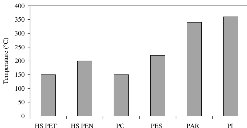
Figure 2.6 Upper operating temperature of base substrates
