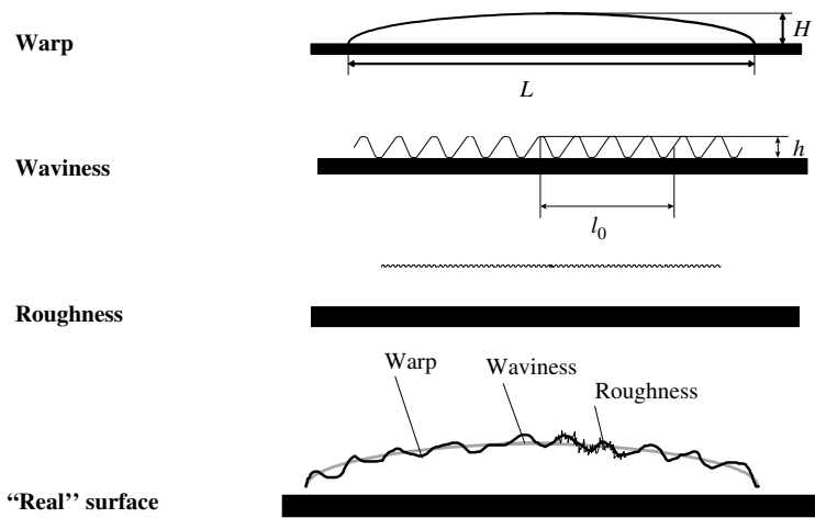
Figure 3.4 Contribution of single quality features to the real glass substrate
