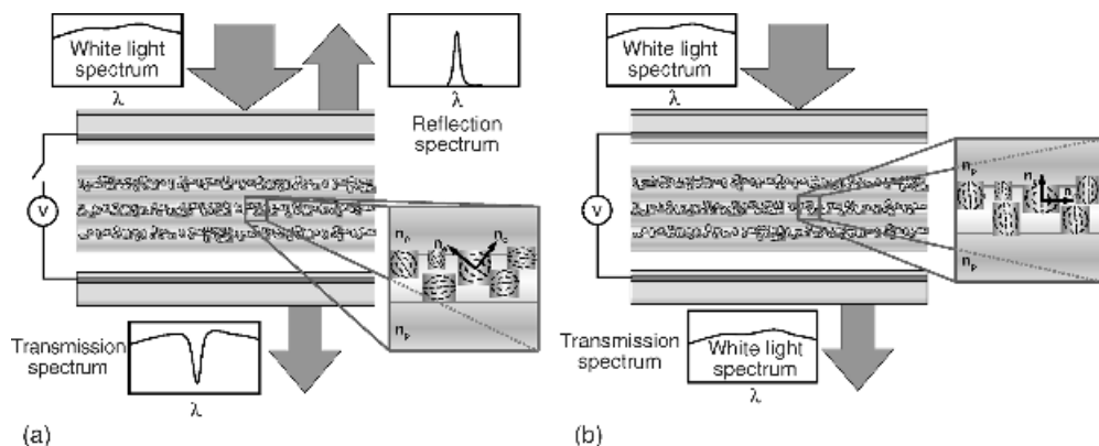
Figure 16.7 Schematic diagram of the H-PDLC display in (a) reflecting and (b) transmissive states
