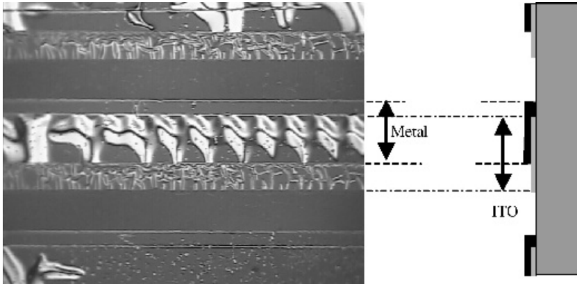
Figure 6.14 Different buckling sizes below 100 nm ITO and 600 nm metal on top of ITO
