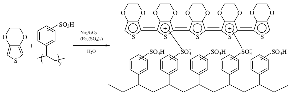
Scheme 8.14 Chemical synthesis of poly(3,4-ethylenedioxythiophene)/polystyrenesulfonic acid (PEDT/PSS) (Groenendaal et al. 2000)
