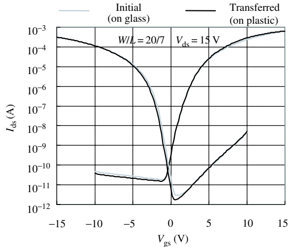
Figure 23.5 A set of typical transfer characteristics of TFTs: grey tint is before the transfer process (on glass) and solid black is after the transfer process (on plastic). Reproduced by permission of SID
