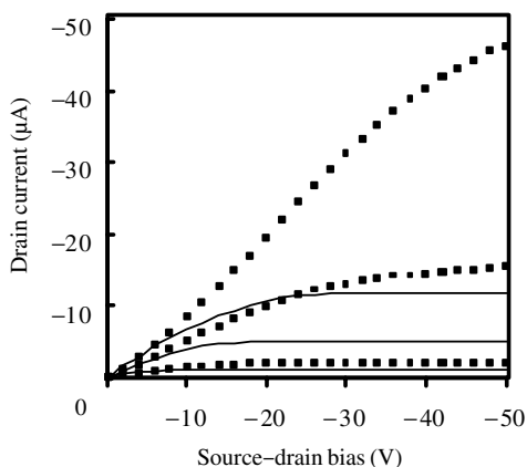
Figure 12.4 Device characteristics for a PQT-based OTFT with L = 3 \mu\text{m} . Output characteristics are shown for V_G = -10, -20 , and -30 \text{ V} according to the transistor model (solid line) and measured (squares). Reproduced by permission of the American Institute of Physics
