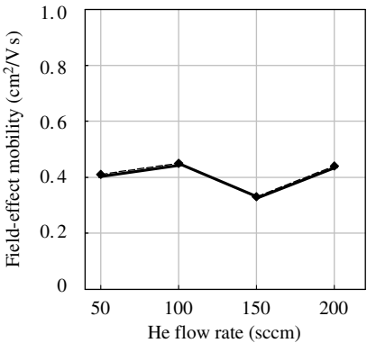
Figure 22.3 Field-effect mobility of the a-Si:H TFTs fabricated under different He flow rates for SiN x deposition
