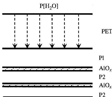
Figure 4.4 Schematic of the multilayer structure used in this study. The plastic substrate is polyester (PET), the P1/P2 layers are vacuum-deposited acrylic polymers, and the \text{AlO}_x is sputtered aluminum oxide
