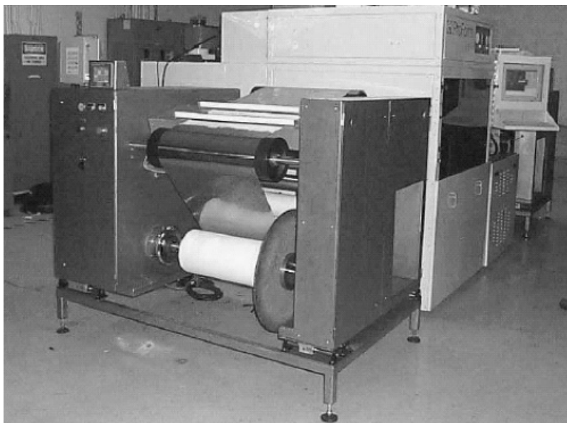
Figure 21.9 A Perkin Elmer expoler running 28 in wide 17 mil stainless steel
