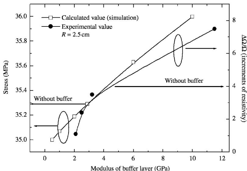
Figure 7.5 Dependence of the increment of electrical resistivity and stress distribution in ITO films on Young's modulus of buffer layers
