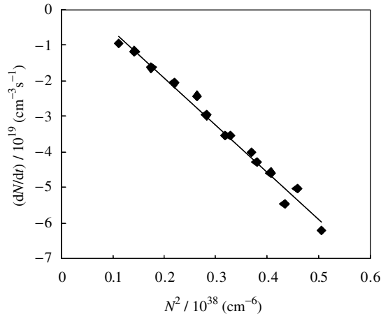
Figure 12.7 Bias stress data expressed as a function of channel carrier density for PQT. The linearity of the plot is the strongest evidence for holes forming stationary pairs and no longer participating in channel conduction. dN/dT measured at fixed time, k = 1.3 \times 10^{-18} \text{ cm}^2/\text{s} . Reproduced by permission of the American Physical Society
