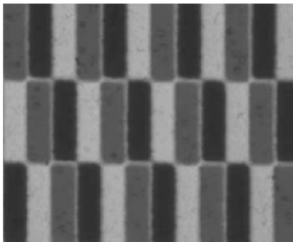
Figure 10.6 The color filters produced using the photoisomerizable cholesteric copolymer. Image courtesy of J. Lub and D. Broer, Philips
