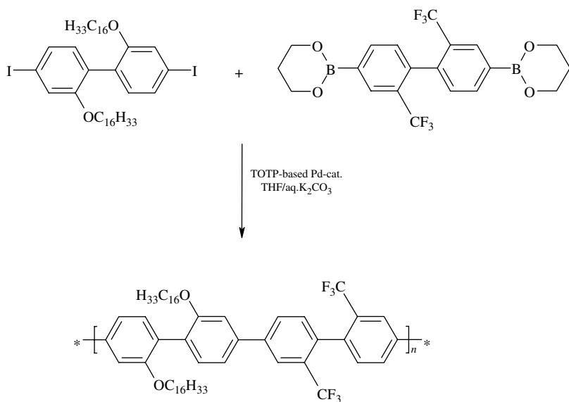
Scheme 8.5 Synthesis of polyphenylenes via a Suzuki-type polymerization (Goodson et al. 1998)
