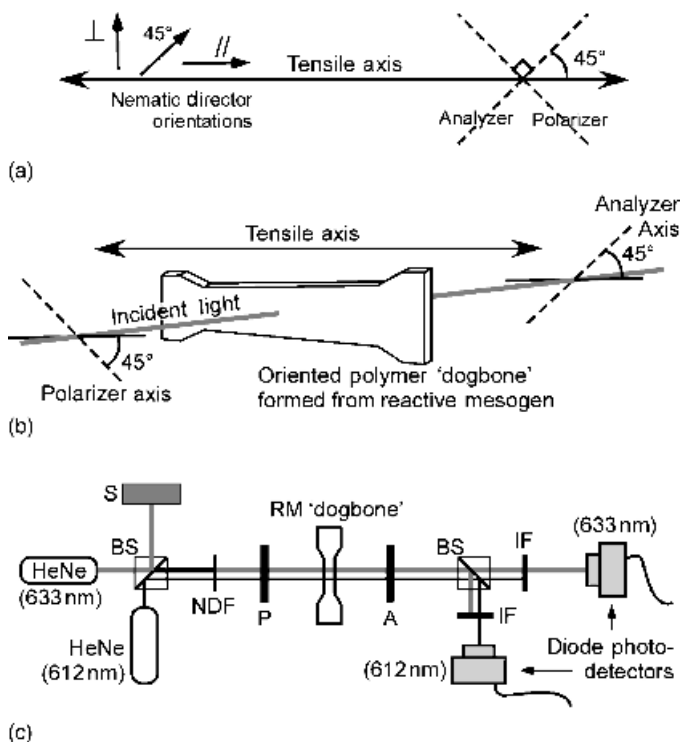
Figure 10.4 The optomechanical setup used for testing reactive mesogen retarder films. (a) The nematic director and crossed polarizer orientations. (b) The reactive mesogen orientation with respect to incident light and tensile axis. (c) The experimental setup: NDF = neutral density filter, BS = beam splitter, S = beamstop, P = polarizer, A = analyzer, IF = interference filter. Reproduced by the permission of American Institute of Physics
