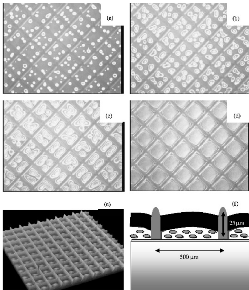
Figure 18.6 (a–d) Four stages of the polymerization-enforced stratification that has been localized in boxes due to the presence of the polymer walls: (a) nucleation at the start of the phase separation, (b, c) coalescence of LC droplets, (d) end result, within each box a (small) continuous LC layer is formed. After observation with optical microscopy (d) and interferometric microscopy (e), a schematic cross section (f) can be deduced
