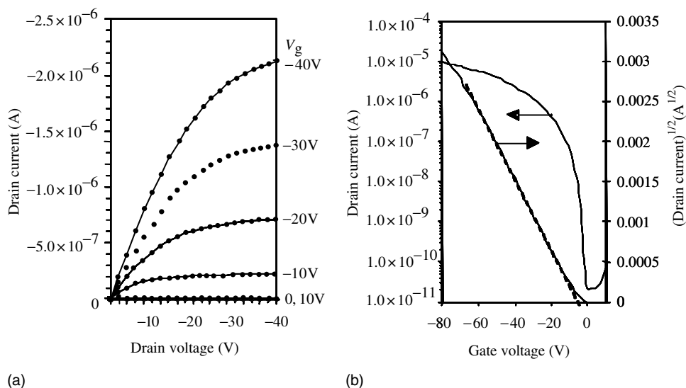
Figure 12.9 I - V characteristics of an exemplary 1a-OTFT with channel length ( L ) = 165 \mu\text{m} and channel width ( W ) = 5000 \mu\text{m} : (a) output curves at different gate voltages and (b) transfer curves at V_D = -80 V
