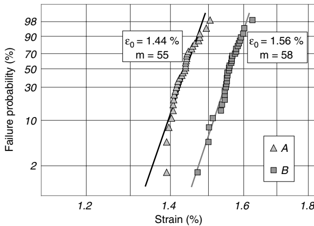
Figure 6.9 Weibull plot showing failure strain of ITO on two composite polymer substrates
