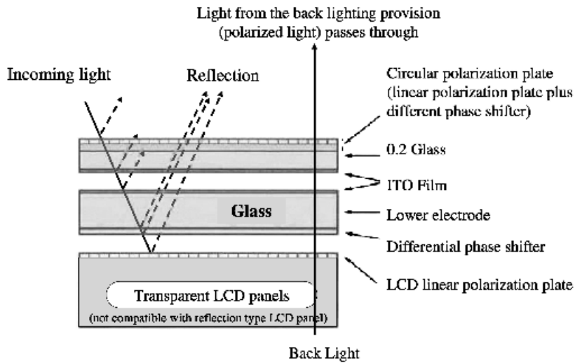
Figure 3.17 Principal structure of a touch panel
