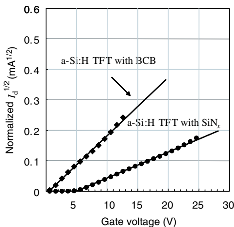
Figure 22.9 Square root of drain current plotted as a function of gate voltage to compare the field-effect mobility and threshold voltage between the a-Si:H TFTs with and without an organic gate insulator
