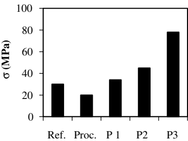
Figure 3.13 Edge strength \sigma of processed (coated) substrates at a failure probability of 1%: Ref. = reference glass (not processed); Proc. = processed glass without coating; P1, P2, P3 = processed glass with different coatings
