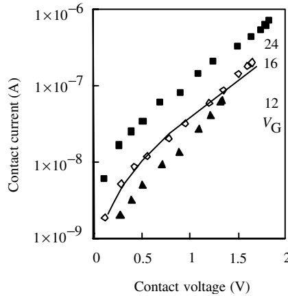
Figure 12.3 The dependence of drain current on contact voltage, I_D(V_C) , obtained from a coplanar F8T2 OTFT and deduced from a fit to the output characteristics. The solid line is a fit to (12.10)
