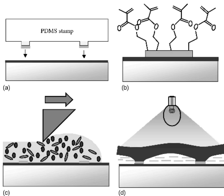
Figure 18.9 Via offset printing. (a) The alignment layer is locally modified with an adhesion promoter. (b) The adhesion promoter contains functional groups that can react with the forming polymer during polymerization. (c) After coating the modified alignment layer with the LC/prepolymer mixture, there is a single UV exposure step. (d) The UV exposure creates the LC-filled polymer boxes
