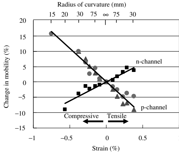
Figure 23.11 The change in electron and hole mobilities as functions of the strain in the polycrystalline silicon layer. Reproduced by permission of SID
