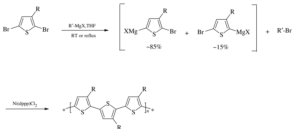
Scheme 8.13 Synthesis of regioregular poly(3-alkylthiophene)s via the GRIM method (Loewe et al. 2001)
