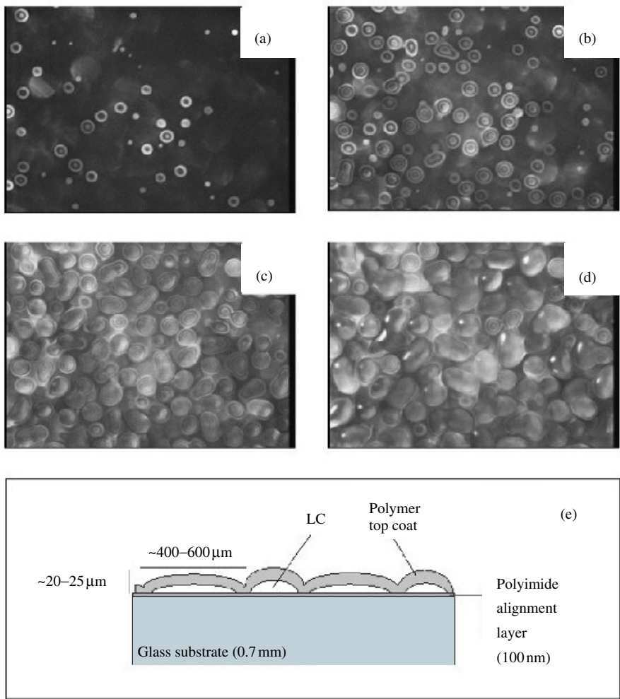
Figure 18.4 (a–d) Four stages of the polymerization-enforced stratification of the thin E7/reactive monomer film seen from the top. (e) Schematic cross section of the stratified layer; the dimensions are not to scale. The droplets do not coalesce into a continuous and flat LC layer
