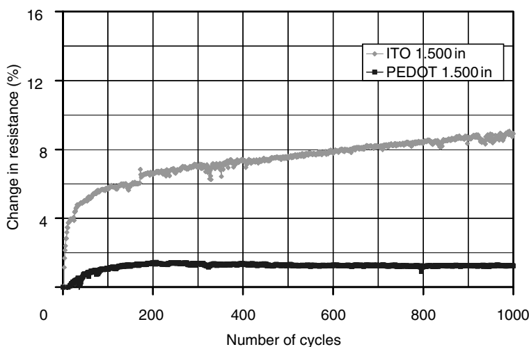
Figure 9.8 Resistance as a function of number of cycles for ITO (upper) and PEDOT:PSS (lower)
