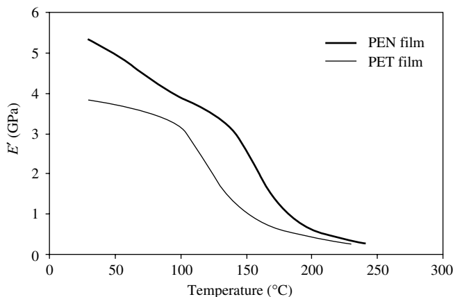
Figure 2.14 Change in stiffness with temperature for polyethylene terephthalate and polyethylene naphthalate film
