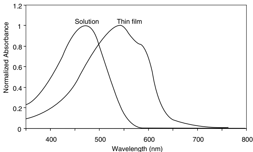
Figure 12.11 Absorption spectral properties of 2a (R = n-C 8 H 17 ): dichlorobenzene solution shows an absorption at \lambda_{\text{max}} \sim 470 nm, and thin film shows a abroad absorption with vibronic splitting at \lambda_{\text{max}} \sim 510 nm (shoulder), 540 nm, and 583 nm (shoulder)
