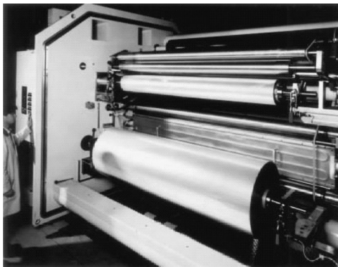
Figure 21.4 A DC magnetron substrate pretreatment system. Reproduced, with permission, from a conference presentation at AIMCAL, March 2, 2001
