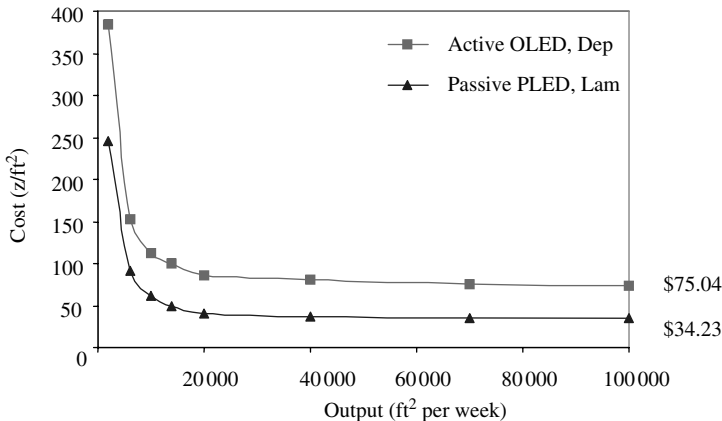
Figure 21.17 USDC results
