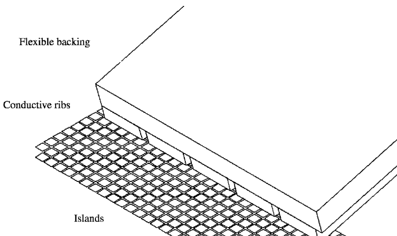
Figure 20.13 A section of a stylus wand linear electrode array for depositing image-wise charge on the islanded surface of a Gyricon display
