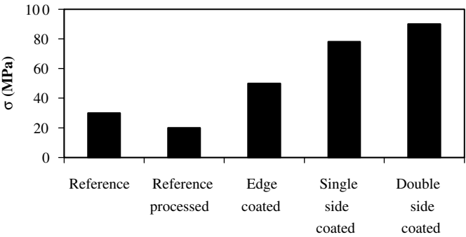
Figure 3.12 Influence of edge and surface (including edges) coating on the edge strength (P2 coating) at a failure probability of 1%
