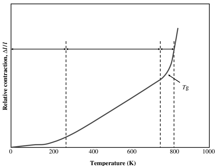
Figure 3.3 Length change of glass as a function of temperature
