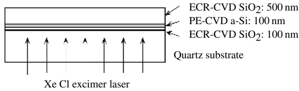
Figure 24.4 Cross-sectional structure of a test piece
