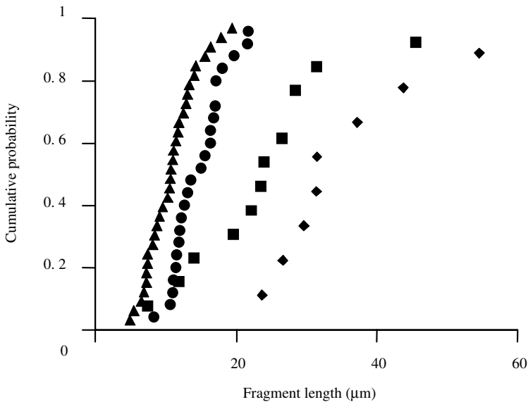
Figure 9.2 Cumulative probability of fragment length for ITO-coated PET at different strains: strained to (◆) 2.4%, (■) 2.6% (●) 3.1%, (▲) 3.7%
