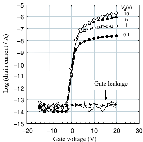
Figure 22.8 Transfer characteristic of an a-Si:H TFT on PES with SiN x /BCB gate insulator
