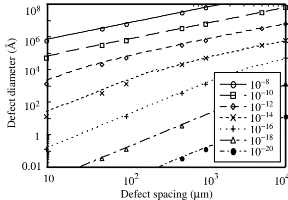
Figure 4.9 Graph showing the relationship between defect size and spacing for different values of effective diffusivity in the \text{AlO}_x layer. The calculations are based on a simple area fraction model described in the text
