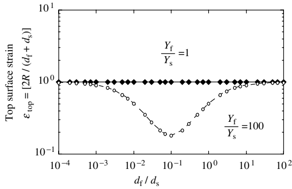
Figure 14.5 Normalized strain in the film as a function of film/substrate thickness ratio. Two types of substrate are illustrated: glass or steel ( Y_f/Y_s \cong 1 ) and organic polymer ( Y_f/Y_s \cong 100 ) (Suo et al. 1999)
