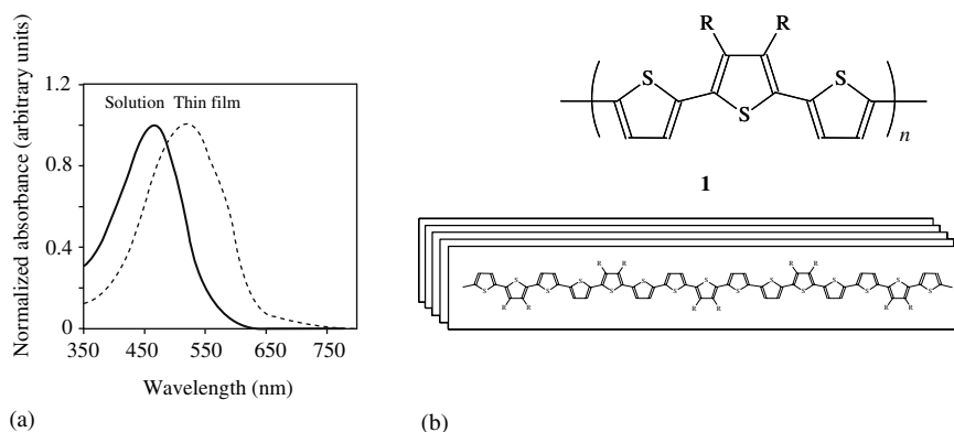
Figure 12.8 (a) Solution and thin film UV-visible spectra of 1a (1, \text{R} = \text{n-C}_{10}\text{H}_{23} ) and (b) face-to-face \pi - \pi stacking order of 1
