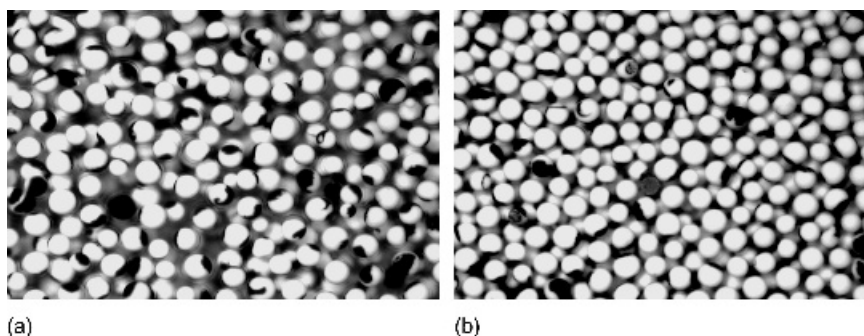
Figure 20.9 Photomicrographs of two Gyricon sheets: (a) a standard sheet and (b) a sheet that has been bead packed and swollen 19% rather than 25%
