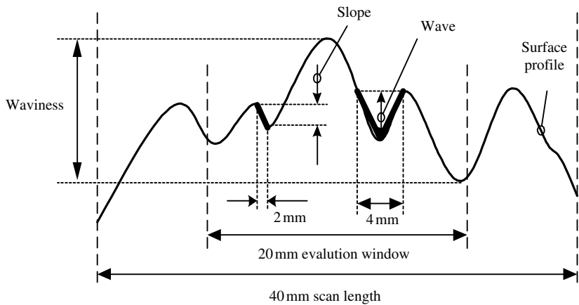
Figure 3.8 Detailed diagram of surface quality requirements for LCD technology
