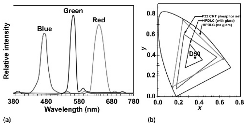
Figure 16.8 (a) The spectral reflectance of an RGB H-PDLC stack and (b) its corresponding chromaticity coordinates compared to a conventional CRT. Reproduced by the permission of the Society for Information Display
