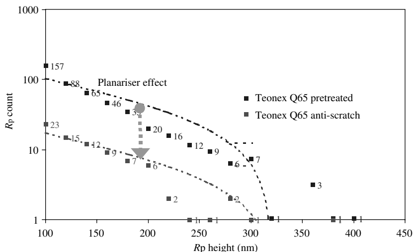
Figure 2.11 Surface peak defect R_p (highest point): frequency distribution of surface-engineered Teonex Q65. White light interferometry measurements, 1.6 \mu\text{m} from lateral resolution, approximately 5 \text{ cm} \times 5 \text{ cm} sampling area in total
