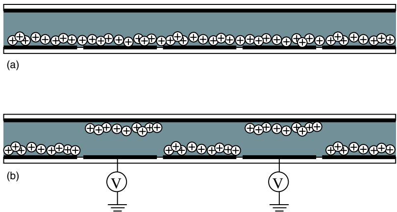
Figure 19.1 A thin electrophoretic film in cross section containing white scattering pigment particles in a dyed fluid. (a) The display appears dark or colored (viewer is above the display) because the pigment is behind the dyed fluid. (b) A voltage is applied to two pixels, driving the pigment over those pixels to the front of the display. These pixels appear white because the pigment is in front of the dyed fluid
