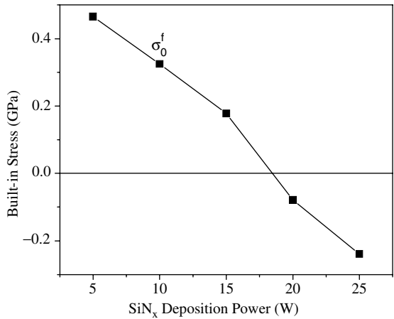
Figure 14.17 Built-in stress in the film when the sample is held in a frame. The stress is calculated or extracted for the samples of Figure 14.15. The horizontal line denotes zero stress. Positive stress stretches and negative stress compresses the film.
