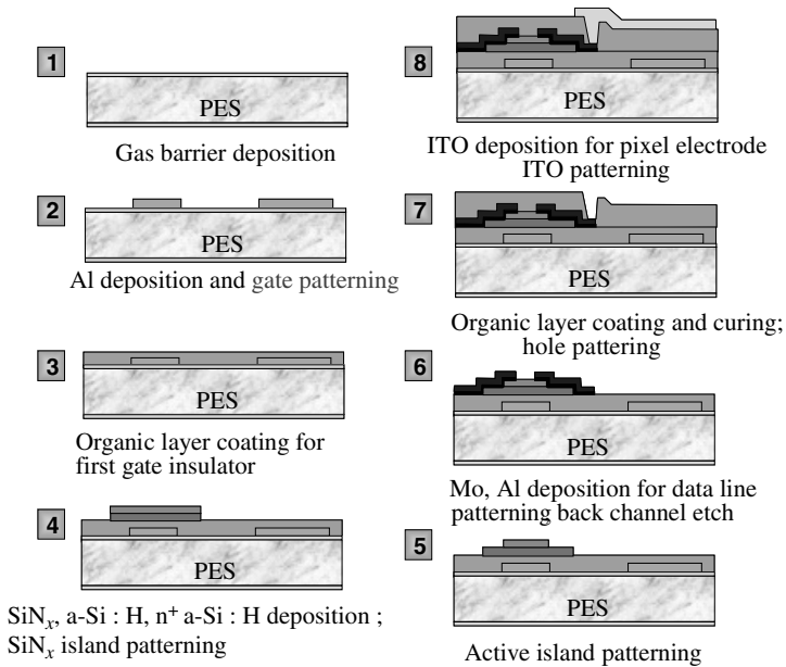
Figure 22.11 Fabrication procedure of an inverted staggered BCE a-Si:H TFT with organic layer as the first gate insulator for a plastic TFT LCD
