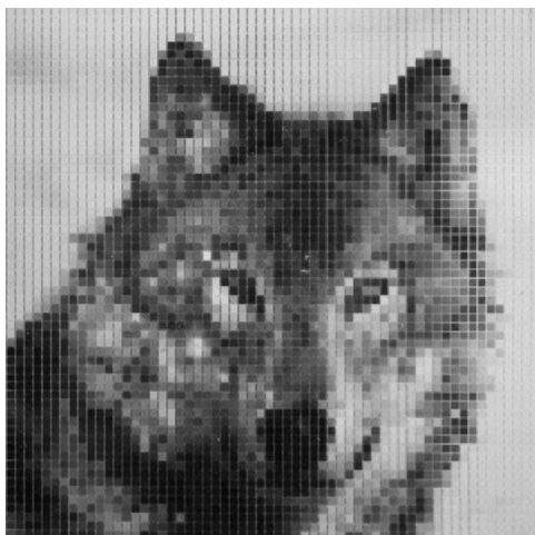
Figure 13.1 An image on a 64 \times 64 display on glass driven by 4096 polymer TFTs, with solution-processed PTV as the semiconductor. An image containing 256 grey levels is shown; the display is refreshed at 50 Hz
