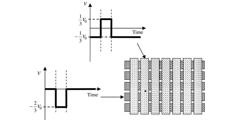
Figure 19.4 A passive matrix addressing scheme. The pixels are defined by row electrodes on one substrate and column electrodes running in the orthogonal direction on the other substrate. Example voltage curves used to address the pixel marked by an asterisk with voltage V_0 are also shown. In this scheme, other pixels in the display experience crosstalk voltages as large as one-third of the addressing voltage
