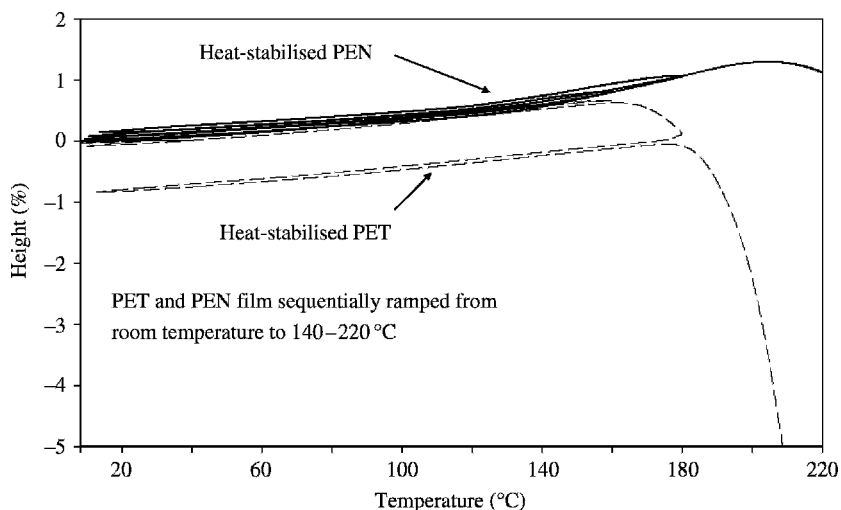
Figure 2.4 Thermal analysis of heat-stabilised polyethylene terephthalate and heat-stabilised polyethylene naphthalate films
