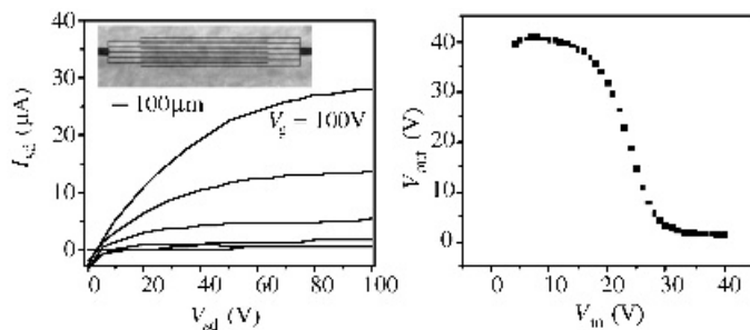
Figure 11.12 The left-hand image shows current–voltage characteristics of an n-channel transistor formed with electrodes patterned by nanotransfer printing. Laminating these electrodes against a substrate (PET) that supports an organic semiconductor (FCuPc), a gate dielectric, and a gate completes the device. The inset shows an optical micrograph of the interdigitated electrodes. The right-hand image shows the transfer characteristics of a complementary logic gate that uses this device and a similar one for the p-channel (pentacene) transistor
