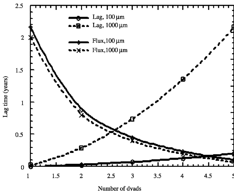
Figure 4.10 Comparison of relative sensitivity of lag time versus steady-state flux given an order of magnitude change in defect spacing
