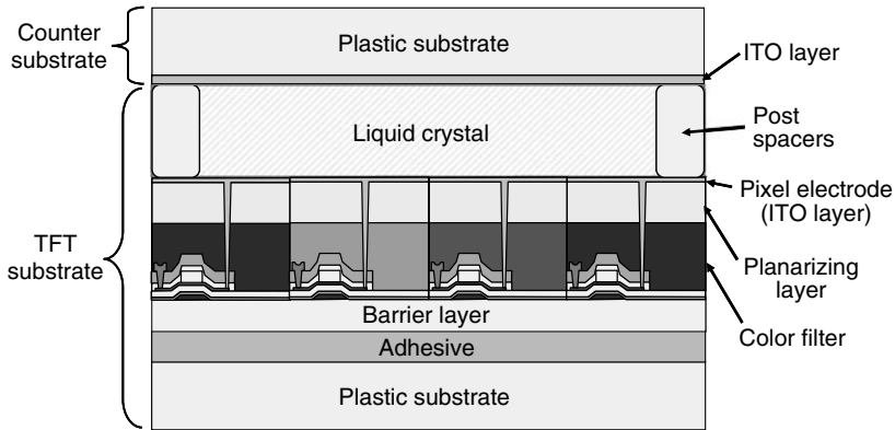
Figure 23.12 Structure of a transmissive color plastic LCD. Polyimide layers are abbreviated
