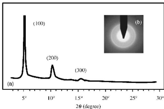
Figure 12.13 (a) XRD of an annealed thin film of PQT showing diffraction peaks at 2\theta = 5.1^\circ (100), 10.3^\circ (200) and 15.4^\circ (300). (b) Transmission electron diffraction pattern of a freestanding film of PQT-12 on a carbon grid showing diffraction at 3.7 \text{ \AA}
