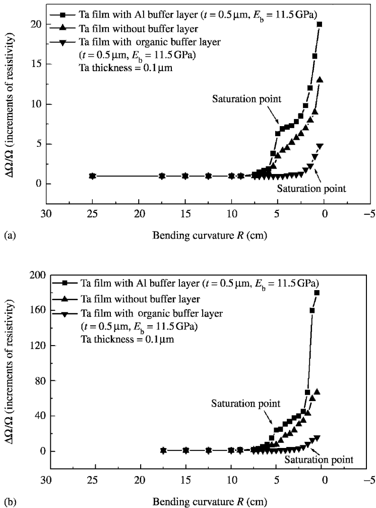
Figure 7.6 (a) Dependence of the increment of electrical resistivity in Ta films on buffer layers after exposure to compressive bending force, and (b) the tensile bending force
