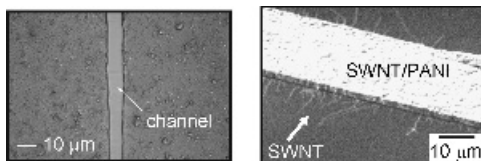
Figure 11.10 The left-hand image shows an optical micrograph of source and drain electrodes of a PANI/SWNT patterned by thermal transfer printing. This structure defines a transistor channel length of \sim 7 \mu\text{m} . The right-hand image is a scanning electron micrograph showing the edge of a printed line. Note the SWNTs that pull out at the edges of this structure. These tubes interact with semiconductors in the transistor channels. Reprinted with permission from Elsevier
