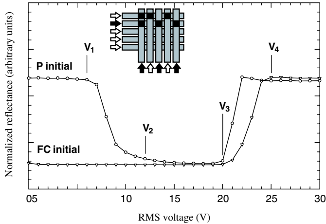
Figure 17.9 Electro-optic response curve of a cholesteric display driven by a voltage pulse, V , with a 250 Hz pulse 100 ms wide in a display with a cell gap of 5 \mu\text{m} . The cholesteric material was reflective in the yellow and formulated with a nematic liquid crystal of \Delta n = 0.22 and \Delta\epsilon = +31.4 . The voltages V_1 , V_3 , and V_4 are the thresholds important for multiplexing a high-resolution display for passive addressing as illustrated in the inset
