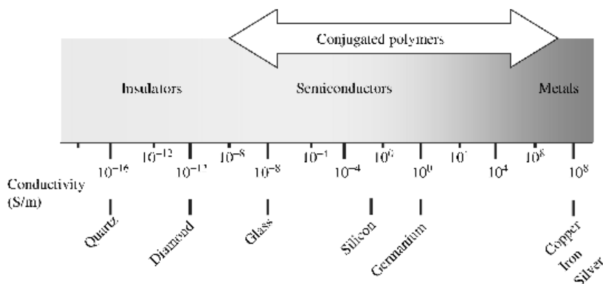
Figure 8.3 Conductive polymers within the conductivity spectrum
