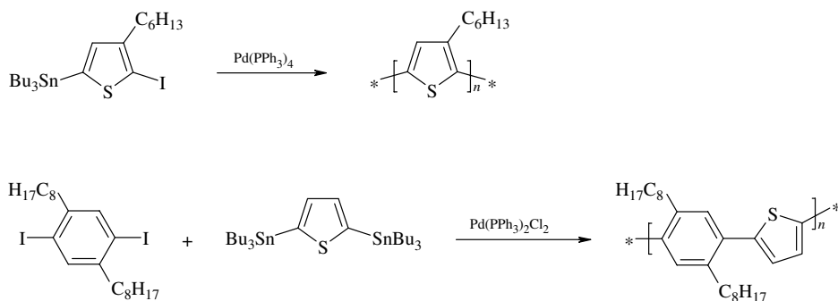
Scheme 8.6 Polymerization reactions via the Stille methodology (Iraqi and Baker 1998; Bao et al. 1995)
