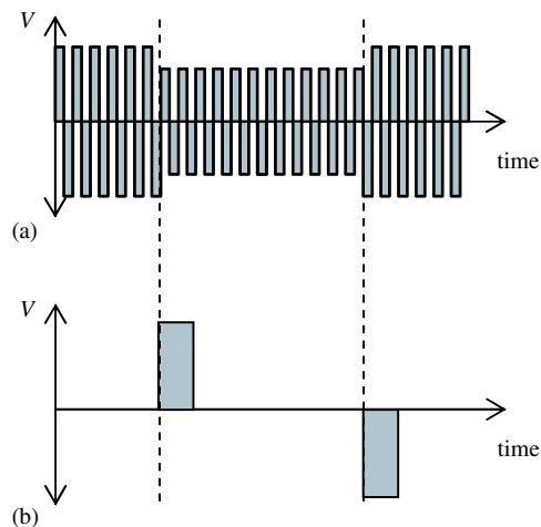
Figure 19.2 Representation of drive voltages required to achieve an image sequence where one begins in one optical state, transitions to another optical state, then goes back to the original optical state. (a) A sample waveform for a twisted nematic display and (b) a sample waveform for an image-stable electrophoretic display
