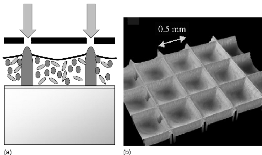
Figure 18.5 The two-step UV exposure to produce paintable LCDs. (a) Formation of the polymer walls. Local consumption of monomers induces a diffusion of monomers towards the exposed areas. (b) The resulting height variations could be observed with the aid of interferometric microscopy
