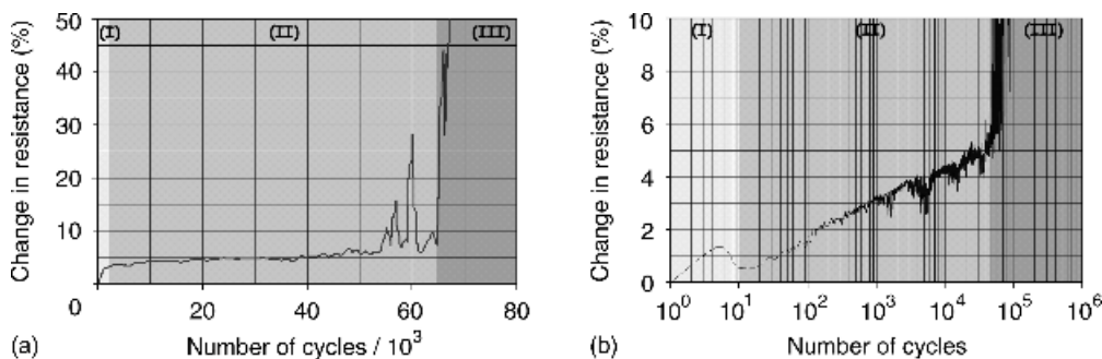
Figure 9.9 Fatigue test until catastrophic failure of ITO samples: linear scale (left) and logarithmic scale (right)
