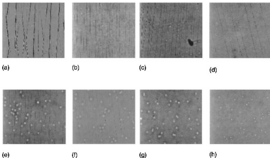
Figure 7.7 Optical images of cracks in ITO films in accordance with bending curvature and buffer layer: (a–d) without buffer, (e–h) with buffer for (a) R = 1 cm, (b) R = 2 cm, (c) R = 4 cm, (d) R = 10 cm, (e) R = 1 cm, (f) R = 2 cm, (g) R = 4 cm, (h) R = 10 cm
