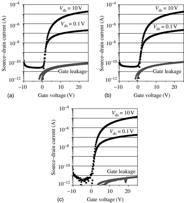
Figure 14.19 Transfer characteristics of the TFTs in Figure 14.17: (a) 5 W \text{SiN}_x , (b) 12 W \text{SiN}_x , (c) 25 W \text{SiN}_x . The TFT gates are 80\text{ }\mu\text{m} wide and 10\text{ }\mu\text{m} long (Cheng 2004)
