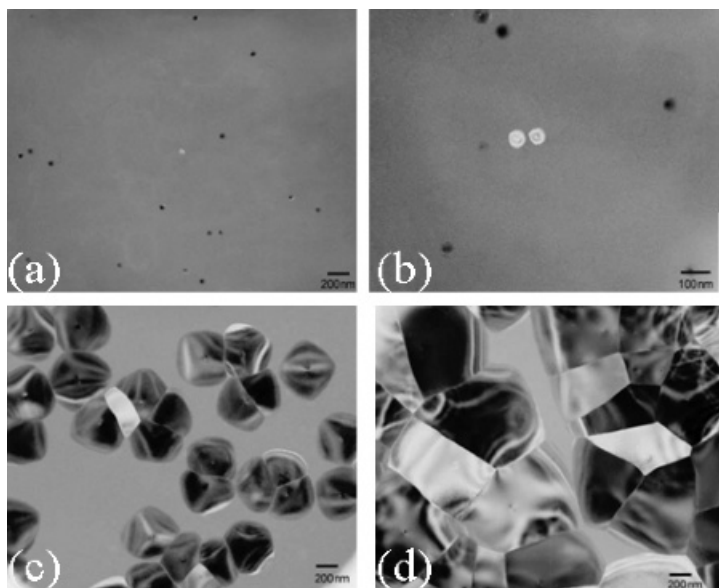
Figure 5.6 In situ TEM showing crystallization of DC magnetron sputter deposited amorphous ITO during annealing at 250 °C for approximately (a) 0, (b) 0.5, (c) 2.5, and (d) 5 h
