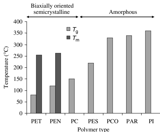
Figure 2.1 Comparison of a range of plastics by glass transition
