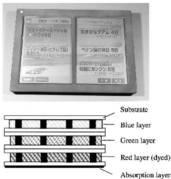
Figure 17.11 Two A4 size, 2048 × 1440 pixel, 180 dpi cholesteric reflective display by Minolta on plastic substrates in RGB color in a stacked configuration for full-color operation. Photo reproduced by the permission of Minolta (Kiyofumi Hashimoto). Diagram reproduced by the permission of the Society for Information Display
