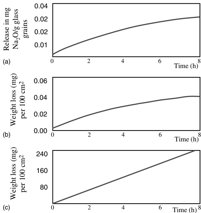
Figure 3.2 Chemical durability of Borofloat against (a) water attack, (b) acid attack, and (c) alkali attack
