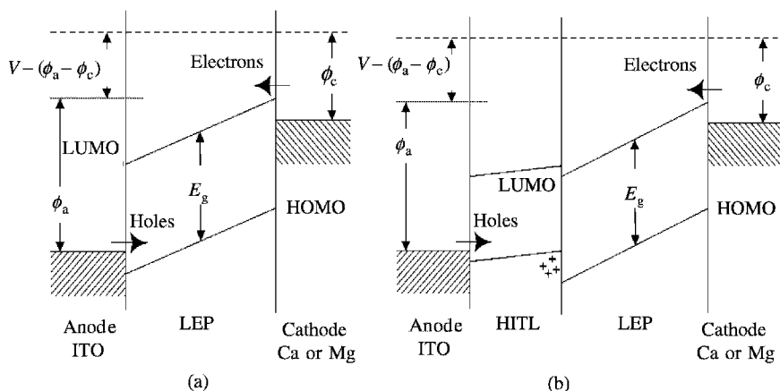
Figure 15.2 Illustrative band diagrams of (a) single-layer and (b) two-layer PLED diodes under a bias V with LEP energy gap E_g , cathode work function \phi_c , and anode work function \phi_a
