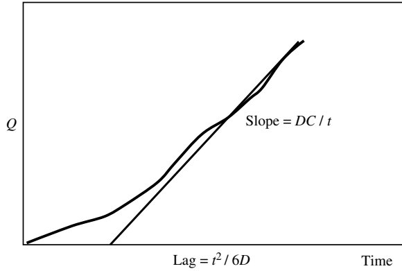
Figure 4.3 Conceptual plot of cumulative permeation data, defining lag time and steady-state regimes for a single-layer system
