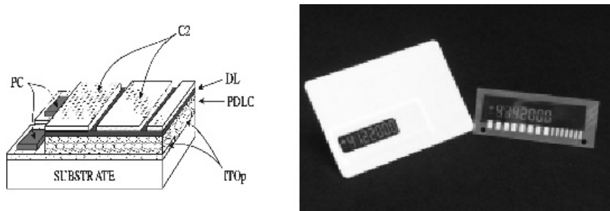
Figure 17.15 (Left) Diagram of the layers in a flexible cholesteric display developed by Kodak using photographic methods showing the backplane conductors (C2), dark layer (DL), and droplet dispersion (PDLC). (Right) A seven-segment cholesteric display fabricated with photographic methods for credit card applications. Reproduced by the permission of the Society for Information Display
