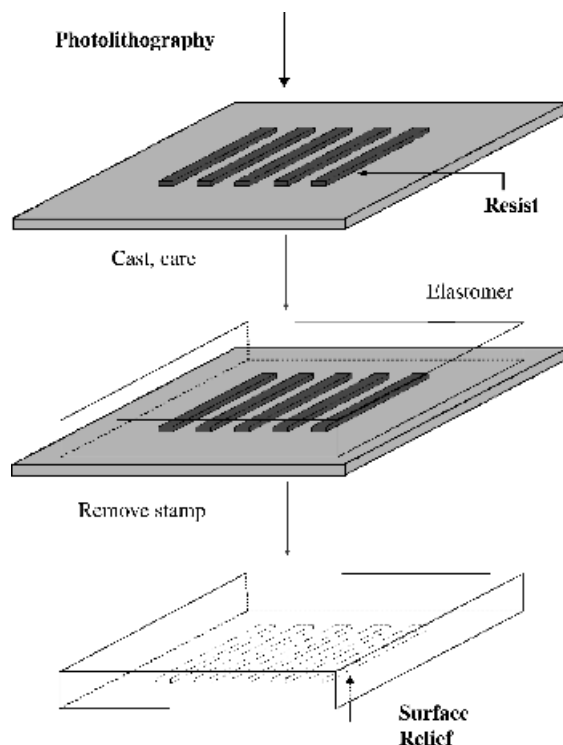
Figure 11.2 Casting and curing procedures for building high-resolution stamps. The first step involves patterning a layer of resist on a flat substrate to define a master. It is convenient to use a technique such as photolithography for this purpose. Casting, curing (thermally or optically) and then peeling the resulting polymer away from the master yields a stamp. Many stamps can be made with a single master and each stamp can be used many times. Reproduced by the permission of the American Institute of Physics
