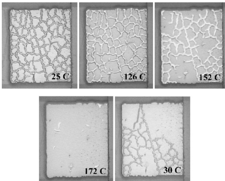
Figure 6.16 Buckling pattern during heating and subsequent cooling
