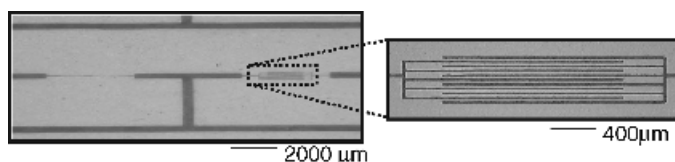
Figure 11.8 Optical micrographs of thermal transfer printed patterns of the doped conducting polymer PANI/SWNT. The left-hand image shows printed source and drain electrodes and interconnections for a complementary logic gate. The right-hand image shows a magnified view of interdigitated source and drain electrodes for the n-channel transistor of this simple circuit. Reprinted with permission from American Physical Society
