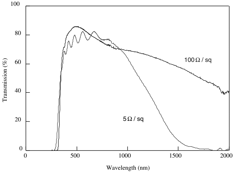
Figure 5.1 Transmission curves for two TCO films of SnO 2 having different sheet resistances. Note the decrease in long-wavelength transmission for the lower-resistivity material. Courtesy of D. Ginley, NREL
