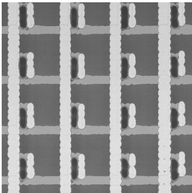
Figure 12.16 Portion of a 128 \times 128 all-jet-printed OTFT array. An array pitch of 340 \mu\text{m} corresponds to a 75 dpi array. Gate lines run horizontally and source lines run vertically through the photomicrograph. The semiconductor, nanoPQT, is printed into the channel, where it wets the print-patterned gold source and drain. No pixel electrode or pixel capacitor is shown. The dielectric was deposited by PECVD
