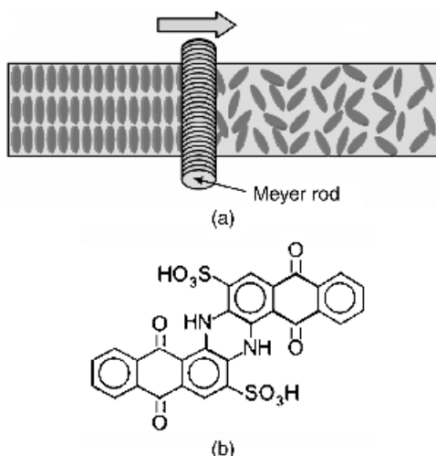
Figure 10.1 (a) Schematic diagram of the Meyer rod coating technique used to produce thin crystal film polarizers. The directors of the molecules align in the direction of the shear force during the coating process. (b) Indanthrone disulfonate, a blue discotic dye used in the fabrication of thin crystal film polarizers
