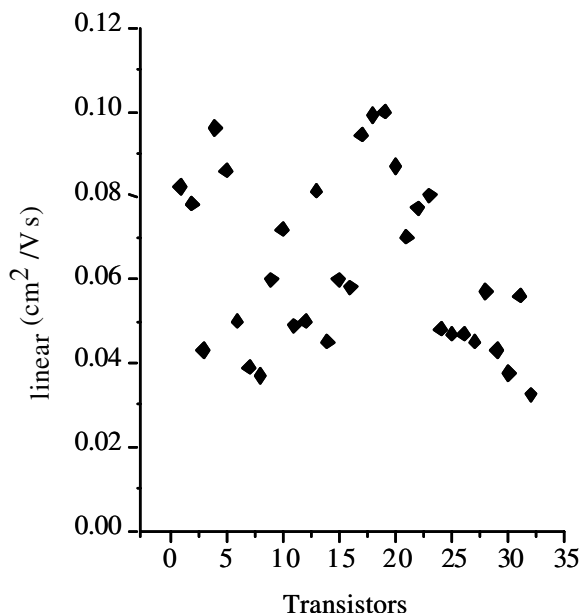
Figure 12.17 Uniformity of mobility across a printed array. Mean = 0.063 \text{ cm}^2/\text{V s} , deviation = 0.021 \text{ cm}^2/\text{V s} , linear regime V_D = 1 \text{ V}
