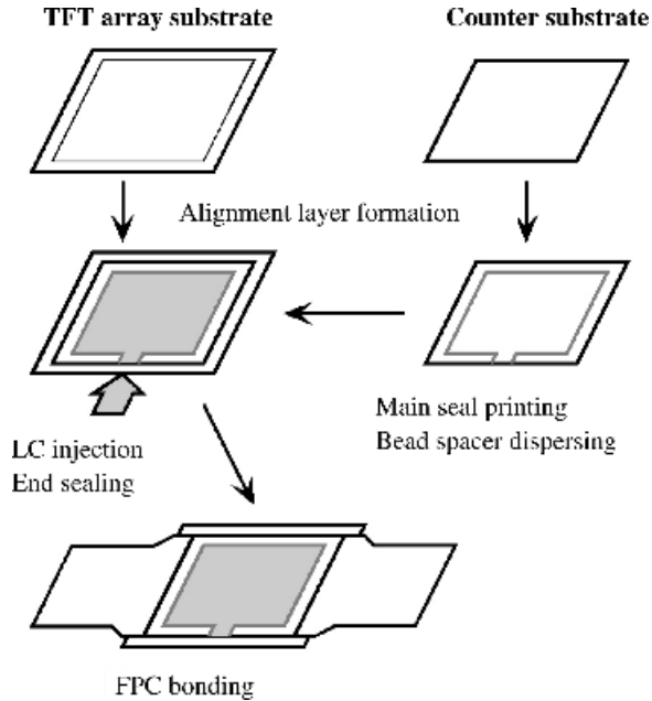
Figure 24.13 TFT LCD assembly process
