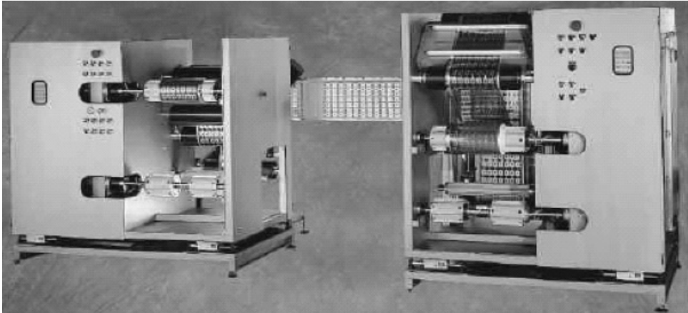
Figure 21.7 Web handling: Northfield Automation's vertical process unwind/rewind with accumulation and tension control
