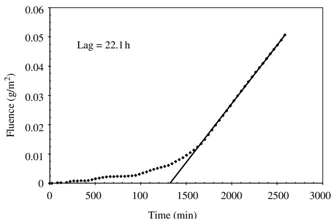
Figure 4.6 Representative data from the four-layer system (PET/P1/AlO x /P2) water vapor permeation experiments showing a lag time of approximately 22 h
