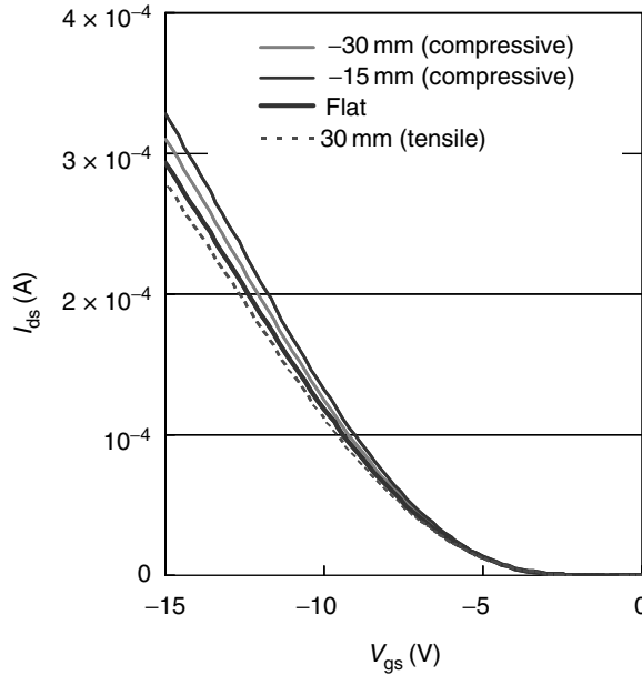
Figure 23.8 Plots of p-channel TFT performance ( I_{ds} versus V_{gs} ) at various curvatures
