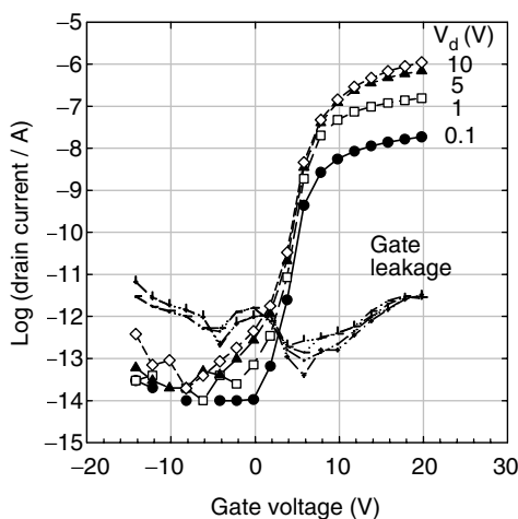
Figure 22.6 Transfer characteristic of an a-Si:H TFT on PES with \text{SiN}_x gate insulator
