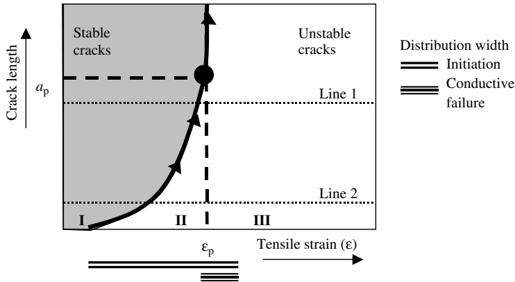
Figure 6.12 Schematic representation of the growth size at increasing strain levels
