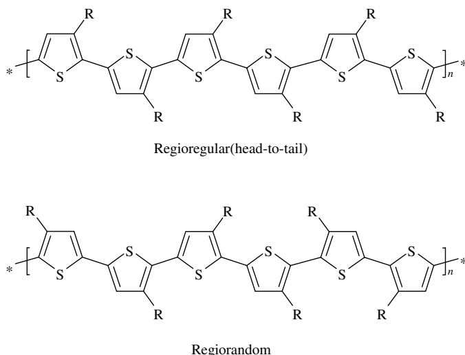
Figure 8.8 Regioregular versus regiorandom poly(3-alkylthiophene)
