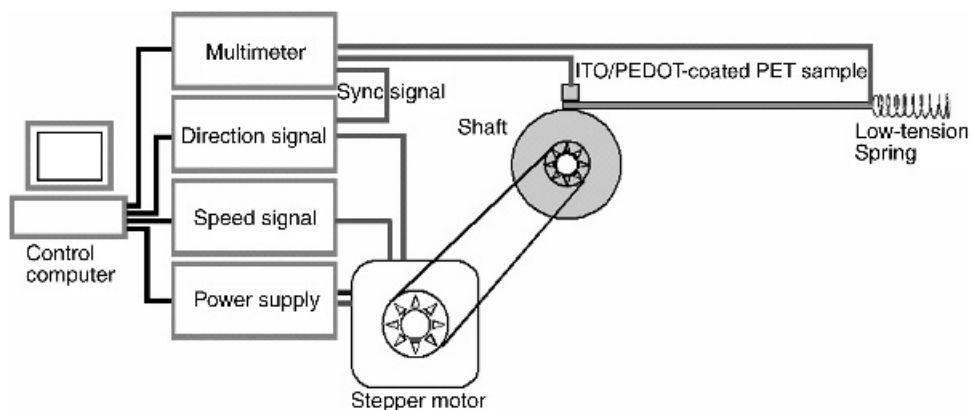
Figure 9.7 Schematic of custom-built apparatus to monitor resistance during cyclic mandrel bending
