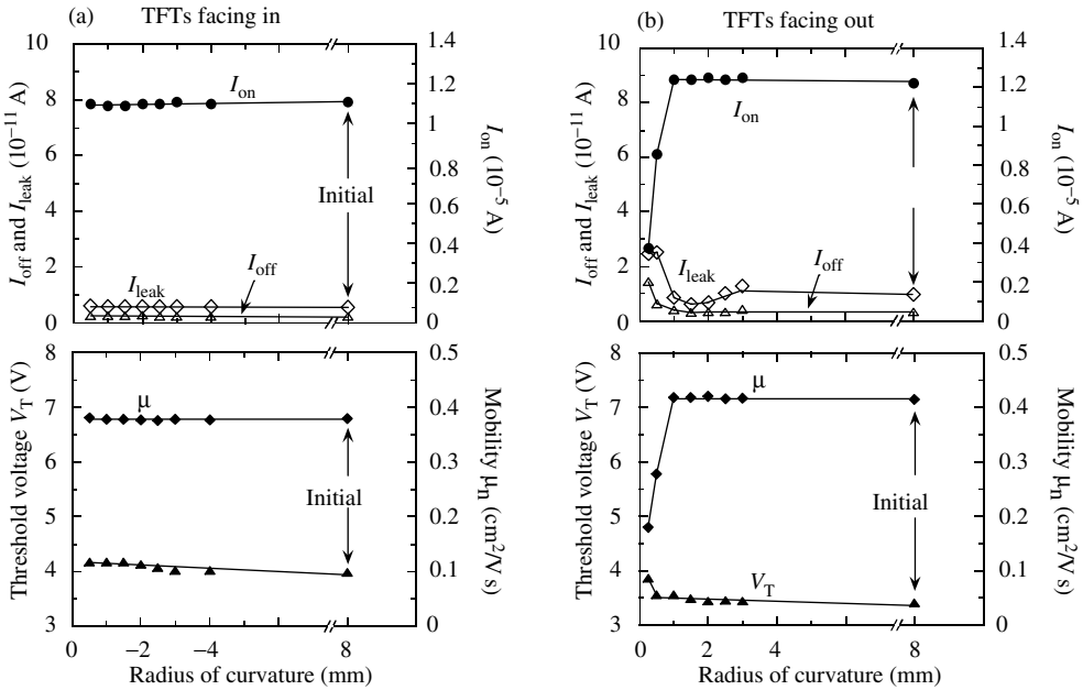
Figure 14.20 On-current, source-gate leakage current, off-current, electron mobility and threshold voltage in the saturation regime as functions of bending radius. I_{off} is the smallest source-drain current at V_{ds} = 10 V, I_{on} is the source-drain current for V_{ds} = 10 V and the gate voltage V_{gs} = 20 V, and I_{leak} is the source-gate current for V_{ds} = 10 V and V_{gs} = 20 V. Outward bending R is defined positive, inward bending negative. The as-fabricated radius, before bending, was 8 mm. Differences between the “initial” characteristics reflect spread between as-fabricated TFTs (Gleskova et al. 1999)
