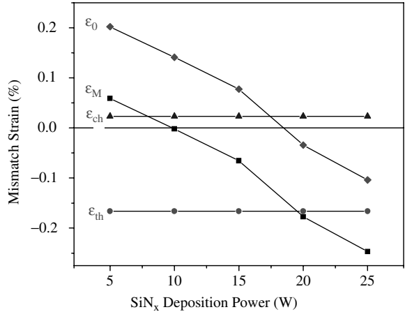
Figure 14.16 Mismatch strain components calculated or extracted for the samples of Figure 14.15. The horizontal line denotes zero strain. The film is under tension at positive strain and compression at negative strain. (Cheng, 2004a)
