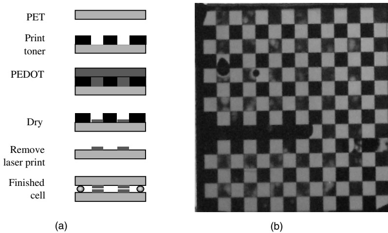
Figure 17.17 (a) The steps in patterning conducting polymer, PEDOT, electrodes with a standard office printer. (b) Cholesteric reflective display passive matrix demonstration fabricated with conducting polymer electrodes using this method
