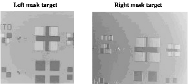
Figure 15.5 Metal deposition and patterning on the same substrate as in Figure 15.4 increases misalignment to \sim 25\text{ }\mu\text{m}
