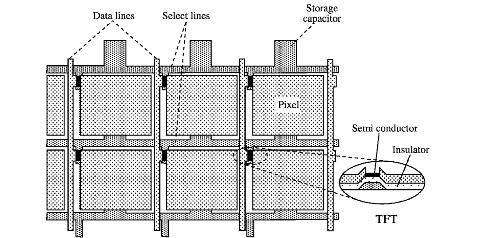
Figure 19.5 One type of active matrix backplane. The horizontal select (row) lines control whether the thin film transistor (TFT) is in depletion (insulating) or accumulation (conducting). Data (column or source) lines run vertically and bring voltages to the pixel electrodes. In this example, storage capacitors are formed by extending the select line from the previous row beneath the pixel electrode. In other variants, separate horizontal conductor lines form the storage capacitors
