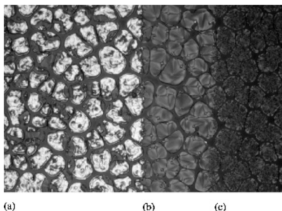
Figure 17.14 Domain textures in cholesteric droplets where the microscope photo is of a display cell that overlaps two pixels and the area between. The pixel on the left was electrically switched to the planar texture whereas the pixel on the far right was switched to the focal conic texture. The area between the cells has no electrode and could not be electrically switched; however, it was thermally cooled into the focal conic state. Note that droplets at the electrode edge have both textures
