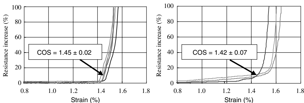
Figure 6.7 Normalized resistance change during bending (left) and tensile (right) loading of 100 nm thick ITO coatings on polymer films, in the vicinity of the critical strain for failure. Reproduced by the permission of SVC
