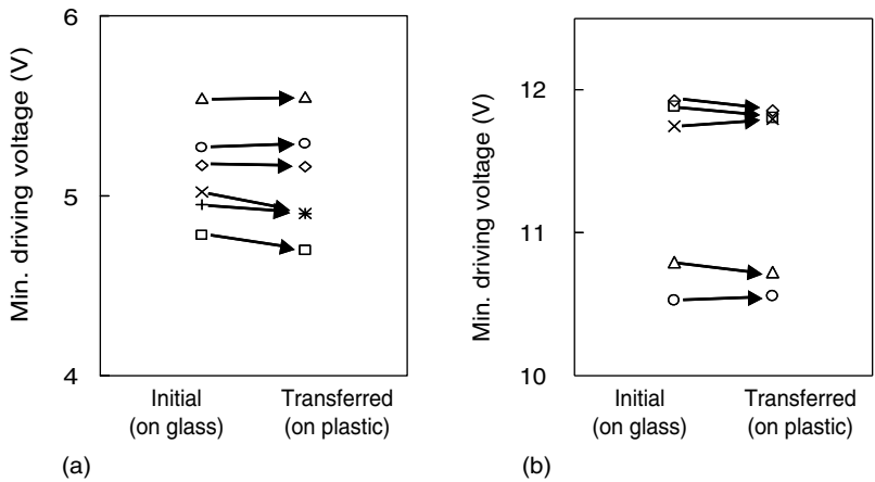
Figure 23.6 The change in the minimum driving voltage for (a) scanning and (b) data drivers on a 1.5 in transmissive LCD before and after the transfer process
