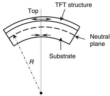
Figure 14.3 A film-on-foil structure bent to a cylindrical roll. When a TFT backplane of thickness d is rolled to a radius r , the thin film is put into a well-defined strain, which is tensile when the film is on the outside of the roll and compressive when the film is on the inside
