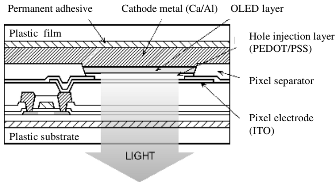
Figure 24.17 Cross section of the pixel circuit of the TFT OLED display circuit
