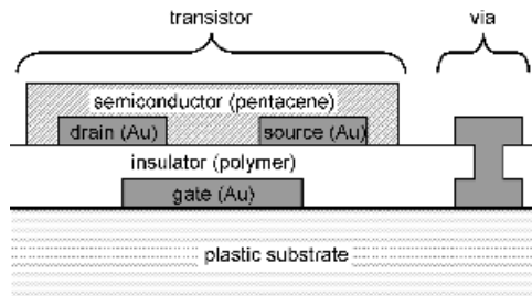
Figure 13.2 Cross section of a TFT and vertical interconnect (via)
