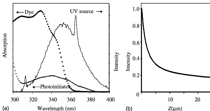
Figure 18.3 (a) The spectrum of the UV source used in the experiments and the absorption spectra of the stilbene dimethacrylate compound and the photoinitiator. In acetonitrile the extinction coefficient of the stilbene dimethacrylate compound is 25\,000\text{ M}^{-1}\text{cm}^{-1} at 340 nm. Light above 370 nm is not absorbed by the stilbene dimethacrylate, so a small part of the UV light emitted by the UV source can penetrate the whole layer. (b) A typical gradient calculated for a 25 \mu\text{m} film at the onset of irradiation
