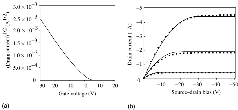
Figure 12.2 Current–voltage characteristics of OTFT on glass with PQT-12, W = 200 \mu\text{m} and L = 50 \mu\text{m} . (a) Saturation regime for V_{DS} = -30 V. From this we can obtain \mu = 0.07 \text{ cm}^2/\text{V s} and V_T = -1 V. (b) Output characteristics for V_G = -10, -20, -30 V (squares) and computed (line). Note that even for such a long transistor, some variation from the model is indicated by the current variation for high V_{DS}
