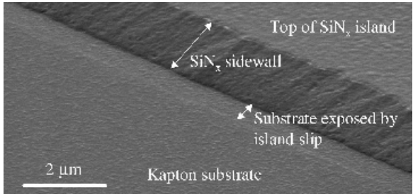
Figure 14.11 SEM micrograph of the edge of an SiN x island on a polyimide foil after deformation of the foil to a dome. The substrate exposed by island slip is seen at the edge of the island (Bhattacharya 2003)
