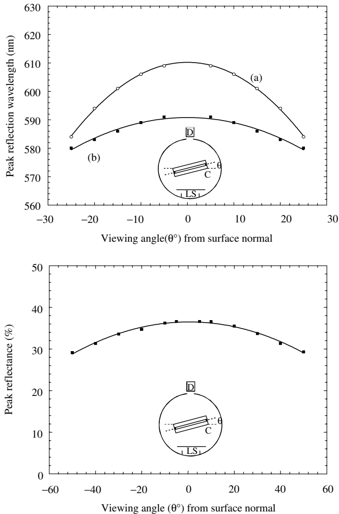
Figure 17.5 The upper figure shows the effect of domain size on color shift with (a) the change in the peak wavelength for a large domain texture and (b) a small domain texture. The lower figure shows reflectance versus view angle. The measurements were made under diffuse lighting conditions
