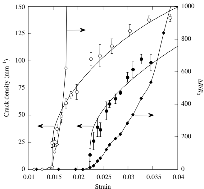
Figure 6.8 Density of tensile cracks and normalized resistance change during tensile loading of ITO coatings on polymer substrate. The coating thicknesses are (●) 50 nm and (○) 100 nm. Reprinted from “Mechanical Integrity of Transparent Conductive Oxide Films for flexible Polymer-Based Displays”, vol 460, Leterrier Y., Médico L., Demarco F., Manson J.-A. E., Bouten P., DeGoede J., Nisato G., Nairn J. A., “Thin Solid Films”, pp. 156–166 (2004) with permission from Elsevier
