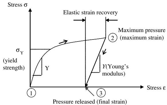
Figure 14.12 Stress-strain diagram illustrating the tensile shaping of a polymer substrate (step 1 to 2) followed by elastic snap-back (step 2 to 3) (Hsu et al. 2002b)
