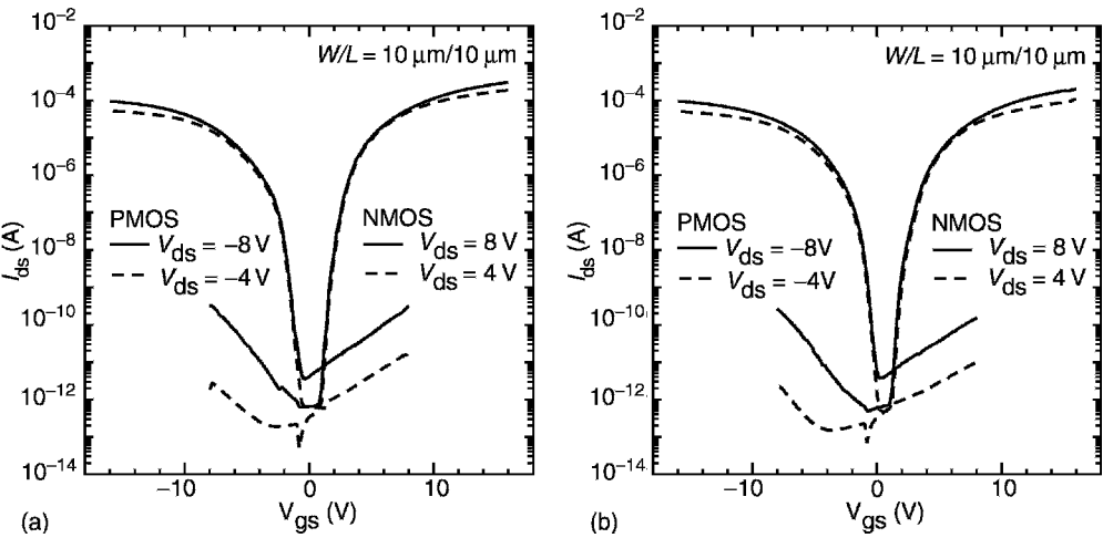
Figure 24.9 Transfer characteristics of the TFTs measured (a) before and (b) after transfer
