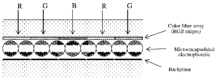
Figure 19.10 Schematic representation of a full-color microencapsulated electrophoretic film. On the front sheet, a color filter with red, green, and blue stripes is registered to subpixels on the backplane. Three subpixels constitute a full-color pixel. The three subpixels on the left form a pixel, and the particle configuration gives a yellow color. This is because light is back-reflected through the red and green stripes, and light passing through the blue stripe is absorbed
