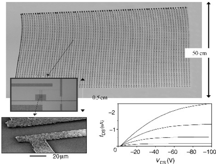
Figure 11.21 Active matrix backplane circuit formed by thermal transfer. A photograph of a 50 cm × 75 cm printed panel is shown at the top. The micrograph at the middle left illustrates a unit cell of the circuit. The scanning electron micrograph at the bottom left provides a high-resolution view of the source and drain electrodes and the channel region. The graph at the bottom right shows the electrical characteristic of one of the transistors in the large printed panel. The gate voltage varies from 0 to -100 V in -20 V steps
