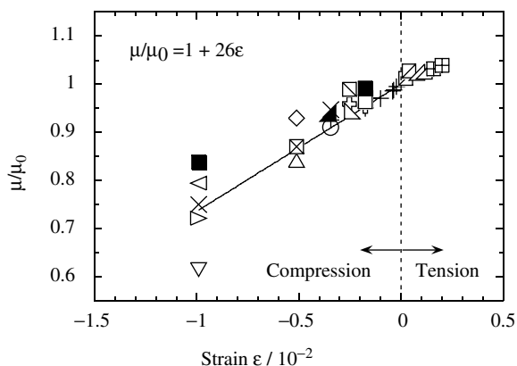
Figure 14.7 Electron mobility in a-Si TFTs plotted as a function of strain. Each symbol represents a different TFT. Empty and full symbols correspond to TFTs with the bending direction parallel and perpendicular to the source–drain current path, respectively. The linear fit is for TFTs with the bending direction parallel to the source–drain current path (Gleskova et al. 2002)
