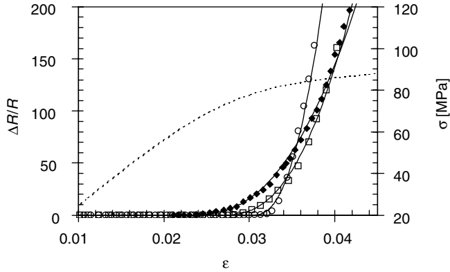
Figure 9.3 Fractional change in resistance \Delta R/R of ITO-coated PET as a function of strain \varepsilon (left-hand axis). Experimental data for three thicknesses are shown as points: ( \blacklozenge ) 105 nm, ( \square ) 42 nm, and ( \circ ) 16.8 nm; modeled fits are shown as solid lines. The stress–strain curve for ITO-coated PET (right-hand axis) is shown as a dotted line. Reprinted, with permission, from Applied Physics Letters 76 , 1425 (2000)
