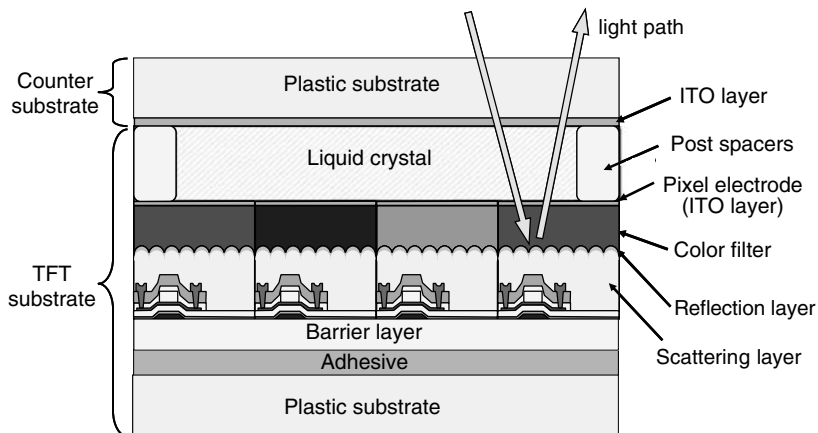
Figure 23.13 Structure of a reflective color plastic LCD. Polyimide layers and contact holes are abbreviated
