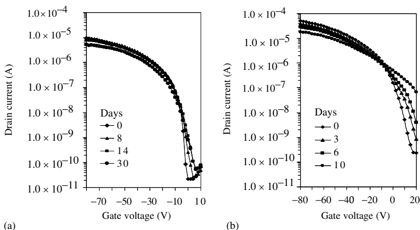
Figure 12.10 Transfer characteristics in the saturated regime of OTFTs ( L = 165 \mu\text{m} ; W = 5000 \mu\text{m} ; V_D = -80 V) as a function of time: (a) 1a-OTFT; and (b) HT-P3HT-OTFT. The devices were stored in air in the dark at 30% relative humidity and characterized under ambient conditions and annealed before measurement
