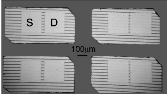
Figure 11.18 Optical image of a set of TFTs formed on a plastic substrate with aligned arrays of single crystal silicon ribbons as the semiconductor.
