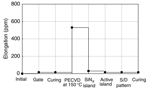
Figure 22.13 Elongation of the substrate during the TFT process step for an a-Si:H TFT on PES with BCB as the first gate insulator
