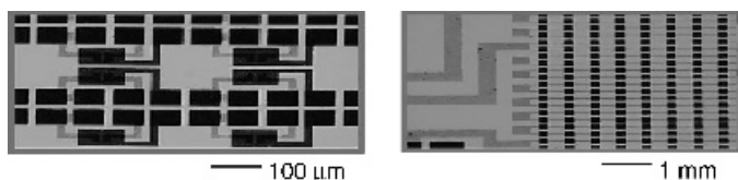
Figure 11.9 Optical micrographs of some patterns that consist of multiple thermal transfer printed layers of conducting films. The results illustrate multilayer printing with good registration
