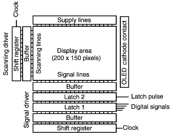
Figure 24.15 Block diagram of the TFT OLED display circuit
