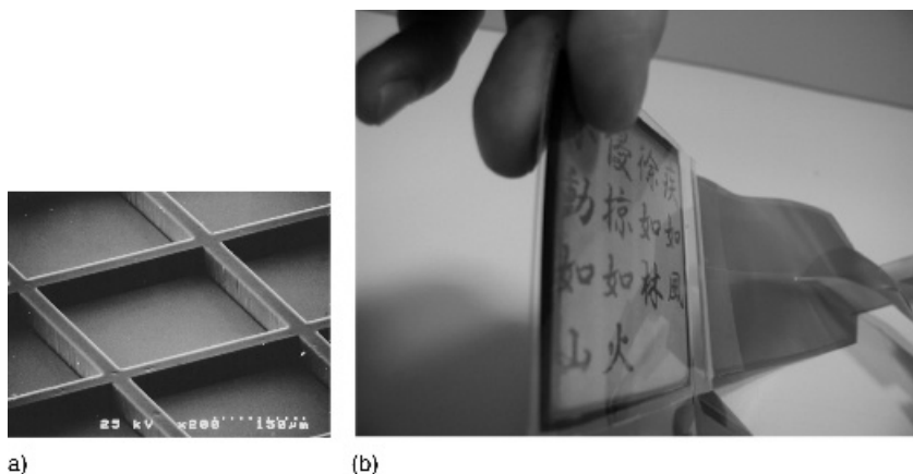
Figure 19.14 (a) Microscope image of the rib structure on a substrate used to make the air-gap electrophoretic film. (b) A 160 \times 160 passive matrix display made on a plastic substrate by Bridgestone and Kyushu University. Part (a) reproduced by the permission of the Society for Information Display
