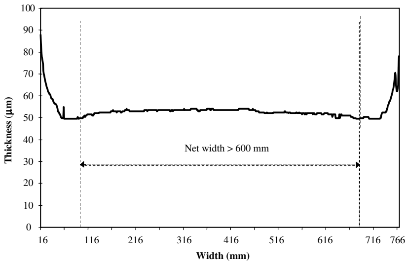
Figure 3.7 Thickness data for a large 50 \mu\text{m} thin glass sheet produced by the DD technology
