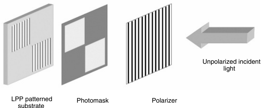
Figure 10.7 Schematic diagram of the fabrication process used for creating a multidomain LPP alignment layer
