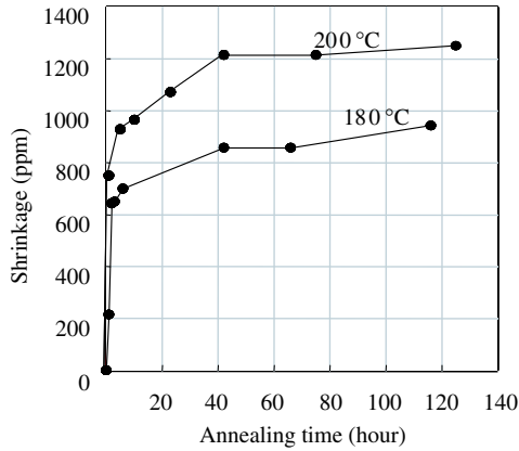
Figure 22.12 Shrinkage of a PES during the annealing process at 180 and 200 °C
