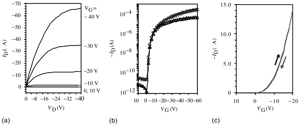
Figure 12.14 I - V characteristics of exemplary PQT-12 OTFTs with 90\text{ }\mu\text{m} channel length and 5000\text{ }\mu\text{m} channel width: (a) output curves at different gate voltages; (b) two transfer curves in the saturated regime scanned from positive to negative gate voltages (o and \times , V_D = -60\text{ V} ) and the transfer curve in the linear regime ( \Delta , V_D = -6\text{ V} ); (c) two transfer curves scanned in different directions between +10\text{ V} and -20\text{ V}
