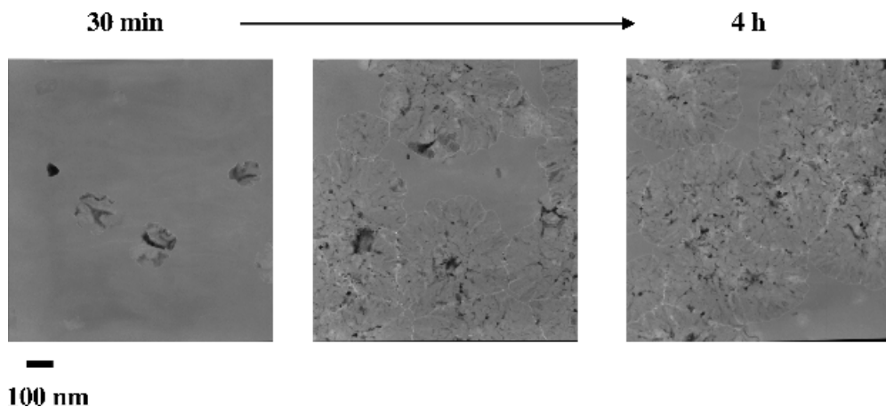
Figure 5.7 TEM image showing the amorphous (a) to crystalline (c) transformation of IZO in air at 500 °C. Note the regions of lighter contrast at the grain boundaries and at the a/c interface indicating the depletion of In
