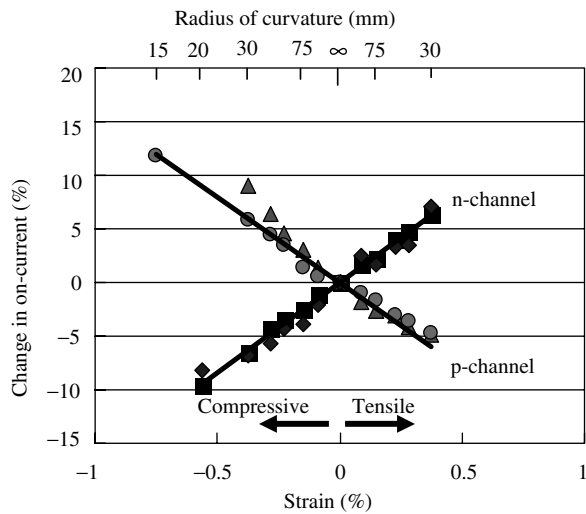
Figure 23.10 The change in on-current as a function of the strain in the polycrystalline silicon layer and as a function of the radius of curvature. Reproduced by permission of SID
