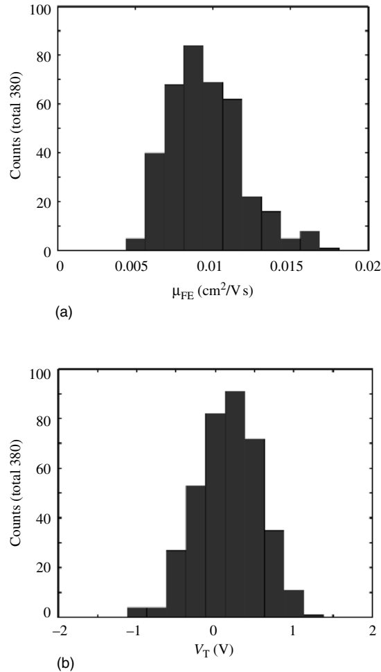
Figure 13.8 Impression of the uniformity of a QVGA active matrix backplane based on measurements of 380-pixel TFTs. (a) Distribution of the mobility, extracted from the transfer characteristics for V_{gs} = -20 V and V_{ds} = -1 V. (b) Distribution of the threshold voltage, obtained by fitting (13.1) to the transfer characteristics for V_{ds} = -1 V
