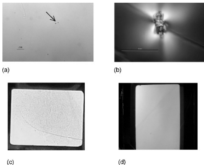
Plate 15.1 (a) Defects on commercially available optical grade PET; (b) magnification of defect; (c) display made with PET substrate having poor surface quality shows low output, grainy appearance, and line defect; (d) display made on PET substrate with improved surface quality has improved characteristics
