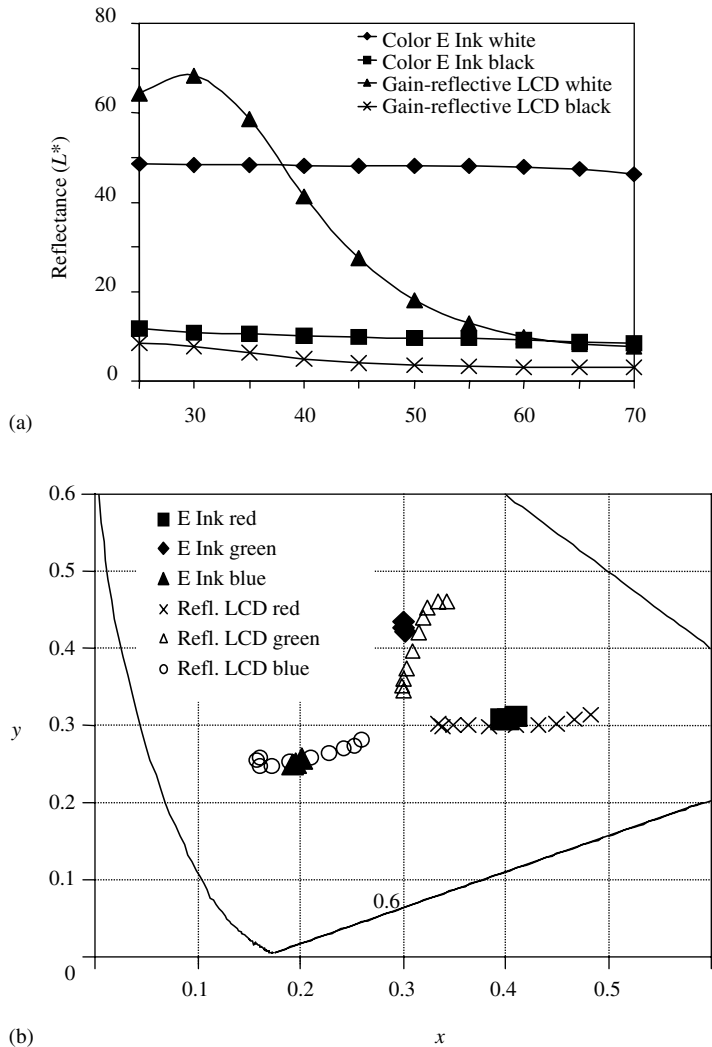
Figure 19.11 (a) Reflectivity and (b) color coordinates of a reflective E Ink electrophoretic color display and a commercial reflective color twisted nematic display as a function of illumination angle. The white and dark states of the E Ink display are insensitive to illumination angle, as are the color and saturation of red, green, and blue states
