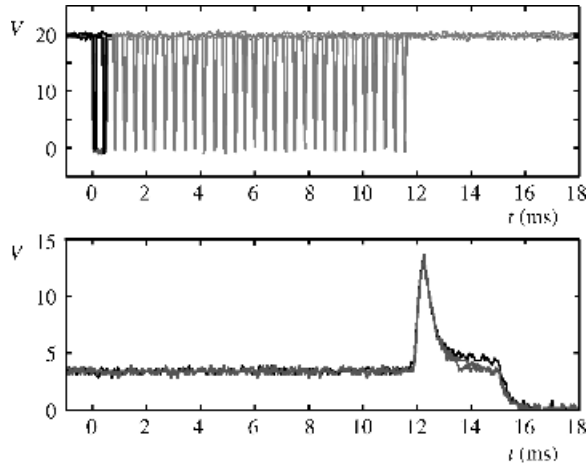
Figure 13.12 Measurement results of the 32-stage shift register: the top graph shows the clock pulses and the start pulse; the bottom graph shows the output pulse of the 32nd stage after 0, 2, and 4 h
