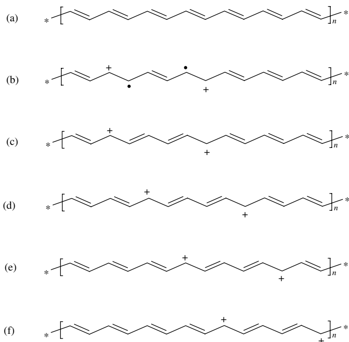
Figure 8.2 Transport of charges within conductive polymers (polyacetylene has been taken as an example): (a) neutral PAC, (b) PAC doped by oxidant, (c) radicals recombine; (d, e, f) transport of charges along the PAC backbone ( www.nobel.se/chemistry/laureates/2000/illpres )
