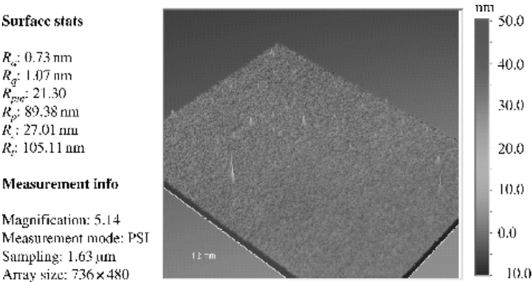
Figure 2.9 Surface smoothness of Teonex Q65 with an adhesion pretreat
