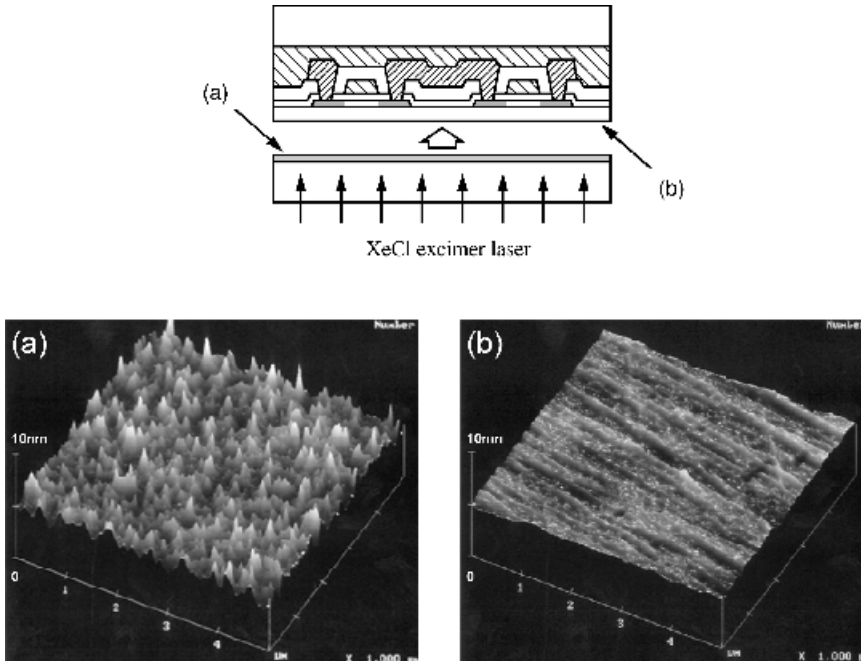
Figure 24.8 AFM images of the surface of (a) the sacrificial silicon layer and (b) the TFT underlayer of \text{SiO}_2 after transfer
