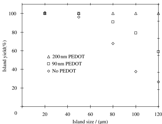
Figure 14.13 Yield of crack-free ITO islands on PET versus island size, without PEDOT cover and for two different thicknesses of PEDOT coverage (Bhattacharya et al. 2004)
