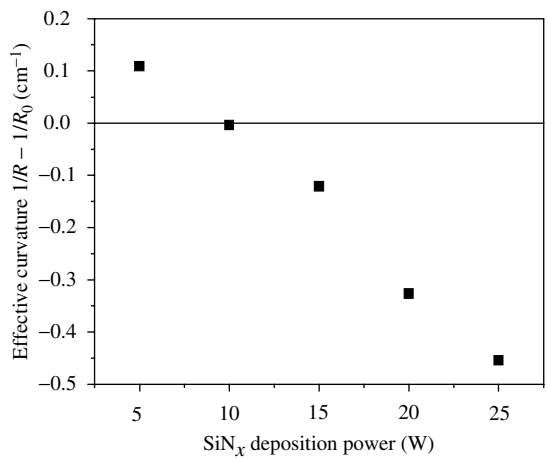
Figure 14.15 Effective curvature produced by PECVD deposition of 300 nm thick SiN x at 150 °C on 51 μm thick Kapton E polyimide substrates. Substrates are preheated for 50 min in vacuum; radii are measured after 30 min cooling in vacuum, at room temperature and RH = 29% (Cheng 2004)
