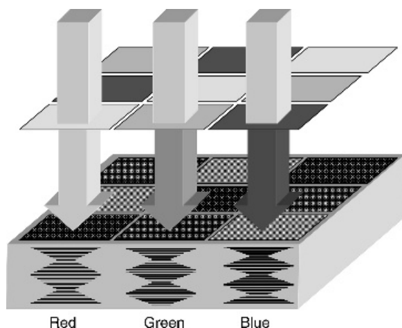
Figure 10.5 The single exposure step process used to fabricate color filters from cholesteric reactive mesogens
