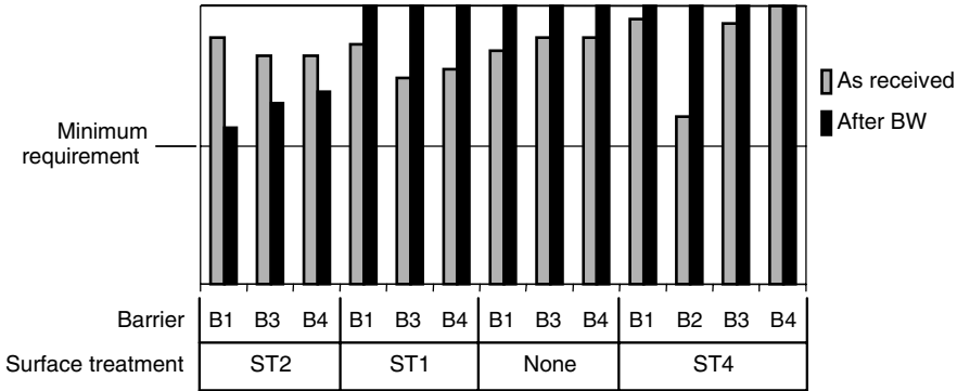
Figure 15.3 Adhesion of barrier layers on Teonex Q65 with various surface treatments; tests were performed on samples as received and after immersion in boiling water (BW)
