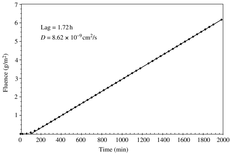
Figure 4.5 Representative data from the (PET/P1) water vapor permeation experiments
