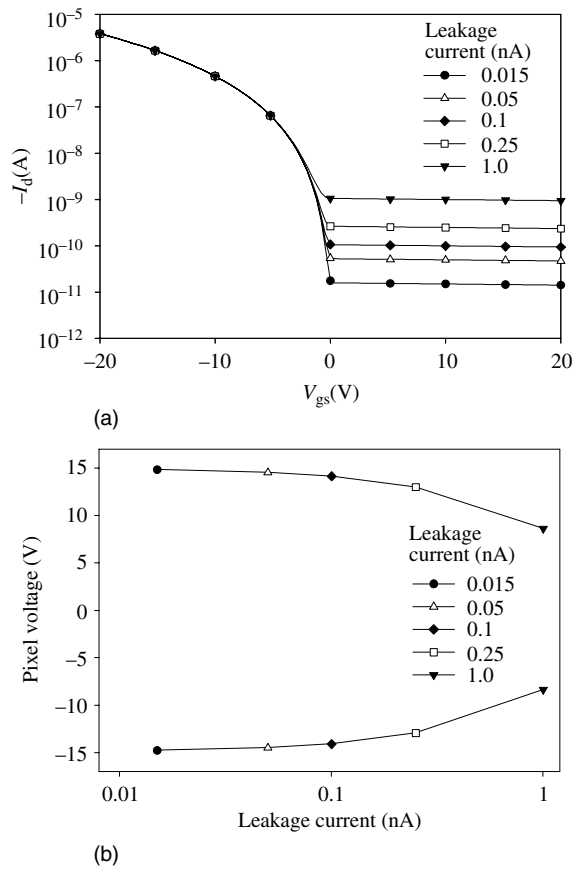
Figure 13.6 (a) Simulated transfer characteristics for V_{sd} = 20\text{ V} at five different values of the leakage current (A) shown in the key. The field-effect mobility was set to 0.05\text{ cm}^2/\text{V s} . (b) Simulated charging behavior of a pixel with the same five values for the leakage current. The vertical axis shows the pixel voltage, the horizontal axis the leakage current. The simulated frame rate was 50 Hz
