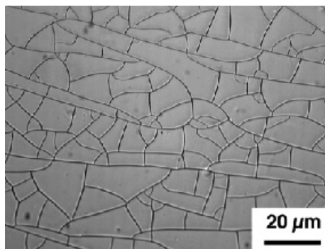
Figure 6.6 Biaxial tensile failure of a 100 nm thick ITO coating on polymer substrate
