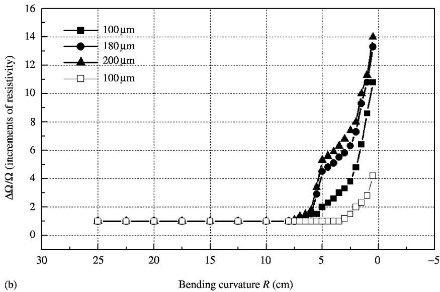
Figure 7.4 Dependence of electrical resistivity in ITO films (a) on the bending curvature and buffer material, and (b) on bending curvature and substrate thickness. In (a) the substrate is 100 \mu\text{m} polycarbonate and the ITO film has t = 0.1 \mu\text{m} . In (b) the organic buffer layer t = 0.1 \mu\text{m} and E_b = 2.1 \text{ GPa} and the ITO film has t = 0.1 \mu\text{m} ; the values in the key are substrate thicknesses
