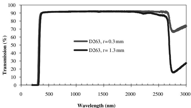
Figure 3.1 Transmission of D263 in the visible and near-IR spectrum
