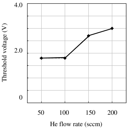
Figure 22.2 Threshold voltages of the a-Si:H TFTs fabricated on glass with the SiN x deposited at different He dilution
