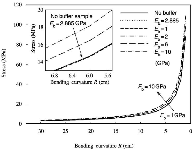
Figure 7.3 Effect of a buffer layer on the stress of mechanically deformed ITO–polymer substrate systems with respect to Young's modulus of the buffer layer. The data in this figure were calculated from (7.14) by considering the ITO films on PC substrate with t_s = 100\ \mu\text{m} , t_b = 0.5\ \mu\text{m} , t_f = 0.1\ \mu\text{m} and E_s = 5.3\ \text{GPa} . The inset figure shows the stress with bending curvature range from 6.9 cm to 5.6 cm
