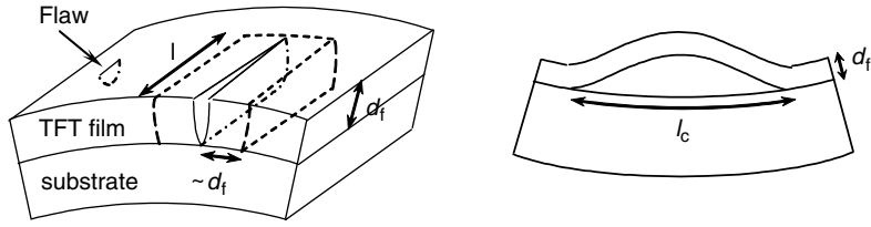
Figure 14.8 Failure mechanisms of a-Si TFT layers in (a) tension and (b) compression (Suo et al. 1999)
