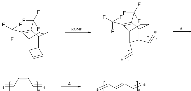
Scheme 8.11 Synthesis of polyacetylene via the polymer precursor/Durham route (Edwards and Feast 1980)
