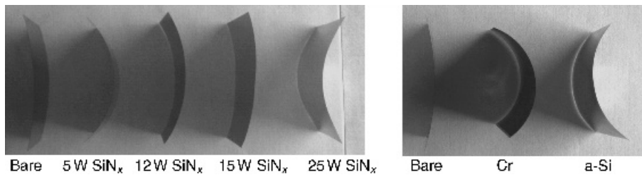
Figure 14.14 Stress-induced curvatures of (a) SiN x films deposited at various deposition powers and (b) Cr and a-Si films, all on 51 μm thick Kapton E polyimide substrates. The 300–500 nm thick SiN x and the 250 nm a-Si films were deposited at 150 °C; the thermally evaporated Cr film is 80 nm thick. The built-in stress in the SiN x film can be adjusted by deposition power. The built-in stresses of Cr and a-Si:H films are tensile and compressive, respectively. The films are on the left-hand side of the substrates (Cheng 2004)
