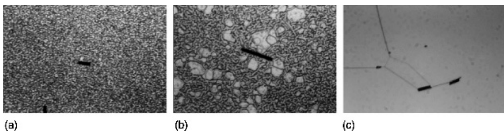
Figure 17.3 Microscope texture photographs of the planar texture with differently prepared substrates to create different domain sizes (the spacer in each photo is 5 \mu\text{m} wide): (a) small domains, less than 5 \mu\text{m} in diameter; (b) mixture of domain sizes from \sim 5 to 50 \mu\text{m} ; (c) large domains \sim 100 \mu\text{m} and larger. Reproduced by the permission of the Society for Information Display
