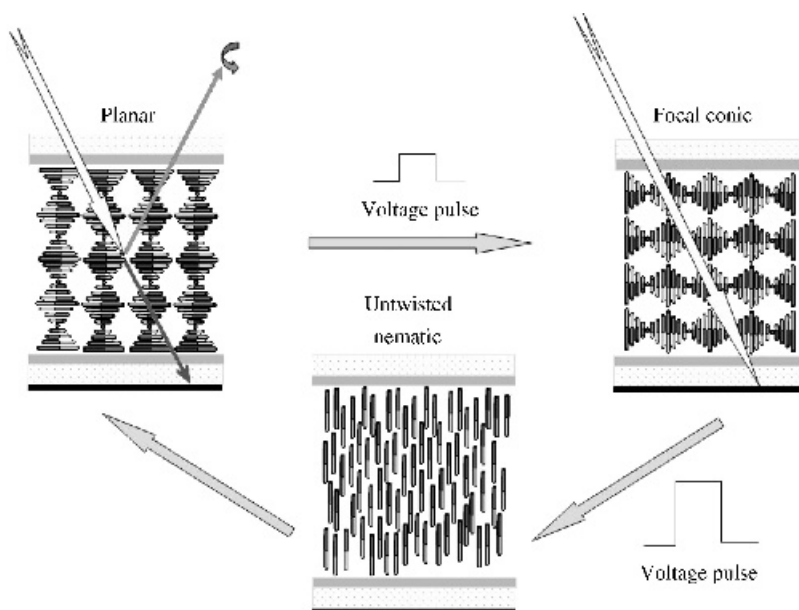
Figure 17.2 Textures of a bistable cholesteric material in a display cell. A small voltage pulse drives the material to a stable transparent focal conic texture whereas a large voltage pulse drives the material through an unstable homeotropic texture to a stable color-reflecting planar texture
