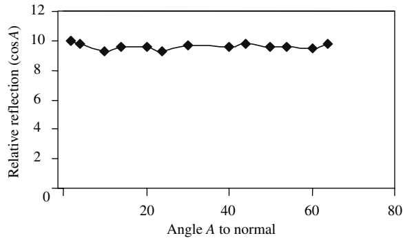
Figure 20.7 The ratio of diffuse angular reflection to the cosine of the angle is nearly a straight line, indicating Lambertian (or paper-like) scattering
