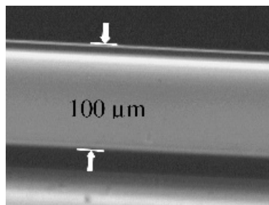
Figure 3.16 Edge quality of improved cutting equipment (using a diamond)
