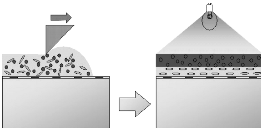
Figure 18.1 Schematic representation of the stratification process. The separation of a coated film into two discrete layers as the result of a photopolymerization-induced phase separation in the vertical direction. The formed LC layer at the bottom can be switched, by in-plane electrical fields, for example. On top of the polymer cover, the other necessary optical layers (e.g. polarizer, reflector) can be stacked
