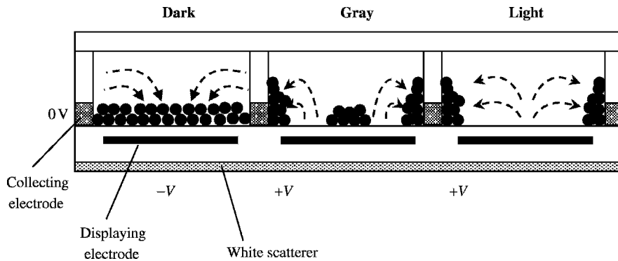
Figure 19.15 Cross section of one of Canon's in-plane electrophoretic films. Pixels are separated by vertical supports, and a collecting electrode is built into the supports and held at zero volts. A display electrode under every pixel drives the black pigment over the display surface to achieve a dark state or toward the collecting electrode to expose the white scatterer below. The left-hand pixel is driven dark, the middle pixel to a midtone, and the right-hand pixel to white reproduced by the permission of the Society for Information Display
