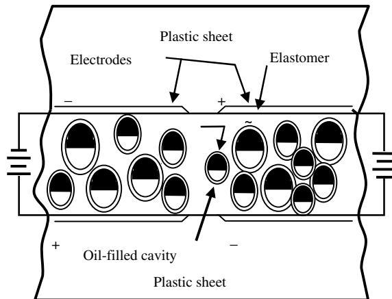
Figure 20.1 The Gyricon display consists of spherical beads, with optically contrasting hemispheres, dispersed in a transparent rubber sheet. A spherical cavity around each bead is filled with oil
