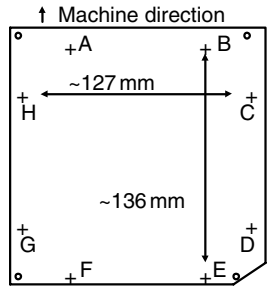
Figure 15.6 Eight-point measurement to assess dimensional change of a 6 in substrate
