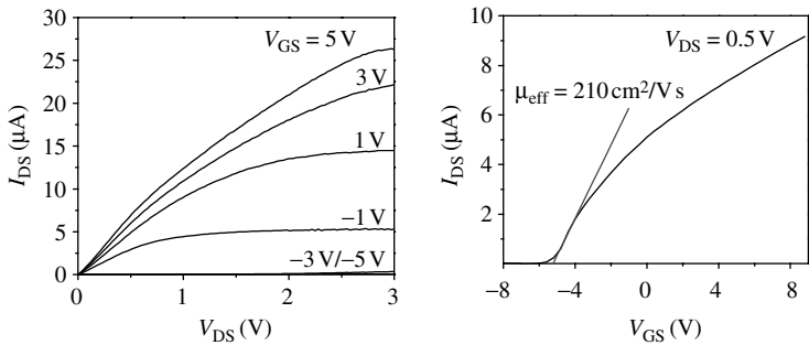
Figure 11.19 Electrical properties of a TFT that uses a single silicon ribbon solution cast onto a substrate of \text{SiO}_2/\text{Si}
