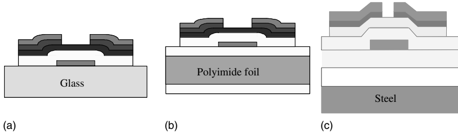
Figure 14.2 Schematic cross sections of back channel cut a-Si TFTs on (a) glass (Gleskova et al. 1996), (b) polyimide passivated on both sides with silicon nitride (Gleskova et al. 1998), (c) steel planarized with spin-on glass and then passivated with silicon nitride (Ma et al. 1997)
