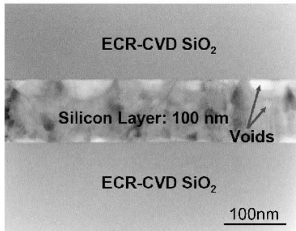
Figure 24.7 Cross-sectional TEM image of the sacrificial silicon layer after laser irradiation
