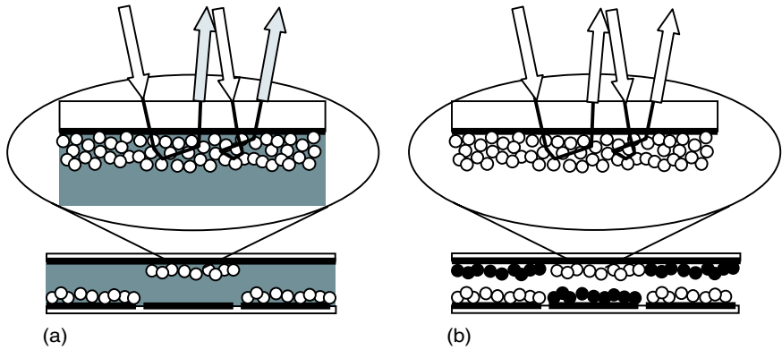
Figure 19.8 Light reflectance of (a) particle-dye and (b) dual-particle electrophoretic films in the white state. Interstitial dye in the particle-dye formulation taints the reflected light
