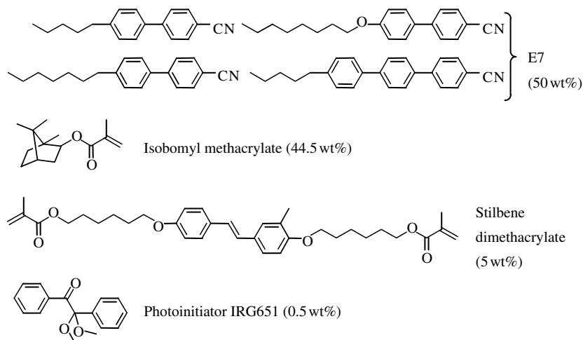
Figure 18.2 The structures of the liquid crystal blend E7 and the reactive monomers isobornyl methacrylate and stilbene dimethacrylate, as well as the photoinitiator Irgacure 651. The relative amounts of the compounds in the coating mixture are shown in parentheses
