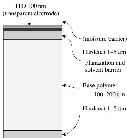
Figure 6.1 Generic substrate structure
