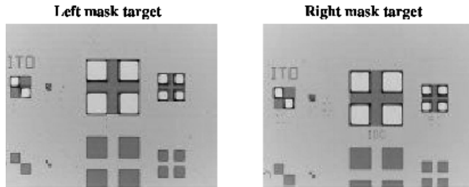
Figure 15.8 Alignment of metal layer achieved with compensation artwork
