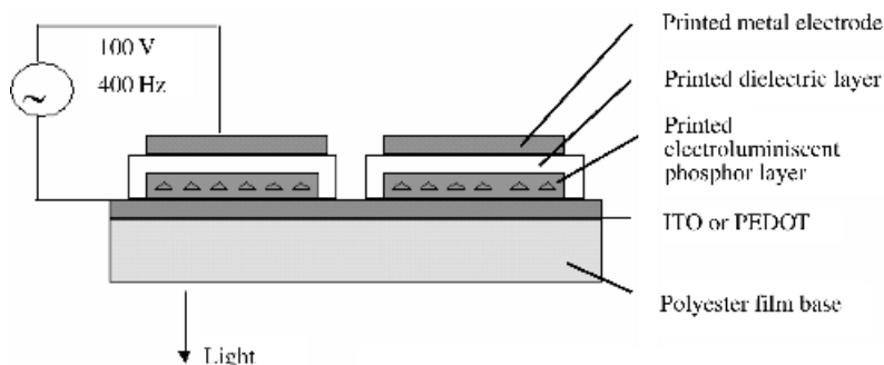
Figure 8.9 PEDT/PSS as electrode material in electroluminescent lamps: surface resistance = 60–2500 \Omega/\text{sq} and transparency = 85%
