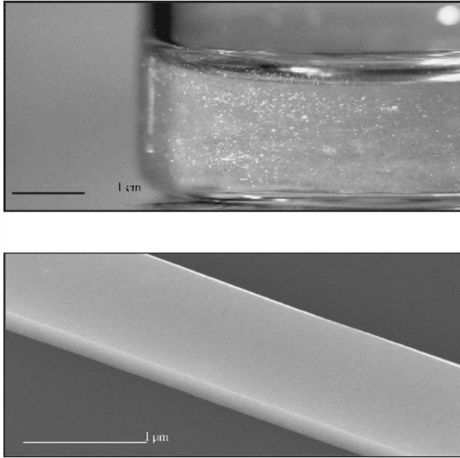
Figure 11.17 High-resolution images of transferred silicon wires and ribbons
