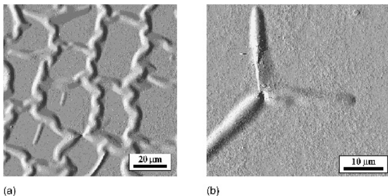
Figure 6.13 AFM images of buckling patterns: (a) biaxially loaded layer (b) initiation point
