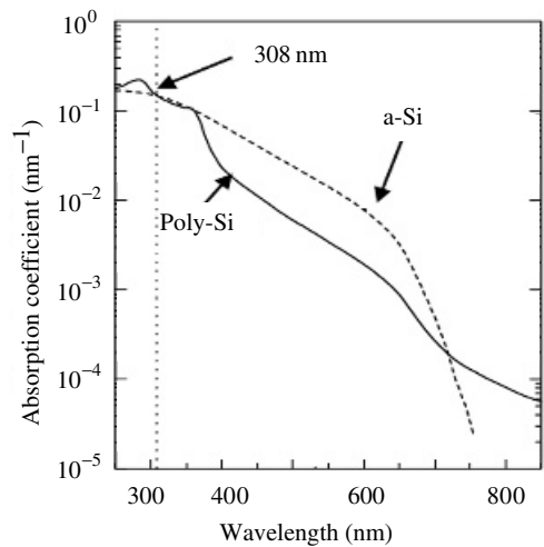
Figure 24.3 Light absorption coefficients of silicon films as a function of wavelength for the incident light
