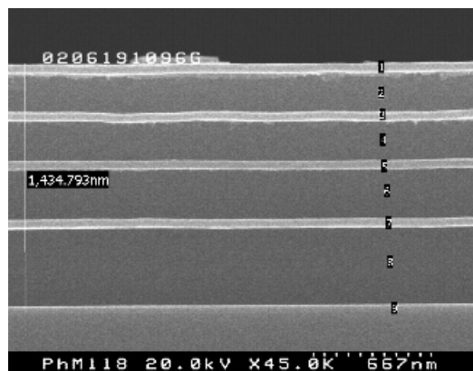
Figure 4.1 SEM cross section of a typical multilayer organic/inorganic barrier stack
