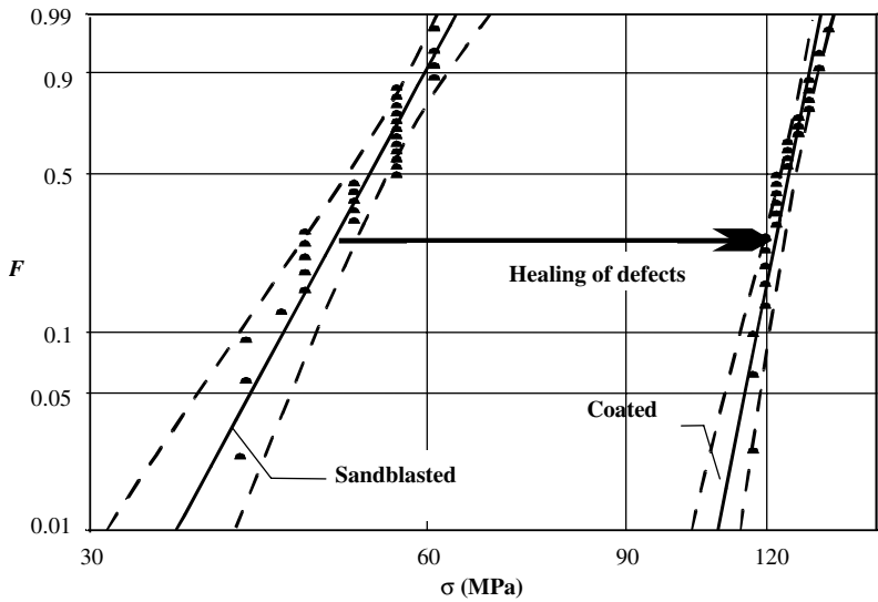
Figure 3.14 Improved surface strength of damaged (sandblasted) glass surface by coating
