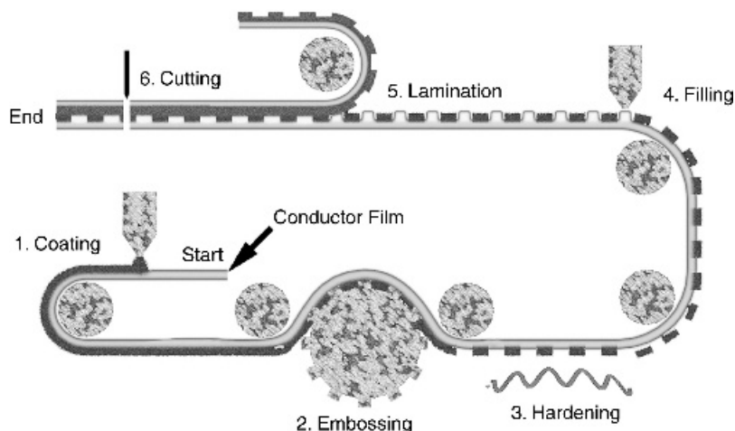
Figure 16.10 Schematic diagrams of roll-to-roll processing for Microcup LCD manufacturing where a polymer template is made through embossing and subsequently hardened before liquid crystal filling. Adapted from Liang and Tseng (2000)
