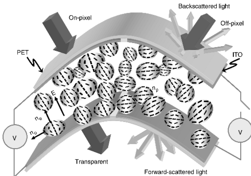
Figure 16.2 Operation of the PDLC in the transparent state (left pixel) and in the scattering state (right pixel). In the transparent state, a voltage is applied to the pixel, thereby aligning the liquid crystal within the droplet and creating an index matching condition where n_o matches n_p . In the scattering state, the symmetry axes of the droplets are randomly oriented, creating an index mismatch between droplets and the encapsulating matrix. Reproduced by the permission of the Society for Information Display
