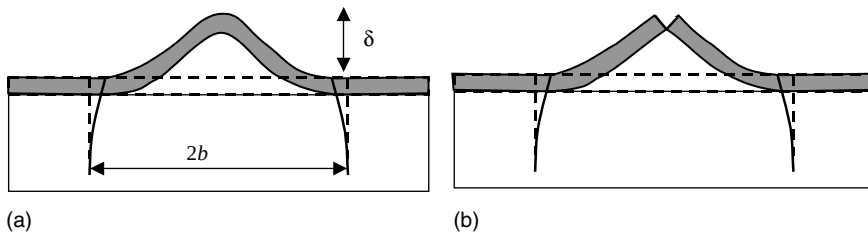
Figure 6.15 Schematic cross section of buckling patterns
