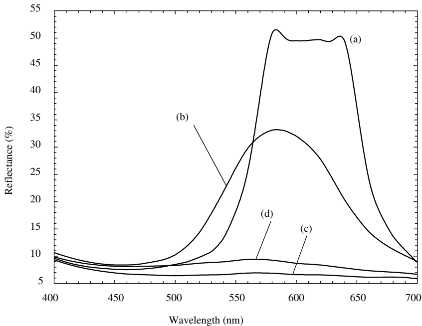
Figure 17.4 Reflection spectra for (a) large domain, near perfect planar texture such as in Figure 17. 2(c); (b) small, high-density domain texture such as in Figure 17.2(a); (c, d), focal conic states for large and small domains, respectively
