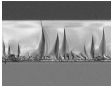
Figure 3.15 Edge quality of standard cutting equipment (using a diamond wheel)
