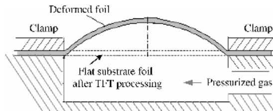
Figure 14.9 Apparatus for shaping a flat TFT backplane to a dome (Hsu et al. 2002b)
