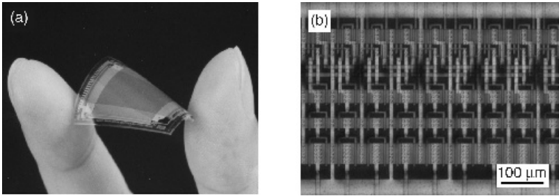
Figure 24.12 (a) The appearance and (b) the micrograph of the TFT LCD circuit transferred onto the plastic film
