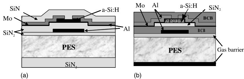
Figure 22.5 (a) A cross-sectional view of an a-Si:H TFT with SiN x gate insulator and (b) an a-Si:H TFT with SiN x /BCB gate insulator
