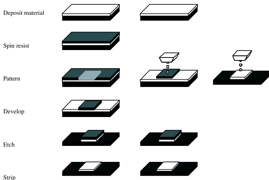
Figure 12.15 Advantages of printing organic electronics. The first column depicts a typical lithographic process. Subject material is deposited on the substrate. Photoresist is applied, exposed, and developed. The subject material is etched and the photoresist is stripped. The second column depicts a subtractive printing process. Subject material is deposited on the substrate. A mask is printed and the subject material is etched. The resist is then stripped. The third column depicts an additive printing process in which an ink carrying the subject material is printed only where necessary.
