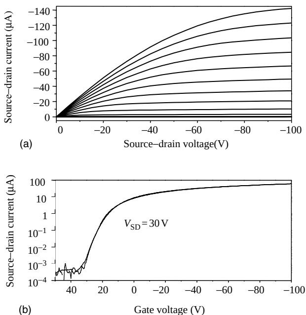
Figure 11.15 Current–voltage characteristics of a field effect transistor that uses a single crystal of the organic semiconductor rubrene. (a) Variation of current with source–drain voltage at several gate voltages. Typical p-type behavior is observed, with well-resolved linear and saturation current regimes. The channel is normally off and turns on at successively more negative gate voltage (from +20 to –100 V). (b) Transfer characteristics measured at V_{SD} = 30 \text{ V} . On/off ratios are of order 10^5 and mobilities are as high as 20 \text{ cm}^2/\text{V s} .
