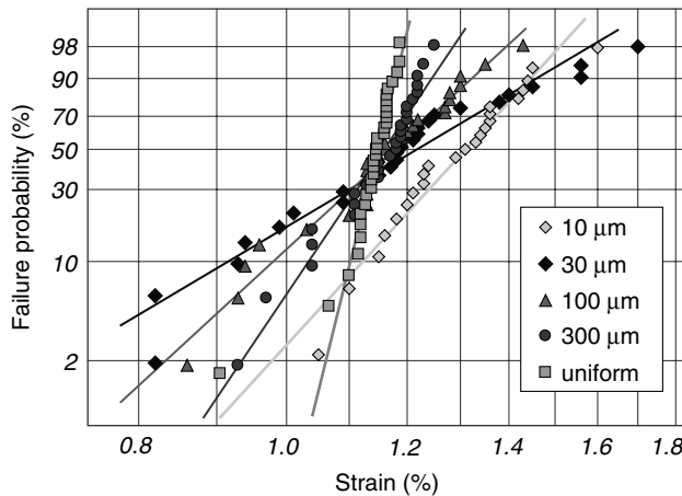
Figure 6.10 Weibull plot showing failure strain of ITO lines of different width
