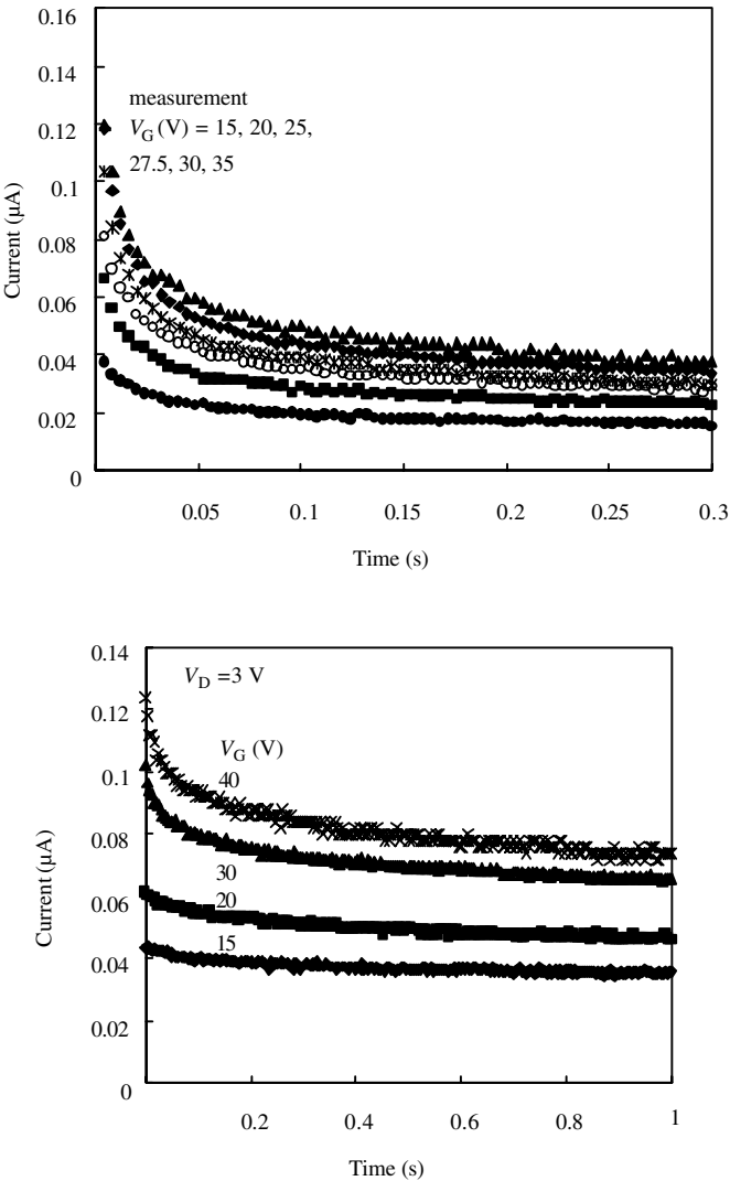
Figure 12.5 Bias stress in two polymer TFTs. Transistors are held with V_G = 0 V and constant V_D until stabilized. V_G is then raised quickly while I_D is monitored. Two semiconductors are compared: (a) F8T2 and (b) PQT (b). Reproduced by permission of the American Physical Society
