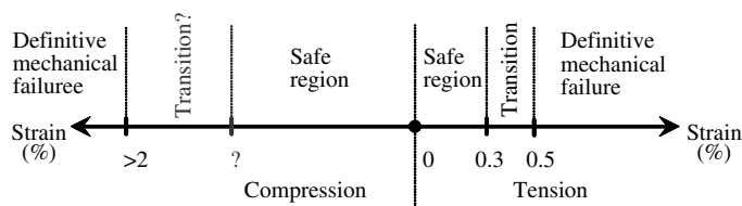
Figure 14.6 Summary of the response of a-Si TFTs to mechanical strain
