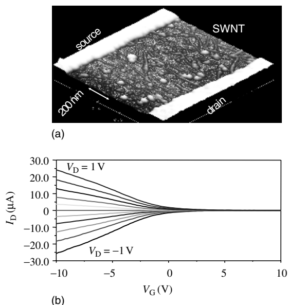
Figure 11.16 (a) An atomic force micrograph of the channel region of a thin film transistor that uses an array of SWNTs as the semiconductor. (b) Transfer characteristics of such a device
