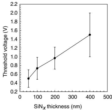
Figure 22.10 Threshold voltage of the a-Si:H TFTs on PES as a function of SiN x thickness
