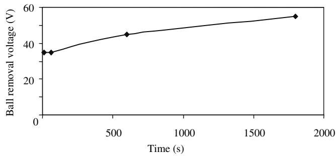
Figure 20.6 The threshold voltage for removal of a bichromal bead from wall adhesion increases with residence time on the wall
