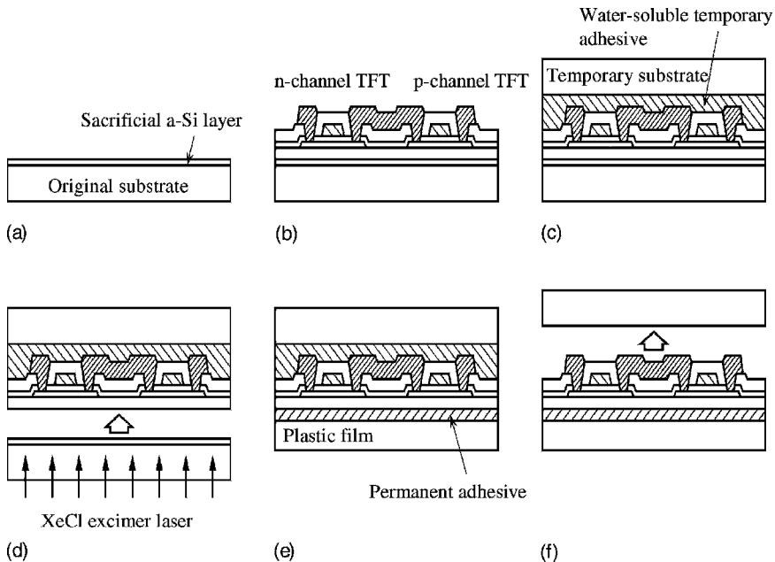
Figure 24.2 Schematic diagram of the TFT transfer process sequence
