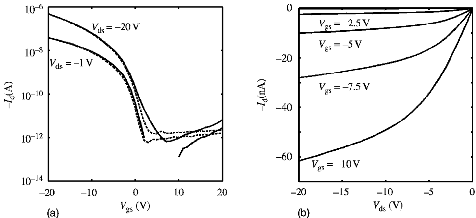
Figure 13.7 Characteristics of a pixel TFT with typical mobility 0.01 \text{ cm}^2/\text{V s} : (a) transfer characteristics and (b) output characteristics
