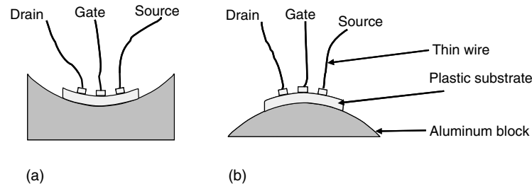
Figure 23.7 Sample configurations for measuring TFT characteristics with substrate bending: (a) compressive and (b) tensile
