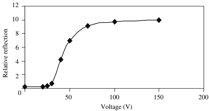
Figure 20.4 Diffuse reflection of light from the Gyricon as a function of an applied electrical voltage
