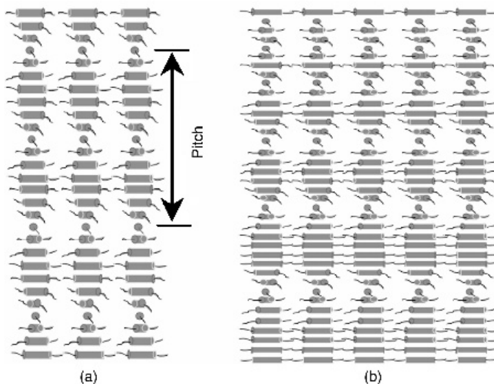
Figure 10.2 Schematic diagram of a chiral nematic liquid crystal. (a) A conventional chiral material; the pitch is defined as the length corresponding to one complete 360^\circ rotation of the director. (b) A chiral material with a pitch gradient. Image courtesy of D. Broer, Philips
