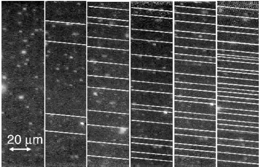
Figure 9.1 Optical micrographs showing the evolution of cracking of the ITO layer in tension. Strain increases from 2% to 3.3% from left to right
