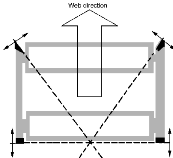
Figure 21.15 Steering guide systems
