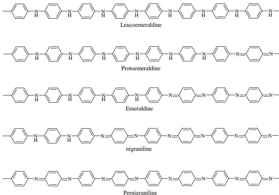
Figure 8.7 Different forms of polyaniline
