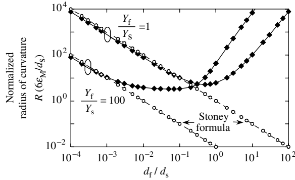
Figure 14.4 Normalized radius of curvature as a function of film/substrate thickness ratio. Two different substrate types are illustrated: glass or steel ( Y_f/Y_s \cong 1 ) and organic polymer ( Y_f/Y_s \cong 100 ). We assume that \nu_f = \nu_s . Full lines represent the exact solution of (14.7); dashed lines represent the approximation (14.4) for a thick, stiff substrate (Gleskova et al. 1998)
