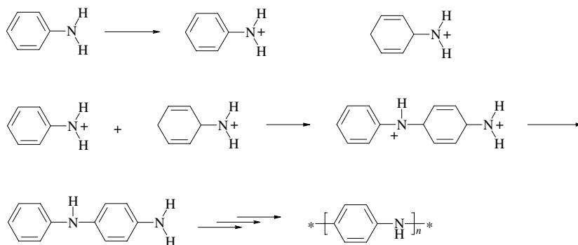
Scheme 8.12 Mechanism of electrochemical polymerization of aniline to polyaniline
