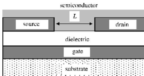
Figure 11.1 Schematic cross-sectional view of an organic thin film transistor. A semiconductor layer coats source and drain electrodes that are electrically isolated from a gate electrode by a dielectric layer. The separation between the electrodes defines the channel length, L
