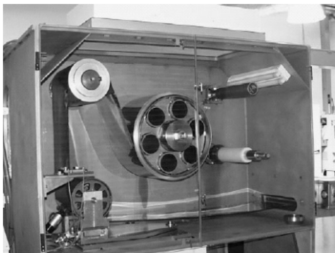
Figure 21.13 Minienvironment web payoff station for a roll-to-roll aqueous washer
