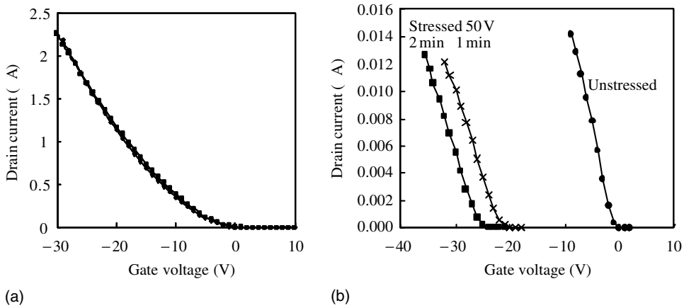
Figure 12.6 Bias stress in two polymer TFTs. Device transfer characteristics are measured (a) twice in succession for PQT and (b) three times under bias for F8T2
