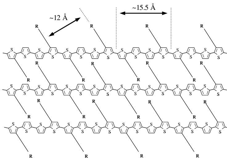
Figure 12.12 Schematic representation of lamellar structural order of PQT-3
