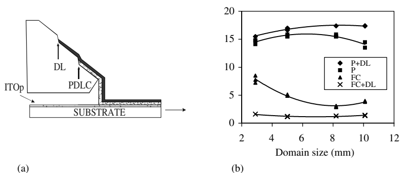
Figure 17.12 (Left) Diagram of the Kodak photographic coating process for laying down multiple coats with a dark coat, DL, coated on top of the cholesteric droplet dispersion. (Right) Droplet size versus reflectance for Kodak emulsion coatings with and without the dark layer overcoat. Reproduced by the permission of the Society for Information Display
