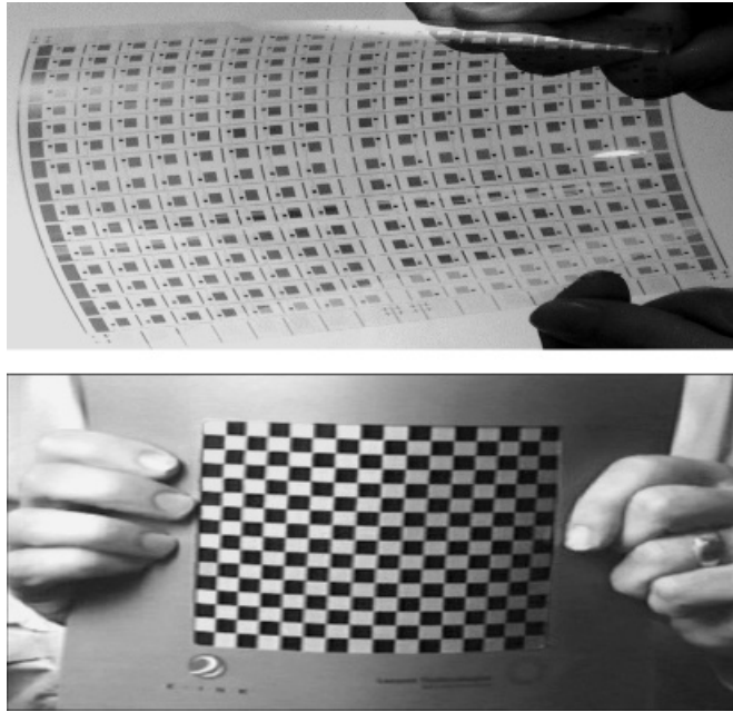
Figure 11.20 Mechanically flexible plastic active matrix circuit (top image) for an electronic paper-like display (bottom image). Microcontact printing defined the critical features in the organic transistors of this circuit
