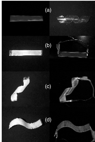
Figure 16.5 Actual conformed PDLC samples in the off (left) and on (right) states: (a) an ITO/PET substrate, (b) a control PDLC (nonconformed), (c, d) a spiral and wavy conformed PDLC sample. Reproduced by the permission of the Society for Information Display
