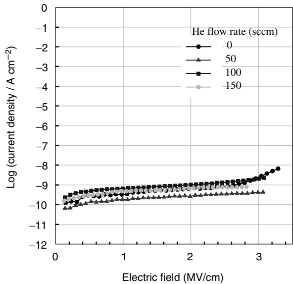
Figure 22.1 I – V characteristics of the SiN x films deposited at 150 °C with different He flow rates
