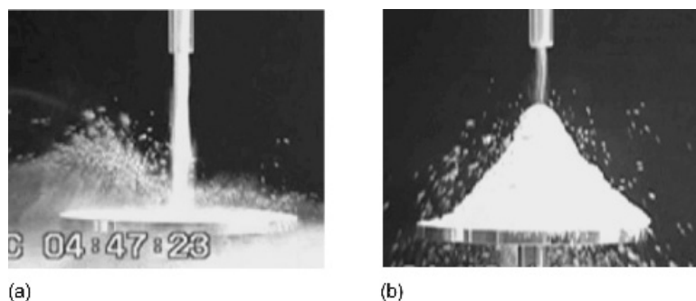
Figure 19.13 (a) Liquid powder made by Bridgestone and (b) an ordinary powder poured onto a platform. The liquid powder does not form a pile in this experiment, and an ordinary powder does. Reproduced with permission of the Society for Information Display
