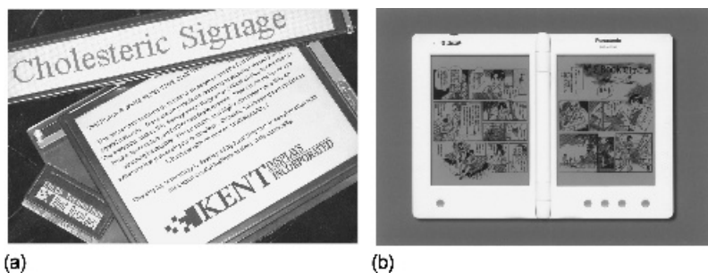
Figure 17.1 (a) Various reflective cholesteric display products on rigid glass substrates: wide 12.1 in sign-type display (blue/white), large 9.4 in ebook-type display (black/white) and small 2.3 in instrumentation-type display (green/black) of Kent Displays, Inc. (b) The electronic book Sigma Book by Matsushita/Panasonic with two cholesteric reflective displays. Part (b) reproduced by the permission of Panasonic
