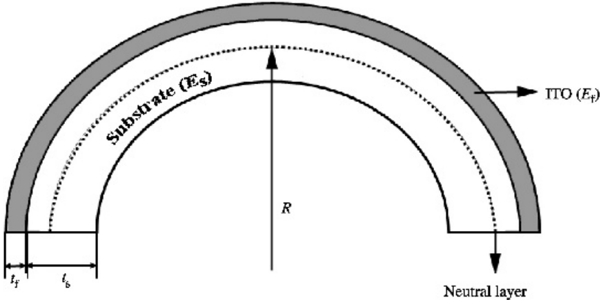
Figure 7.1 A cross-sectional view of a double-layer sturcture in bending state
