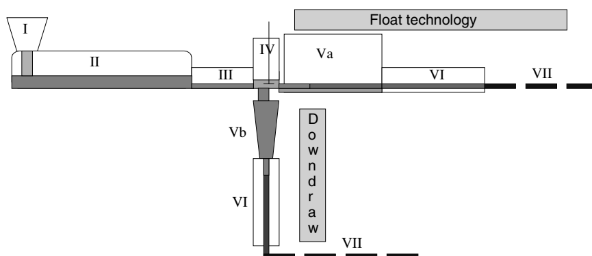
Figure 3.5 Basic process steps of modern glass production: I = mixing raw materials, II = melting, III = refining, IV = homogenization, Va = float technology, Vb = downdraw (DD) technology, VI = annealing, VII = cutting
