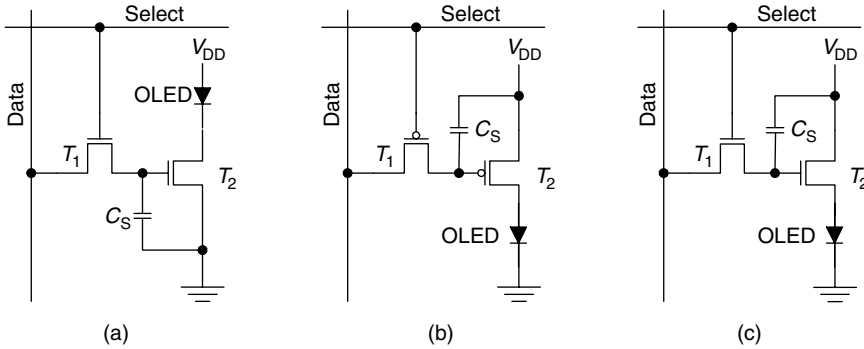
Figure 15.9 Basic 2-TFT circuits for AMOLED: (a) n-channel and (b) p-channel circuits with OLED on the drain side of the TFT; (c) n-channel TFT with OLED on the source side of the TFT, but with the TFT in contact with the OLED anode instead of the OLED cathode as in (a)
