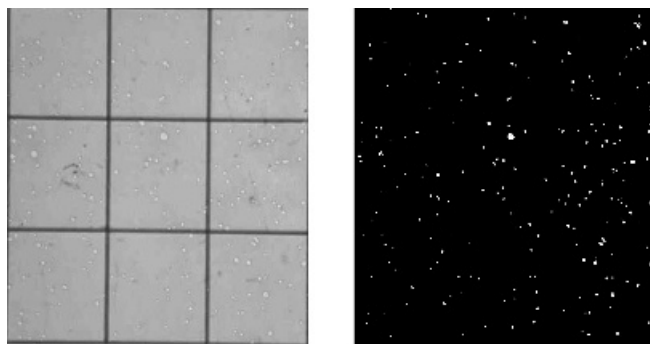
Figure 4.2 Optical micrograph (left) of Ca deposited on a five-dyad PET/barrier substrate after 1632 h of atmospheric exposure. Image analysis (right) of optical view after converting grayscale to pure black and white. White regions are reacted Ca. Total image area = 2.25 mm 2
