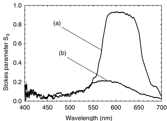
Figure 17.6 S_3 as a function of wavelength for (a) the large domain structure of Figure 17.3(c) and (b) the small, high-density domain structure of Figure 17.3(a). Reproduced by the permission of the Society for Information Display
