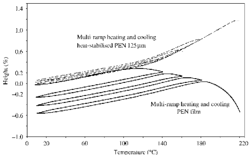
Figure 2.3 Thermomechanical analysis of 125 \mu\text{m} PEN and heat-stabilised 125 \mu\text{m} polyethylene naphthalate films
