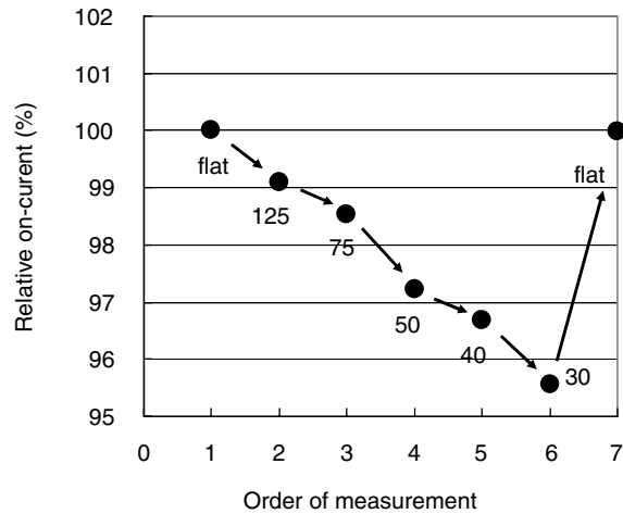
Figure 23.9 The change in on-current with substrate bending for a p-channel TFT. The radius of curvature (mm) is shown
