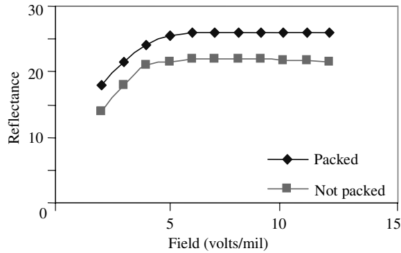
Figure 20.10 A higher density of (packed) beads in the top layer increases the brightness of the Gyricon display
