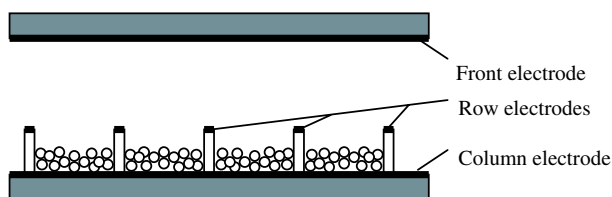
Figure 19.3 Control grid structure for driving electrophoretic films. The pigment is trapped in potential wells because of a voltage difference between the row electrode and column electrode
