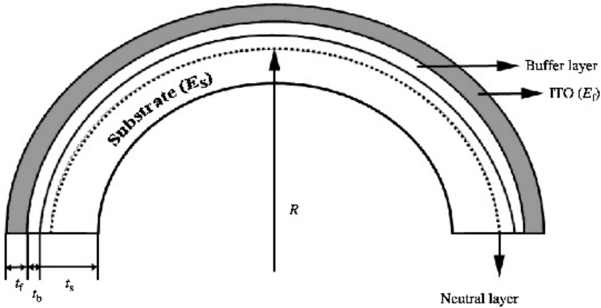
Figure 7.2 A cross-sectional view of a triple-layer structure with a buffer layer
