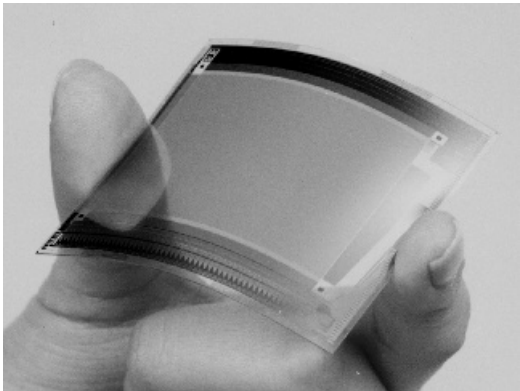
Figure 24.18 Appearance of the TFT OLED display circuit transferred onto the plastic film
