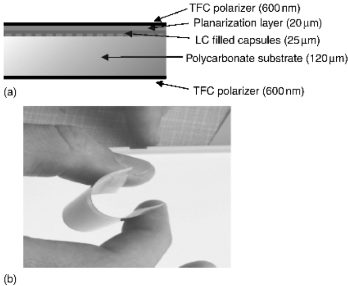
Figure 18.10 (a) Schematic representation of a stack of layers including coatable TCF polarizers. (b) Photograph of a paintable LCD bent to a curvature radius of less than 1 cm. The total thickness of this ultra-thin and flexible LCD is less than 170 μm
