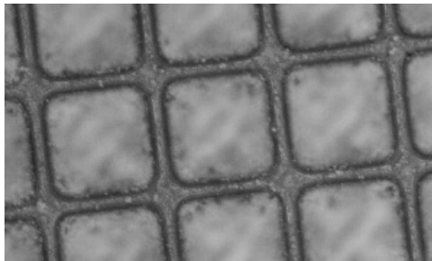
Figure 19.12 A Microcup electrophoretic film constructed with an embossed rib pattern and cells filled with an electrophoretic fluid, then sealed with an overcoat. Courtesy of SiPix
