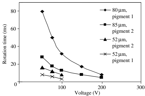
Figure 20.5 High bead rotation rates have been obtained with some experimental materials
