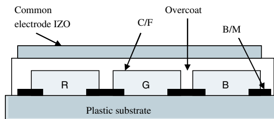
Figure 22.14 A cross-sectional view of a color filter on plastic
