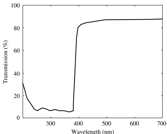
Figure 2.2 Percentage transmission of Teonex Q65
