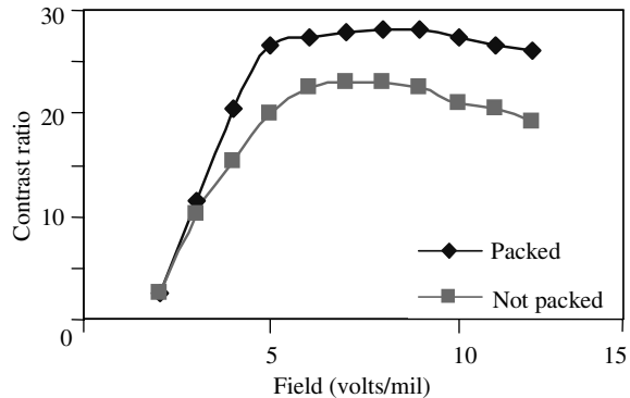
Figure 20.11 A higher density of beads packed into the first layer also improves the contrast
