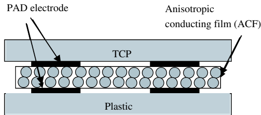
Figure 22.16 Connecting a TCP to a TFT array on plastic using an ACF
