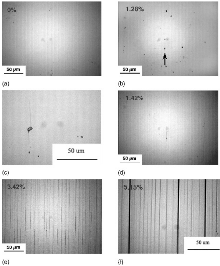
Figure 6.5 Progressive cracking of a 100 nm thick ITO coating on a hardcoated polyester substrate during tensile loading along the horizontal direction; strains are listed in the micrographs; (c) and (d) are at 1.42% strain. Parts (a), (b), (d) and (e) reprinted from “Mechanical Integrity of Transparent Conductive Oxide Films for flexible Polymer-Based Displays”, vol 460, Leterrier Y., Médico L., Demarco F., Månson J.-A. E., Bouten P., DeGoede J., Nisato G., Nairn J. A., “Thin Solid Films”, pp. 156–166 (2004) with permission from Elsevier. Parts (c) and (f) reproduced by the permission of SVC
