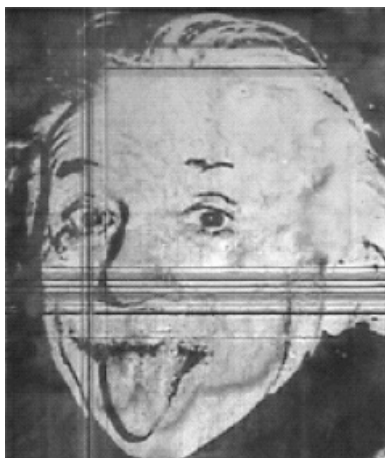
Figure 19.16 Active matrix, 260 ppi, 5.32 cm \times 5.32 cm grayscale display prototype using Canon's in-plane electrophoretic film. Reproduced with permission of the Society for Information Display
