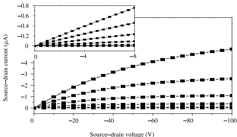
Figure 11.14 Current–voltage characteristics of an organic transistor that uses thermal transfer printed source and drain electrodes of PANI/SWNT. A thin (25 nm) film of pentacene deposited onto the electrodes provides the semiconductor. The gate voltage varies from 0 to -100 V in steps of -20 V. The channel length is 15\text{ }\mu\text{m} and the channel width is 0.5\text{ mm} . The inset shows the linear behavior of the device at small source–drain voltages. Reprinted with permission from American Chemical Society
