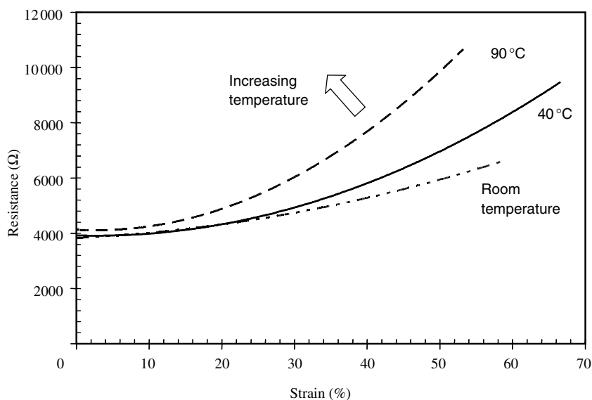
Figure 9.4 Resistance versus strain for PEDOT:PSS-coated PET deformed in uniaxial strain at room temperature, 40 °C, and 90 °C. The rate of increase of resistance with increasing strain increases with temperature
