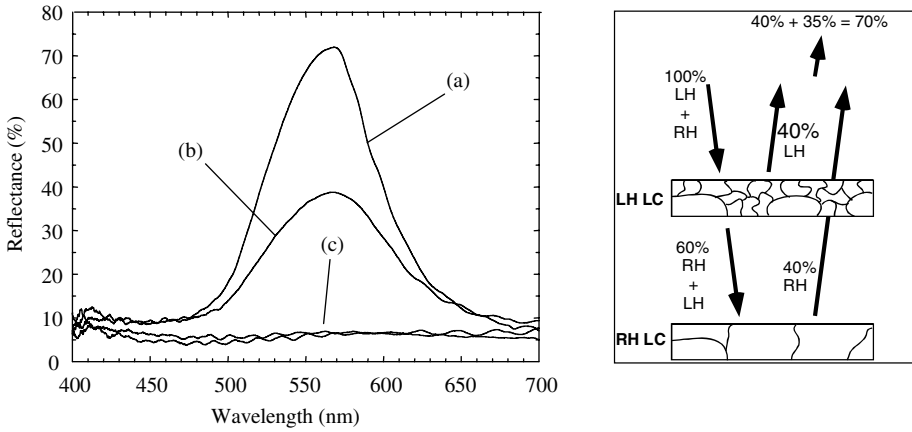
Figure 17.7 Comparison of reflectivity from a stacked display cell with layers of opposite twist. (a) High brightness is achieved when the layers possess large domains structures yielding high S_3 values, as illustrated on the right. (b) Both layers possess small domains which yield small S_3 values. (c) Reflectivity from the focal conic state of both stacked cells arrangements
