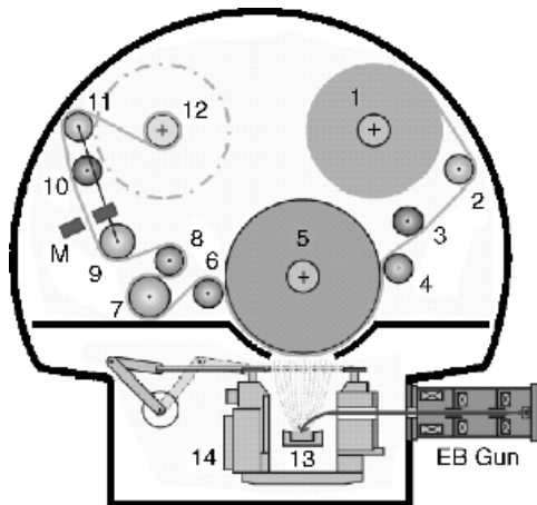
Figure 21.2 Tools for roll-to-roll processing: (1) unwinder, (2, 9, 11) guide rolls, (3, 10) spreader roller, (5) coating drum, (4, 6, 8) tension measurement roller, (6, 8) measurement roller, (7) tension isolation roller, (12) rewinder, (13) crucible, (14) magnetic trap, (M) optical measurement
