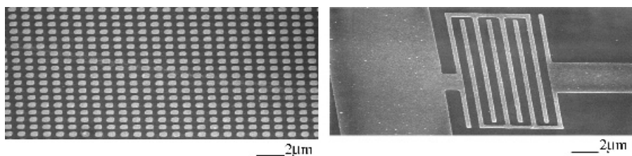
Figure 11.4 Scanning electron micrographs of structures formed by microcontact printing a self-assembled monolayer ink of hexadecanethiol onto a thin metal film of Au (left) and Ag (right) followed by wet etching of the unprinted areas. The left-hand image shows an array of Au (20 nm thick) dots with \sim 500\text{ nm} diameters. The right-hand image shows a printed structure of Ag (100 nm thick) in the geometry of interdigitated source and drain electrodes for a transistor in a simple inverter circuit. An edge resolution of \sim 100\text{ nm} can be achieved with this technique. Reproduced by permission of the American Institute of Physics
