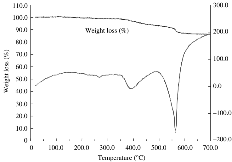
Figure 2.12 Thermogravimetric analysis of the coating used as a smoothing coat
