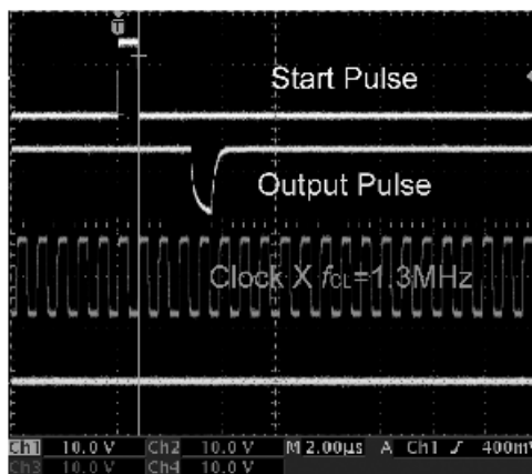
Figure 24.11 The operation of the 107-stage static shift register measured after transfer onto the PES film: (a) the circuit diagram and (b) the waveforms during operation
