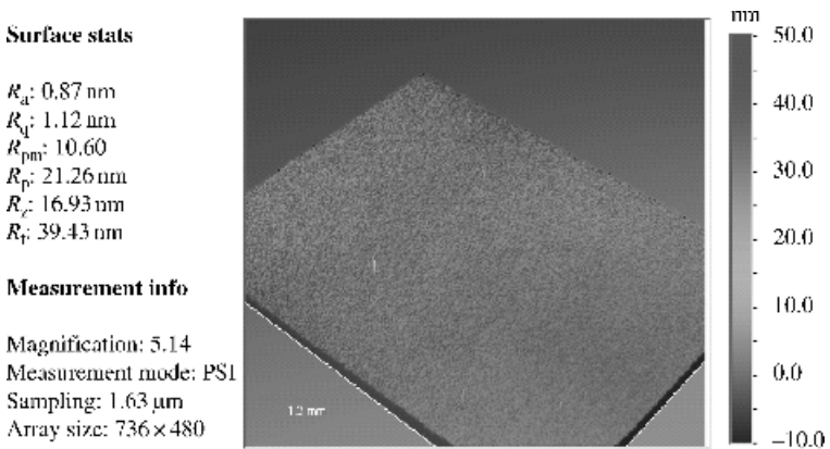
Figure 2.10 Surface smoothness of surface-engineered Teonex Q65
