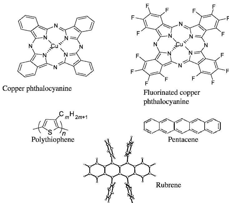
Figure 11.11 Chemical structures of some organic semiconductors. Thin films of these materials act as p-type materials in thin film transistors, except for the compound at the upper right, which exhibits n-type behavior
