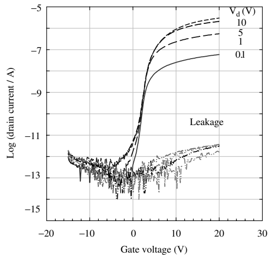
Figure 22.4 Transfer characteristics of the a-Si:H TFT where the SiN x was deposited at an He flow rate of 200 sccm (standard cubic centimeters per minute)
