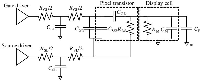
Figure 12.1 Equivalent circuit of a nonemissive active matrix display cell for an m \times n (gate lines \times source lines) array. The gate driver switches between two levels (on and off). The source driver may drive the source line to one of 256 or more levels. R_{GL} is the gate line resistance; C_{GL} is the gate line capacitance, which includes n gate and overlap capacitances distributed along its length. R_{SL} is the source line resistance; C_{SL} is the source line capacitance, which includes m gate–source and overlap capacitances distributed along its length. C_{XO} is the single-pixel overlap capacitance. The transistor is modeled by C_{GD} , the gate–drain capacitance; C_{GS} , the gate–source capacitance; and R_{DS} , the drain source resistance. The display cell is represented by a medium resistance, R_M , and a medium capacitance, C_M . Finally, any capacitance of the pixel to the adjacent gate driver is represented by C_P . (*) connects to the adjacent gate driver, represented as a virtual ground
