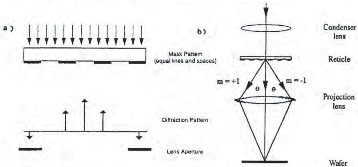
Fig. 7-9 Principle of on-axis illumination: a) Light illuminating the mask from an on-axis direction, and the diffraction pattern from an on-axis coherently illuminated grating mask. The pattern is centered on the entrance pupil of the objective lens. b) Aperture with on-axis illumination showing the 0-order (undiffracted beam) and the two first order diffracted beams, m = +1 and m = -1 .
