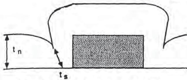
(a) Step Coverage (%) = (t_s / t_n) \times (100\%)
