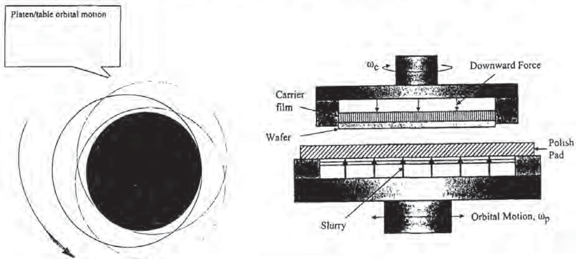
Fig. 8-37 Schematic drawing of orbital platen motion polisher.
