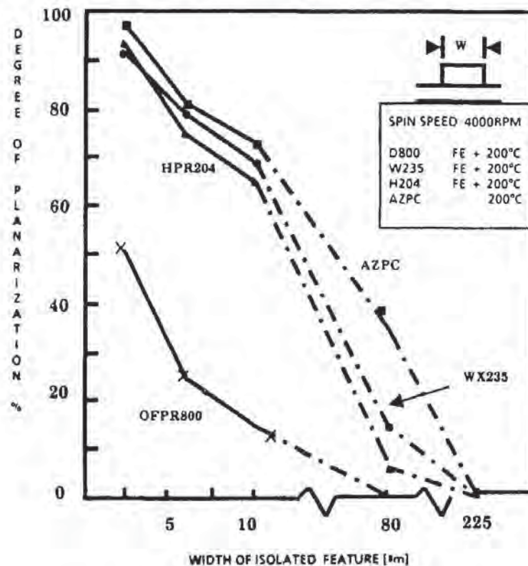
Fig. 8-6 Degree of planarization vs. various feature size for different polymers. 2 (© 1987 IEEE)
