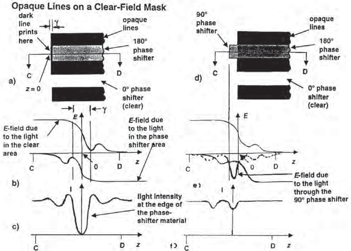
Fig. 7-19 Problem at the edge of a phase-shifter at a clear boundary: (a) ALT-PSM used on lines and spaces pattern with a clear field. Dark lines will print at the boundaries between the edge of the phase shifter and non-shifted clear areas; (b) E -fields along the z -axis between C and D for light incident on the phase shifter and clear area; (c) These two E -fields interfere in the vicinity of z = 0 , causing the intensity of the E -field there to drop, resulting in a dark line printed as shown in (a); (d) Adding an extension of phase shifting material (with \phi = 90^\circ ) at the end of the phase-shifting region (as shown in [d]), helps mitigate the problem; (e) The amplitude of the E -fields of the light for the three phase regions versus z ; (f) Intensity of light versus z when the \phi = 90^\circ extension is present. Note that the intensity drop-off is much smaller when interference occurs, and the dark line may no longer print.
