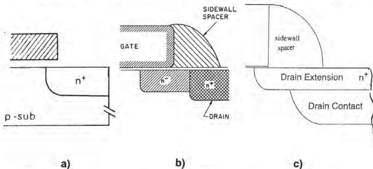
Fig. 1-6 a) Single-region drain in a MOSFET; b) Lightly-doped-drain in a MOSFET; c) Source/drain-extension and contact-drain-regions used in deep-submicron MOSFETs.
