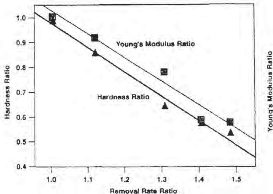
Fig. 8-22 A linear relationship exists between the CMP-removal-rate and the hardness and elastic modulus of F- SiO_2 . Removal-rate, hardness, and elastic modulus are all normalized with respect to those parameters of undoped TEOS-oxides. 18
