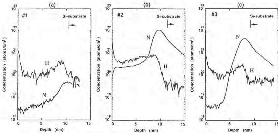
Fig. 3-28 SIMS depth profiles of N and H in three kinds of oxide films: (a) pure SiO 2 (#1); (b) NH 3 -nitrided SiO 2 (#2); and (c) N 2 O-nitrided SiO 2 (#3).
