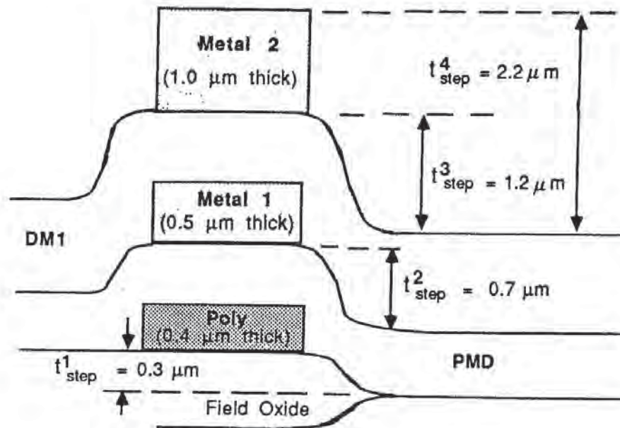
Fig. 8-2 As the number of levels in an interconnect technology is increased, the stacking of additional layers on top of one another produces steps of progressively greater heights.
