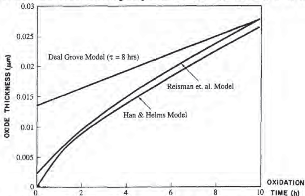
Fig. 3-24 Comparison of three oxidation models for 1 atmos, dry- \text{O}_2 oxidation at 800^\circ\text{C} .
