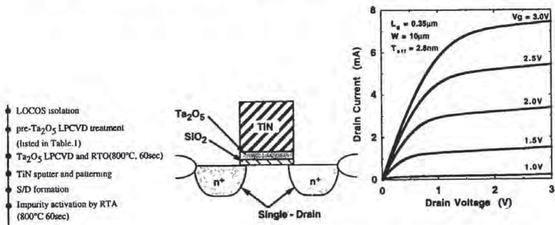
Fig. 4-10 Process flow, cross section, and I-V characteristics of an NMOSFET fabricated with a with a Ta 2 O 5 /SiO 2 gate dielectric. A TiN gate electrode was also employed. 21
