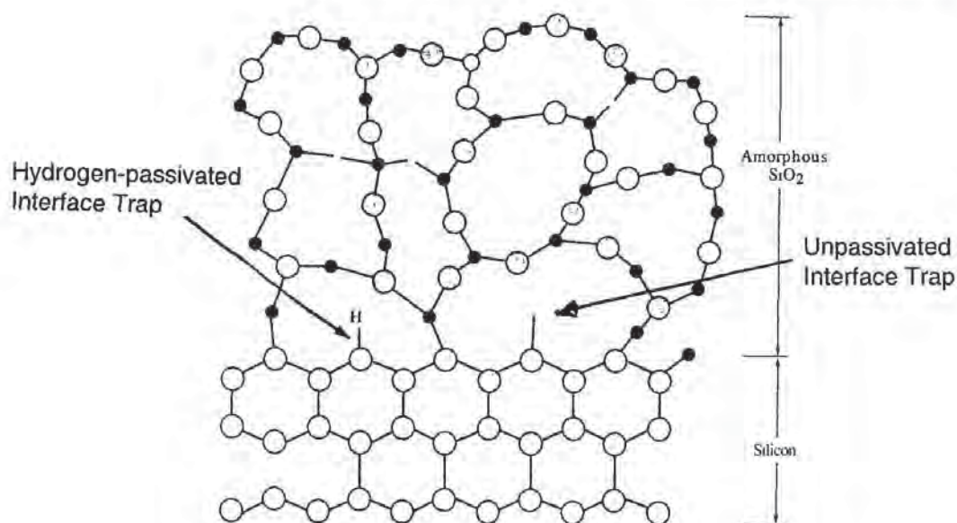
Fig. 3-8 How hydrogen can passivate the dangling bonds at the silicon surface shown in Fig. 3-7c and reduce the interface trap density.
