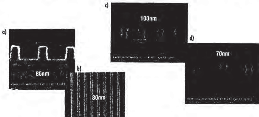
Fig. 6-12 Using 157-nm exposures, phase-shift masks, and 148-nm thick resist on a 70-nm AR layer, various resist recipes resolve at linewidths of: a) and b) 80 nm; c) 100 nm; and d) 70 nm.
