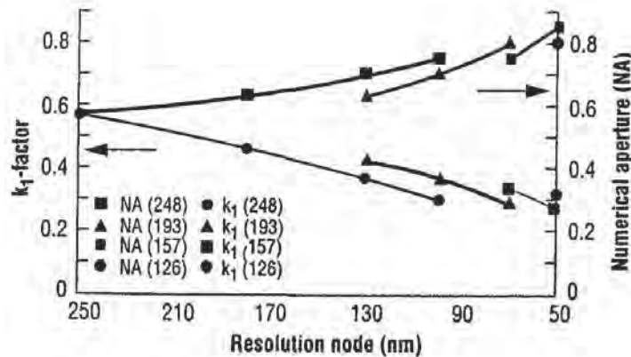
Fig. 7-26 Wavelength, NA, and k_1 for 250 nm to 50 nm resolution nodes. (Courtesy ASML)
