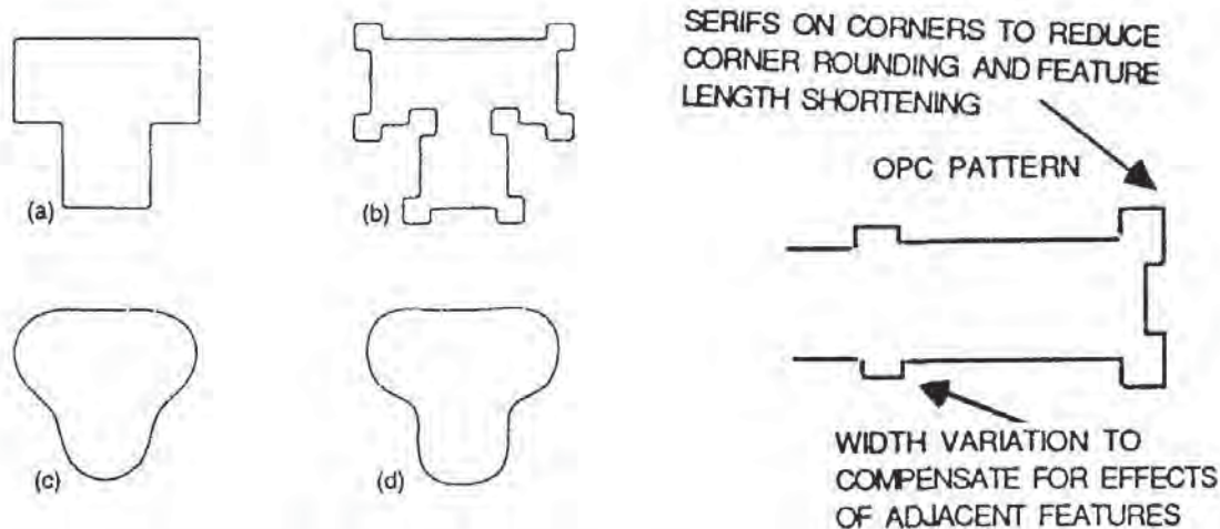
Fig. 7-14 A T-shaped feature (a) with dimensions near the resolution limit of the projection lens is printed as a rather featureless blob (c) on the wafer. Addition of serifs (b) brings the printed image (d) closer to the shape originally designed. Reprinted by permission of Marcel Dekker. (e) Adjustments to the linewidth can correct for the proximity of nearby features, and serifs on the end of a line can correct line shortening effects.
