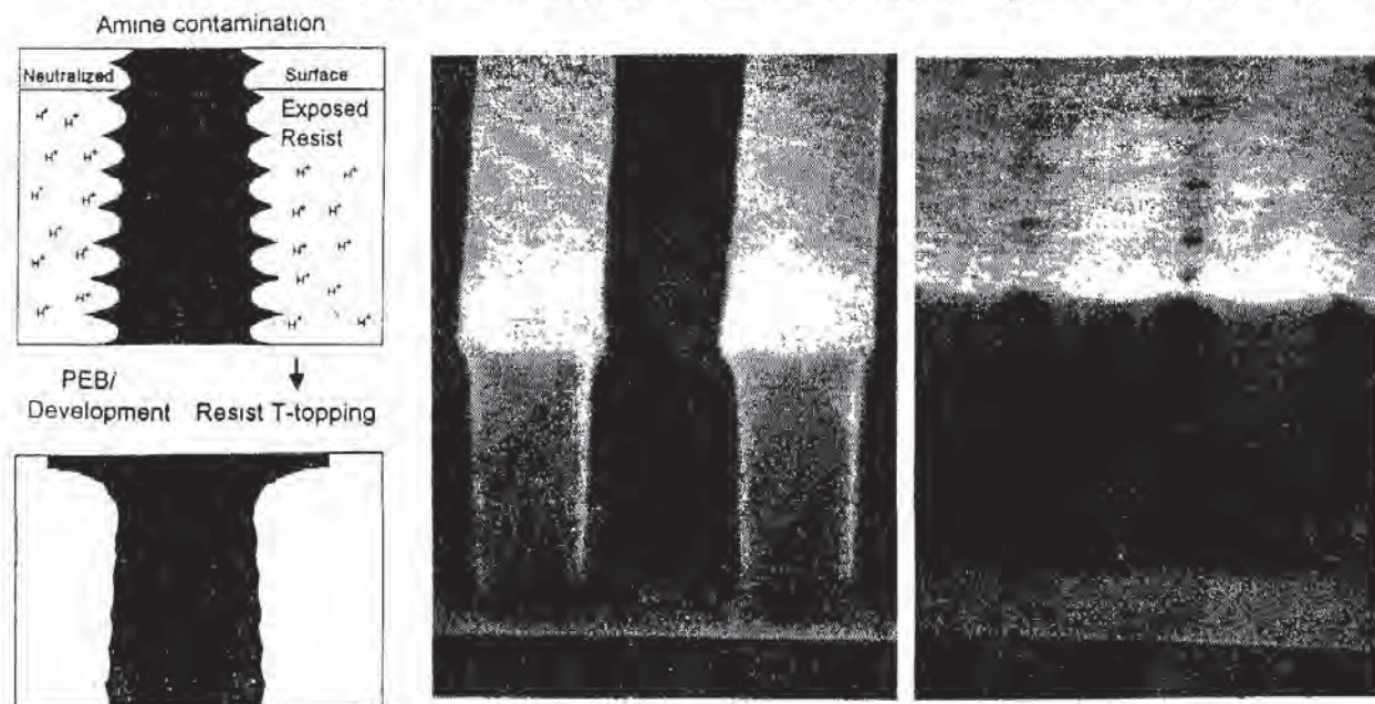
Fig. 6-2 (a) Environmental amine contamination of a chemically amplified resist, resulting in “T-top” formation after development.
