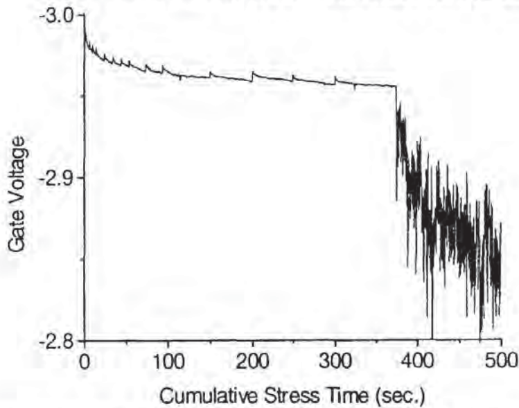
Fig. 3-42 Gate voltage measured during sequential -10 \text{ mA/cm}^2 constant-current stresses of a 2.0-nm gate oxide. Soft breakdown occurs after about 360 seconds. Spikes are visible in the pre-breakdown trace because the stress was removed periodically. 90
