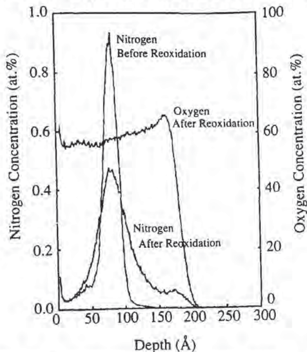
Fig. 3-33 SIMS profile of the oxynitride film grown from 100% \text{N}_2\text{O} at 1100°C before reoxidation, and after 85 min reoxidation. 59 By permission of the Electrochemical Society.
