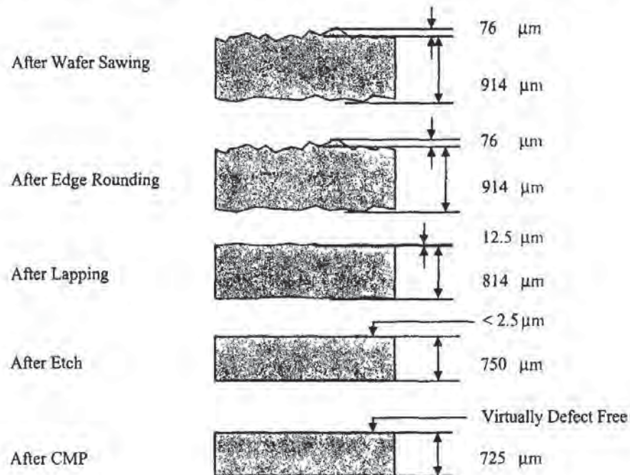
Fig. 2-28 Wafer thickness and surface roughness changes during grinding and polishing.
