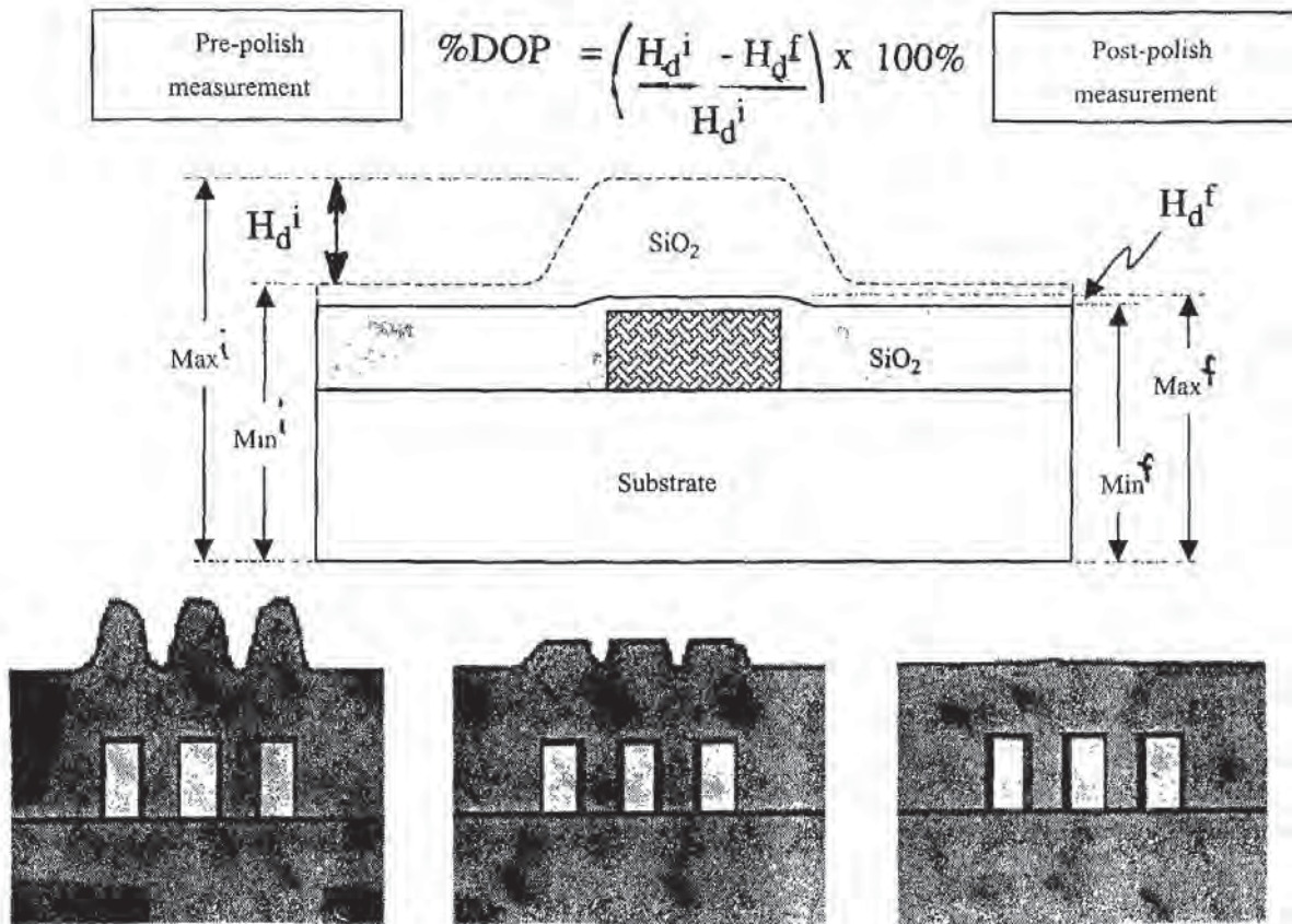
Fig. 8-10 Definition of degree of planarization (DOP) .
