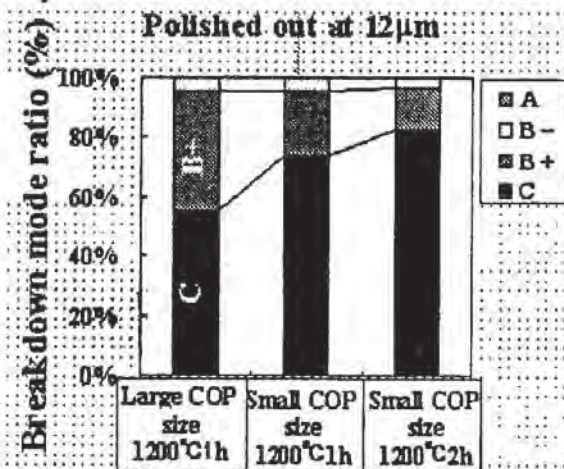
Fig. 2-11 Gate oxide integrity is best on wafers with small COP size ("C" breakdown mode indicates breakdown field of the gate oxide is > 10 MV/cm). 30
