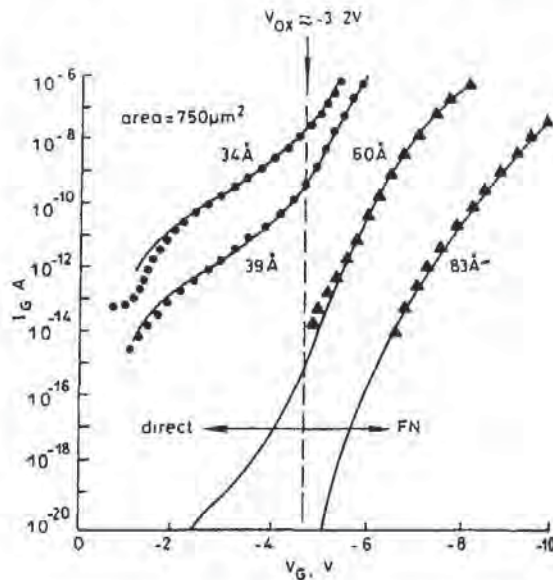
Fig. 3-20 Theoretical (and experimental) tunneling I-V curves of Al-gate n -channel MOS structures under negative gate-bias, illustrating the I-V characteristics of Fowler-Nordheim tunneling in 6-nm- and 8.3-nm-thick oxides and the calculated direct tunneling-currents in 3.9-nm- and 3.4-nm-thick oxides. 19 (© IEEE 1983)
