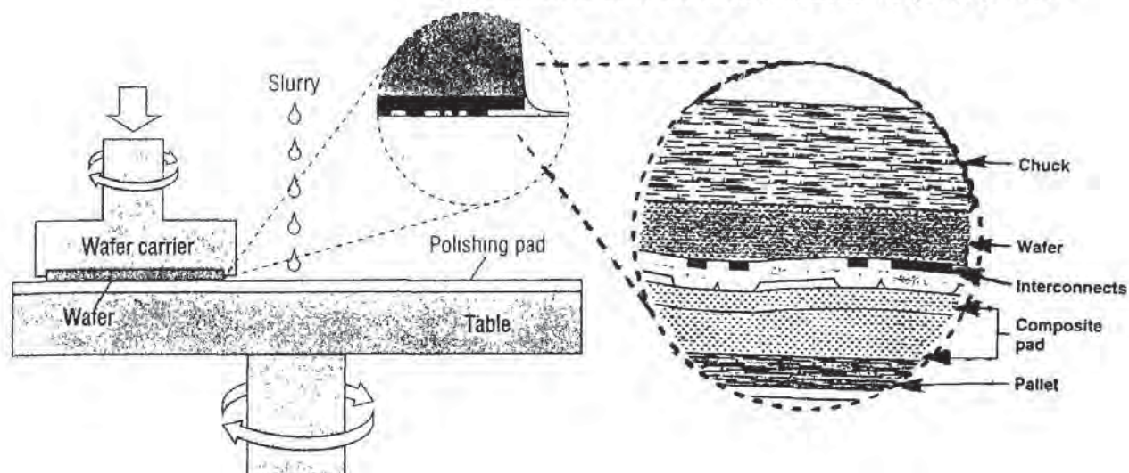
Fig. 8-31 Schematic diagram of a wafer being polished by CMP.
