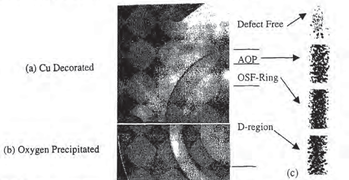
Fig. 2-9 a) Plane x-ray topograph of Cu-decorated CZ-Si wafer; b) Plane x-ray topograph of oxygen-precipitated CZ-Si wafer. The D-region, OSF ring, and defect-free regions are observed. c) Details of the defects delineated in each region.
