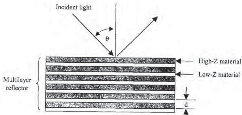
Fig. 7-29 Principle of a multilayer reflector for EUV radiation.
