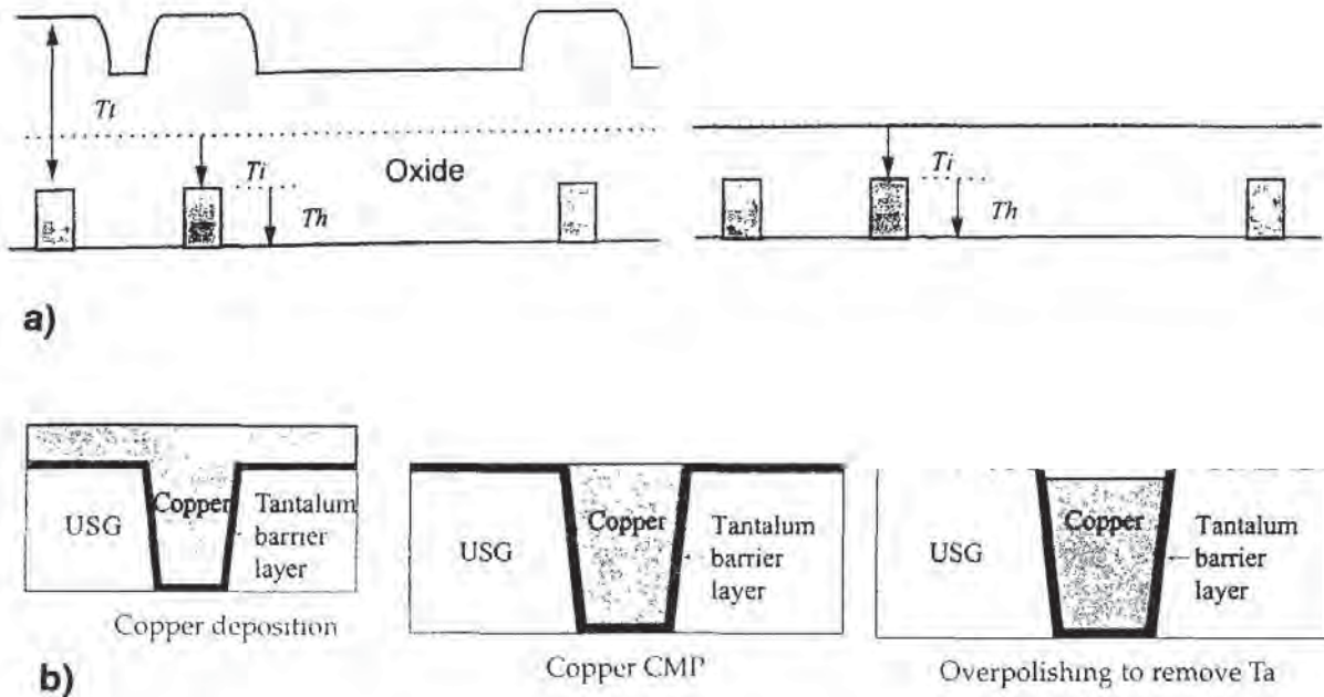
Fig. 8-25 The process of removing material by CMP falls into two categories: a) Removing homogeneous material and stopping while the removal of the surface film is incomplete (e.g., planarization of an ILD oxide); b) Removing deposited material, but continuing until all material is entirely removed on some regions of the wafer surface, while in other regions it remains recessed below the surface (e.g., Cu-damascene feature formation by CMP).
