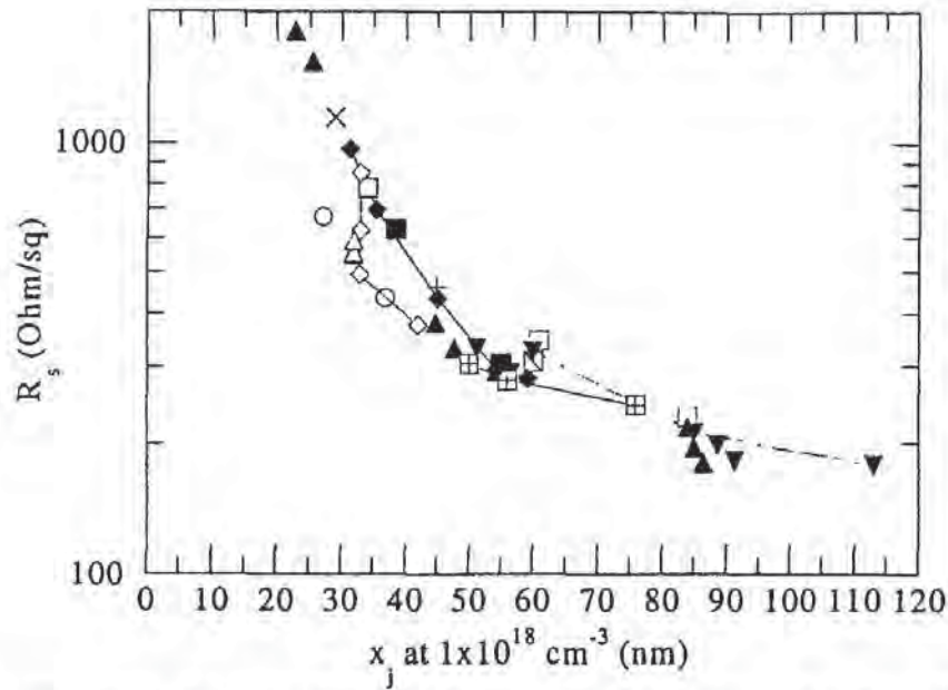
Fig. 5-22 Comparison of p -type sheet-resistance and junction-depth data for spike-anneals using various implant-and-annealing conditions. The data set includes a 400°C/sec ramp-up-rate and 0.2-keV implant-energy. Note that all the data points fall in a rather narrow band. No one has been able to make a 30-nm junction with a 300-Ω/sq sheet-resistance using ion-implantation and conventional rapid-thermal-annealing. 32
