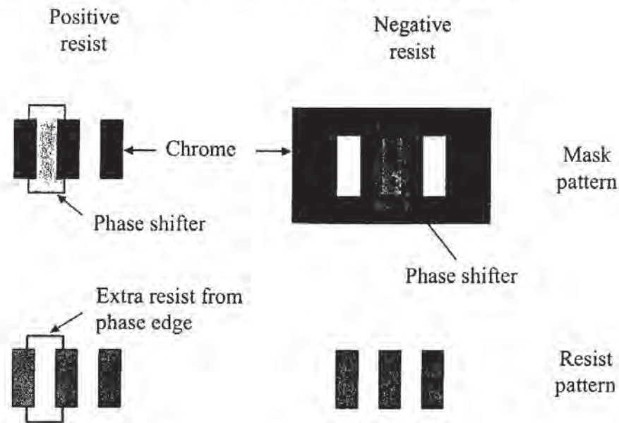
Fig. 7-20 On the left, extra resist printed by the phase edge, for positive photoresist. The right side of the figure shows what occurs with negative resist.
