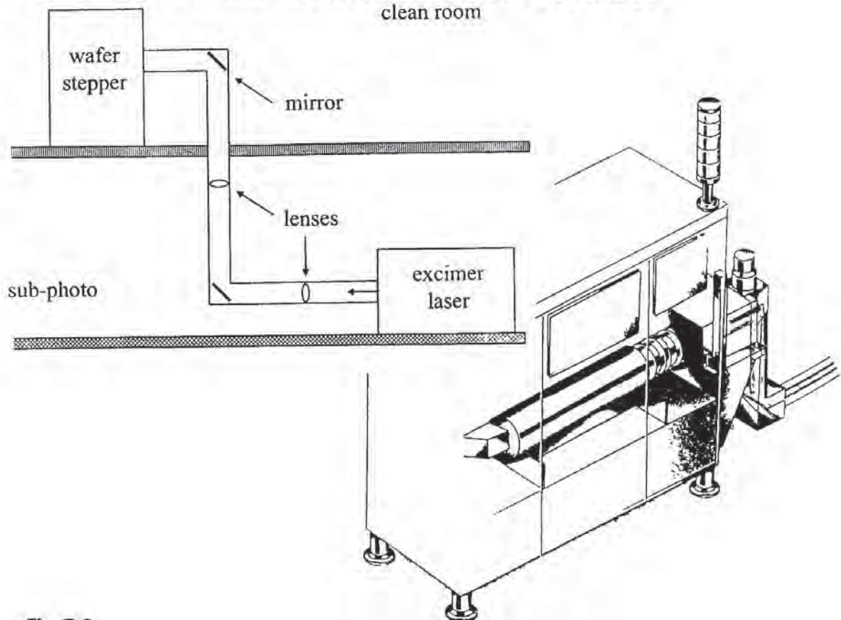
Fig. 7-6 The ASML PAS 5500/900 step-and-scanner. (Courtesy of ASML)
