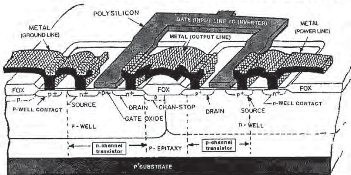
Fig. 1-7 Perspective schematic view of a twin-well CMOS structure.
