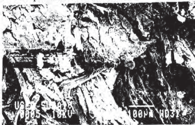
Fig. 8-56 Surface of a glazed pad (Rodel's Suba IV ® pad) after polishing.
