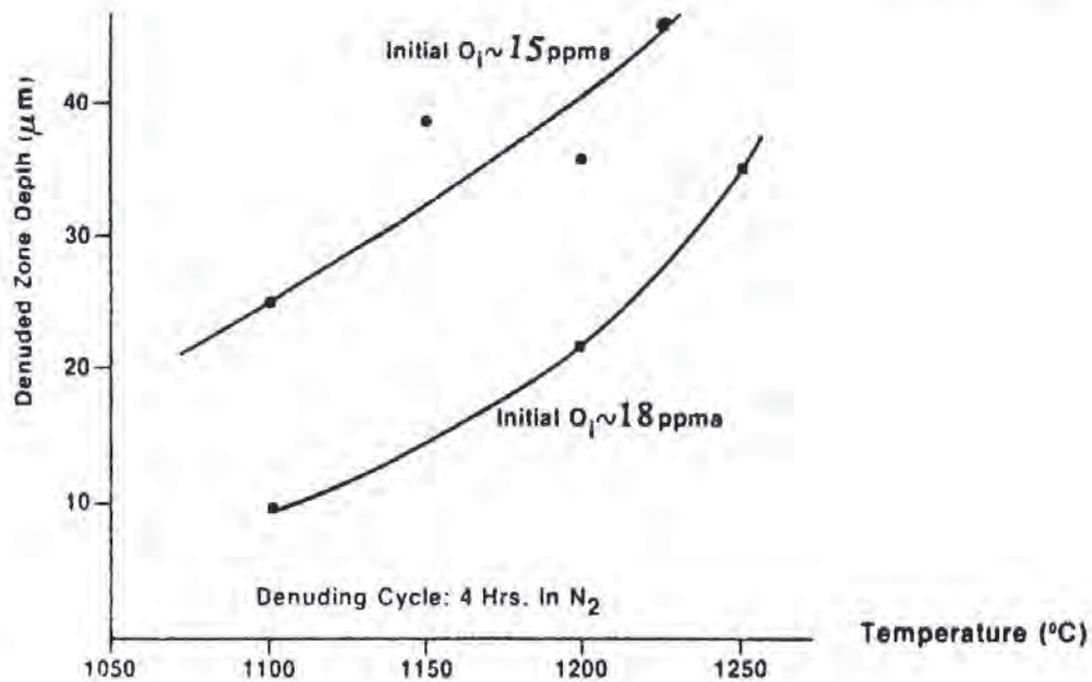
Fig. 2-17 Effect of initial oxygen concentration on the denuded zone depth. 43
