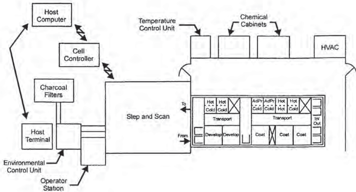
Fig. 6-15 DUV Photo-island.
