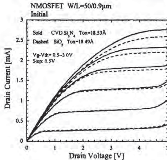
Fig. 4-3 The current-voltage ( I_D - V_{DS} ) characteristics of a 0.9 \mu\text{m} NMOSFET using Si 3 N 4 and SiO 2 as the gate dielectrics. 4
