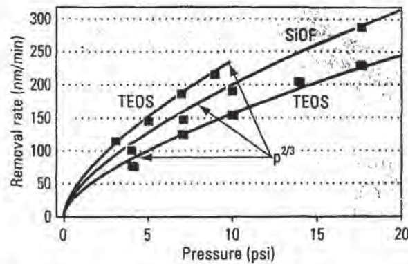
Fig. 8-19 Experimental data correlates well with the P^{2/3} dependence of removal-rate on applied pressure. 16
