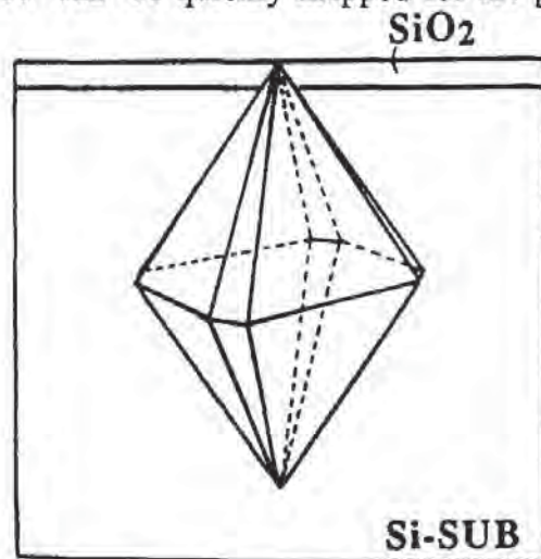
Fig. 2-7 Schematic representation of the octahedral structure of a COP defect.
