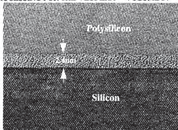
Fig. 3-49 HRTEM of 2.4 nm-thick oxide. 90 (© 1997 IEEE)
