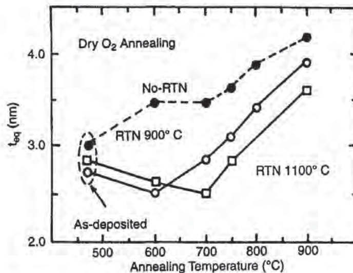
Fig. 4-8 An oxide grows on \text{Ta}_2\text{O}_5 during post-deposition \text{O}_2 annealing. This graph depicts the dependence of t_{\text{oxeq}} of \text{Ta}_2\text{O}_5 on the annealing temperature in a dry- \text{O}_2 atmosphere. 11
