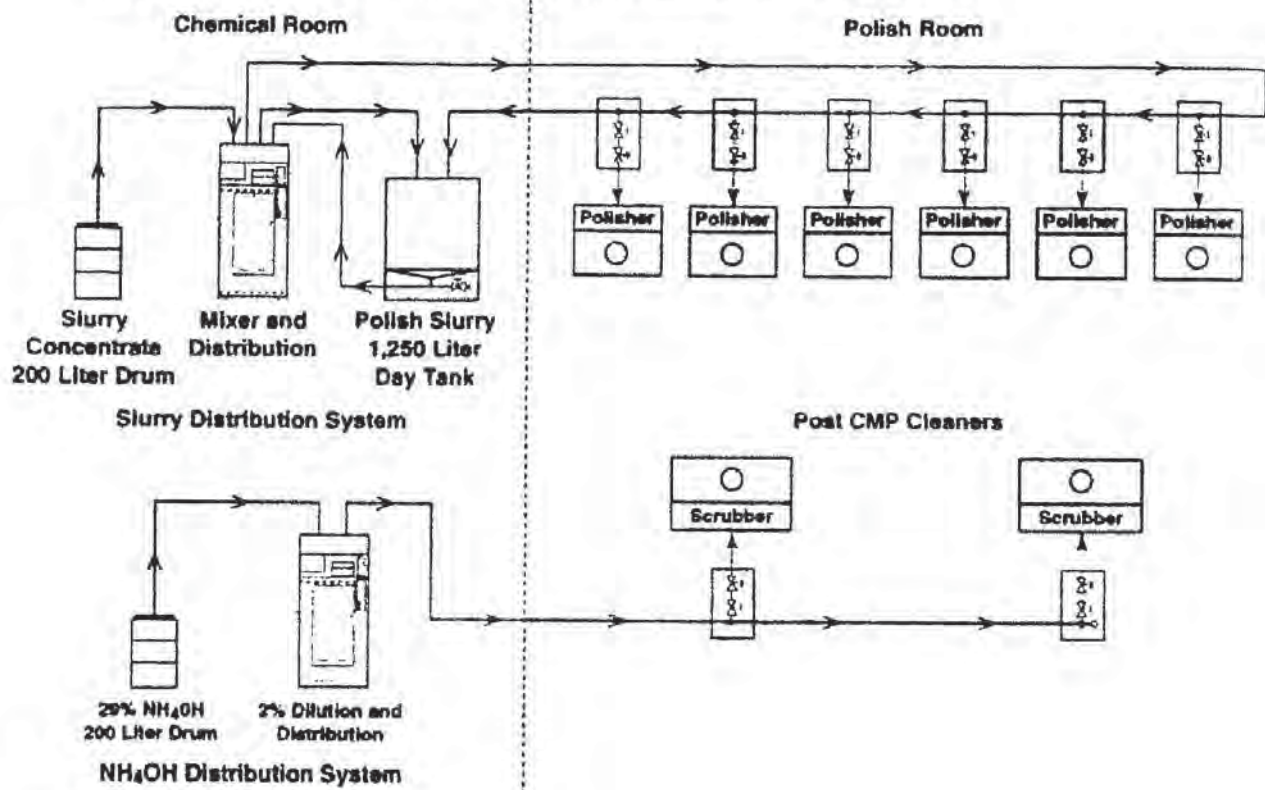
Fig. 8-50 Slurry distribution system.
