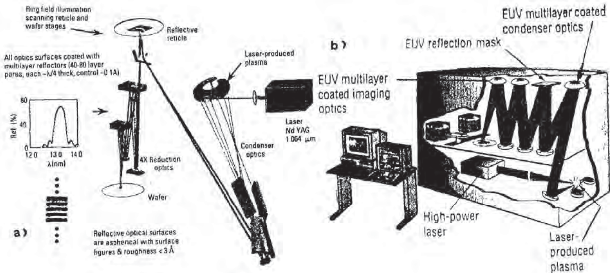
Fig. 7-28 (a) Schematic drawing of the optics of an EUV system. (b) An artists drawing of an EUV lithography system. A laser generates EUV radiation by exciting a laser produced plasma. This radiation is collected by a multilayer condenser system. The radiation illuminates a multilayer coated reflection mask, which is imaged and demagnified onto a resist-coated wafer. 46 Reprinted with permission of Solid State Technology, published by PennWell.
