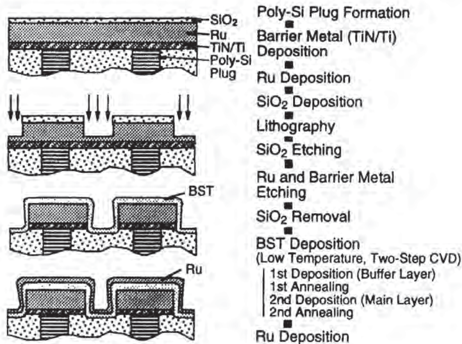
Fig. 4-14 Process flow for the fabrication of Ru/BST/Ru capacitors. 48 (© 2000 IEEE).
