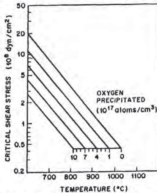
Fig. 2-20 Yield strength of Si showing the influence of oxygen precipitates. 42
