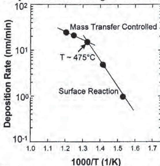
Fig. 4-12 Arrhenius plot showing two regimes of rate-limiting mechanisms for CVD BST deposition using non-adducted precursors. Courtesy of Marcel Dekker Publishing.
