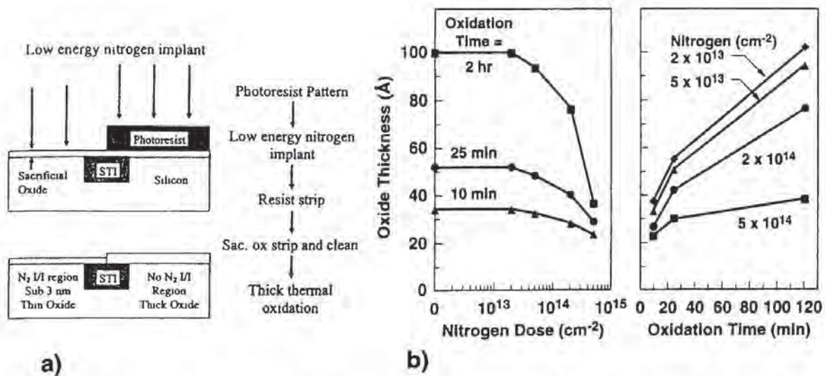
Fig. 3-35 a) Schematic of the process flow for sub-3-nm gate oxide formation on N_2 -implanted substrates. b) Oxide thicknesses obtained in dry- O_2 at 800^\circ C for various nitrogen implant doses (energy = 25 keV) and oxidation times. 89 (© IEEE 1997)
