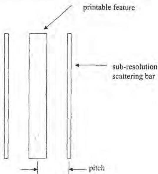
Fig. 7-15 Sub-resolution scattering bars applied to isolated features.
