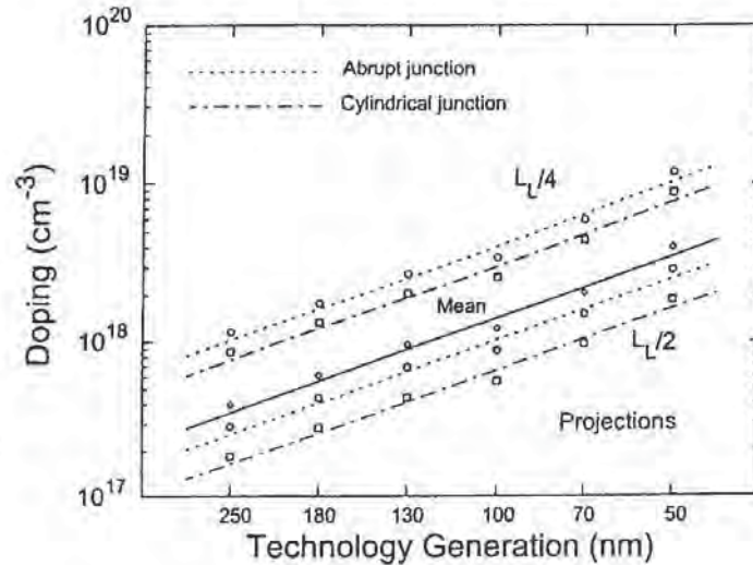
Fig. 5-9 Doping density required for punchthrough control. 11
