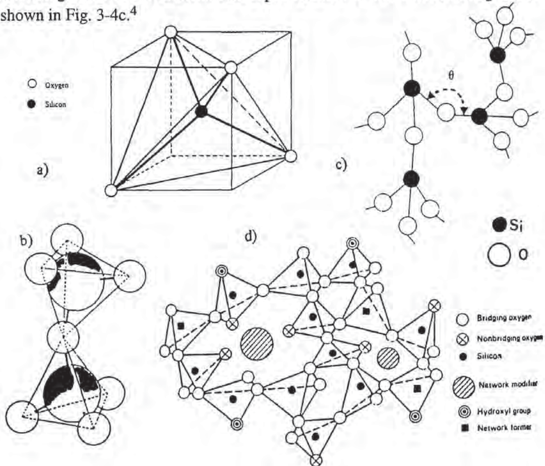
Fig. 3-4 (a) The basic structure of \text{SiO}_2 . 2 (b) Three-dimensional representation of two neighboring \text{SiO}_4 cells, bridged by an oxygen atom. (c) Two-dimensional lattice representing vitreous- \text{SiO}_2 . 2 (d) The structure of thermally grown \text{SiO}_2 showing bridging and non-bridging oxygen atoms and dopant (i.e., network modifier) atoms. 3 (© IEEE 1965)
