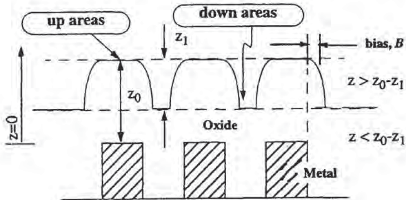
Fig. 8-26 Cross section of conformal dielectric on patterned metal, showing the “up-regions” and “down-regions” of the dielectric film.
