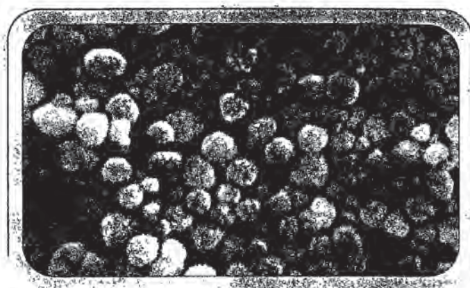
Fig. 8-49 SEM of cerium oxide slurry particles. Courtesy of Fujimi Corporation.
