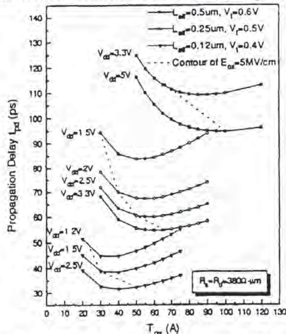
Fig. 3-46 At low V_{DD} (e.g., 2 V) and 0.2\text{-}\mu\text{m} , due to the polysilicon-depletion-effect, optimum speed may require a thicker t_{ox} than that allowed by the 5-MV/cm limit. 84
