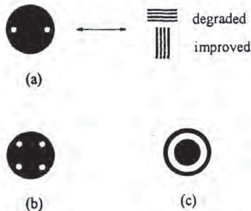
Fig. 7-11 Different types of off-axis illumination apertures. The aperture with holes at the edges or corners - (a) and (b) - will improve lines oriented in one direction (see a1), but will degrade imaging of lines in the orthogonal direction. (c) Annular off-axis illumination aperture. 23
