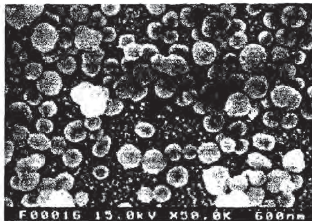
Fig. 8-48 SEM of colloidal-silica slurry particles. Courtesy of Fujimi Corporation
