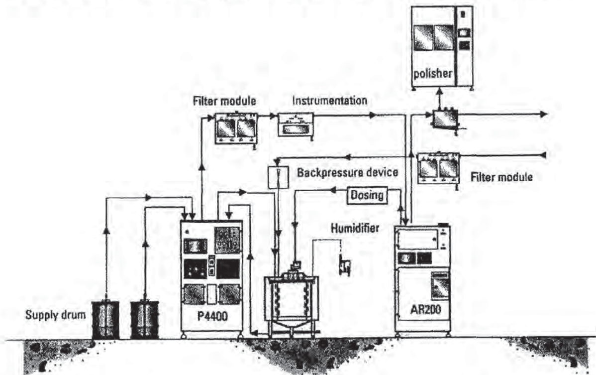
Fig. 8-51 Schematic of a slurry management-system with metrology, auto-dosing and filtration.
