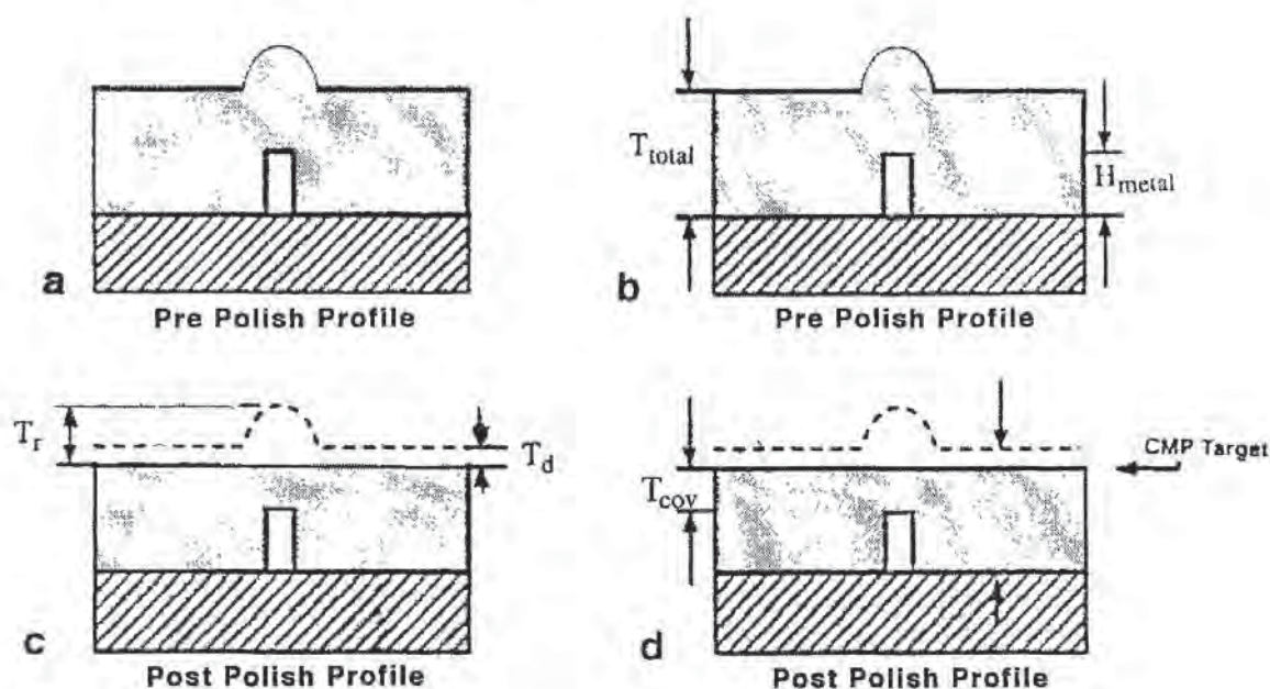
Fig. 8-17 The basic CMP process is one of reducing film-thickness selectivity over the wafer, ending with improved planarity. Here that metric is defined as efficiency of planarization (EOP).
