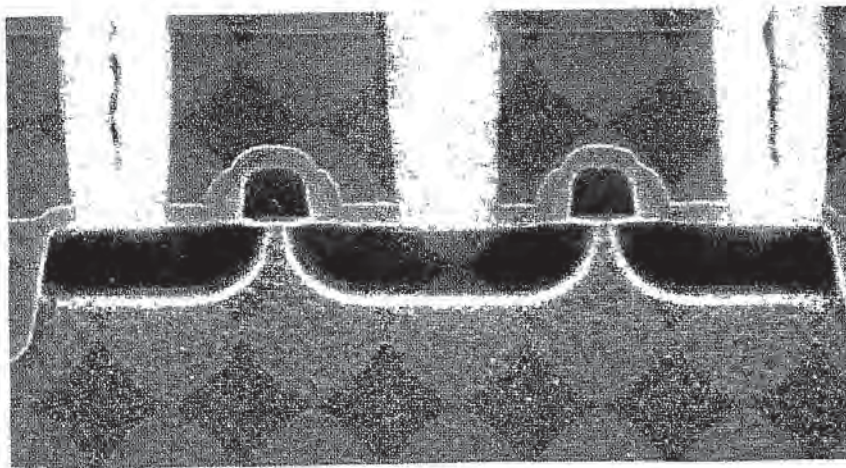
Fig. 1-10 A SEM micrograph of 0.18- \mu\text{m} MOSFET transistors in logic structures.
