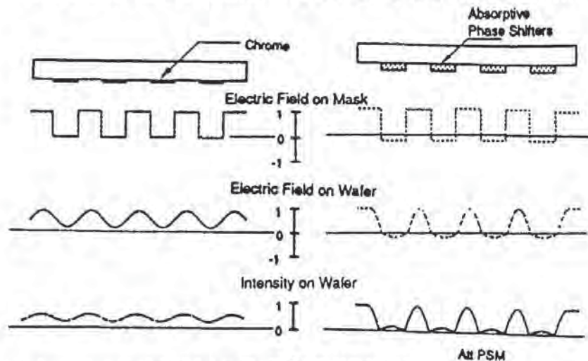
Fig. 7-22 Principle of the attenuated-PSM (attPSM). 31 © IEEE (1993)
