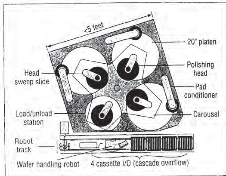
Fig. 8-36 Architecture of the Mirra® three-platen CMP tool. Courtesy of Applied Materials, Inc.
