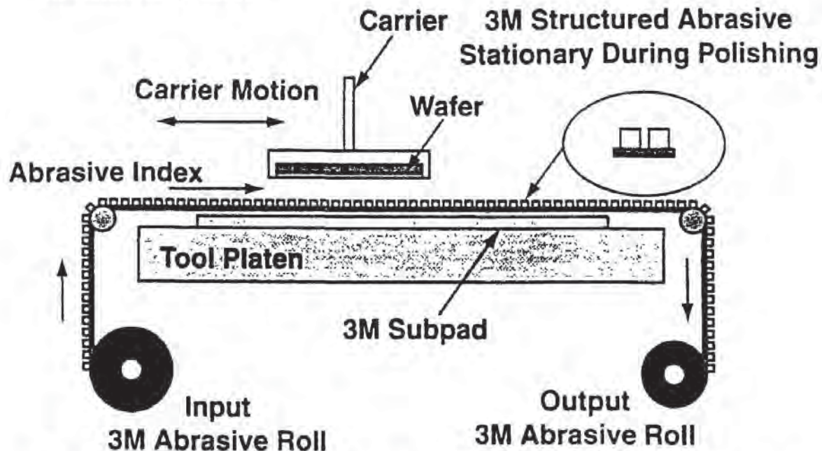
Fig. 8-41 Fixed-table with roll-to-roll pad. Carrier rotates and also executes linear motion.
