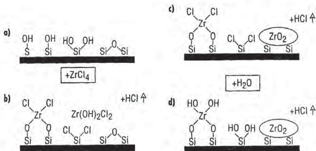
Fig. 4-16 Atomic layer CVD growth mechanism of the high- k dielectric \text{ZrO}_2 from \text{ZrCl}_4 and \text{H}_2\text{O} . Courtesy of ASM International.
