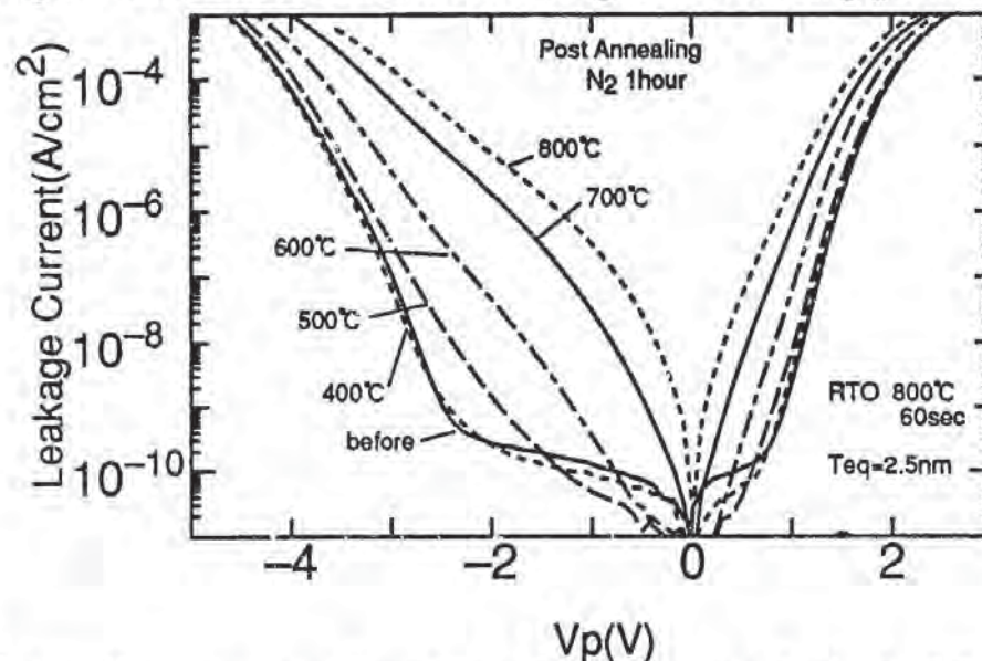
Fig. 4-9 Annealing temperature dependence of leakage current density for 2.5 nm \text{Ta}_2\text{O}_5 capacitors. A rapid thermal oxidation (RTO) is performed after \text{Ta}_2\text{O}_5 film deposition. 19
