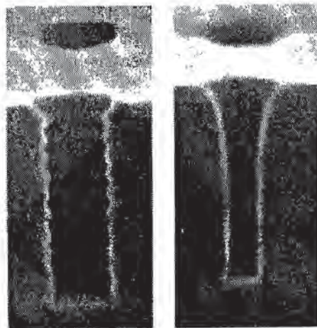
Fig. 6-7 The RELACS process shrinks these KrF-imaged 0.22\text{ }\mu\text{m} contact holes (left) to 0.11\text{ }\mu\text{m} (right) using a coat, diffusion bake, and rinse step after wafer patterning. (Courtesy of Clariant AZ)
