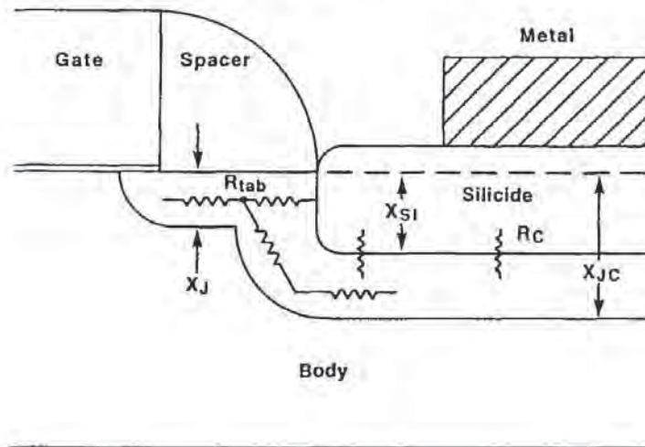
Fig. 5-14 Schematic drawing of the components of source or drain resistance in a deep-submicron MOSFET.
