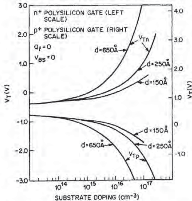
Fig. 3-2 Calculated threshold voltages of n -channel ( V_{Tn} ) and p -channel ( V_{Tp} ) transistors as a function of their substrate's doping, assuming n^+ polysilicon gate (left scale) and p^+ polysilicon gate (right scale). Curves for gate oxide thicknesses d of 150\text{\AA} , 250\text{\AA} , and 650\text{\AA} are shown. From S.M. Sze Ed. VLSI Technology , 2nd Ed., Chap. 11, "VLSI Process Integration." Copyright, 1988 Bell Telephone Labs. Reprinted with permission.
