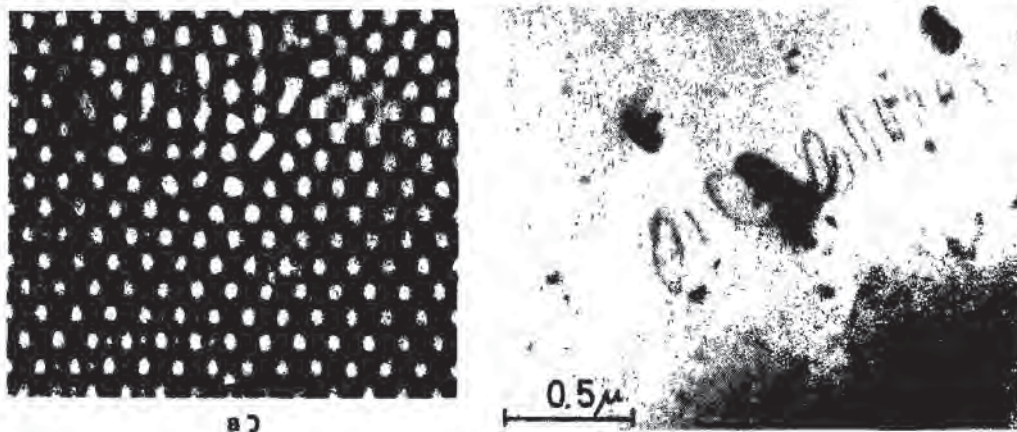
Fig. 2-19 a) Image of the core of a dislocation in Si obtained by high resolution TEM depicts an extra plane of atoms that terminates at the core of the dislocation. A precipitate is at the core. 24 (©1985 IEEE); b) Dislocation loops generated in Si due to prismatic punching by \text{SiO}_2 particles. 25
