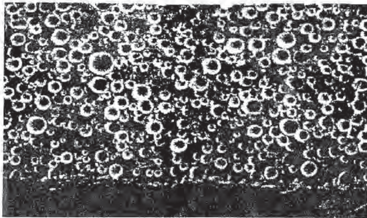
Fig. 8-52 SEM of a new Rodel 1000 IC Pad. Courtesy of Rodel Inc.
