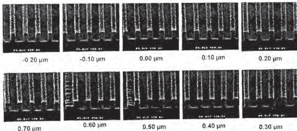
Fig. 6-9 70-nm gates patterned with 193-nm resist and alternating phase-shift mask. Courtesy of Semiconductor International. 21
