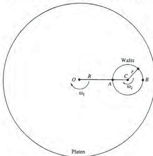
Fig. 8-21 Plan view of a single-carrier single-platen rotary-polisher, showing relative rotary motions of both the carrier and the platen.
