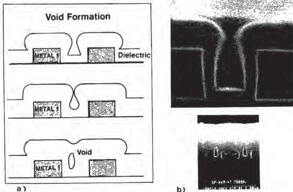
Fig. 8-7 (a) Diagram of void-formation due to cusping of the dielectric. (b) SEM of voids left between 1.5- \mu\text{m} -spaced Metal-1 lines in a 3.0- \mu\text{m} -thick PMD PECVD oxide.
