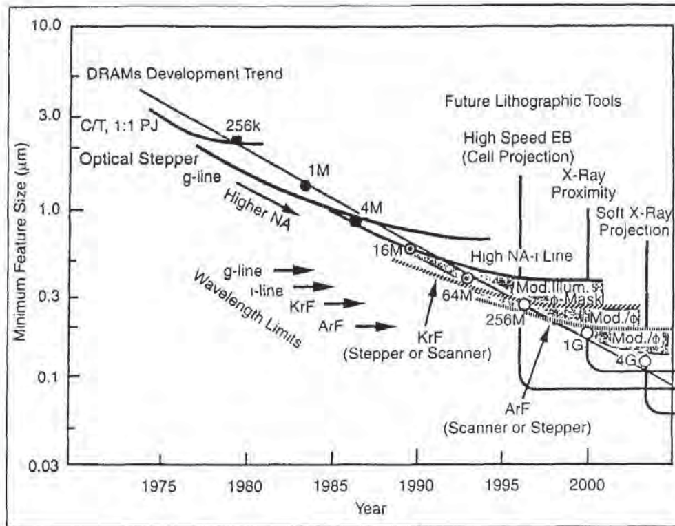
Fig. 6-1 Lithography Scaling Roadmap
