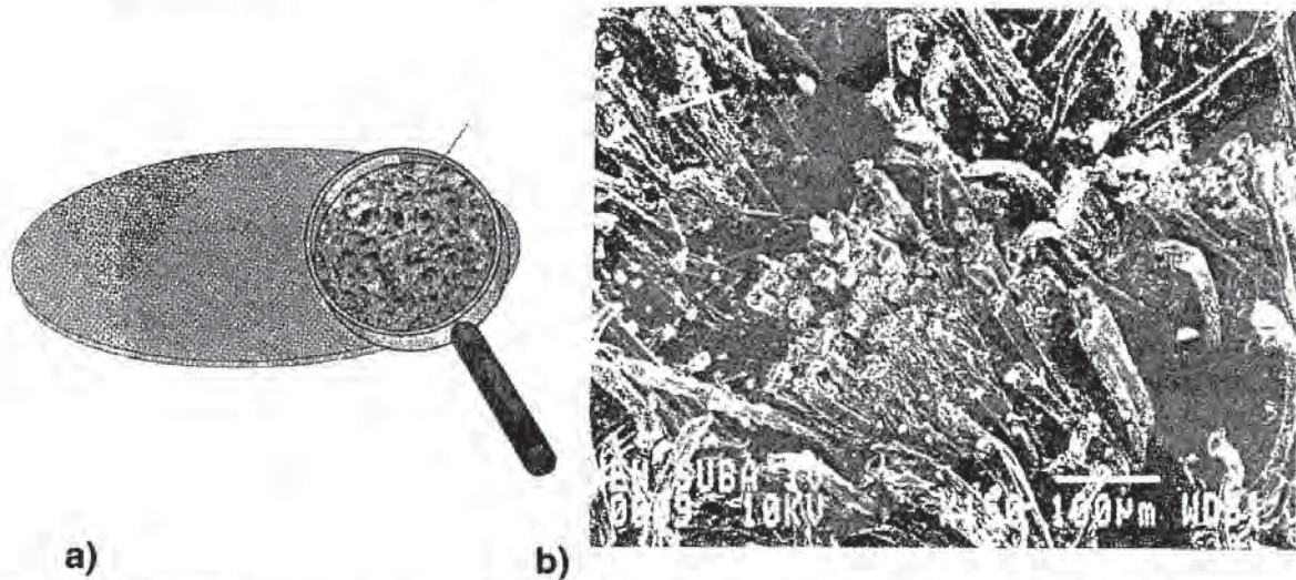
Fig. 8-52 a) Schematic of polishing pad; b) SEM of a new Rodel Suba IV® Pad. Courtesy of Rodel Inc.
