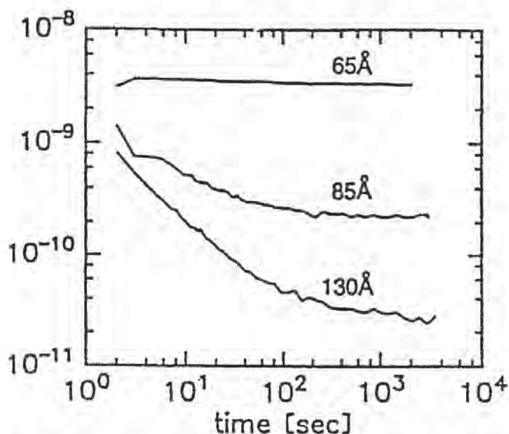
Fig. 3-40 Stress-induced leakage current is a transient current in thicker oxides but is a continuous current in thinner oxides, preventing nonvolatile memory scaling. 81
