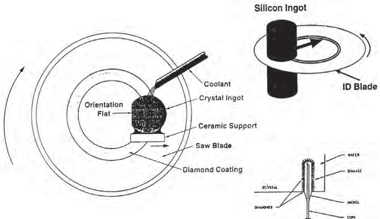
Fig. 2-24 ID saw geometry. 66
