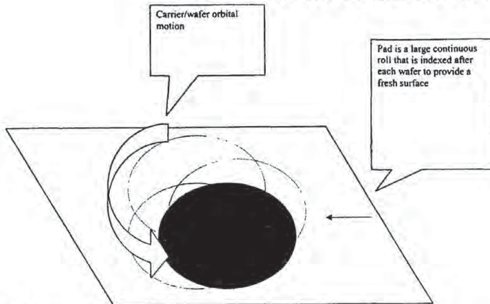
Fig. 8-40 Schematic drawing of orbital carrier-motion with indexing pad.
