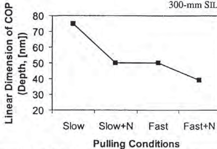
Fig. 2-10 Size of COPs in a silicon wafer as a function of pulling conditions. 28
