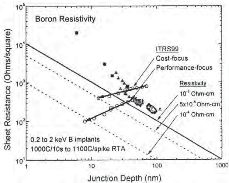
Fig. 5-20 Sheet resistance and source/drain junction depth expectations for CMOS transistors according to the ITRS99 study for cost and performance-focused product and gate sizes from 180 nm towards deeply-scaled devices with gates \sim 20 nm. Also shown are experimental results for sub-keV B^+ implants with “spike” RTA in CZ-Si materials. 59
