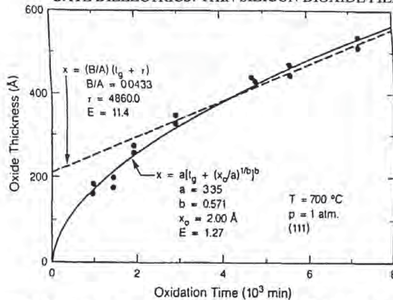
Fig. 3-23 Fits to oxide thickness versus oxidation time using the Deal-Grove model and the Reisman-Nicollian power-law model expression. 24
