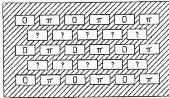
Fig. 7-18 Limitation of ALT-PSMs. There is no way to assign phases so that a 180^\circ -phase difference occurs between adjacent transparent features. In this example, the phases have been assigned to the odd-numbered rows, but there is no way to assign phases consistently to the even rows. 36 Reprinted with permission of Marcel Dekker.
