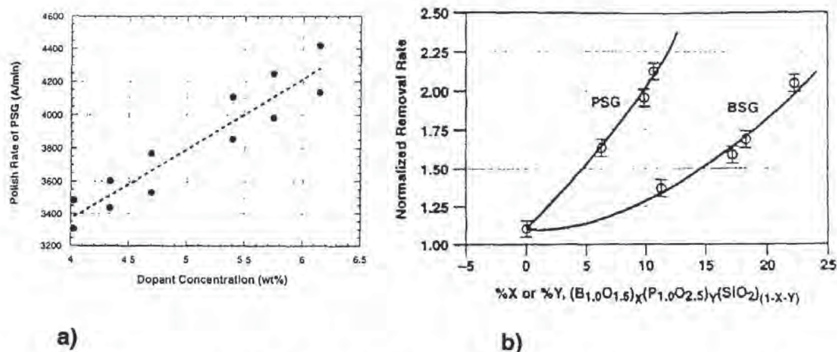
Fig. 8-23 a) Removal-rate of PSG as a function of phosphorus-concentration: pressure 4-psi, table speed: 40-rpm, carrier speed: 643-rpm; b) Removal rates of P-doped oxides and B-doped oxides as a function of P- and B-doping-concentration in the oxide. 19
