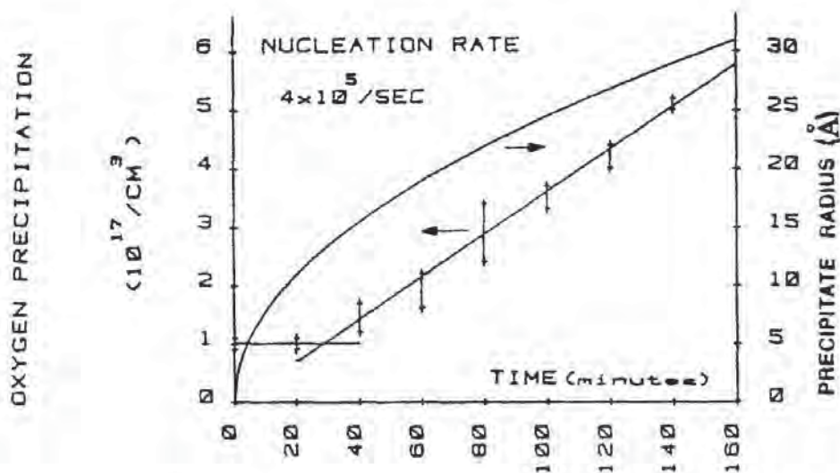
Fig. 2-18 Nucleation rate for oxygen precipitates. The curve is the expected rate of precipitate formation at 880°C. 47
