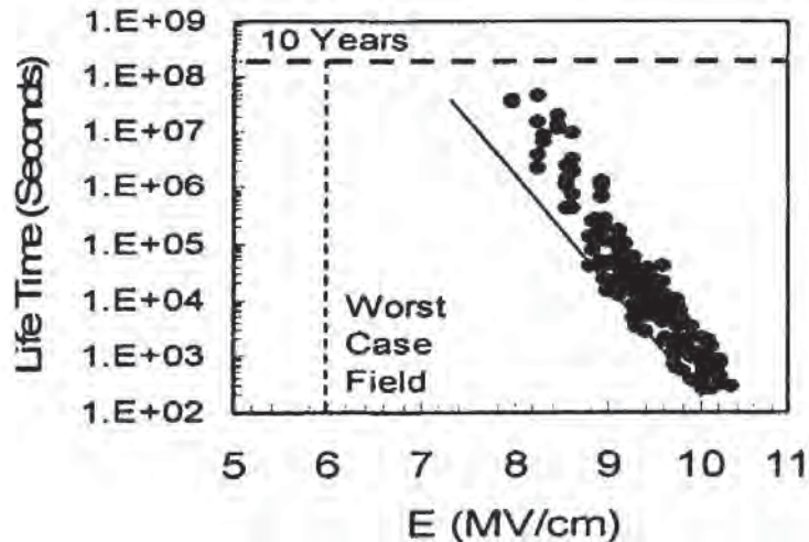
Fig. 3-38 TDDDB data for 2.0-nm thick oxides at 125°C from MOS-capacitor data. 79
