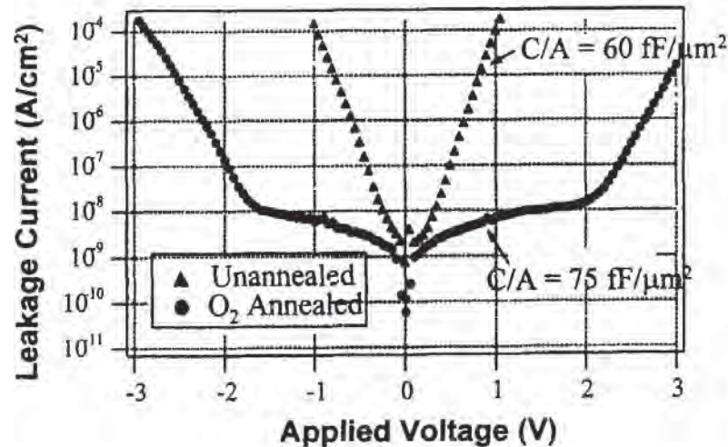
Fig. 4-13 Leakage curves from unannealed and 550°C oxygen-annealed BST films deposited at 600°C. Labels on the leakage curves give the corresponding capacitance densities of the films.
