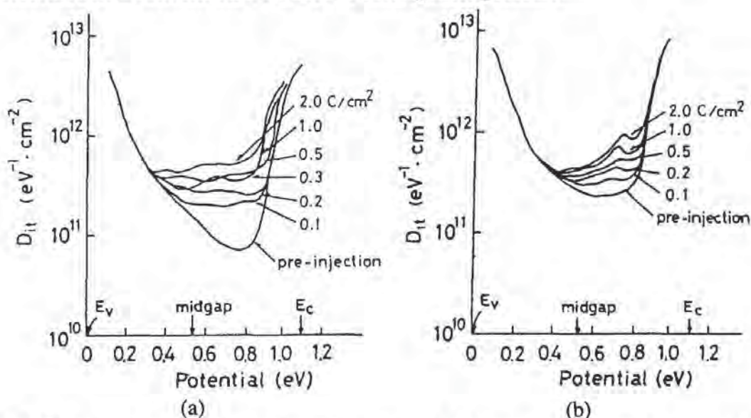
Fig. 3-30 Changes in the interface trap densities of MOS capacitors with: a) pure \text{SiO}_2 ; and b) \text{SiO}_x\text{N}_y by Fowler-Nordheim electron injection. Electrons were injected from the gate electrodes into the oxide films at a current density of \sim 10 \text{ mA}/\text{cm}^2 . 42 (© IEEE 1991)
