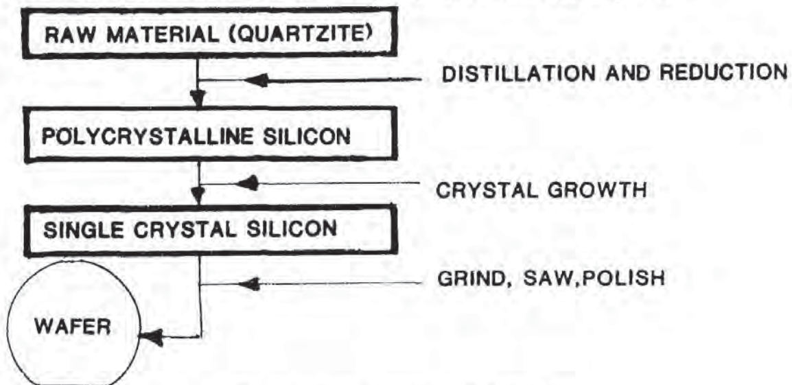
Fig. 2-1 Process sequence: From starting material to polished wafer.
