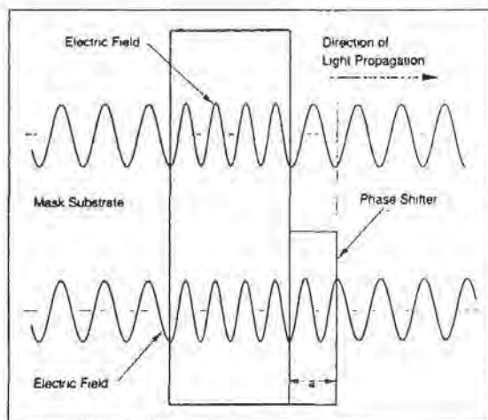
Fig. 7-16 The phase-shifting layer introduces a difference in optical-path-length. Here the difference is \lambda/2 . 30 © IEEE (1993)
