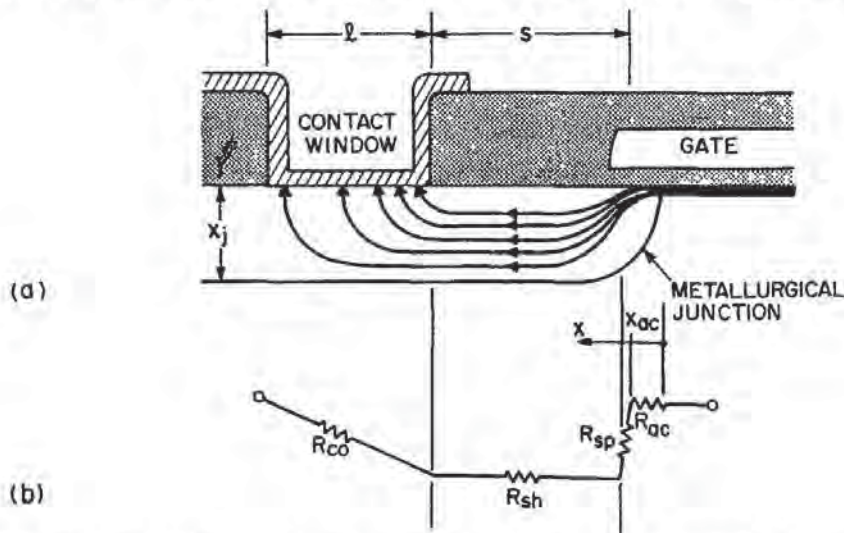
Fig. 5-13 Schematic drawing showing: a) current paths within the source and drain regions, of a planar MOSFET and; b) their corresponding representative series resistance components. 21 (© 1987 IEEE).
