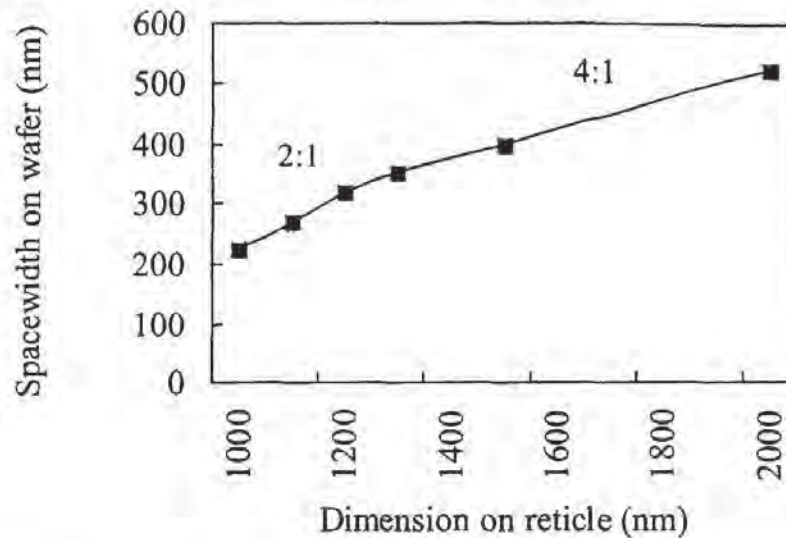
Fig. 7-23 Transfer of features from a reticle to the wafer. The features are reduced in size by 4x for large feature size, but the reduction changes for features near the resolution limit of the lens.
