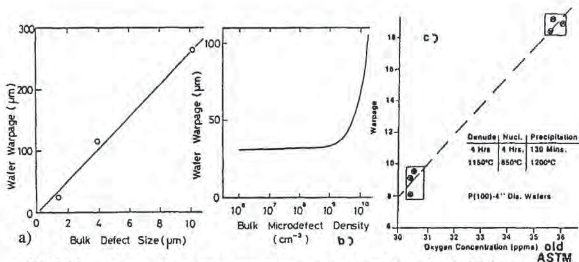
Fig. 2-15 a) Dependence of wafer warpage on bulk microdefect size; b) Wafer warpage as a function of bulk-microdefect-density. 42 c) Effect of Initial Oxygen content of the wafer on warpage.
