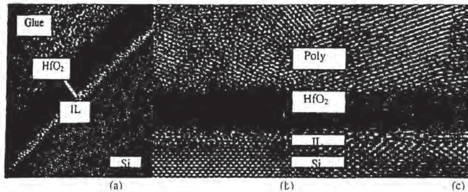
Fig. 4-17 HR-TEM showing \text{HfO}_2 ( \sim 38\text{\AA} ) and IL ( \sim 6\text{\AA} ): (a) after PDA, and (b) and (c) RTA 900^\circ\text{C} and 1000^\circ\text{C} for 1 min, respectively. 33 (© 2000 IEEE).
