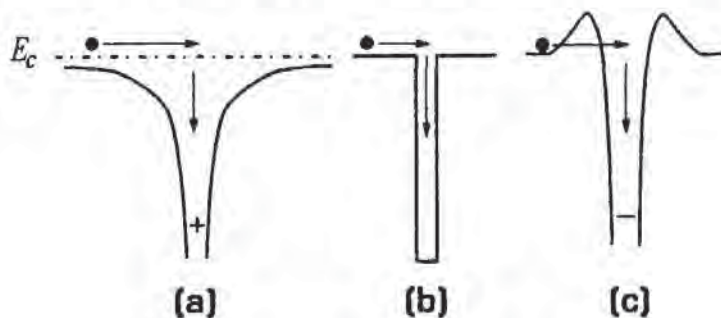
Fig. 3-9 Schematics illustrating the potential wells of electron traps in silicon dioxide: a) Coulomb-attractive trap; b) neutral trap; and c) Coulomb-repulsive trap.
