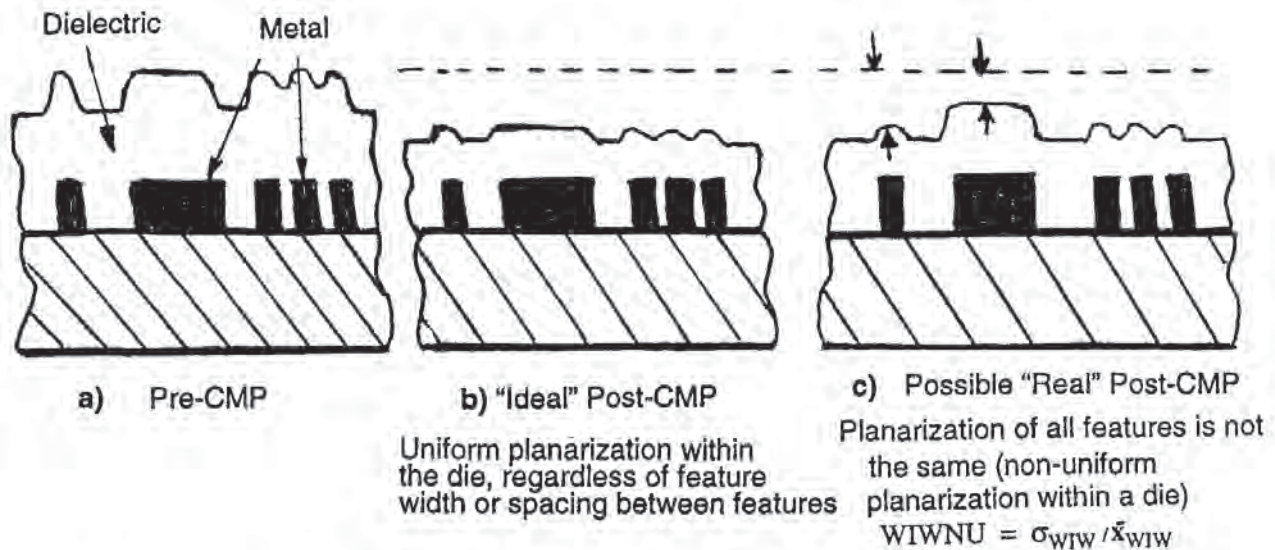
Fig. 8-13 Effect #2 that causes within-die non-uniformity , WIDNU (dishing).
