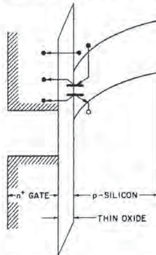
Fig. 3-19 Energy-band diagram for the phenomenon of direct tunneling through the gate oxide for thin oxides. Also shown are both unassisted-tunneling and some possible interface-trap-assisted leakage paths, with trap levels indicated by short, solid bars.
