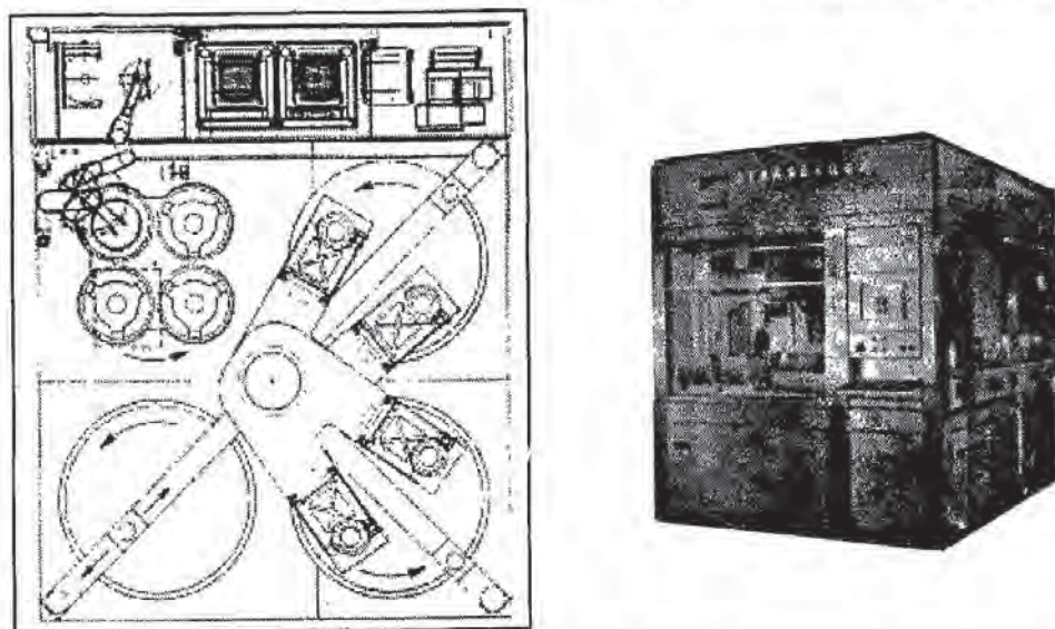
Fig. 8-34 Schematic drawing of the Symphony ® CMP tool. Courtesy of Strasbaugh Corp.
