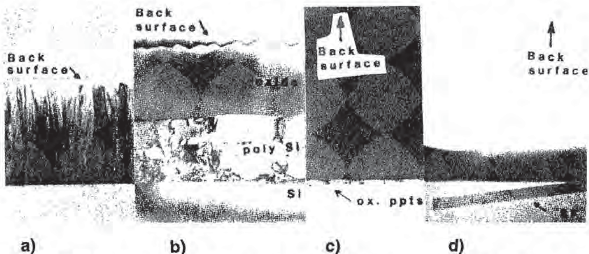
Fig. 2-13 Cross-sectional TEM micrographs of: a) as-deposited poly-Si, then wet oxidized at 1150°C for; b) 100 min; c) 765 min, and; d) 1300 min. 38
