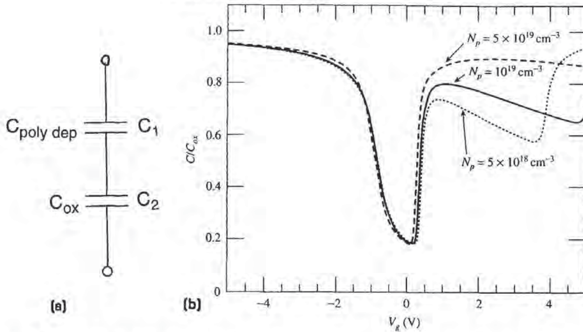
Fig. 3-44 a) Equivalent-circuit diagram of the polysilicon depletion-capacitance in series with the gate-oxide-capacitance. b) Low-frequency C-V curves of p -type MOS capacitor with an n^+ -polysilicon gate doped at several different concentrations. 96
