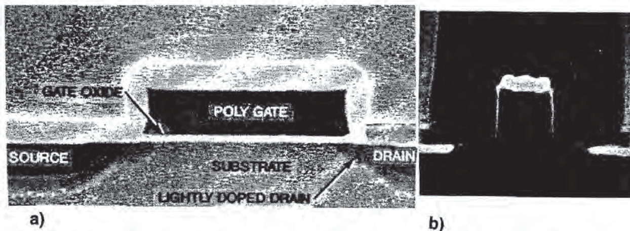
Fig. 1-1 SEMs of MOSFET cross-sections with different gate lengths: a) 2.0 \mu\text{m} ; b) 0.2 \mu\text{m} .
