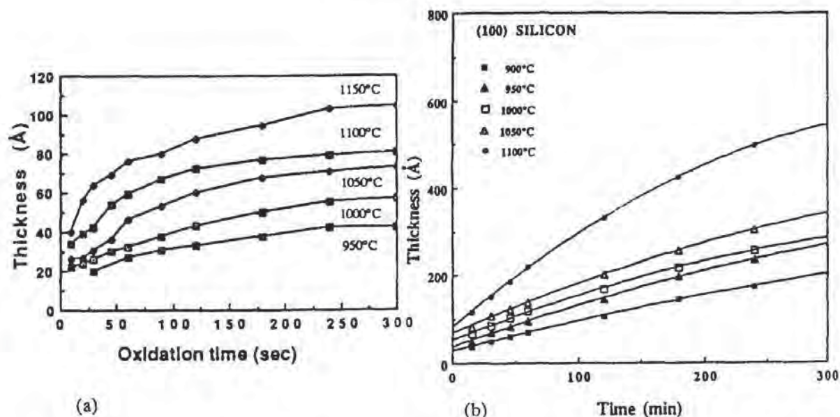
Fig. 3-29 (a) N 2 O oxynitride thickness versus oxidation time using RTP for various process temperatures. Ramp-up rate was 200°C/sec. Oxide thickness was measured at a fixed refractive index (1.46) 40 (© IEEE 1990); (b) N 2 O oxynitride thickness versus time in a furnace-anneal process. (© Electrochemical Society 1993) 45
