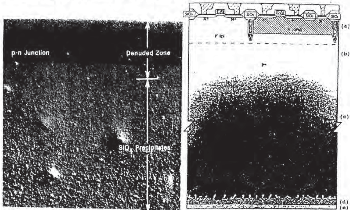
Fig. 2-14 SEM micrograph of a pn junction created by a 450°C anneal for 70 hr in denuded-zoned-Si with SiO x precipitates formed by thermal treatment. 40
