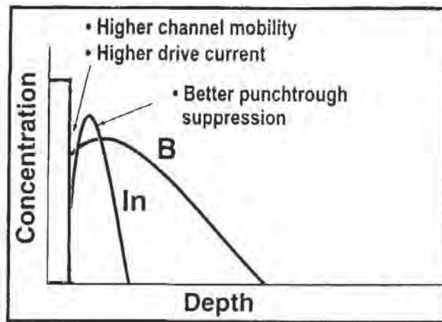
Fig. 1-4 As-implanted doping concentration profiles of threshold-adjust-implants with B and In as the implant species. The In implant produces a super-steep retrograde (SSR) profile.
