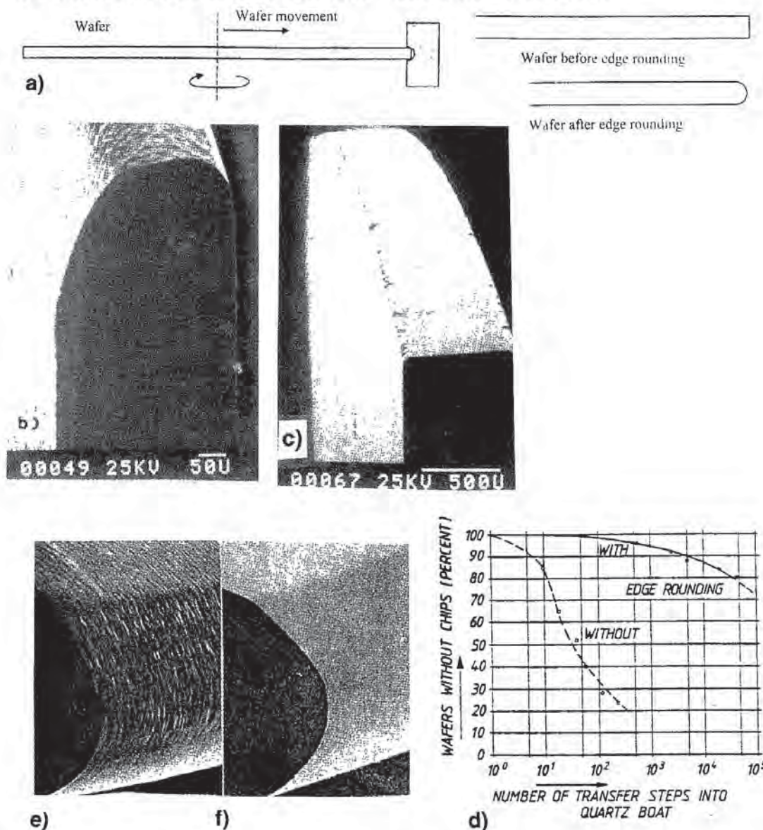
Fig. 2-27 a) Wafer edge-rounding process; b) Edge-rounded wafer; c) Non-edge rounded wafer; d) Mechanical strength of edge-rounded vs. non-edge-rounded wafers; e) Edge-rounded, but non-polished wafer; f) Edge-rounded, polished wafer.
