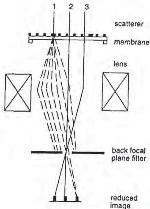
Fig. 7-31 Schematic of the SCALPEL technique. Electrons (1) that hit the scatterer (the metal patterns on the mask) are strongly scattered, and most are filtered out by the aperture. Electrons traveling through the silicon nitride membrane (2, 3) are only weakly scattered and pass through the aperture. These are demagnified to form a high contrast image on the substrate. Courtesy of Lucent Technologies, Inc.
