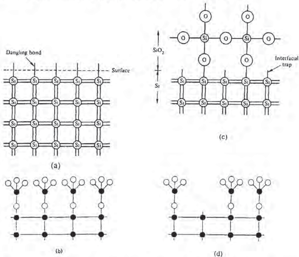
Fig. 3-6 Physical model for the interfacial traps. "Dangling bonds" which occur when the Si lattice is abruptly terminated along a given plane to form a surface. (b) Post-oxidation perfect (ideal) interface. (c & d) Post-oxidation dangling bonds that become interfacial traps. 7 Reprinted with permission of the publisher, the Electrochemical Society.
