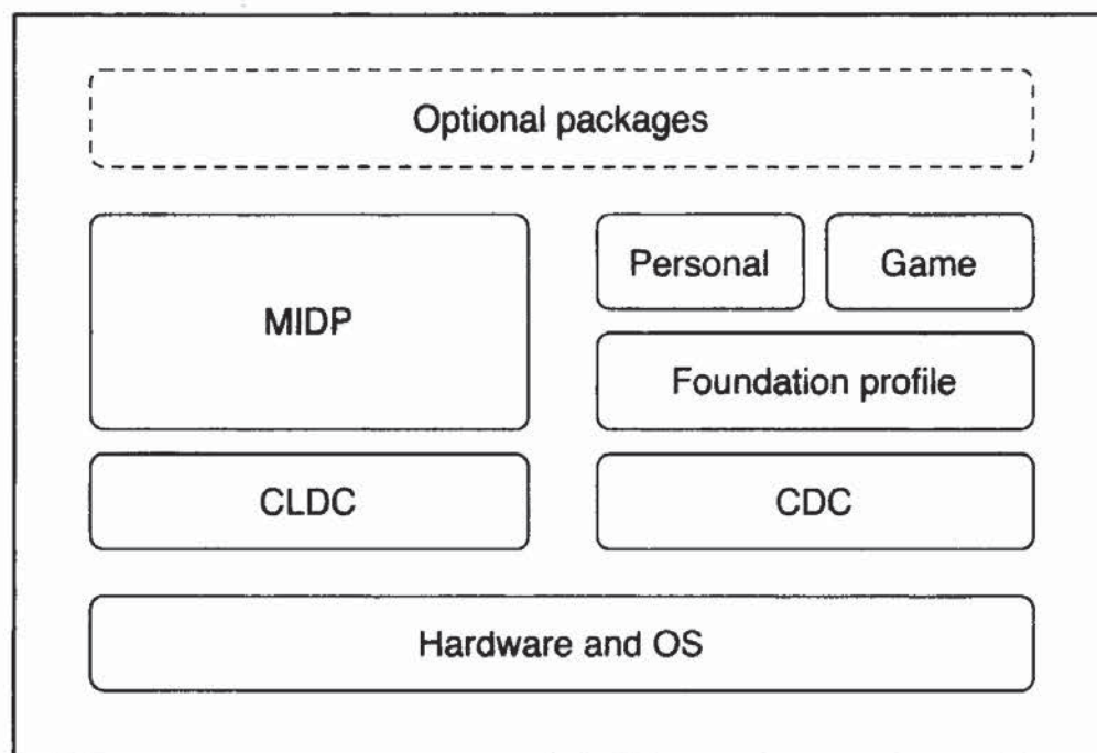
Figure 2–15 The J2ME architecture.
