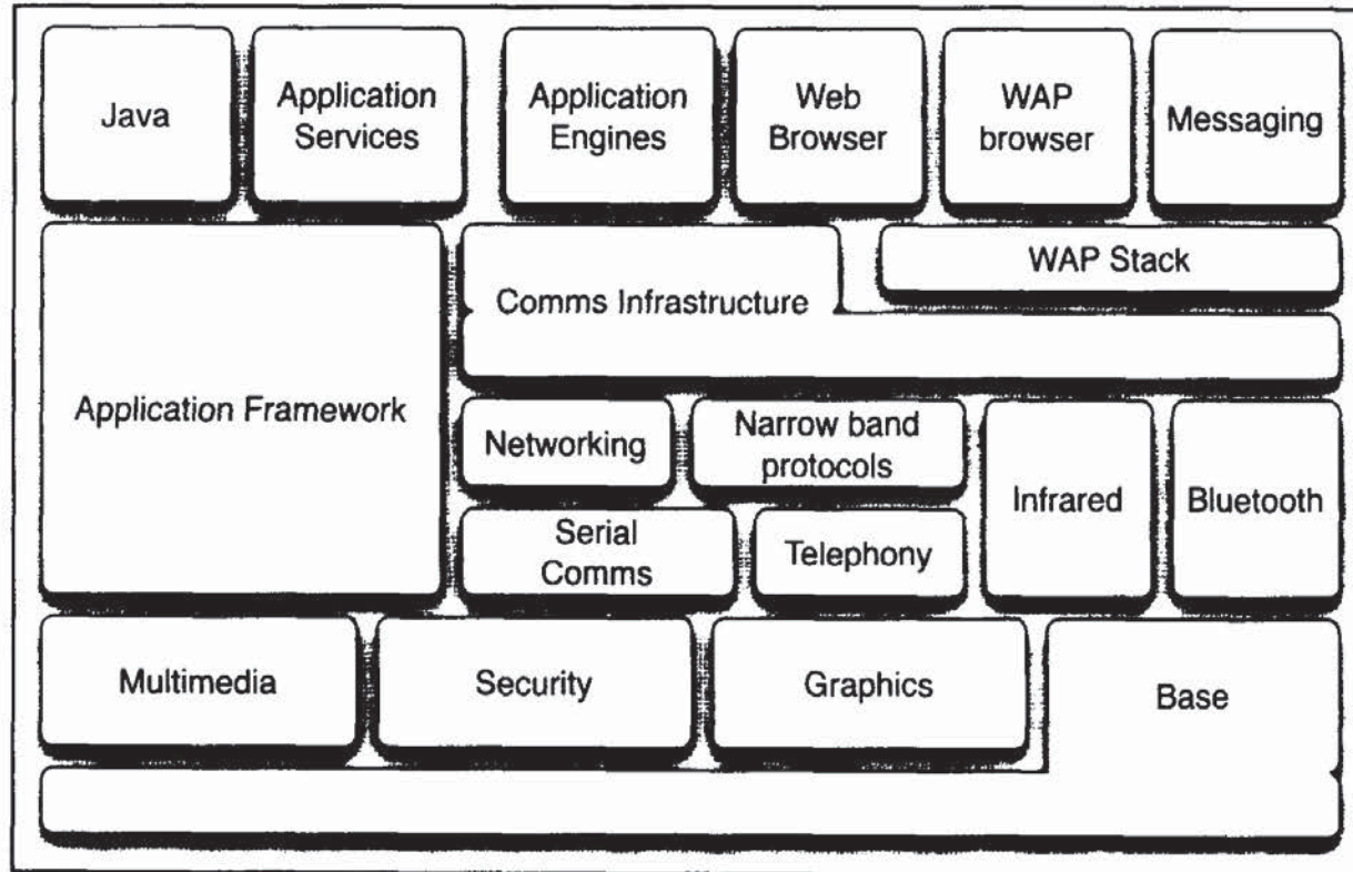
Figure 2-16 The Symbian OS API architecture.
