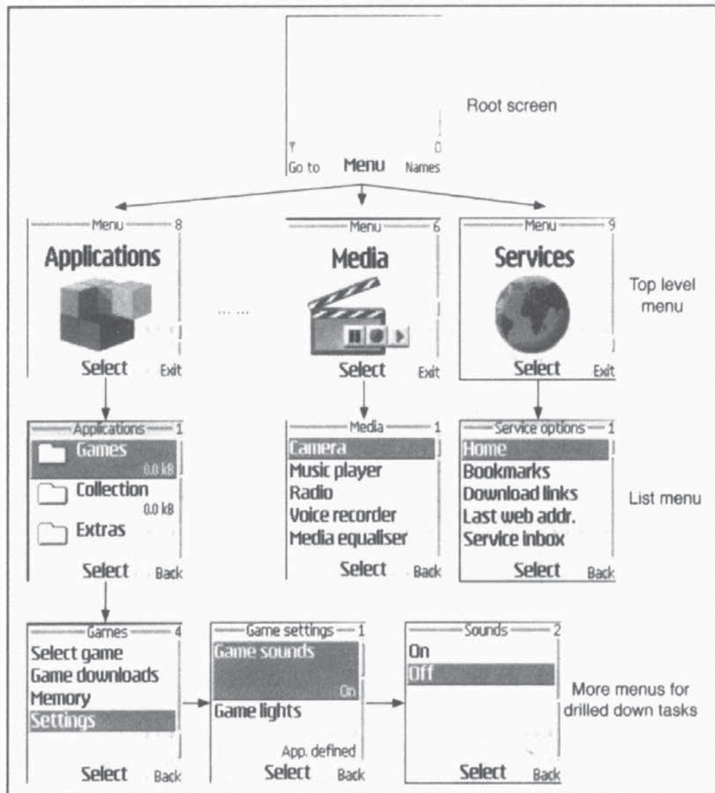
Figure 2-4 The UI menu for devices in the Series 40 Developer Platform.
