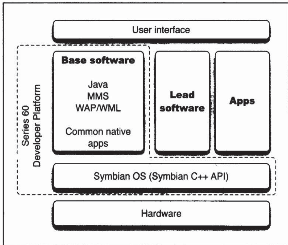
Figure 2-7 Software stack on Series 60 devices.
