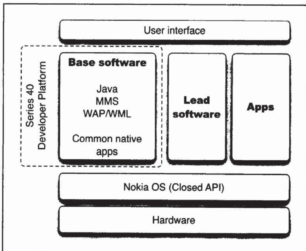
Figure 2-2 Software stack on Series 40 devices.
