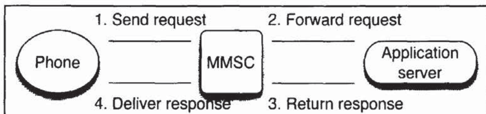
Figure 2-14 The MMS application interaction diagram.
