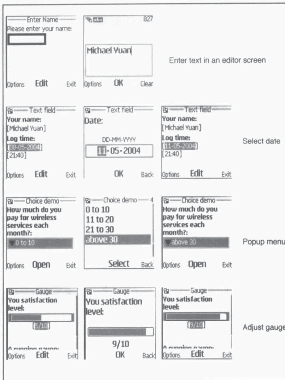
Figure 2-6 Interact with individual elements on a Series 40 device.
