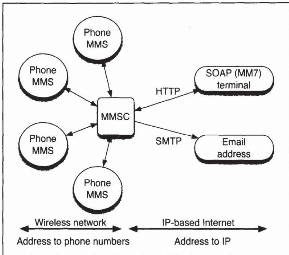
Figure 2-13 The MMS network architecture.
