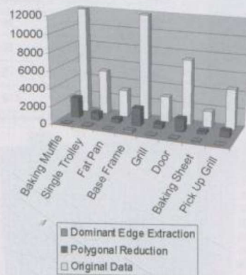
Figure 7: Memory requirements for each component (kilobyte)
