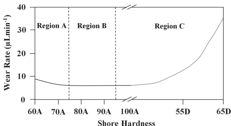
Figure 4. Abrasive wear rate of PU as a function of hardness [38, 39].
