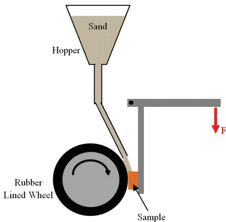
Figure 2. Schematic of standard testing method to measure abrasion resistance by dry sand/rubber wheel apparatus [34].
