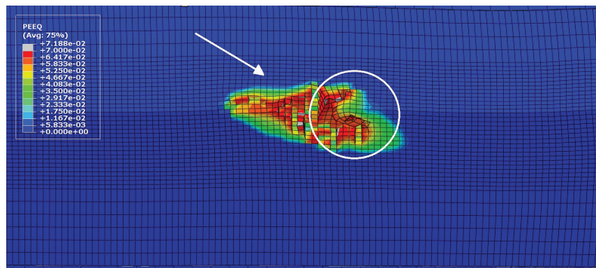
Figure 10. The ridges formed on the surface of an eroded PU as predicted by FE model [49].
