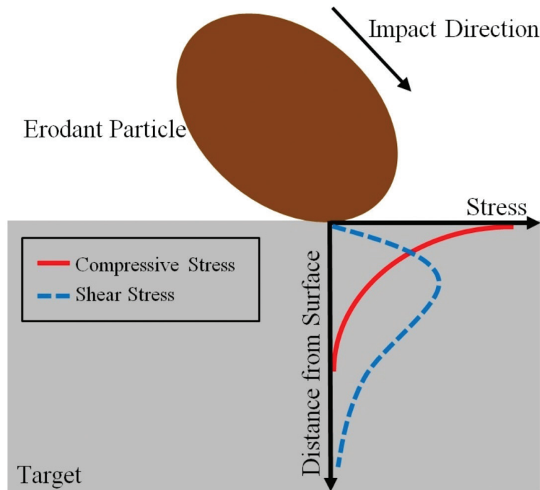
Figure 5. Schematic of stress distribution during abrasion of polymeric elastomers [48].
