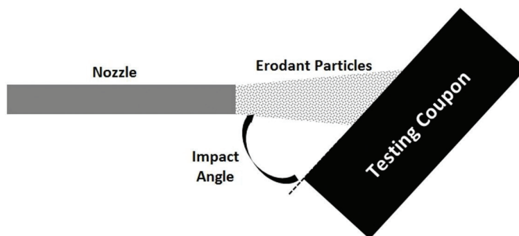
Figure 3. Schematic of erosion testing procedure according to the ASTM Standard G76 [35].
