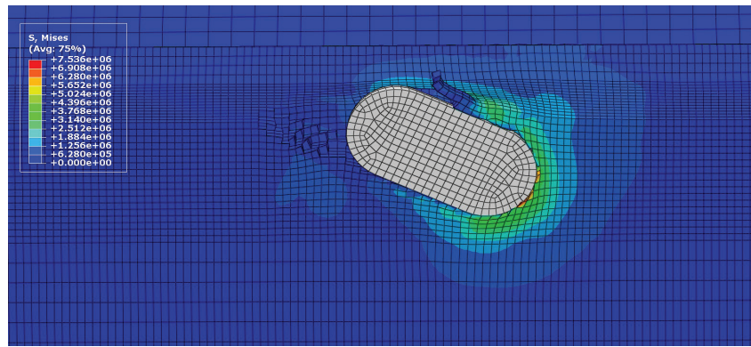
Figure 9. Material removal by cutting mechanism as predicted by the FE model [49].
