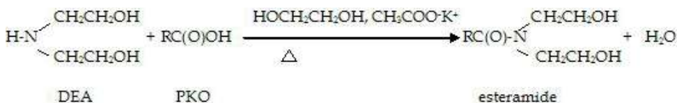
Scheme 2. Conversion of RBD PKO to the esteramide (RBD PKO-based polyol)
