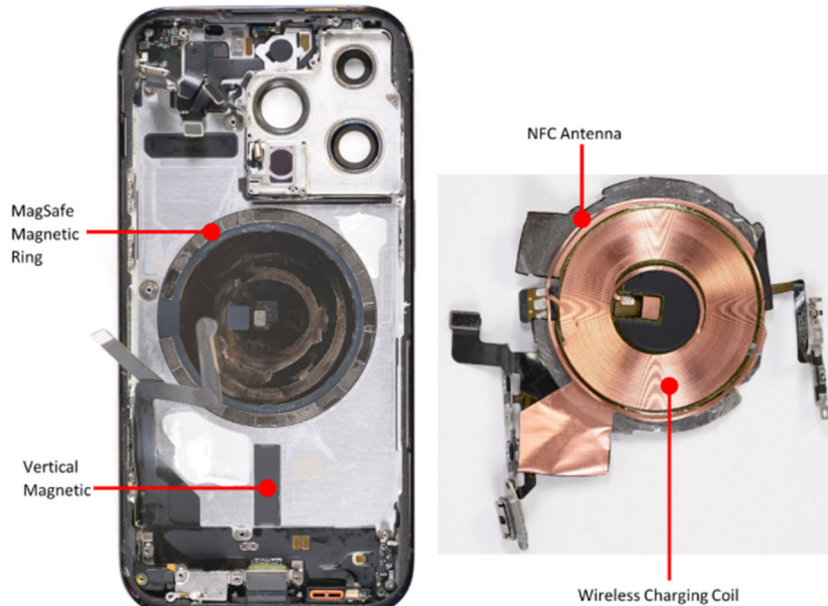
Figure 13: MagSafe system
