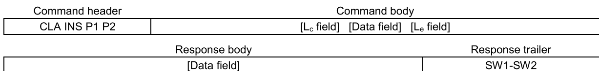
Figure 5 — Command-response pair
