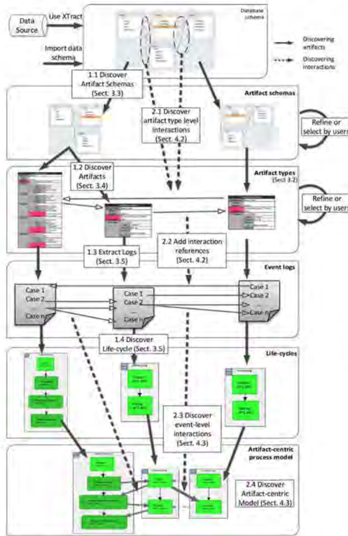
Fig. 4. An overview of our approach.
