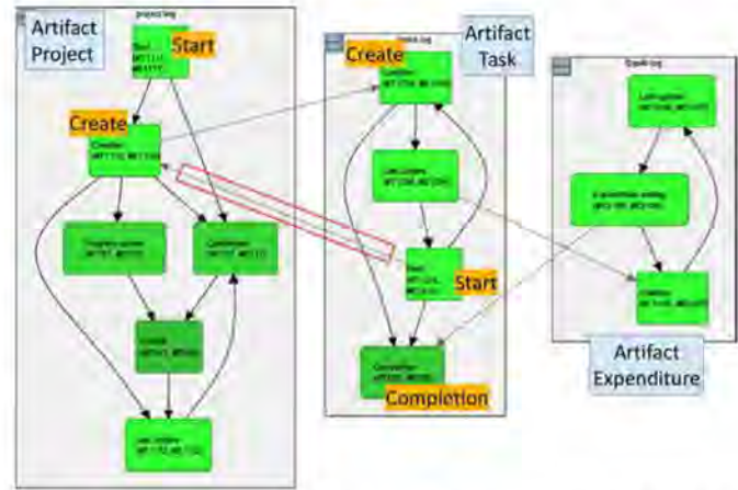
Fig. 15. A proclet system discovered by using the DF-max-EvTI classifier.
