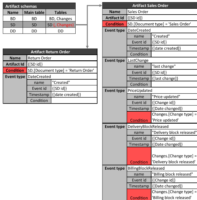
Fig. 5. The artifact schemas of Fig. 1(top left) and two artifact types derived from schema SD.
