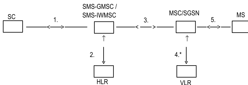
Figure 5: The main network structure serving as a basis for the short message transfer
