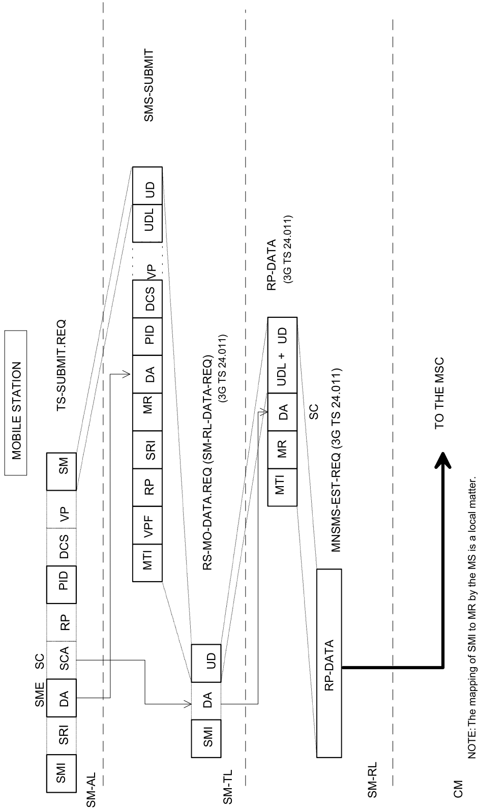
Figure C.9: Mobile originated short message
