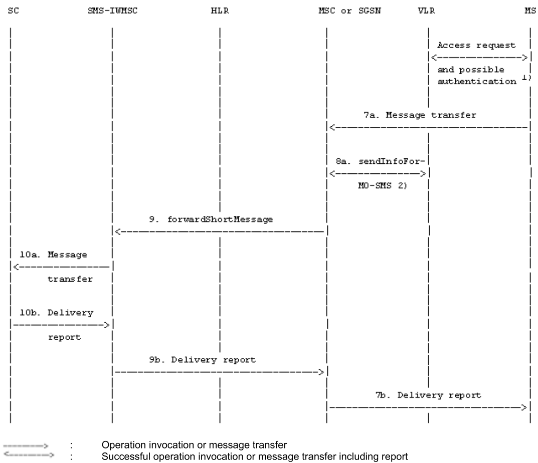
Figure 18a): Successful short message transfer attempt
