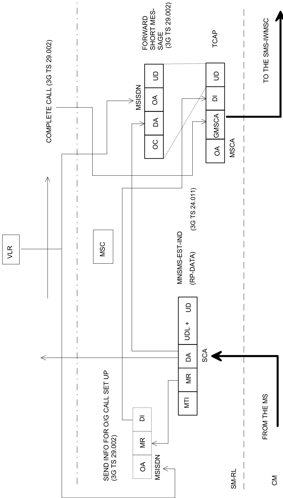
Figure C.10: Mobile originated short message
