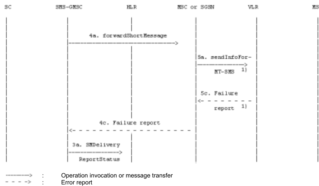
Figure 16b): "Send information for MT SMS" procedure; erroneous case: absent subscriber (e.g. IMSI DETACH or GPRS DETACH)
