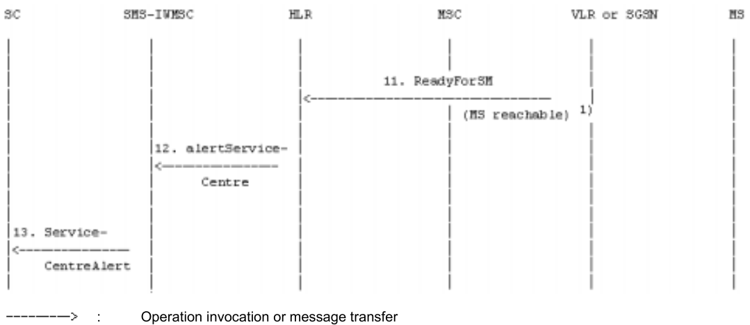
Figure 20a: The alert procedure when the MS becomes reachable, MNRG or both are set and MCEF is not set
