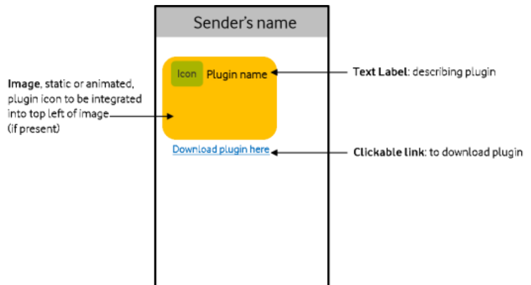
Figure 5: Example of a rich content bubble
