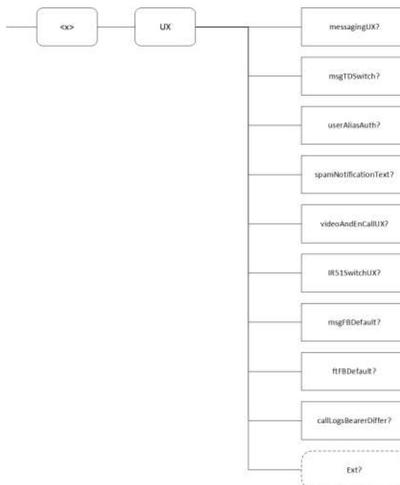
Figure 3: UX MO tree
