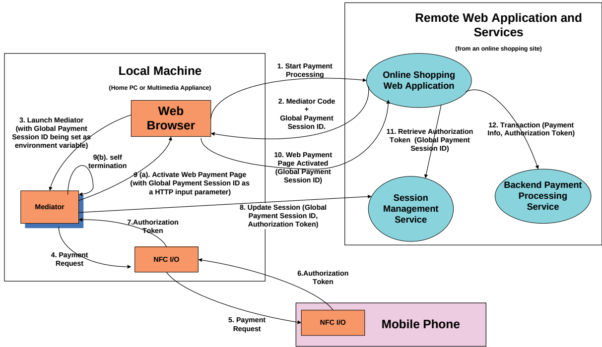
Figure 6. Remote web-based payment transactions enabled by local NFC.
