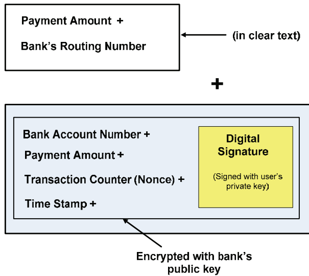
Figure 3. Payment authorization token issued from mobile phones.
