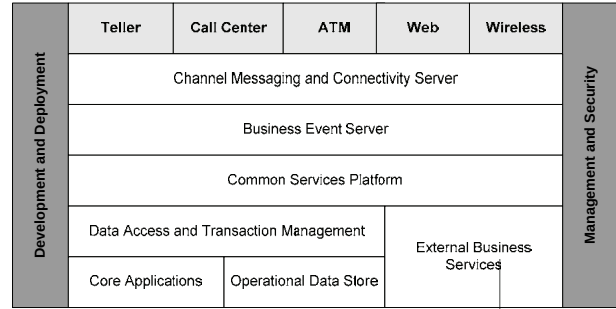
Figure 1. Adaptive Bank multiple channel applications and its layered infrastructure.
