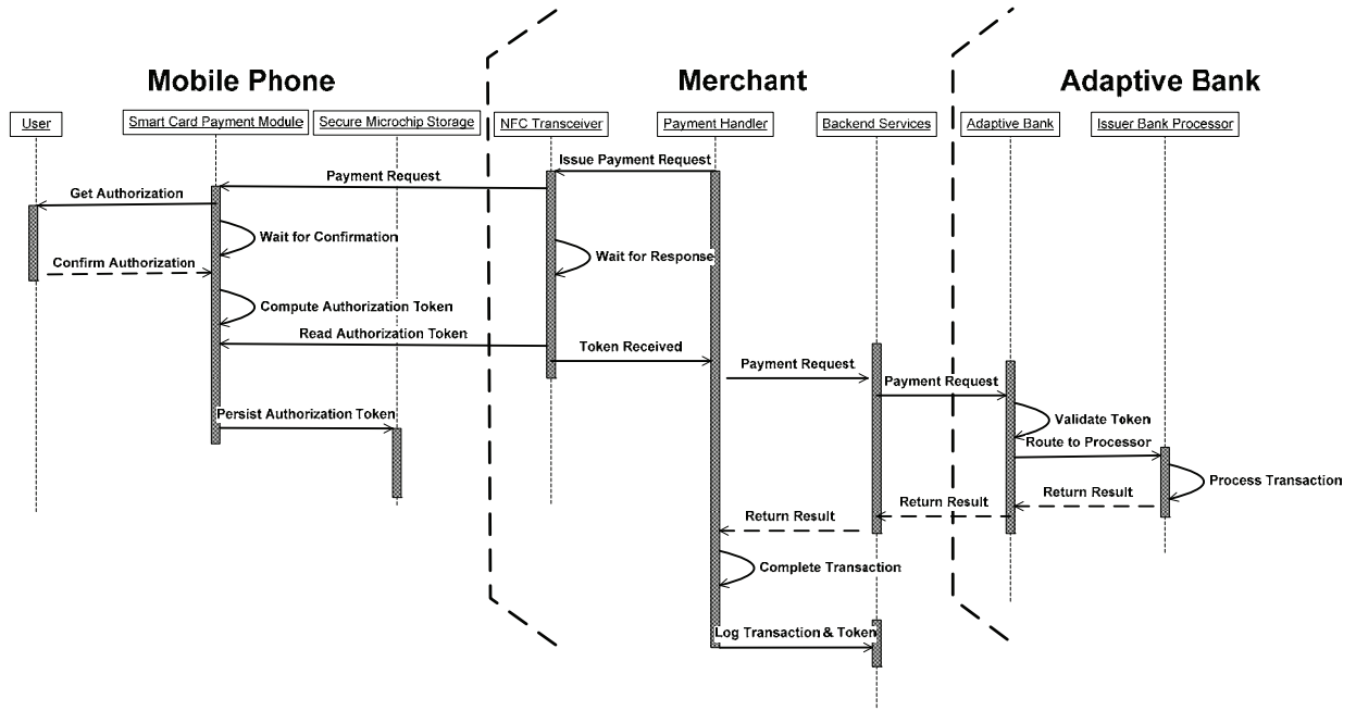
Figure 4. Sequence interaction on mobile phone, local machine and Adaptive Bank.
