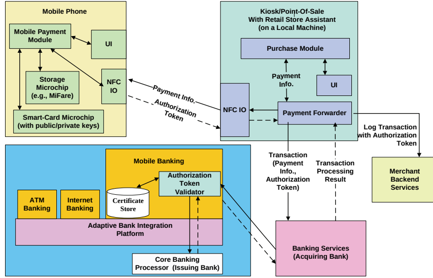
Figure 2. The overall NFC-enabled mobile payment system.
