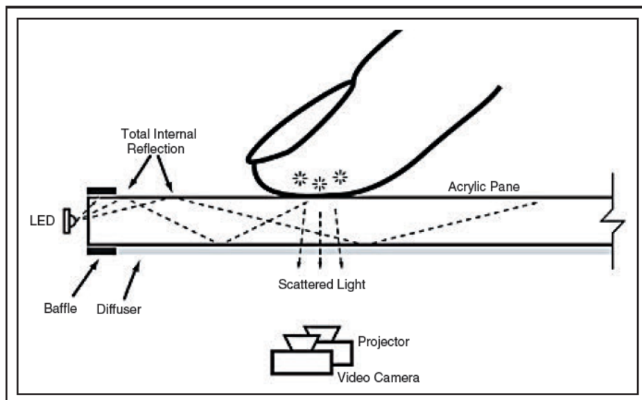
Fig. 4: A schematic representation of Perceptive Pixel's optical-touch technology based on frustrated total internal reflection. Illustration courtesy of Perceptive Pixel.
