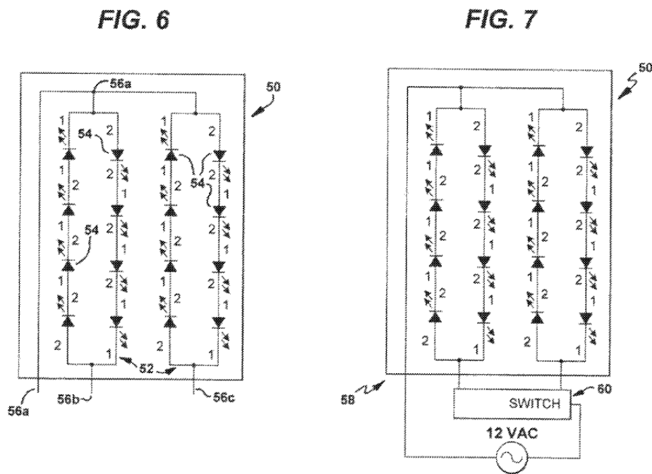
Figures 6 and 7 illustrate schematic diagrams of multi-voltage and/or multi-brightness LED lighting devices.
