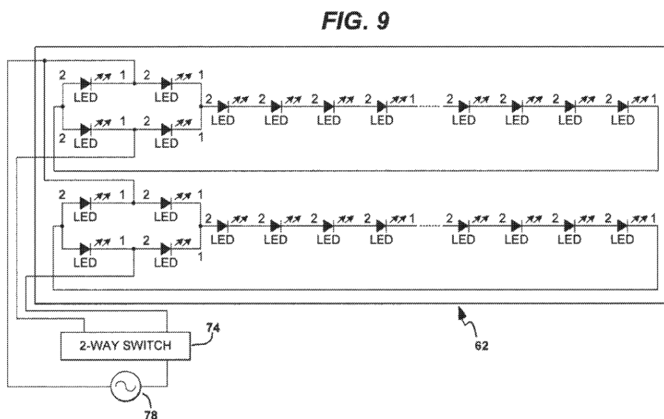
Figure 9 illustrates another schematic diagram of a multi-voltage and/or multi-brightness LED device
