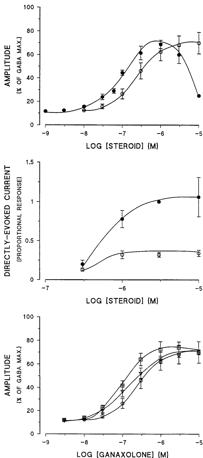
Fig. 3. Top and middle, concentration-response curves for ganaxolone (○) and 3\alpha,5\alpha -P (●) potentiation of GABA-evoked currents (top) or direct activation (middle) of GABA A receptors (human cloned \alpha 1 , \beta 1 and \gamma 2_L ) expressed in Xenopus oocytes. Bottom, concentration-response functions for ganaxolone enhancement of GABA-evoked currents recorded from oocytes expressing human recombinant \alpha 1\beta 1\gamma 2_L (○), \alpha 2\beta 1\gamma 2_L (□) or \alpha 3\beta 1\gamma 2_L (▽) GABA A receptors. Data are expressed as percent potentiation of current elicited by GABA (top and bottom) or response proportional to the current evoked by 3\ \mu\text{M} 3\alpha,5\alpha -P (middle). Each point represents the mean \pm S.E.M. of four to seven oocytes.
