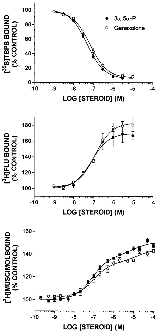
Fig. 2. Concentration-effect curves for inhibition of [^{35}\text{S}]\text{TBPS} binding (top) or enhancement of [^3\text{H}]\text{flunitrazepam} binding (middle) or [^3\text{H}]\text{muscimol} binding (bottom) by ganaxolone and 3\alpha,5\alpha\text{-P} in rat brain cortical membranes. Each point represents the mean \pm S.E.M. of at least three independent experiments.
