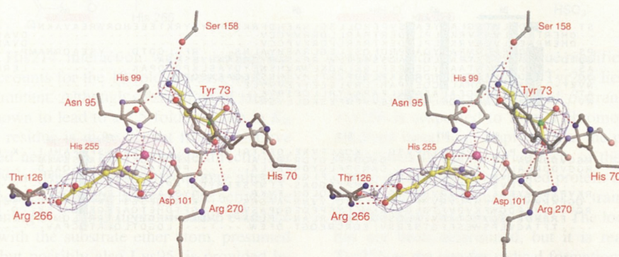
FIGURE 4: Stereodiagram of the active site of TauD. Shown are the protein ligands to the iron, the two substrates and other important protein side-chains. A 2mF_o - DF_c electron density map is shown contoured at 1.0 sigma around the substrate molecules.
