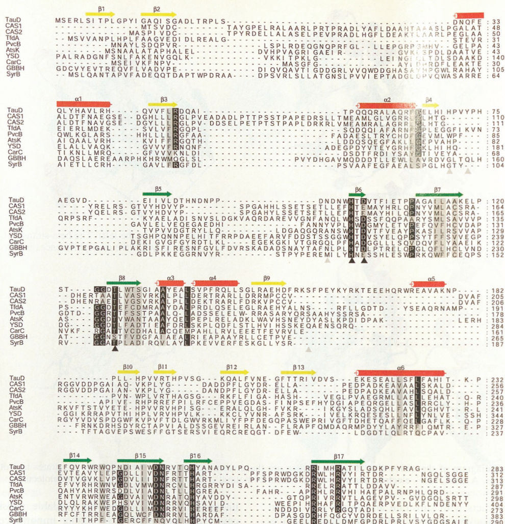
FIGURE 5: Secondary structure based sequence alignment of the group II (10) \alpha KG-dependent dioxygenases. An initial alignment was produced based on a 3D alignment of CAS1 (PDB ID: 1D9Y) and TauD. The other sequences were then aligned to the existing alignment. The sequences (with Swiss-Prot accession numbers) are TauD, E. coli taurine/ \alpha KG dioxygenase (P37610); CAS1, CAS2, Streptomyces clavuligerus clavamate synthase 1 and 2 (Q05581 and Q05582); TfdA, Ralstonia eutropha 2,4-D/ \alpha KG dioxygenase (P10088); PvcB, Pseudomonas aeruginosa pyoverdine biosynthesis enzyme (O30371); AtsK, Pseudomonas putida alkyl sulfate/ \alpha KG dioxygenase (Q9WWU5); YSD, Saccharomyces cerevisiae sulfonate/ \alpha KG dioxygenase (Q12358); CarC, Erwinia carotovora carbapenam biosynthesis enzyme (Q9XB59); GBBH, Pseudomonas sp. \gamma -butyrobetaine hydroxylase (P80193); SyrB, Pseudomonas syringae syringomycin biosynthesis enzyme I (P97053). The TauD secondary structure is colored red for helix, green for \beta -strands of the jellyroll motif, and yellow for other \beta -strands. Conserved Fe(II)- and \alpha KG-binding ligands are marked with black triangles. Taurine-binding ligands within TauD are marked below the alignments with gray triangles. Produced using Alscript (46).
