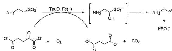
Scheme 1: Reaction Catalyzed by TauD
