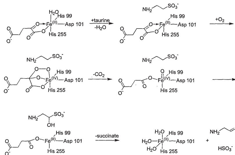
Scheme 2: Proposed Mechanism of TauD
