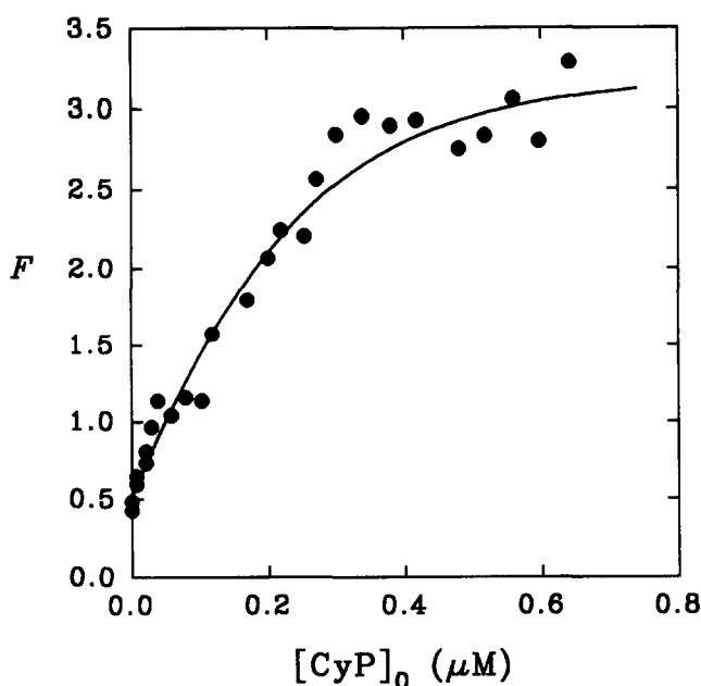
Fig. 1. Fluorescence intensities observed in the competitive binding of cyclosporin A (CsA) and [p\text{-Lys(Dns)}]_8\text{-CsA} to cyclophilin. The concentrations of [p\text{-Lys(Dns)}]_8\text{-CsA} and CsA are 0.2 \mu\text{M} and 0.5 \mu\text{M} , respectively. The dissociation constant for [p\text{-Lys(Dns)}]_8\text{-CsA} was kept constant ( 5.3 \text{ nM} ). The curve represents the best fit to eq. 17.
